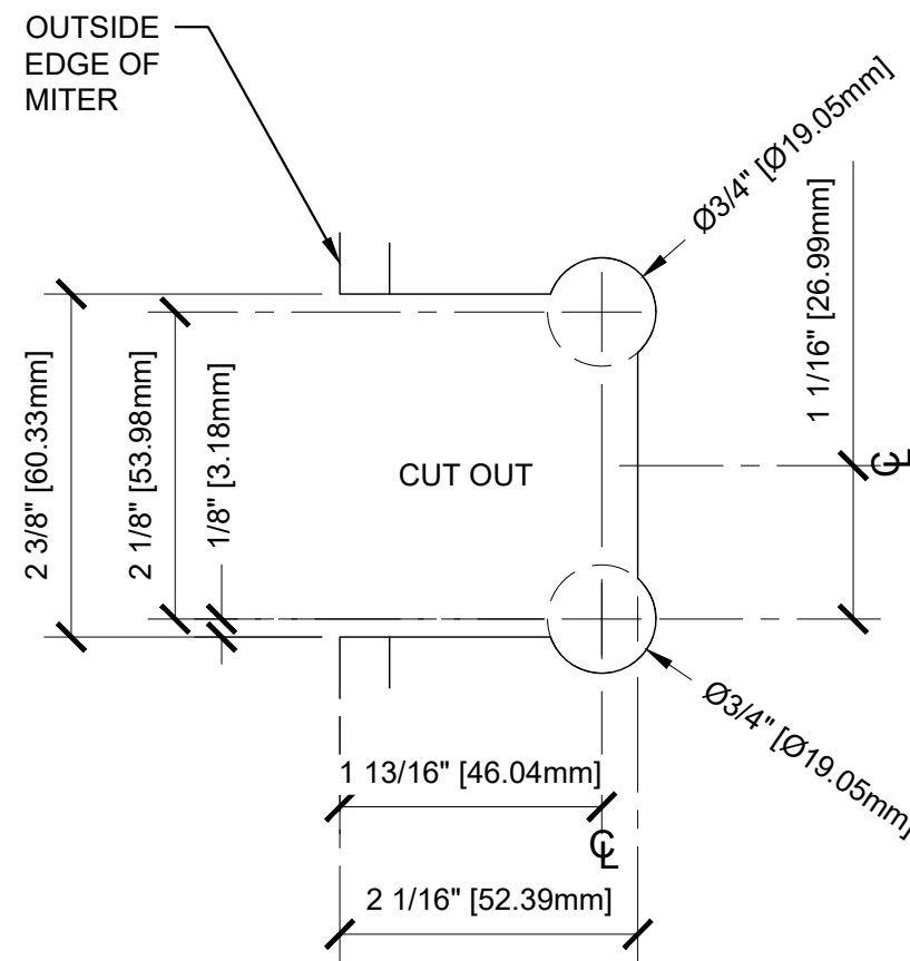
GLASS FABRICATION 45° MITERED FIXED PANEL
