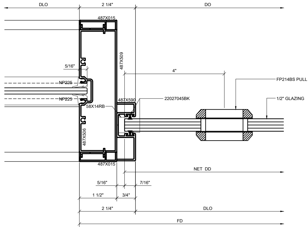
1 SERIES 487 OPS INTEGRATED SLIDER TRANSITION VERTICAL-STANDARD TO STRIKE JAMB (CLOSED)
