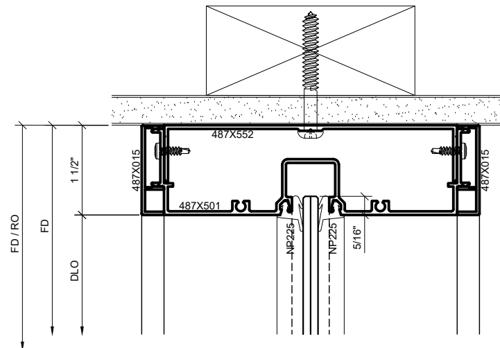
2 SERIES 487 OPS SURFACE MOUNT HEAD DETAIL AT SIDELITE (NO SHIM) 1'-0"=1'-0" ARCH REF: N/A
