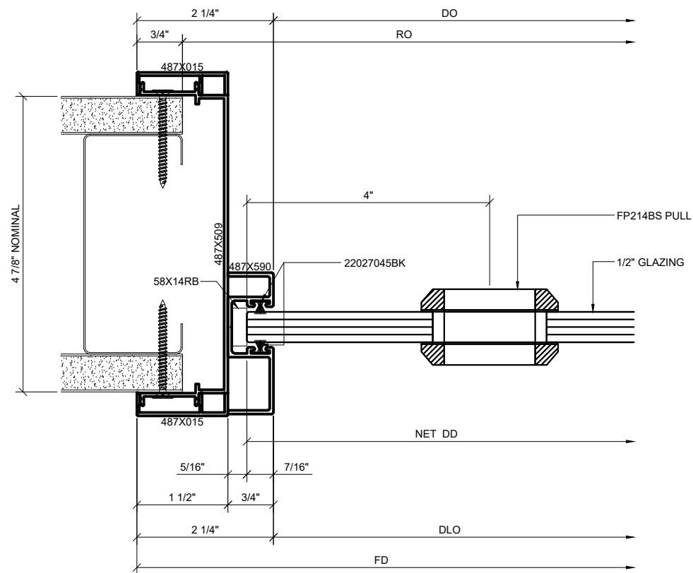
① SERIES 487 OPS INTEGRATED SLIDER STRIKE JAMB DETAIL (CLOSED) 1'-0"=1'-0" ARCH REF: N/A
