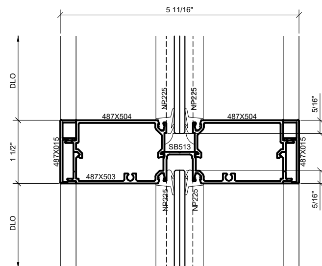
4 SERIES 487 OPS FULL HORIZ. MUNTIN AT SIDELITE 1'-0"=1'-0" ARCH REF: N/A
