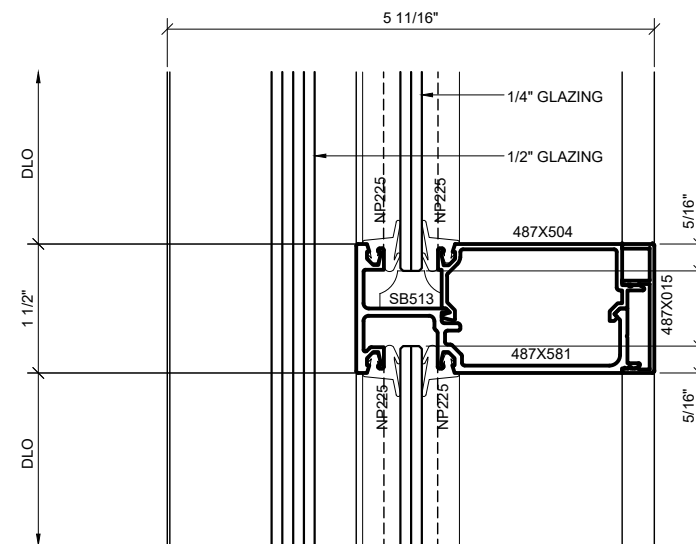
6 HORIZONTAL MUNTIN DETAIL AT SLIDER BAY
