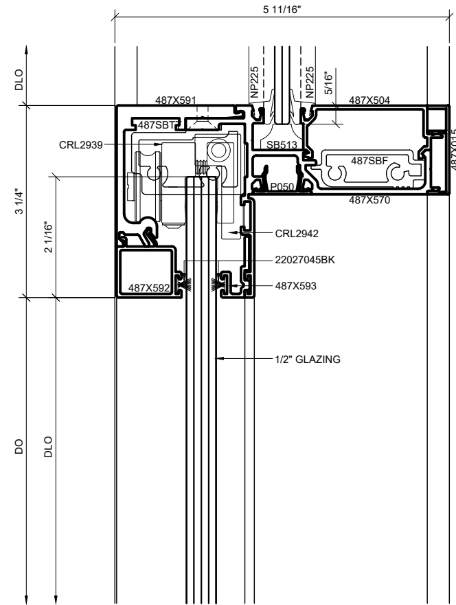
3 HEAD DETAIL AT SLIDER DOOR OPENING WITH TRANSOM
