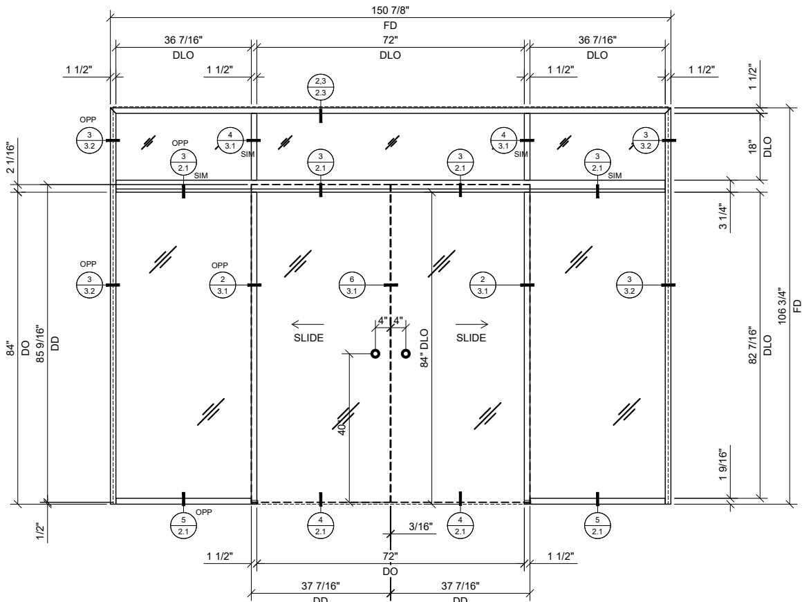
② BI-PART SLIDER WITH BAY & TRANSOM 3/4"=1'-0" ARCH REF: N/A
