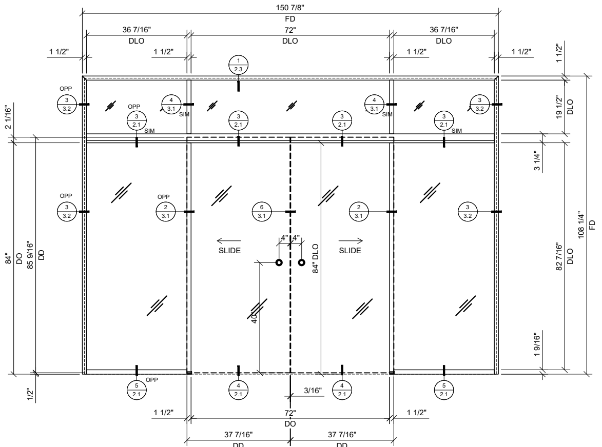
2 BI-PART SLIDER WITH BAY & TRANSOM 3/4\"=1'-0\" ARCH REF: N/A
