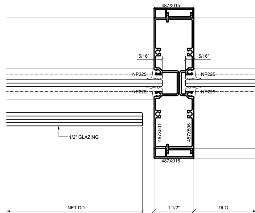
④ SERIES 487 OPS INTEGRATED SLIDER TRANSITION VERTICAL-SLIDER TO STANDARD (OPEN) 1'-0"=1'-0" ARCH REF: N/A
