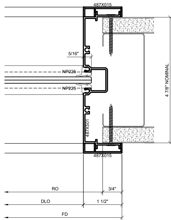
3 SERIES 487 OPS STANDARD JAMB DETAIL
