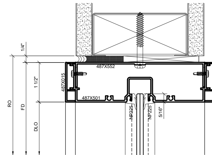
3 SERIES 487 OPS SURFACE MOUNT HEAD DETAIL AT SIDELITE (w/ SHIM) 1'-0"=1'-0" ARCH REF: N/A
