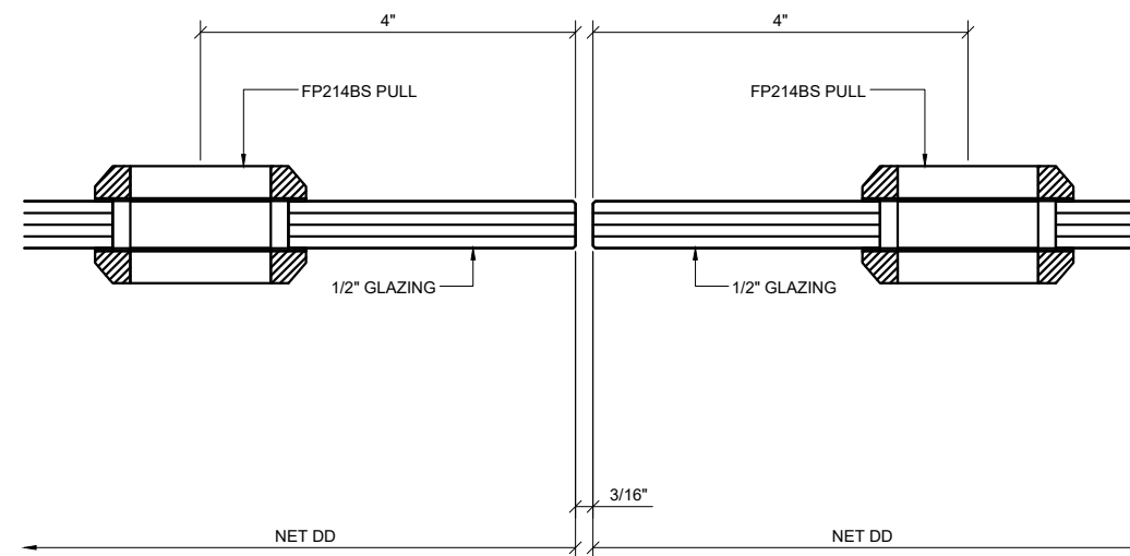
⑥ SERIES 487 OPS INTEGRATED SLIDER MEETING STILES AT DOOR PAIR DETAIL 1'-0"=1'-0" ARCH REF: N/A
