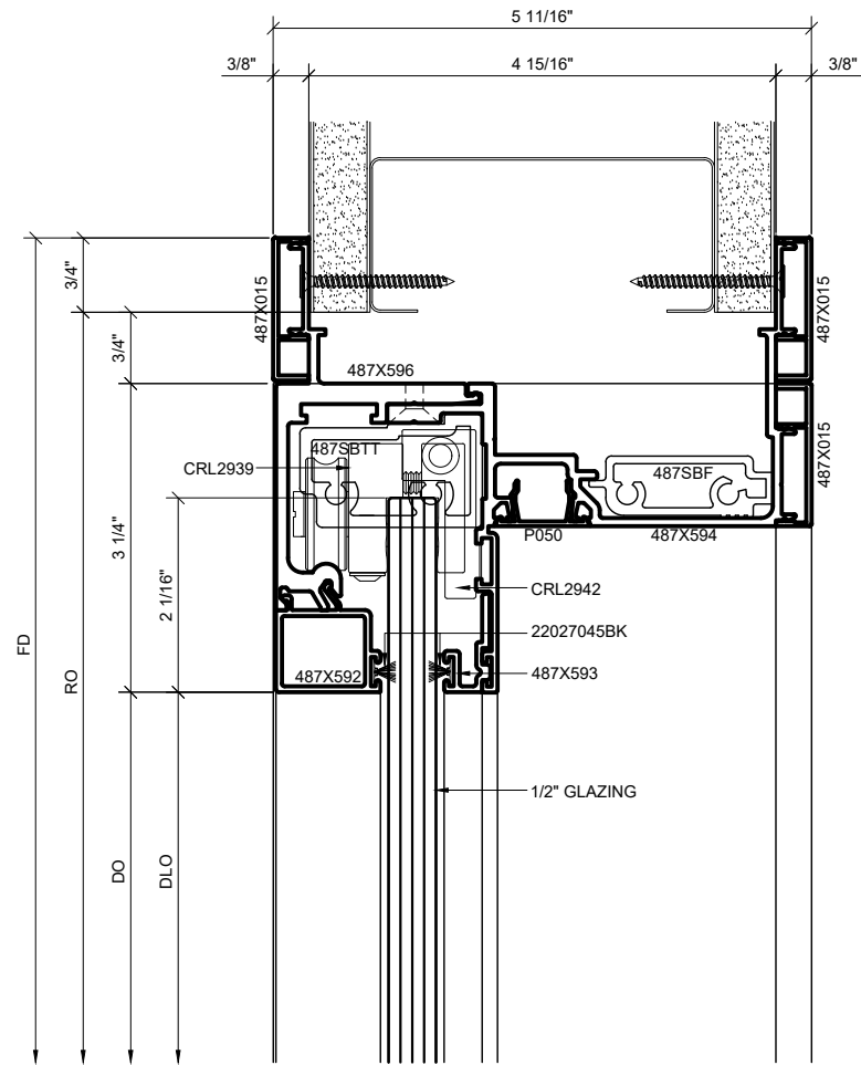
1 WALL-WRAPPED HEAD DETAIL AT SLIDER DOOR OPENING
