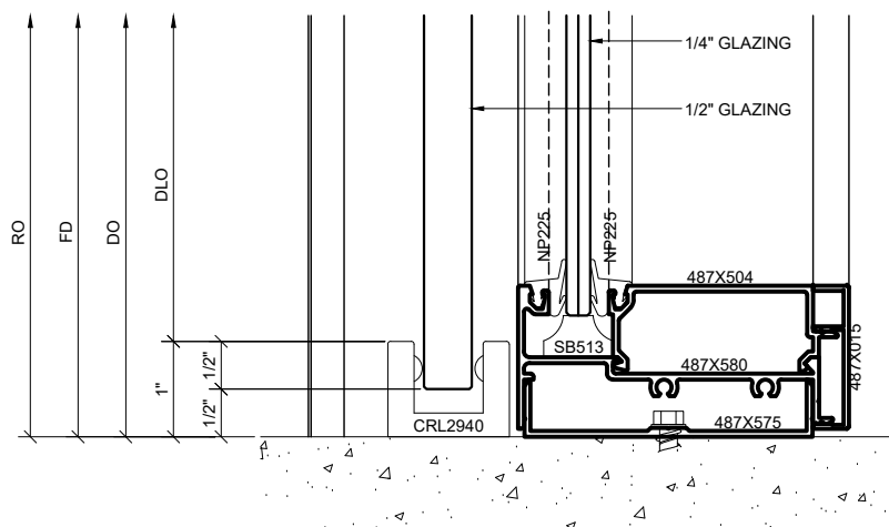
5 SILL DETAIL AT SLIDER SIDELITE
