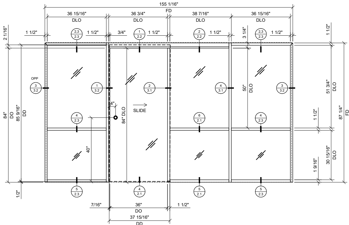
3 SINGLE SLIDER WITH BAY & SIDELITE AT EACH END 3/4"=1'-0" ARCH REF: N/A
