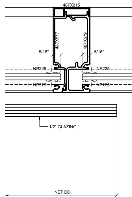
⑤ SERIES 487 OPS INTEGRATED SLIDER SHALLOW INTERMEDIATE VERTICAL DETAIL (OPEN) 1'-0"=1'-0" ARCH REF: N/A
