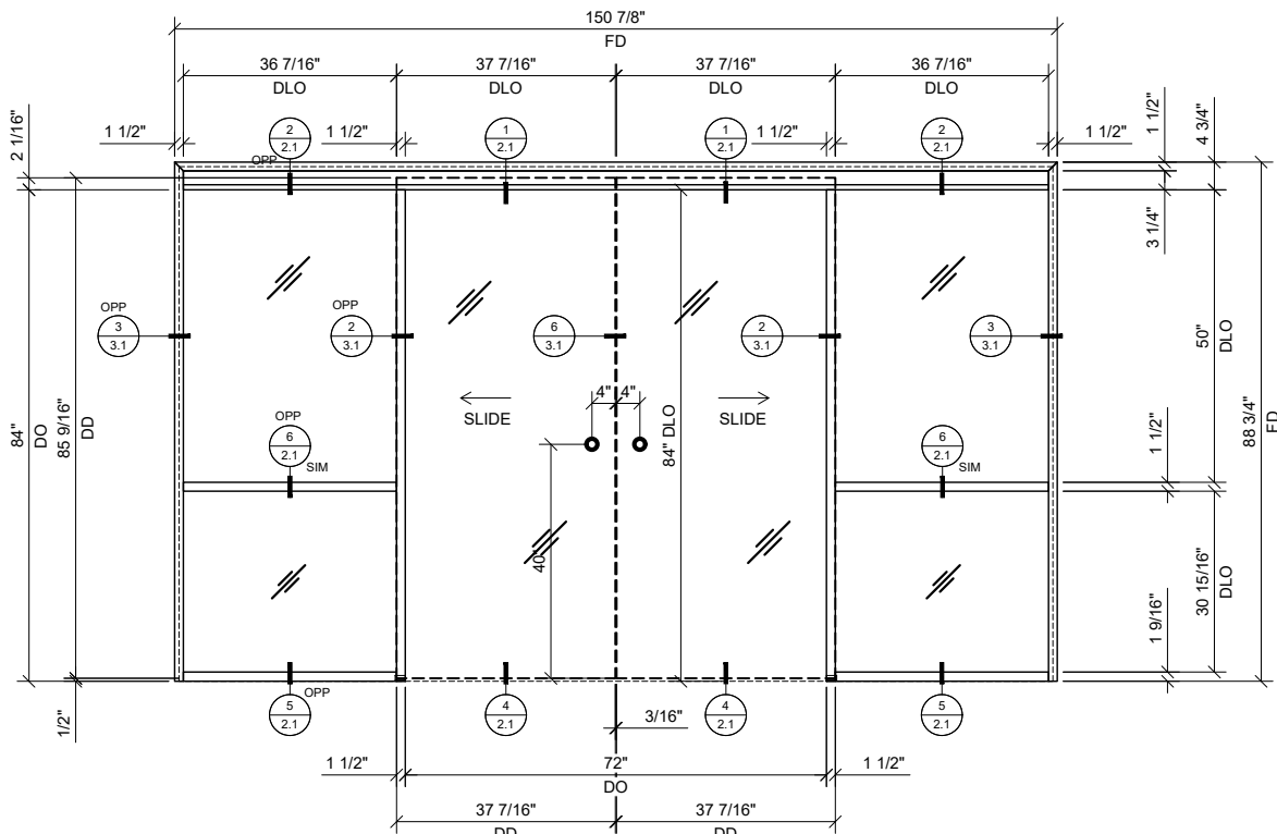
1 BI-PART SLIDER WITH BAY 3/4\"=1'-0\" ARCH REF: N/A
