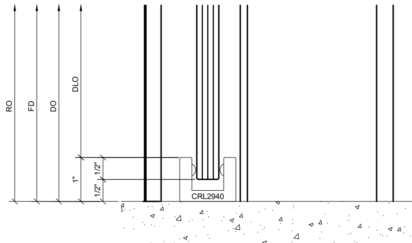
4 SILL DETAIL AT SLIDER DOOR OPENING
