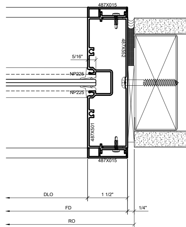
4 SERIES 487 OPS DETAIL FOR SURFACE MOUNT AT JAMBS
