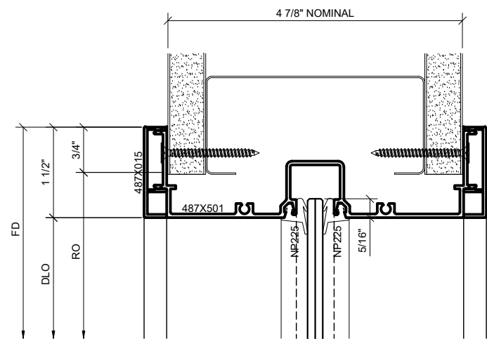
1 SERIES 487 OPS WALL WRAP HEAD DETAIL AT SIDELITE OR TRANSOM 1'-0"=1'-0" ARCH REF: N/A
