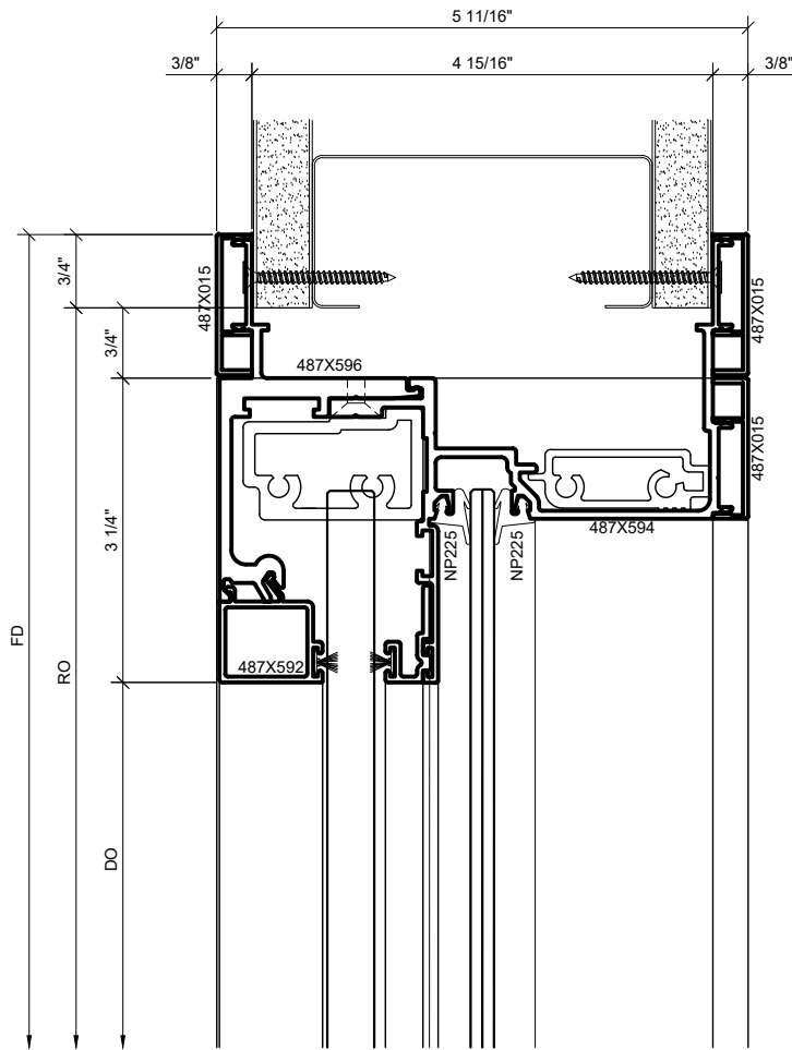
2 WALL-WRAPPED HEAD DETAIL AT SLIDER SIDELITE
