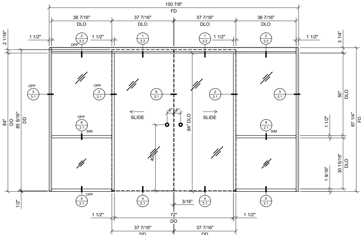
① BI-PART SLIDER WITH BAY 3/4"=1'-0" ARCH REF: N/A
