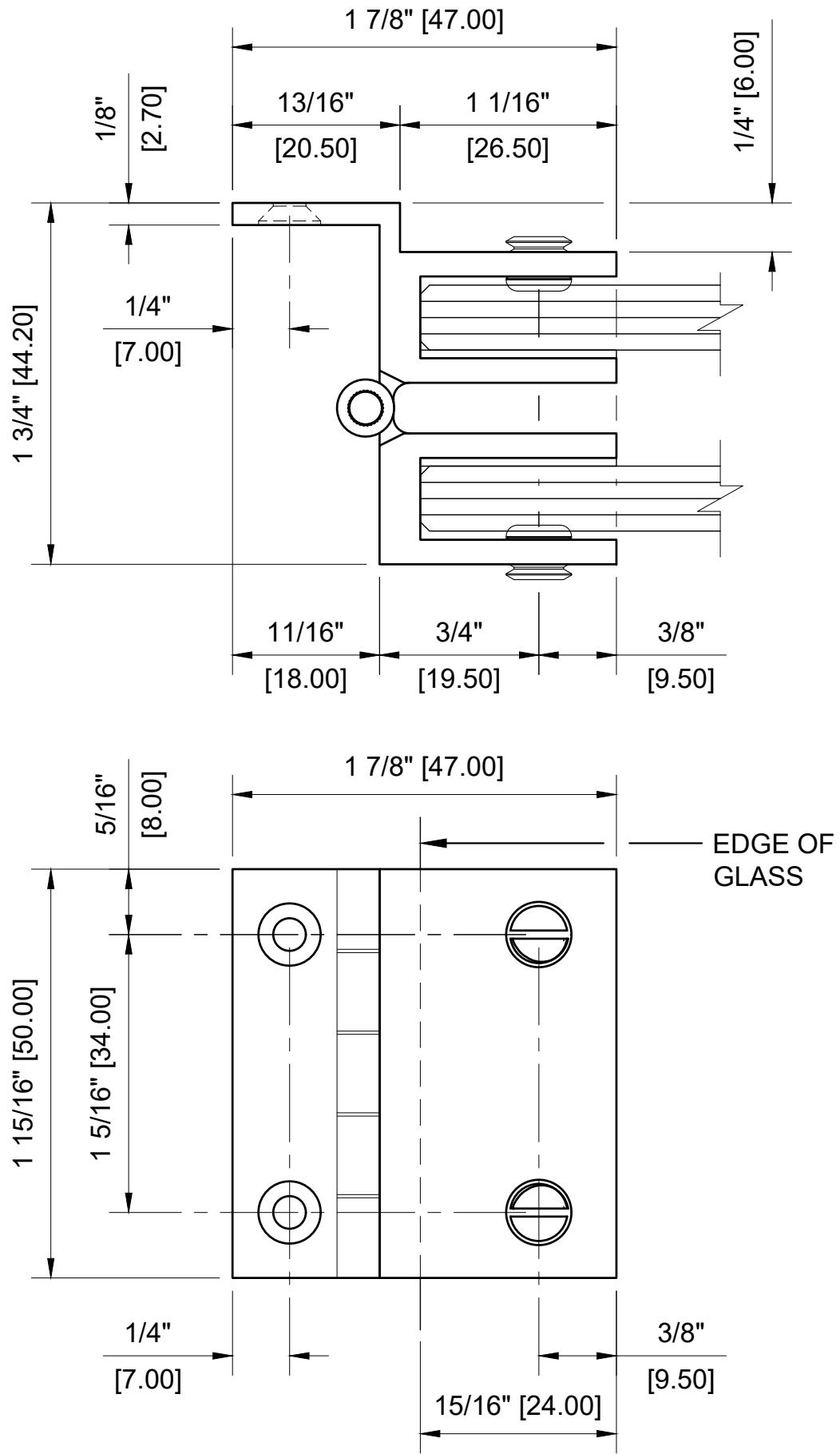
CRL - EH66 CHROME FRAMELESS MIRROR TRIPLE HINGE FOR 1/4" - 5/16" GLASS
