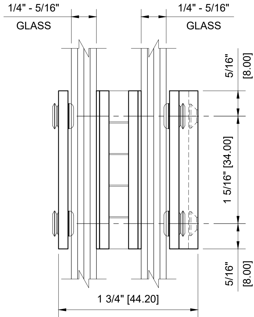
CRL - EH66 CHROME FRAMELESS MIRROR TRIPLE HINGE FOR 1/4" - 5/16" GLASS
