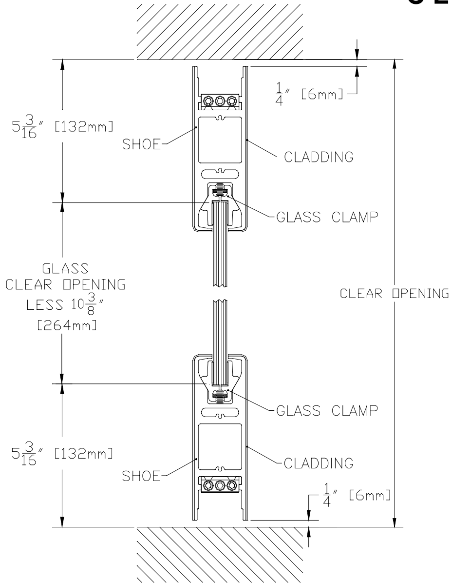
6" SQUARE DOOR RAIL TOP AND BOTTOM CLAD ONLY
