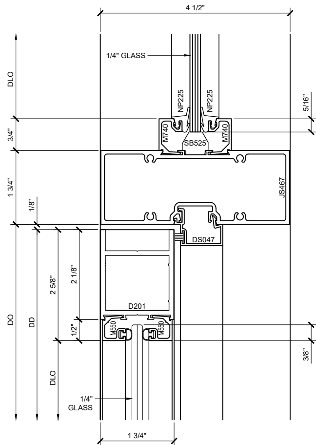
SECTION DETAIL AT CONTINUOUS DOOR HEADER FOR OFFSET DOOR WITH SMC ⑦
