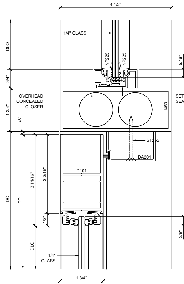
SECTION DETAIL AT CONTINUOUS DOOR HEADER FOR OFFSET DOOR WITH OHCC ⑨
