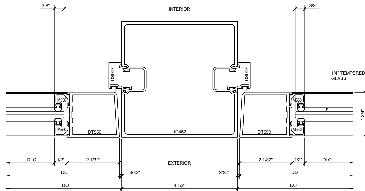
SECTION DETAIL AT INTERMEDIATE VERTICAL ⑥
