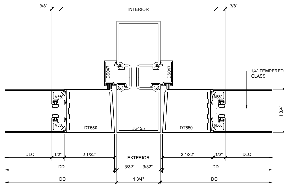
SECTION DETAIL AT INTERMEDIATE VERTICAL (6)
