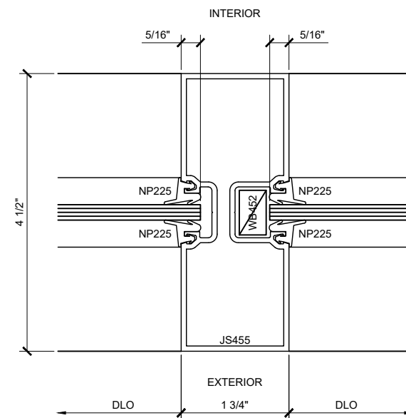
SECTION DETAIL AT INTERMEDIATE VERTICAL (6)
