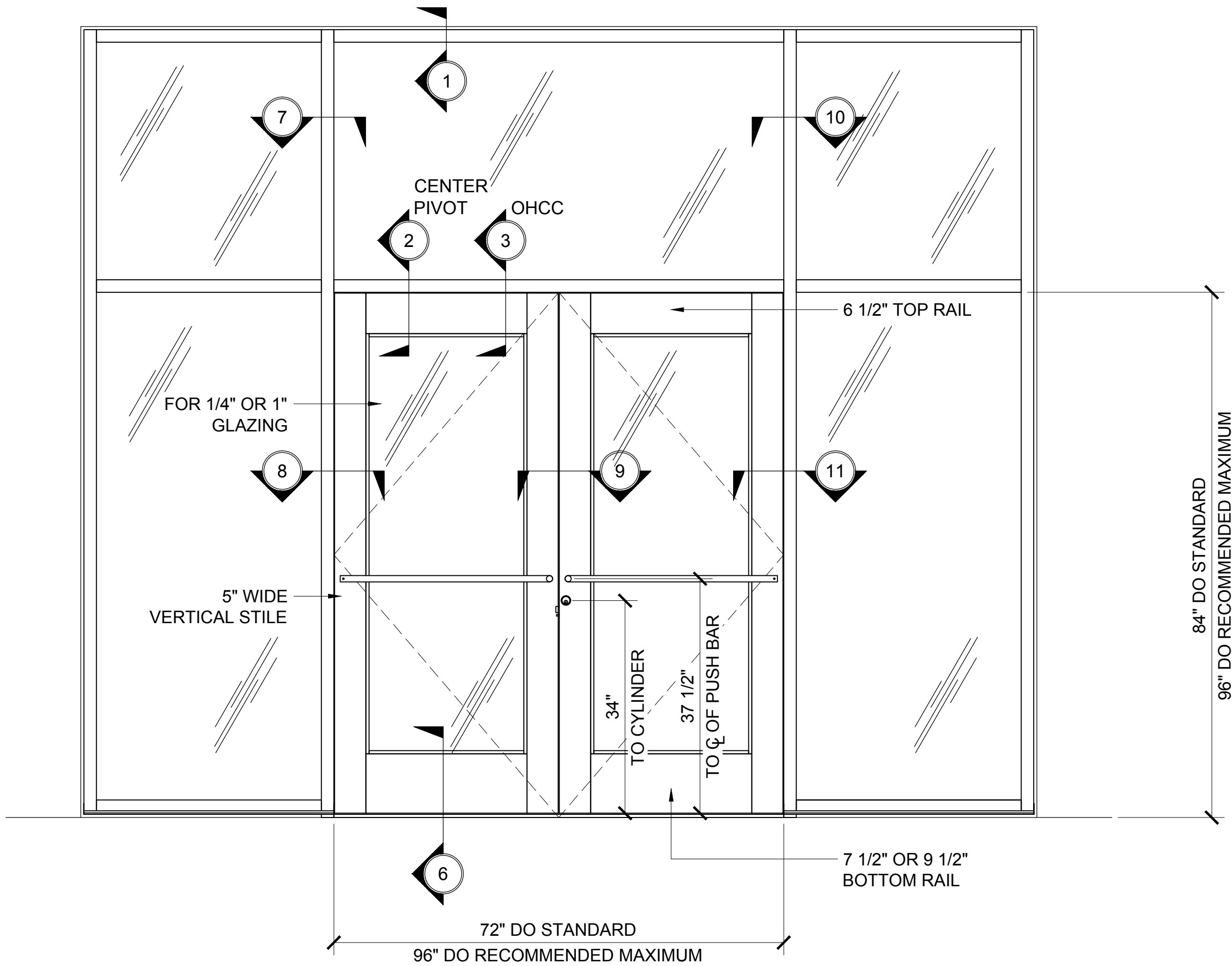
CENTER-HUNG WIDE STILE SERIES 550 DOOR ADA COMPLIANT ELEVATION
