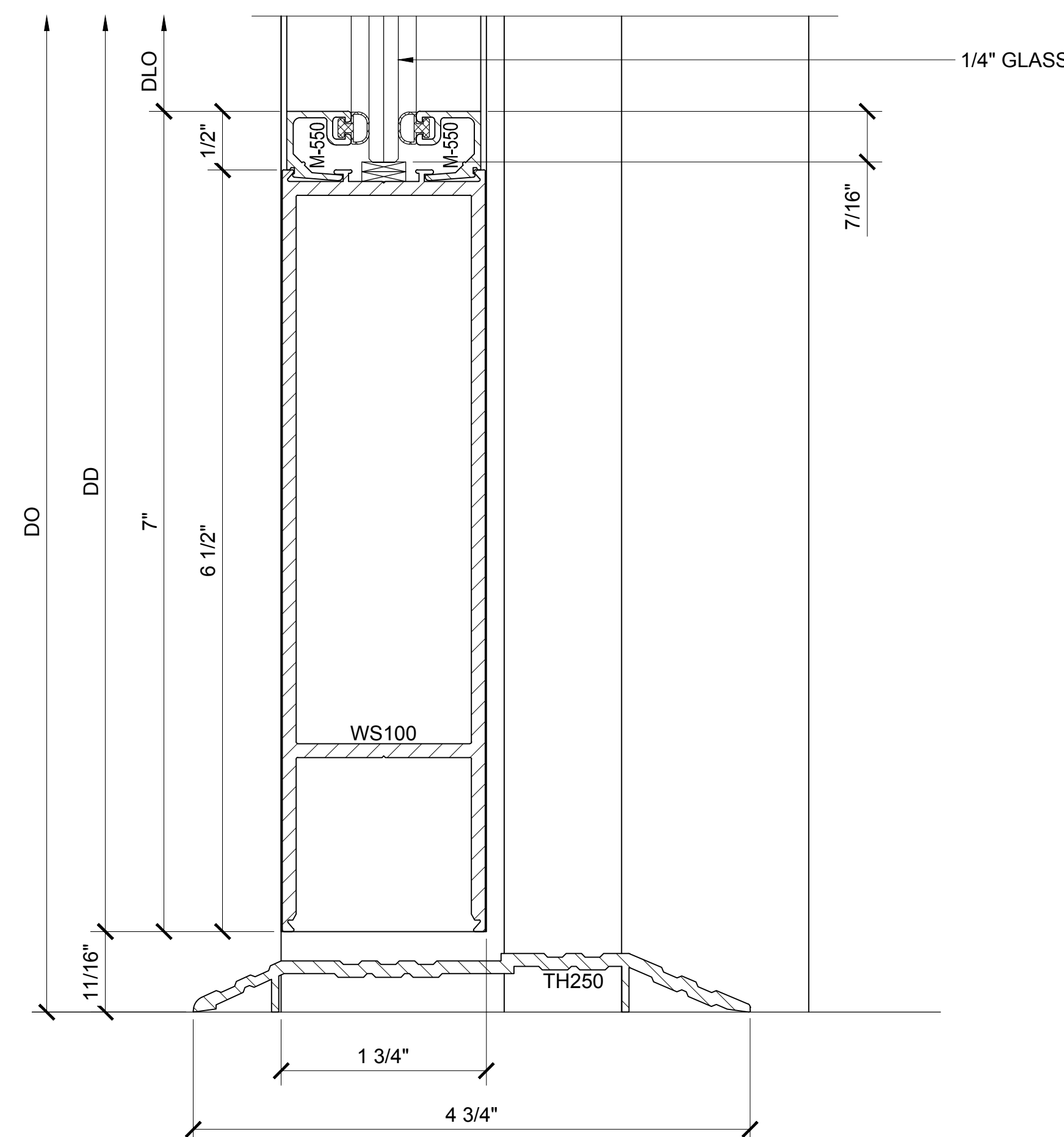
SECTION DETAIL @ DOOR SILL 15
