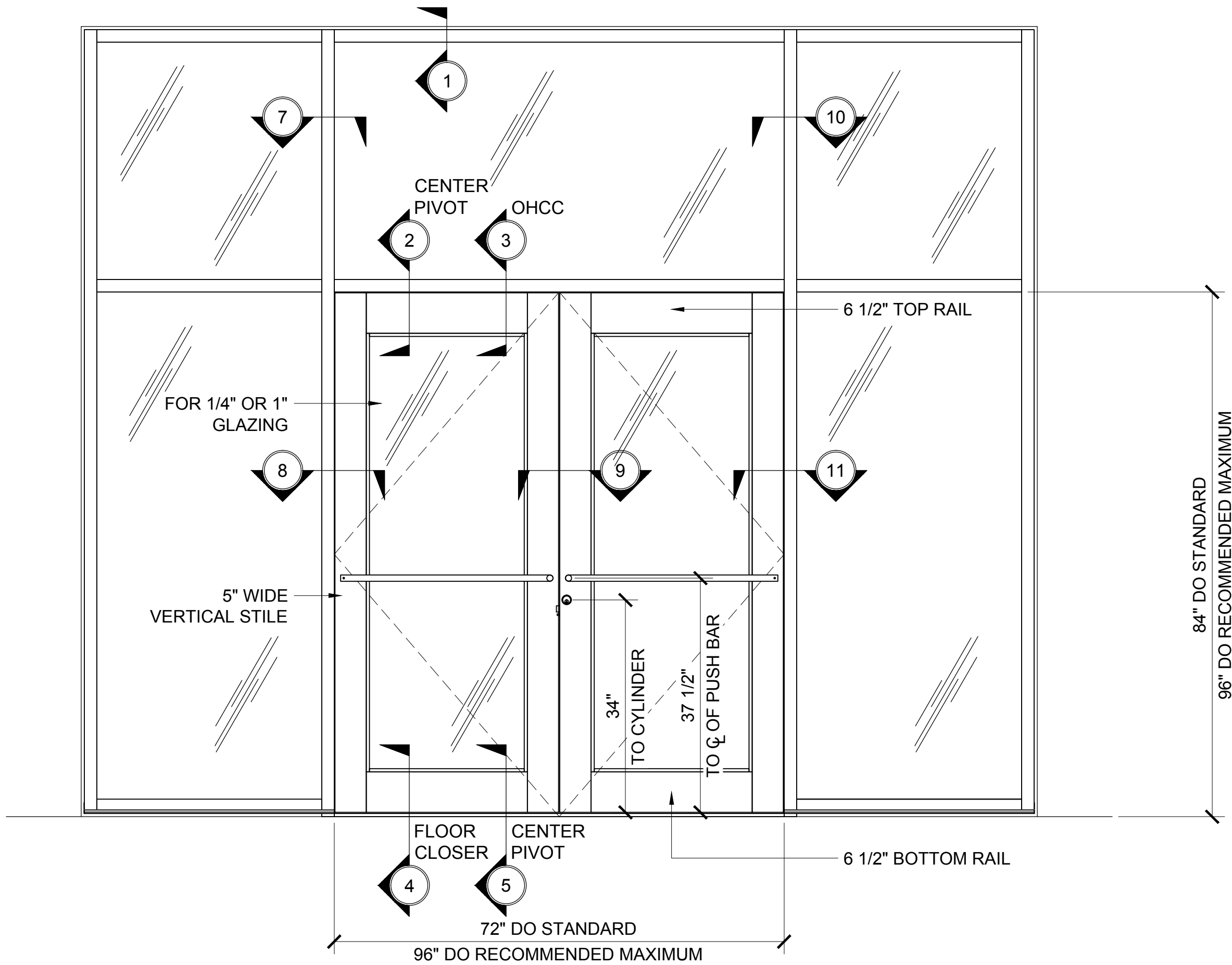
CENTER-HUNG WIDE STILE SERIES 550 DOOR TYPICAL ELEVATION
