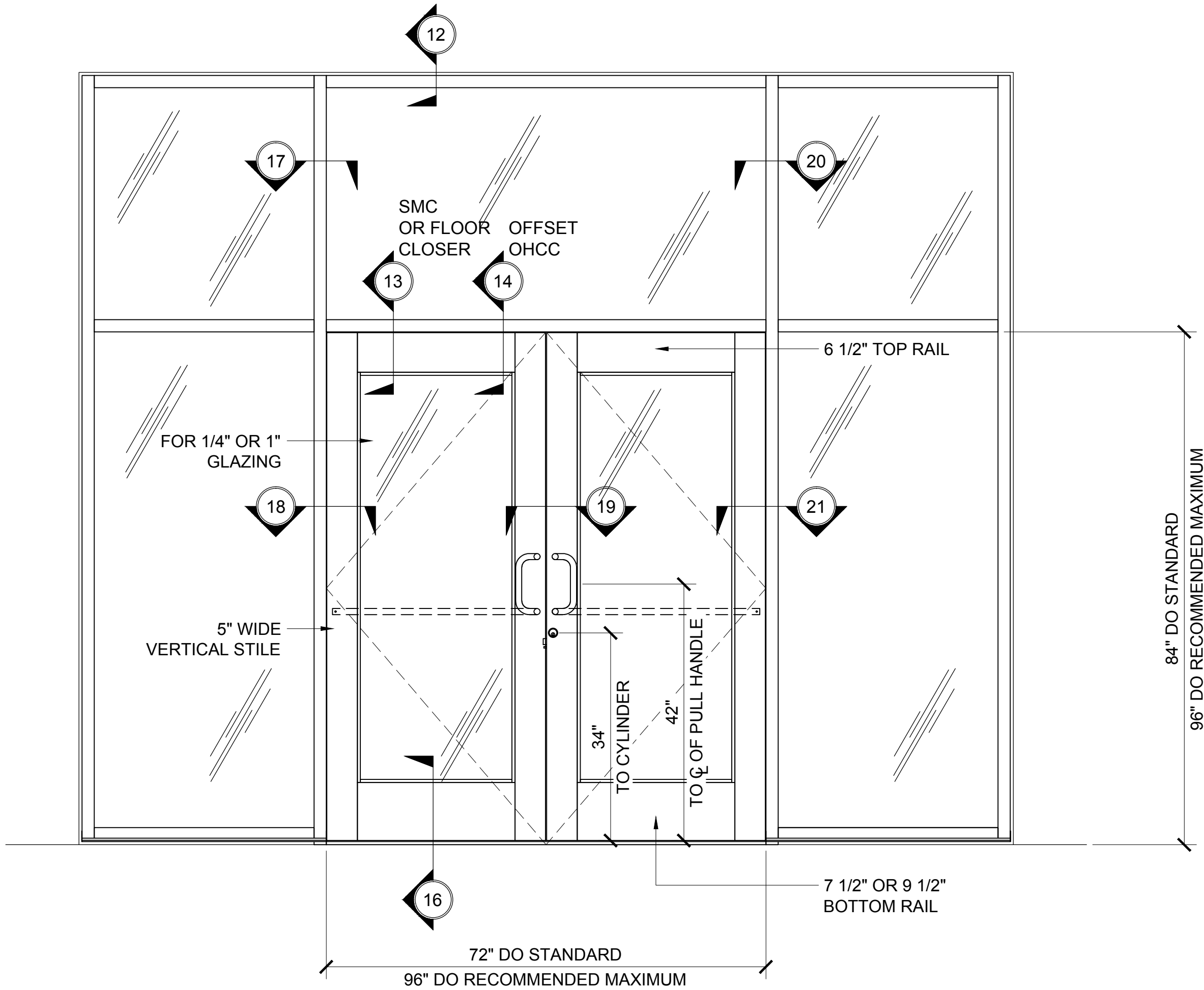
OFFSET-HUNG WIDE STILE SERIES 550 DOOR ADA COMPLIANT ELEVATION
