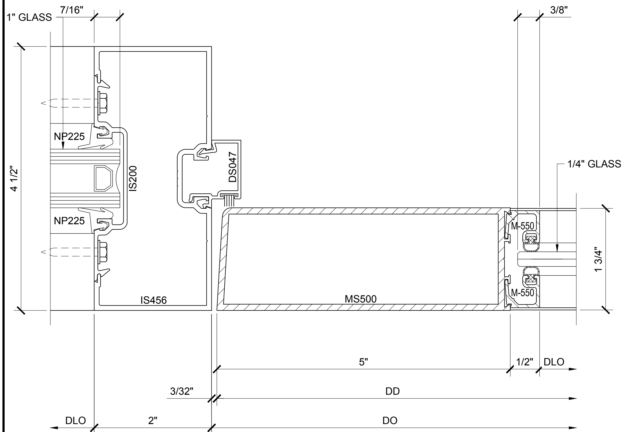
SECTION DETAIL @ DOOR JAMB 18
