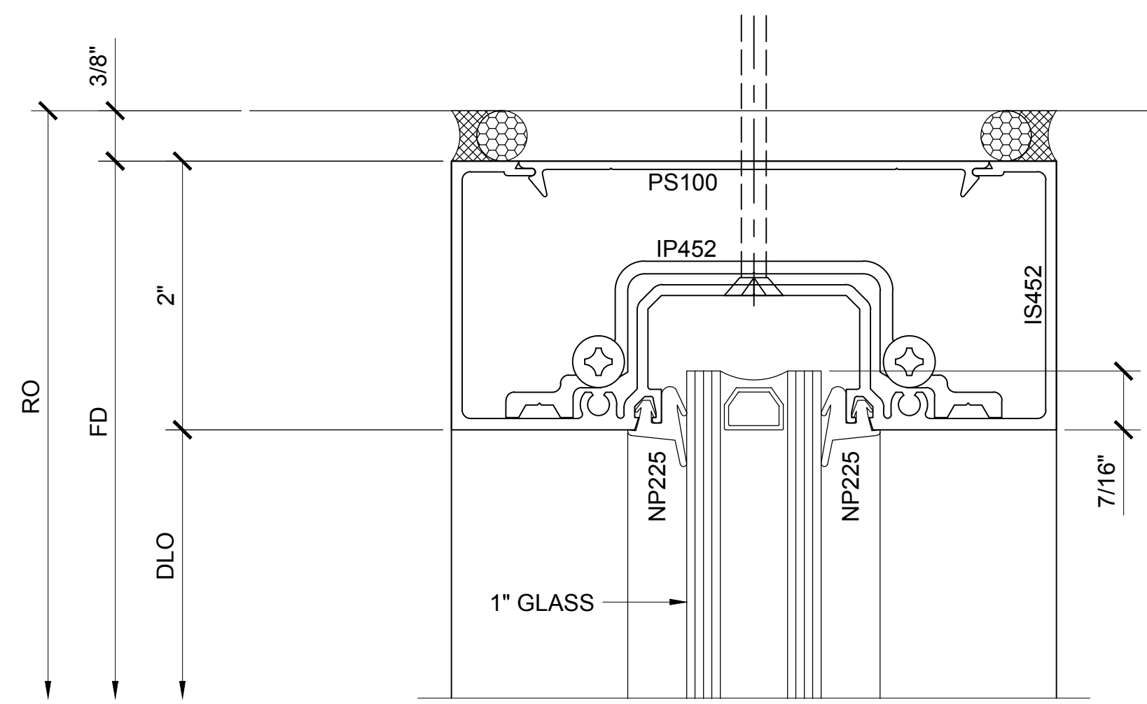
SECTION DETAIL @ STOREFRONT HEAD 12
