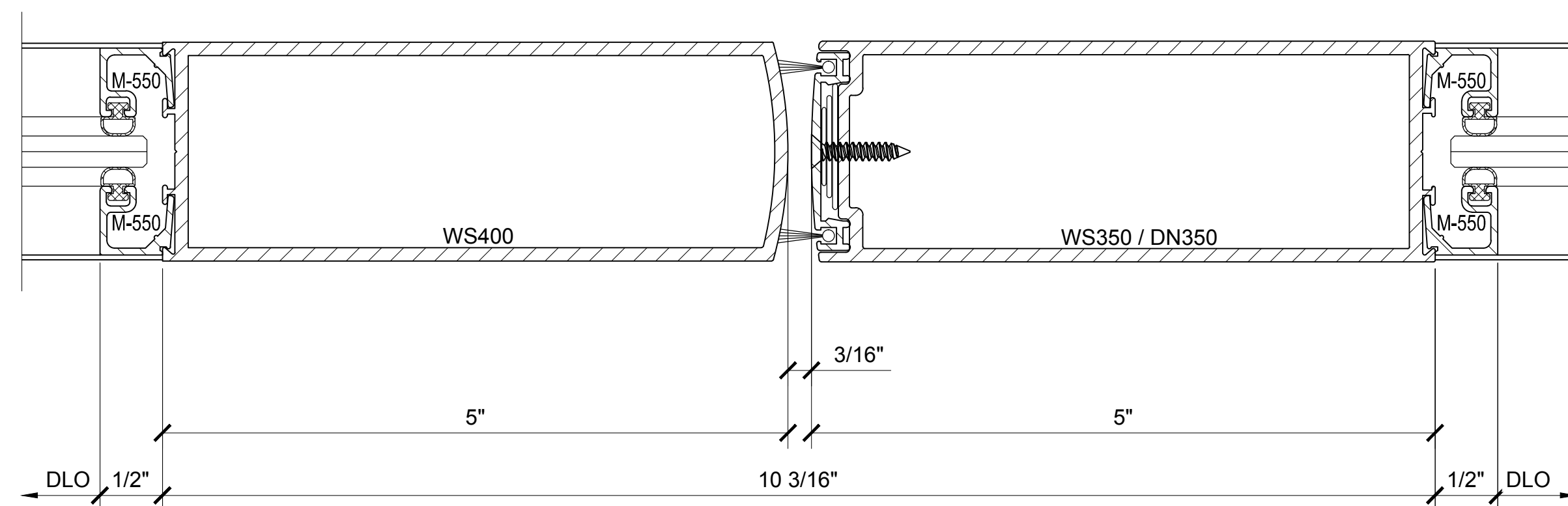
SECTION DETAIL @ MEETING STILES
