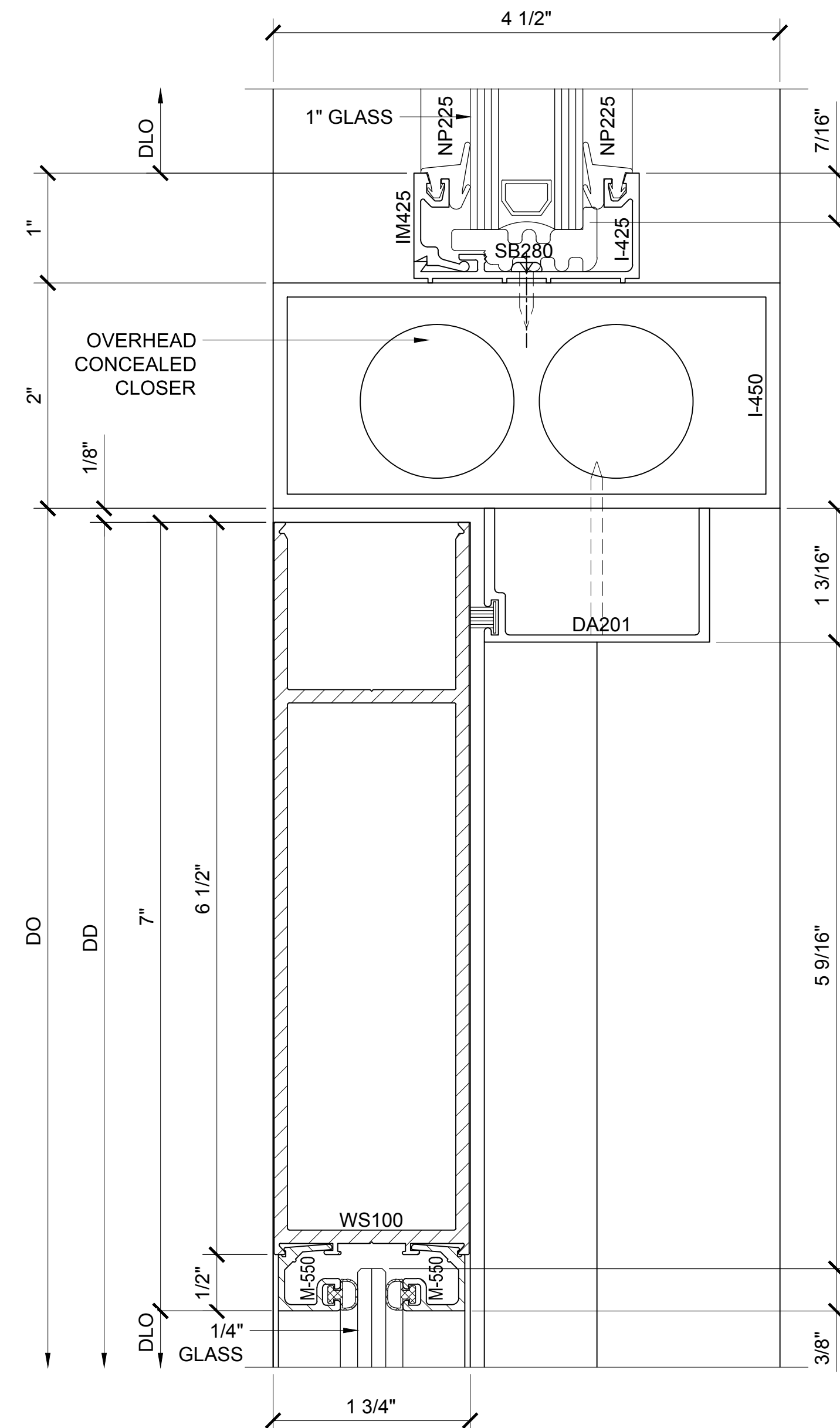
SECTION DETAIL @ DOOR HEAD WITH OHCC 14
