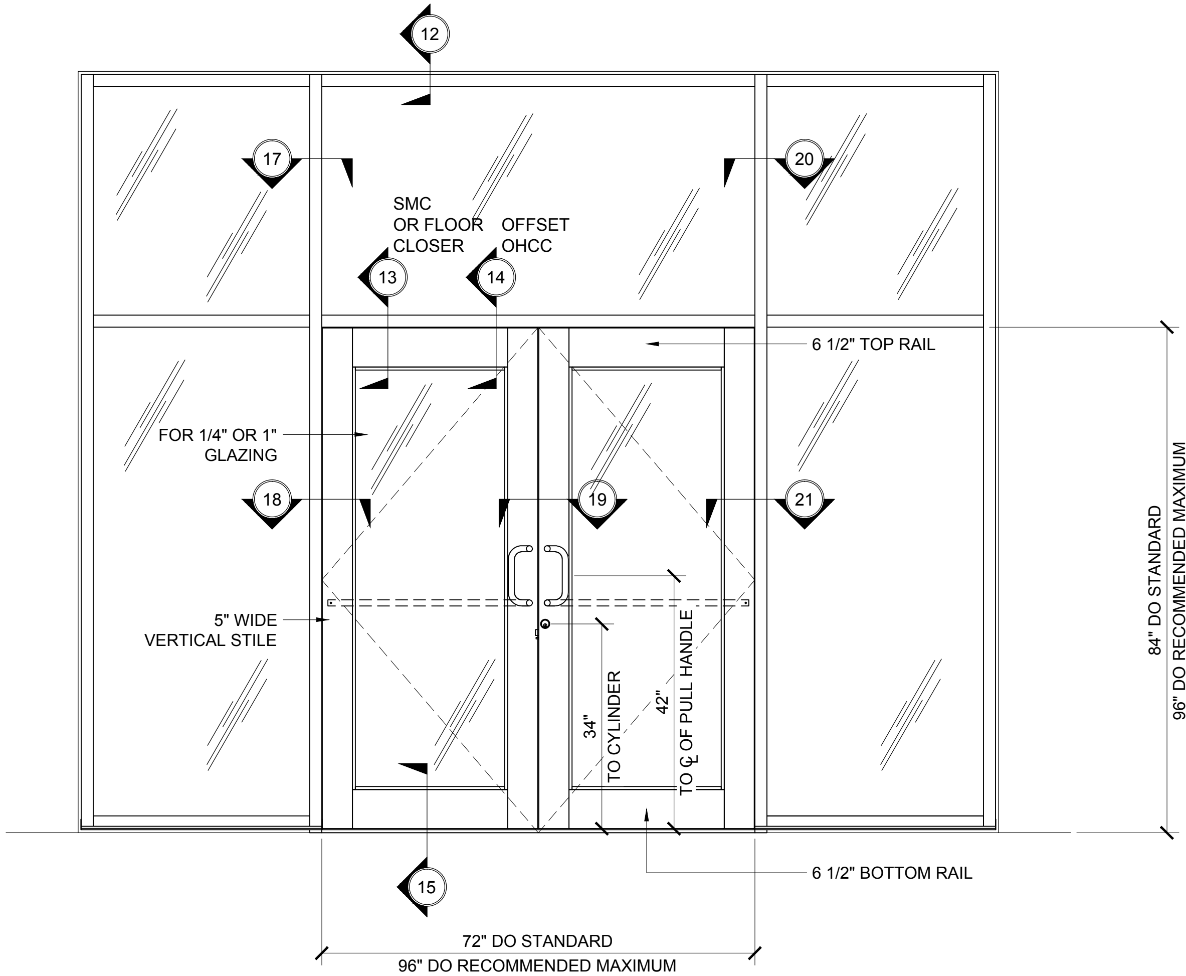
OFFSET-HUNG WIDE STILE SERIES 550 DOOR TYPICAL ELEVATION
