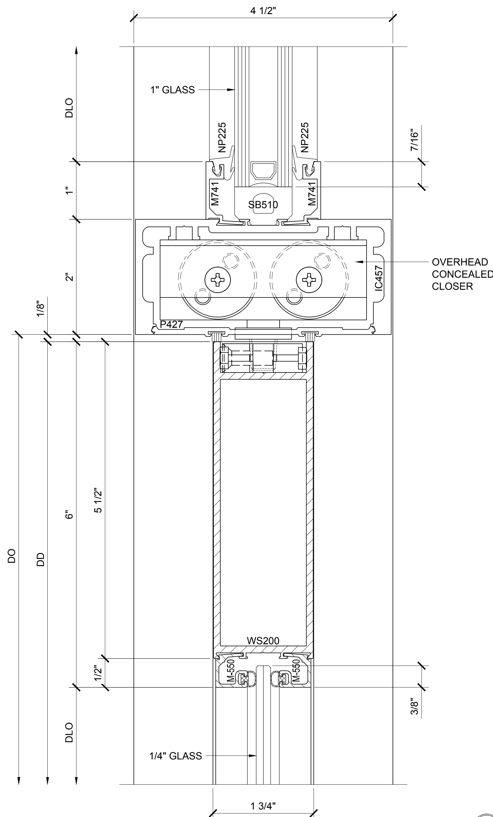
SECTION DETAIL @ DOOR HEAD WITH OHCC ③
