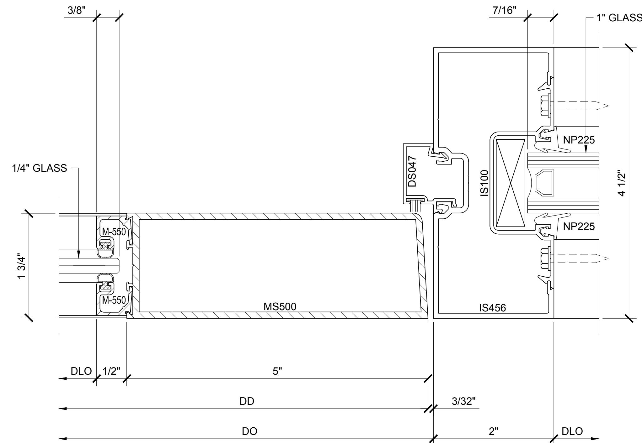
SECTION DETAIL @ DOOR JAMB 21
