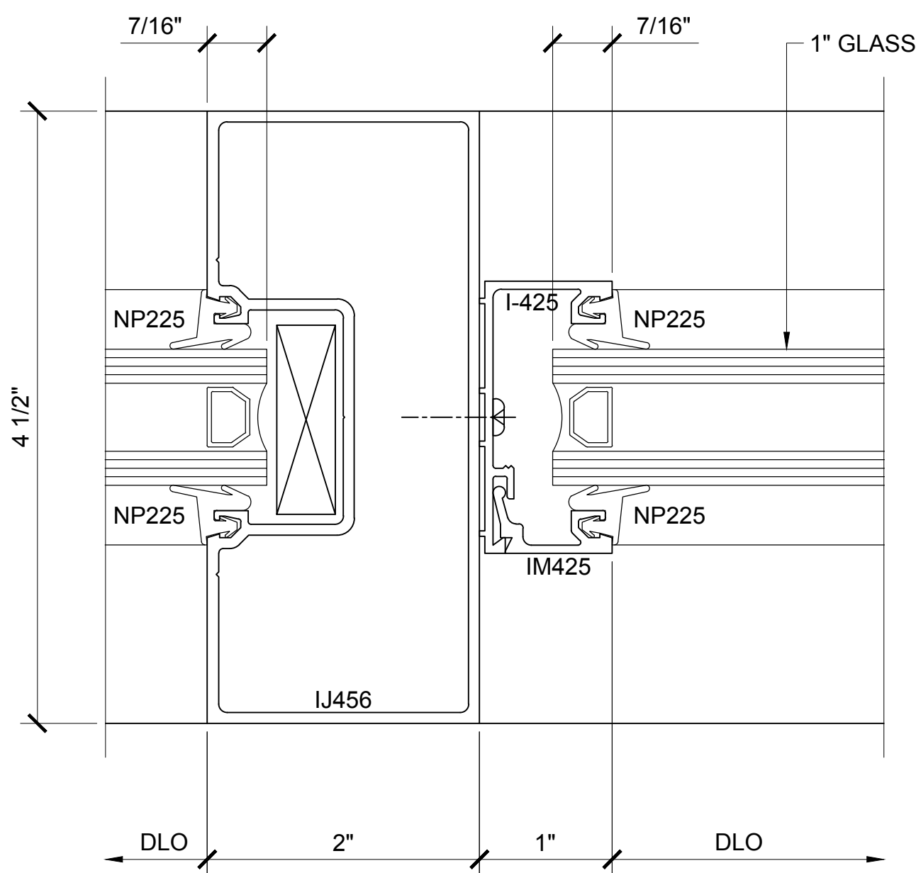
SECTION DETAIL @ VERTICAL
