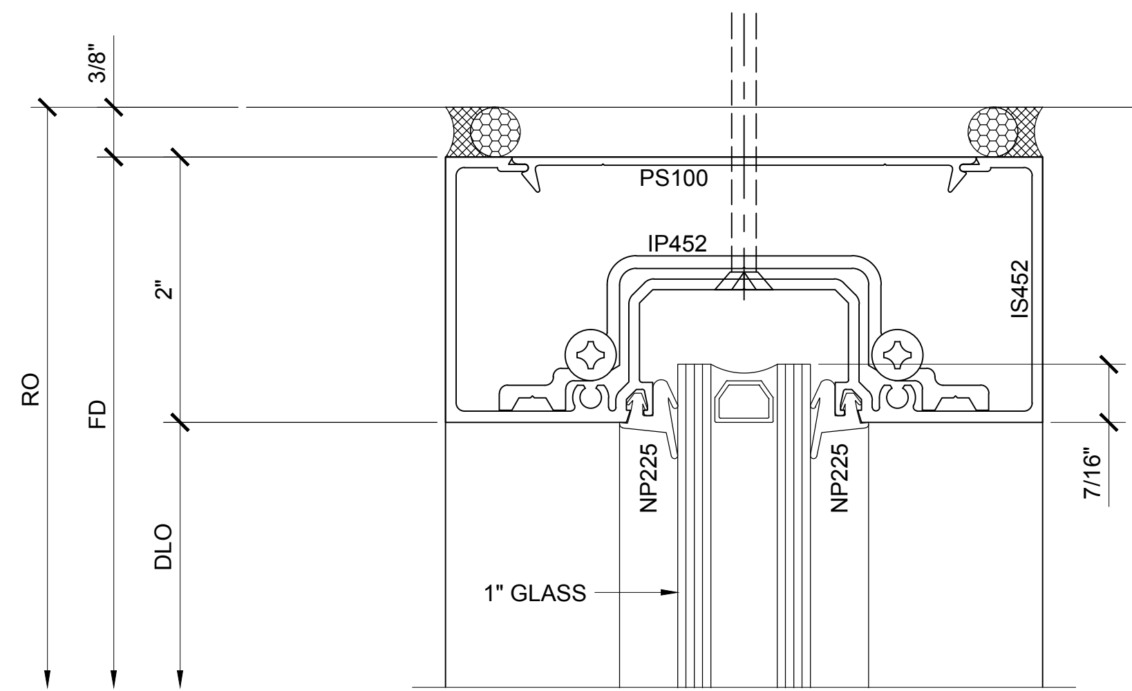
SECTION DETAIL @ STOREFRONT HEAD ①
