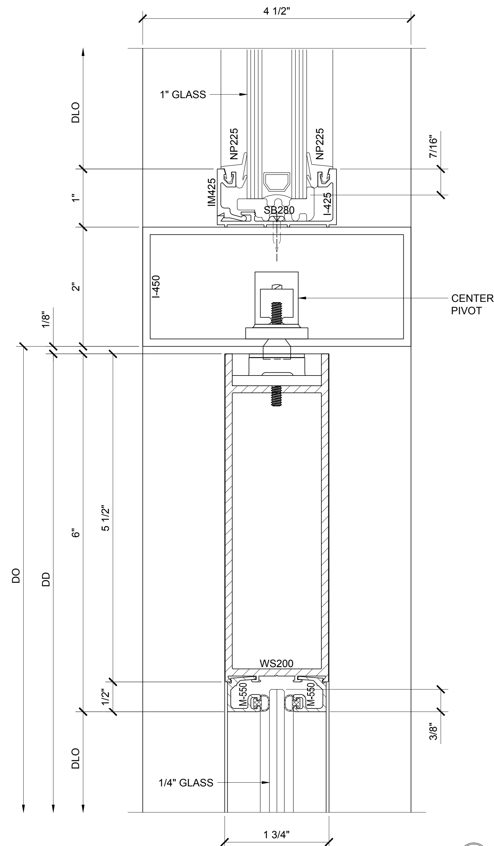
SECTION DETAIL @ DOOR HEAD WITH PIVOT ②
