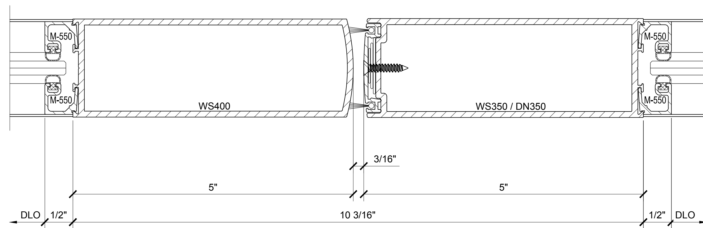
SECTION DETAIL @ MEETING STILES 19
