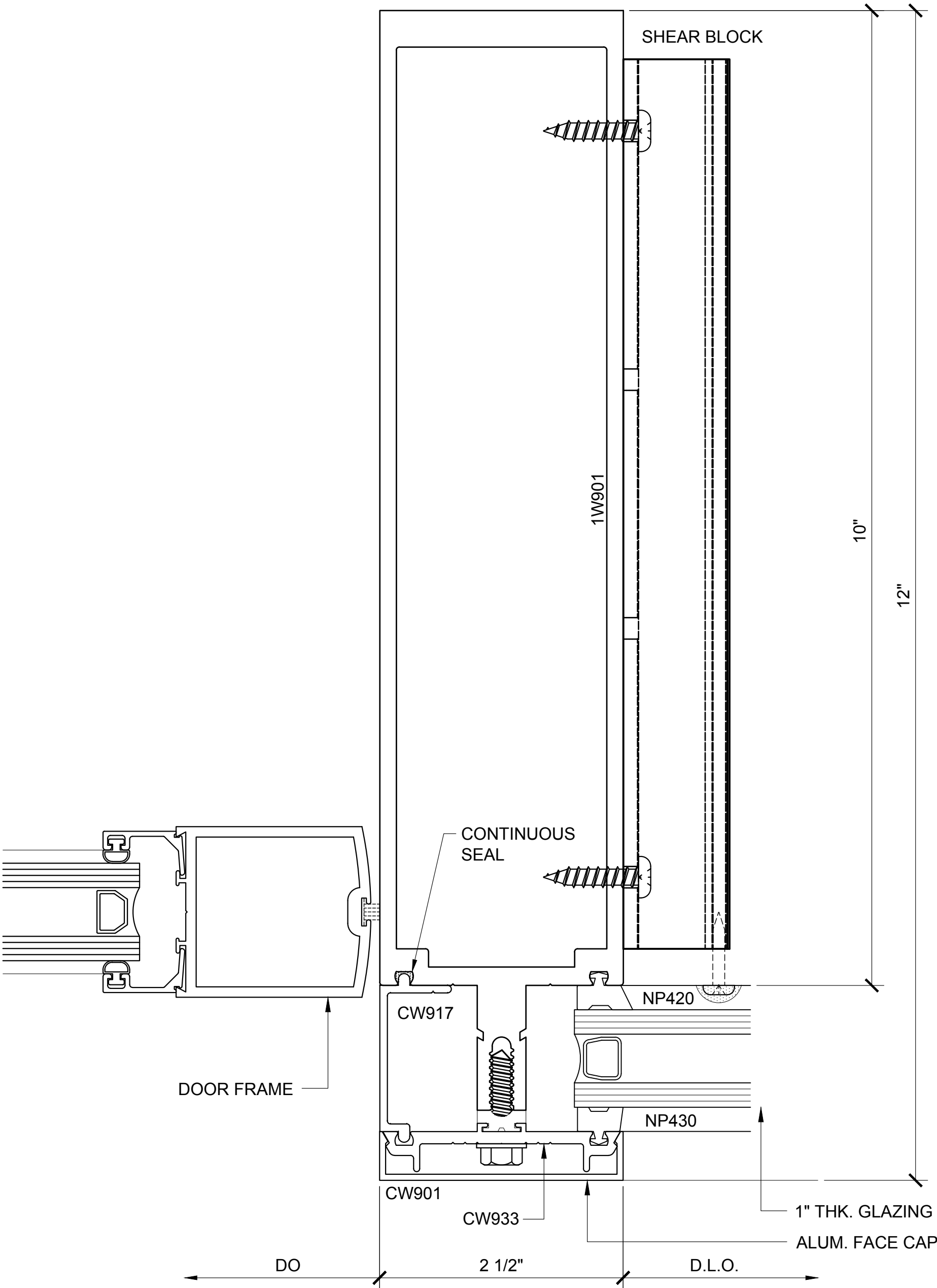
INT. VERT. PLAN 183 3250.3.3.4.183 DOUBLE GLAZED 10" VERTICALS W/ 10" BACK MEMBER CH DOOR FRAMING
