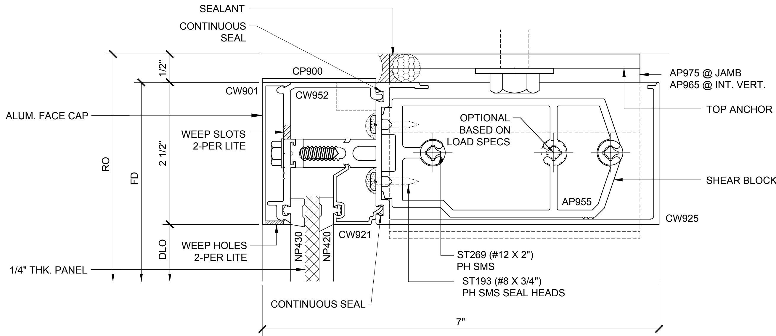
HEAD SECTION 105
