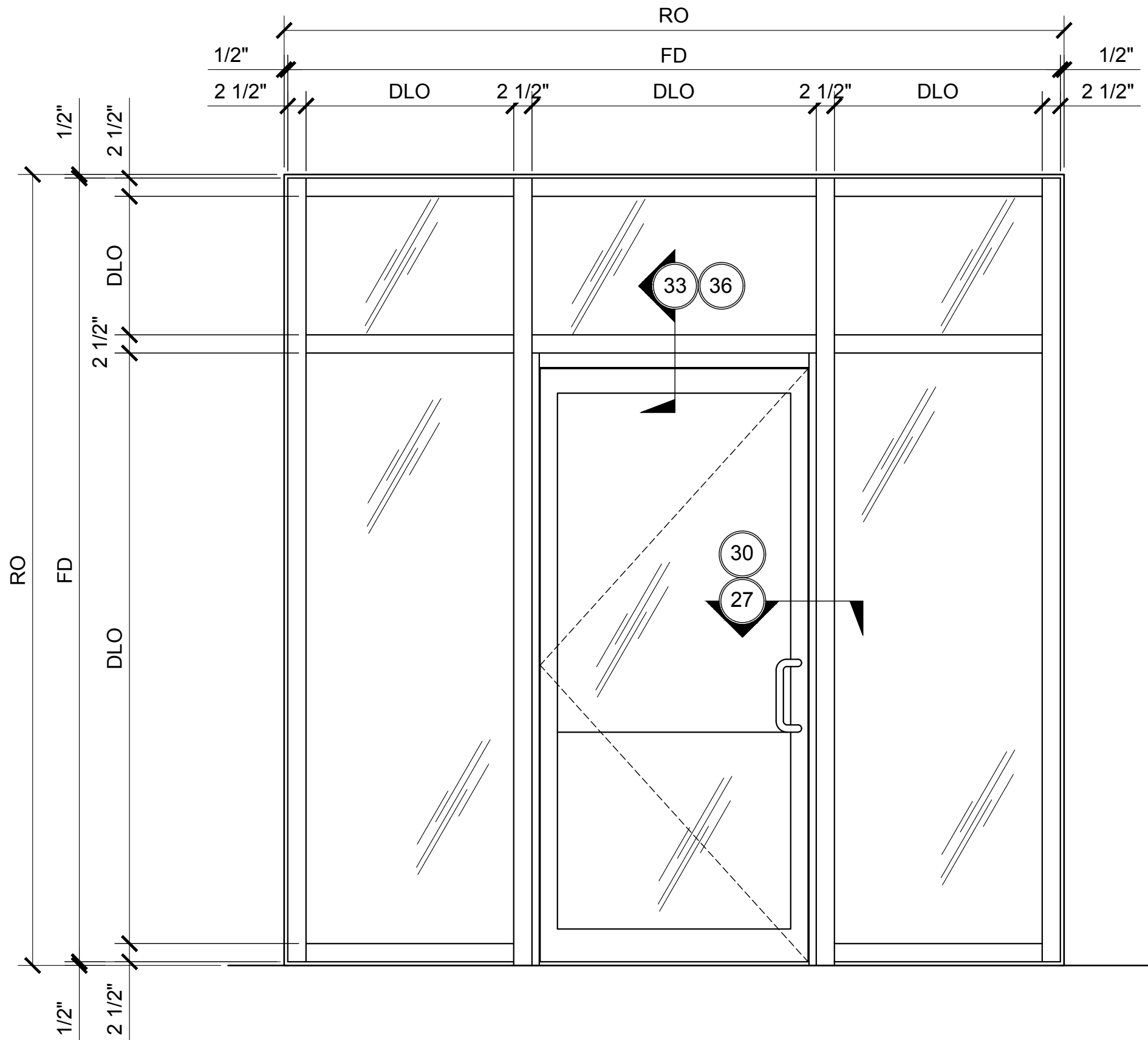
CENTER-HUNG DOOR FRAMING ELEVATION
