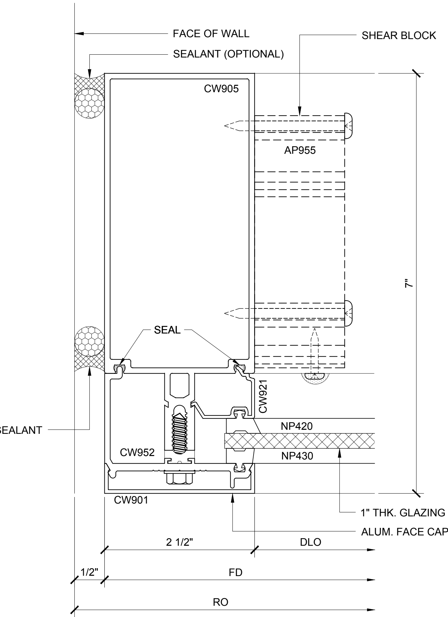
JAMB PLAN 52A 3250.2.2.4C.052A DOUBLE GLAZED 5" BACK MEMBER
