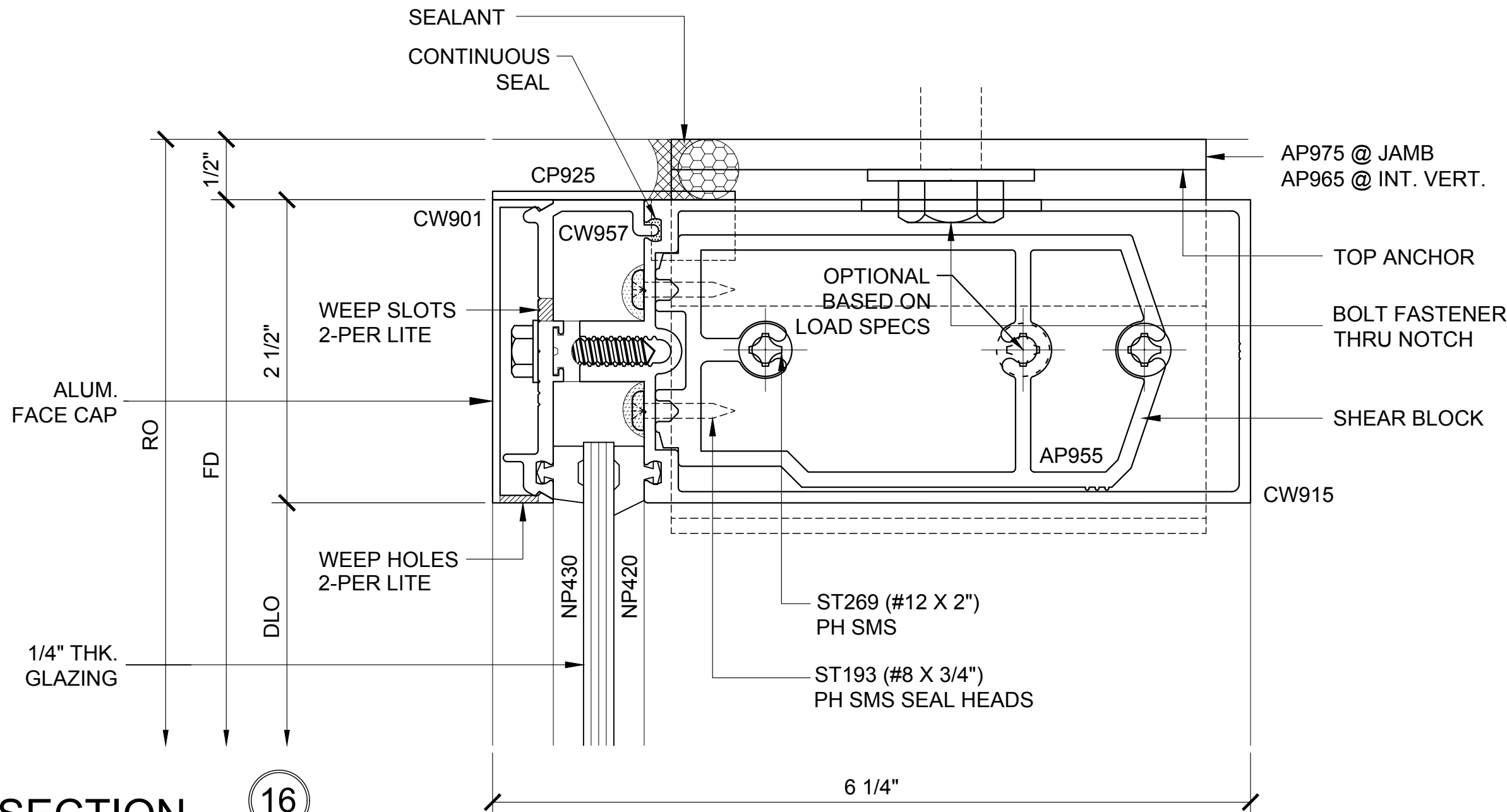
HEAD SECTION 16
