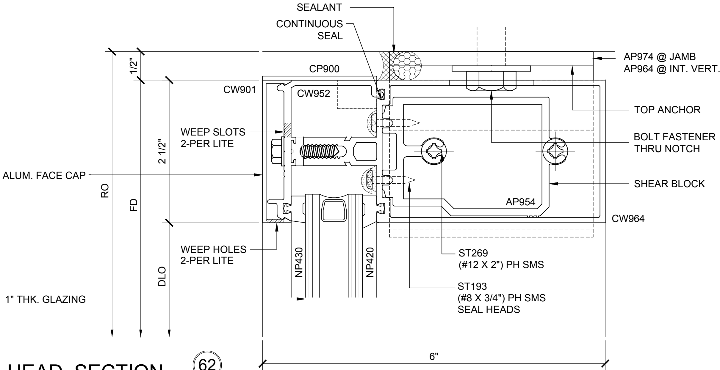
HEAD SECTION
