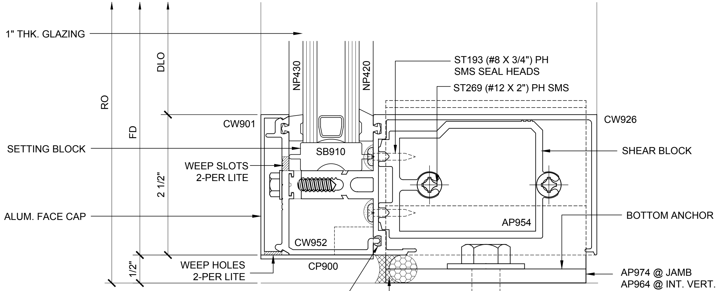
SILL SECTION
