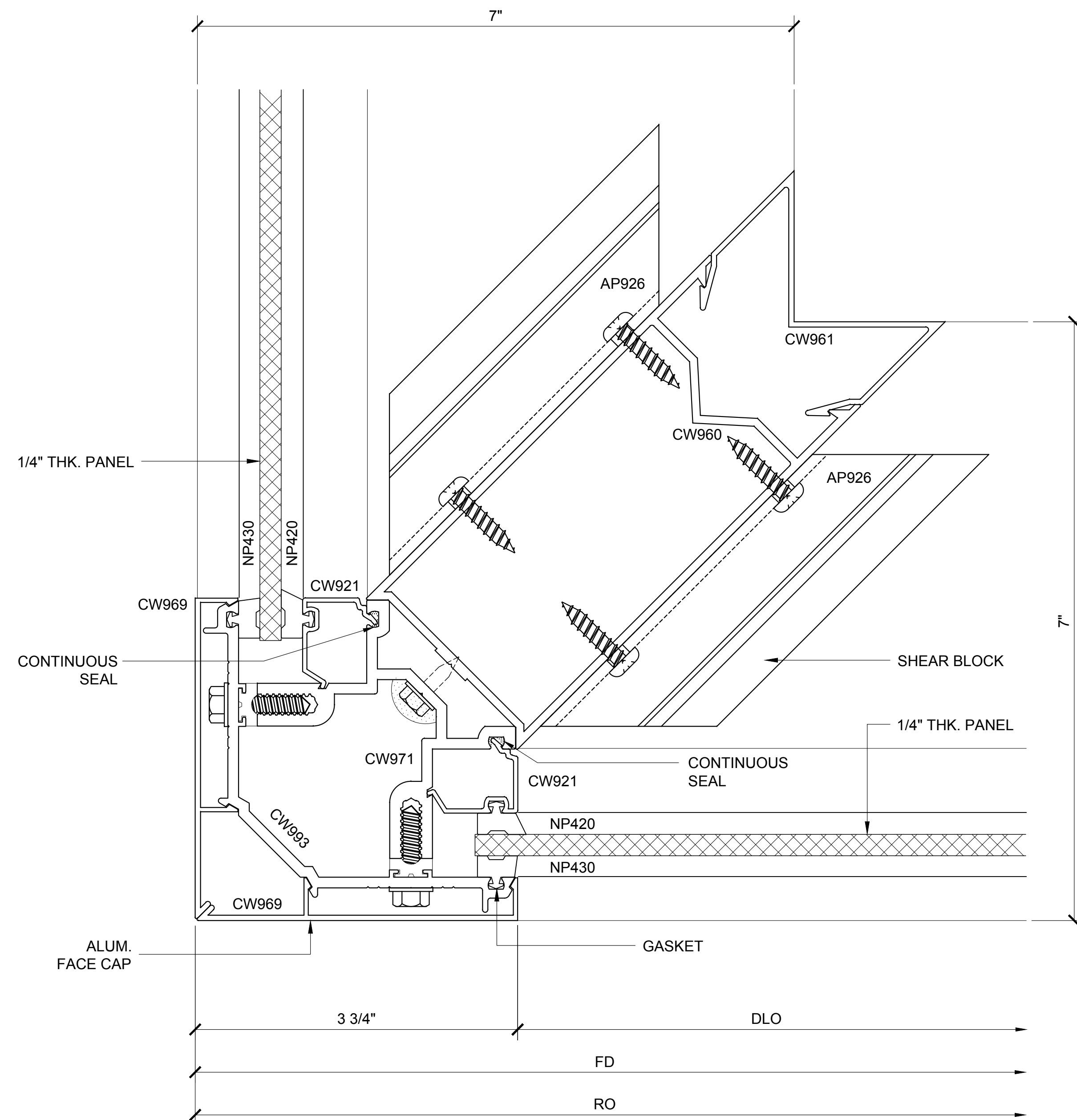
COR. VERT. SECTION 115
