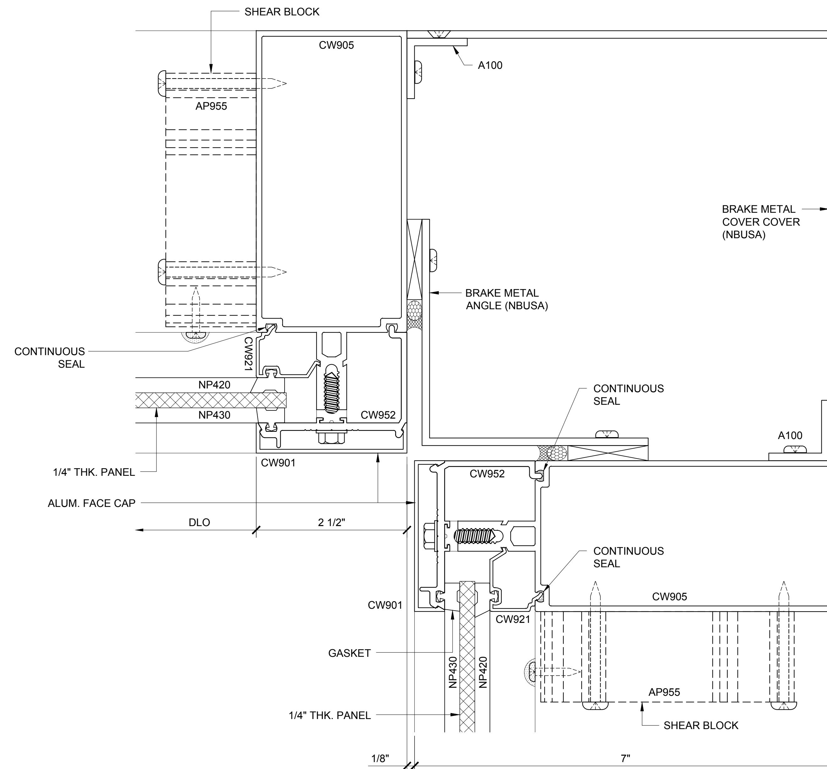
COR. VERT. SECTION 74A
