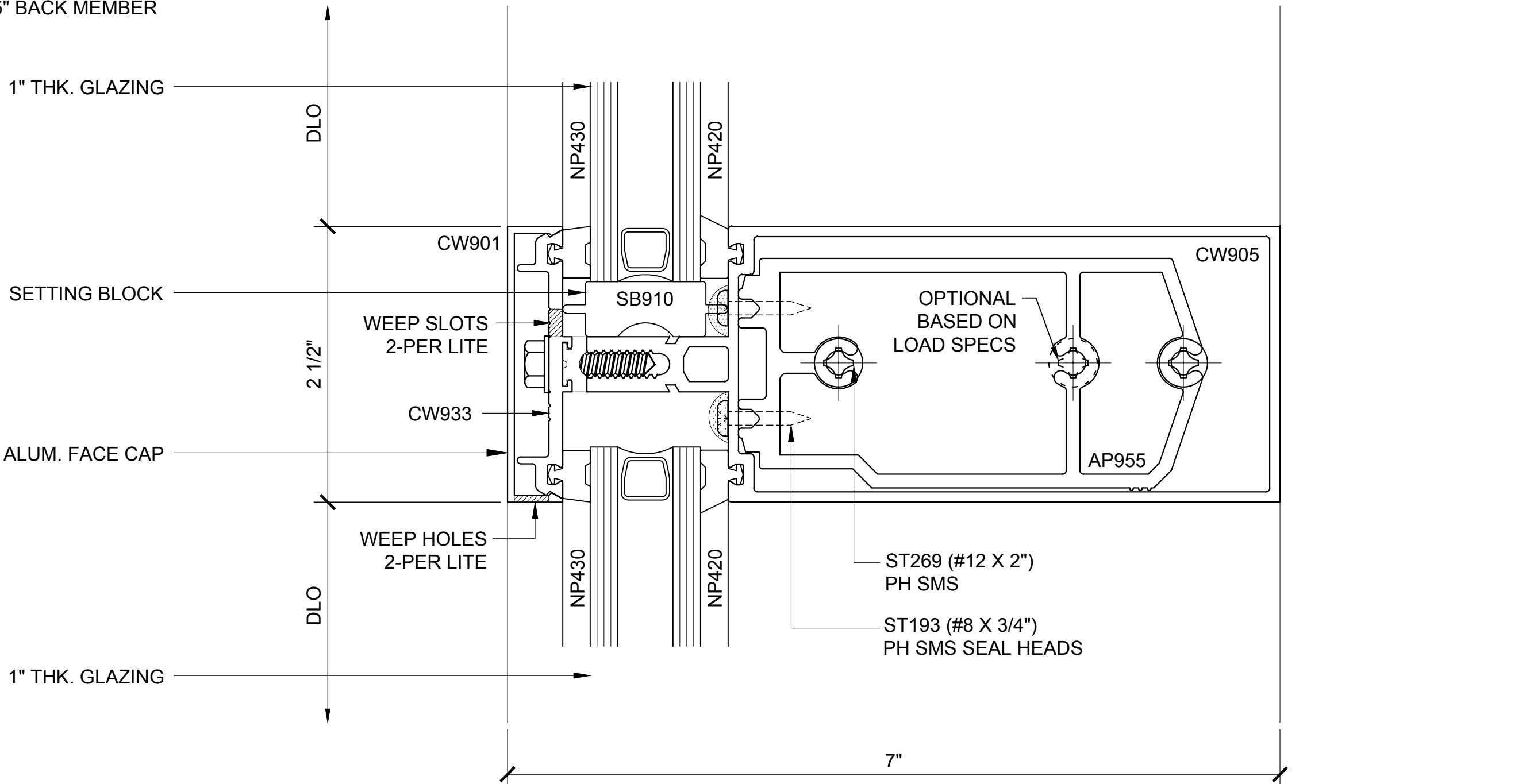
INT. HOR. SECTION
