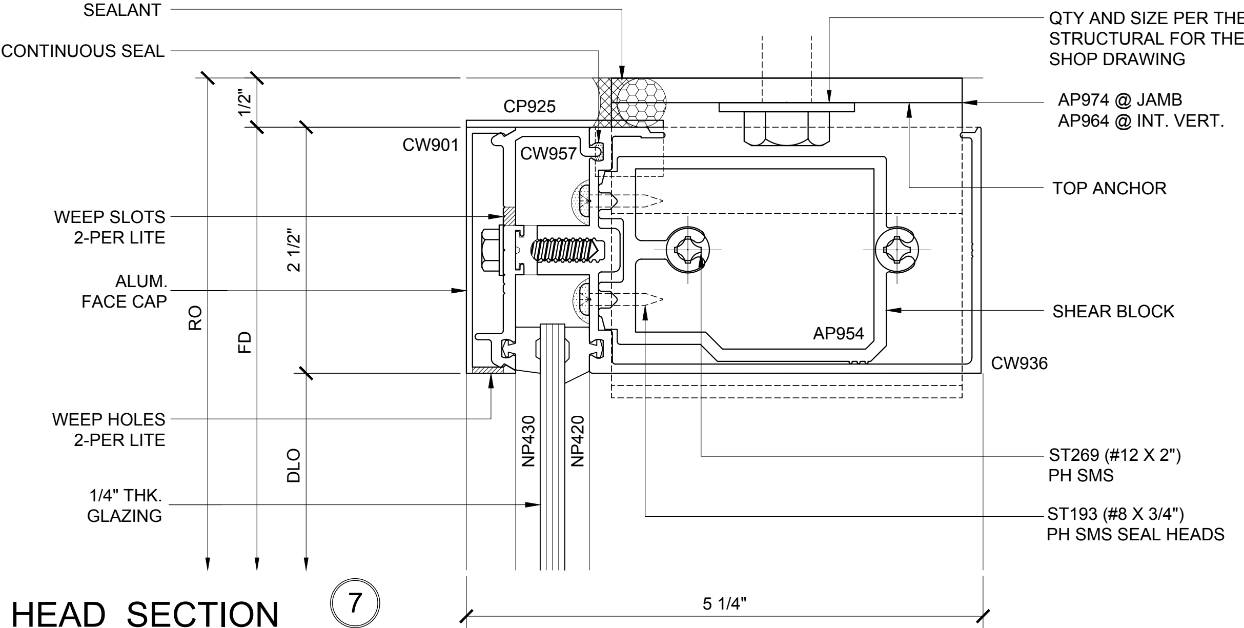
HEAD SECTION 7
