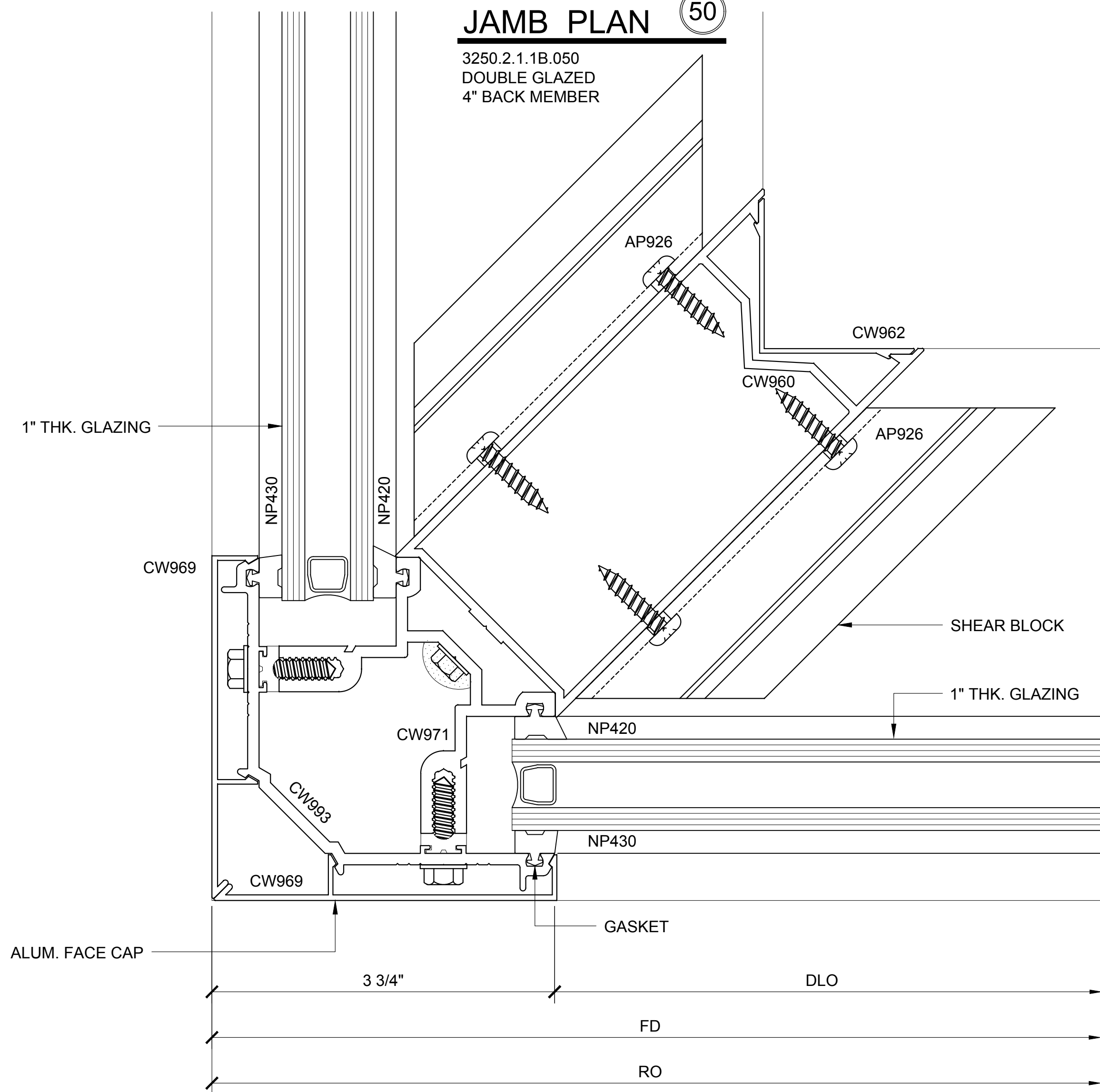
COR. VERT. PLAN 71 3250.2.1.1B.071 DOUBLE GLAZED 4" BACK MEMBER
