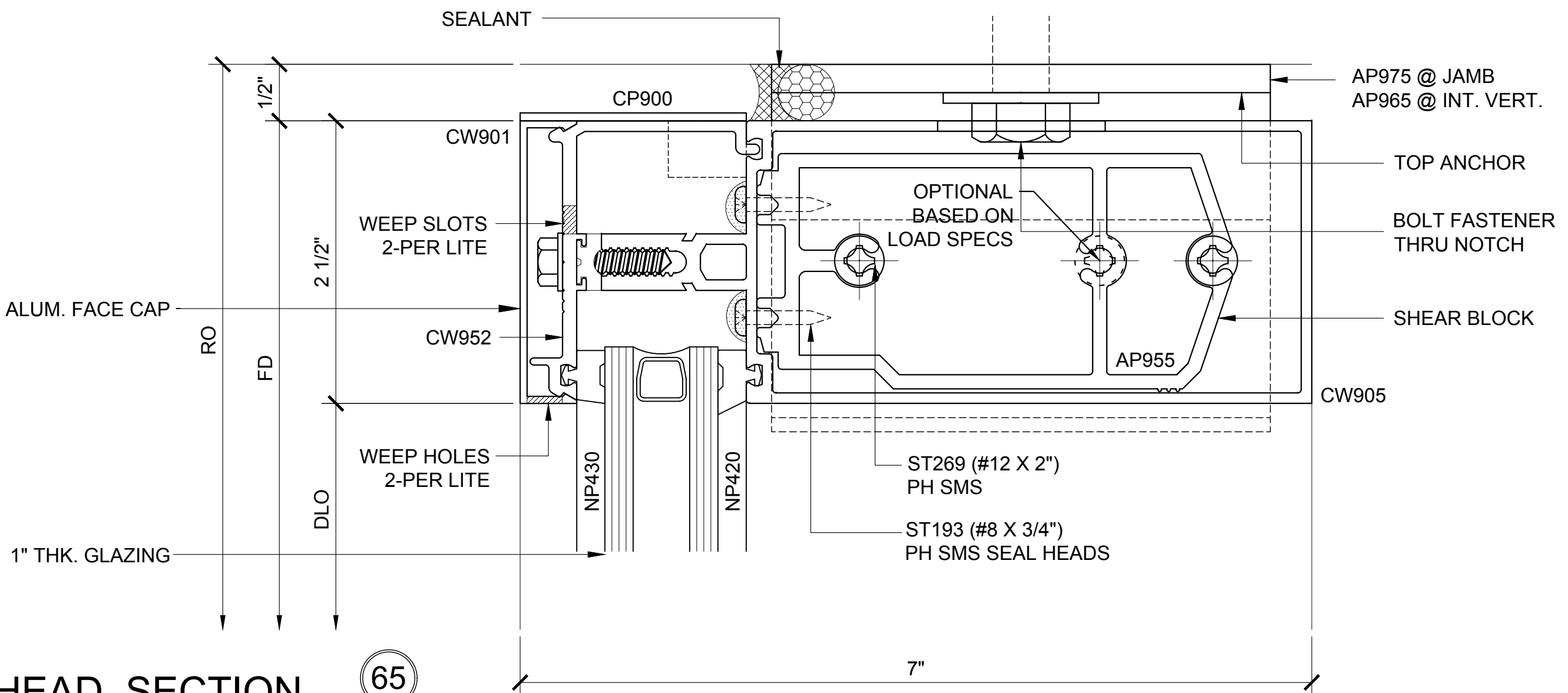
HEAD SECTION
