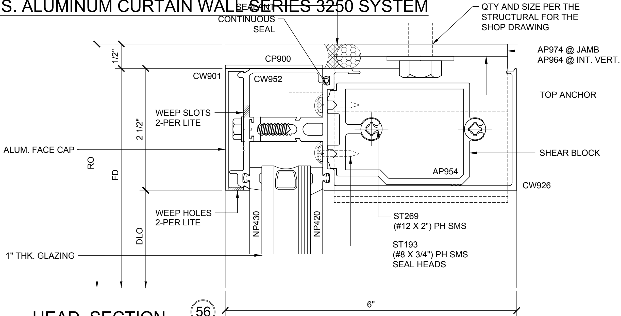
HEAD SECTION
