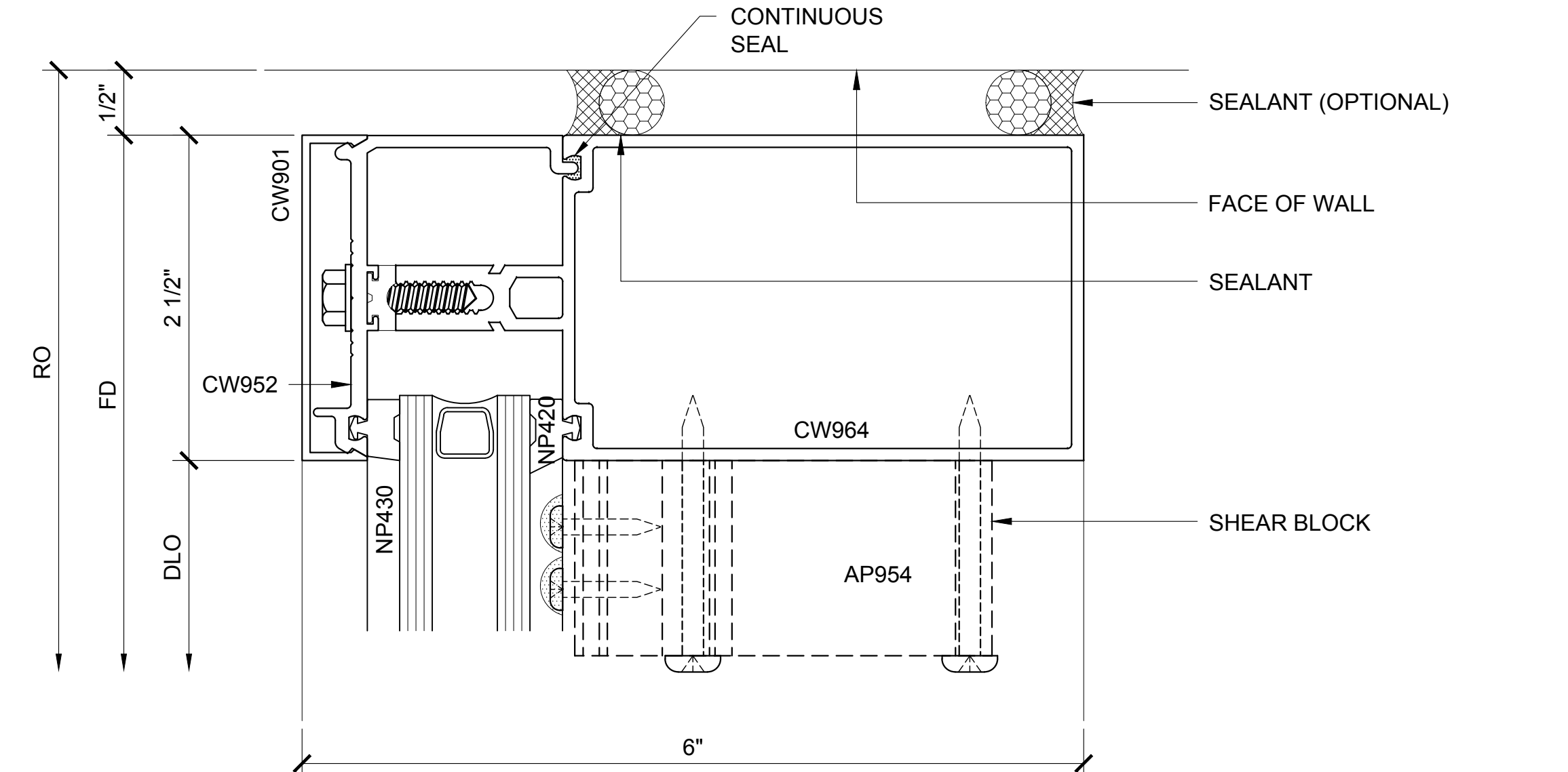
JAMB PLAN 50 3250.2.1.1B.050 DOUBLE GLAZED 4" BACK MEMBER
