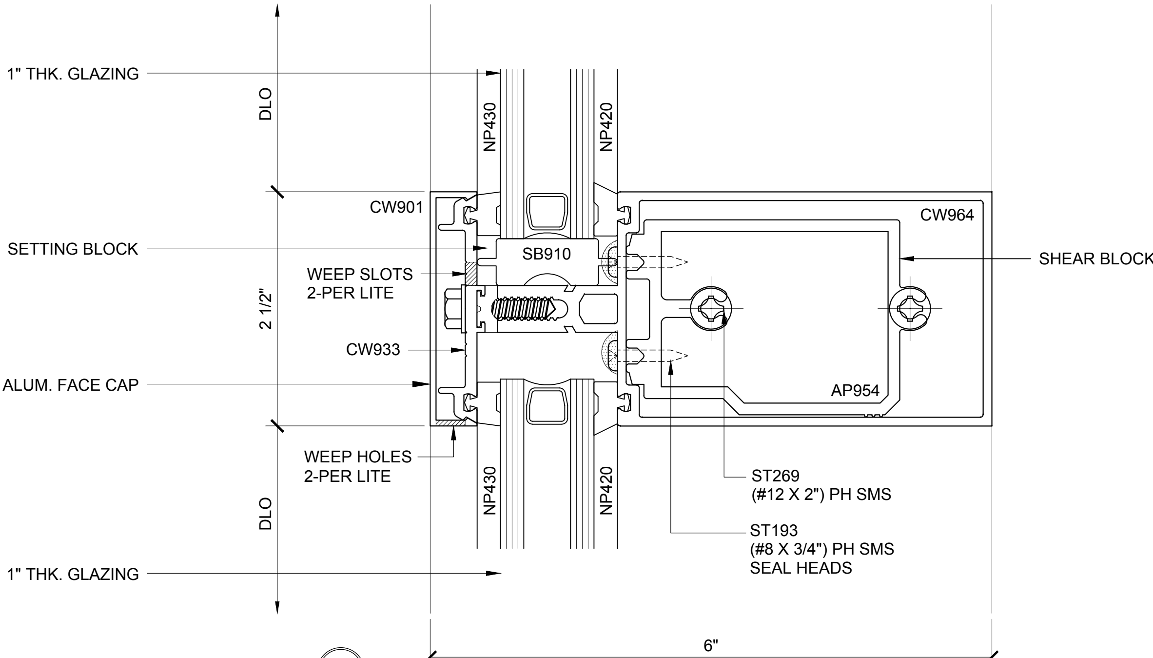
INT. HOR. SECTION
