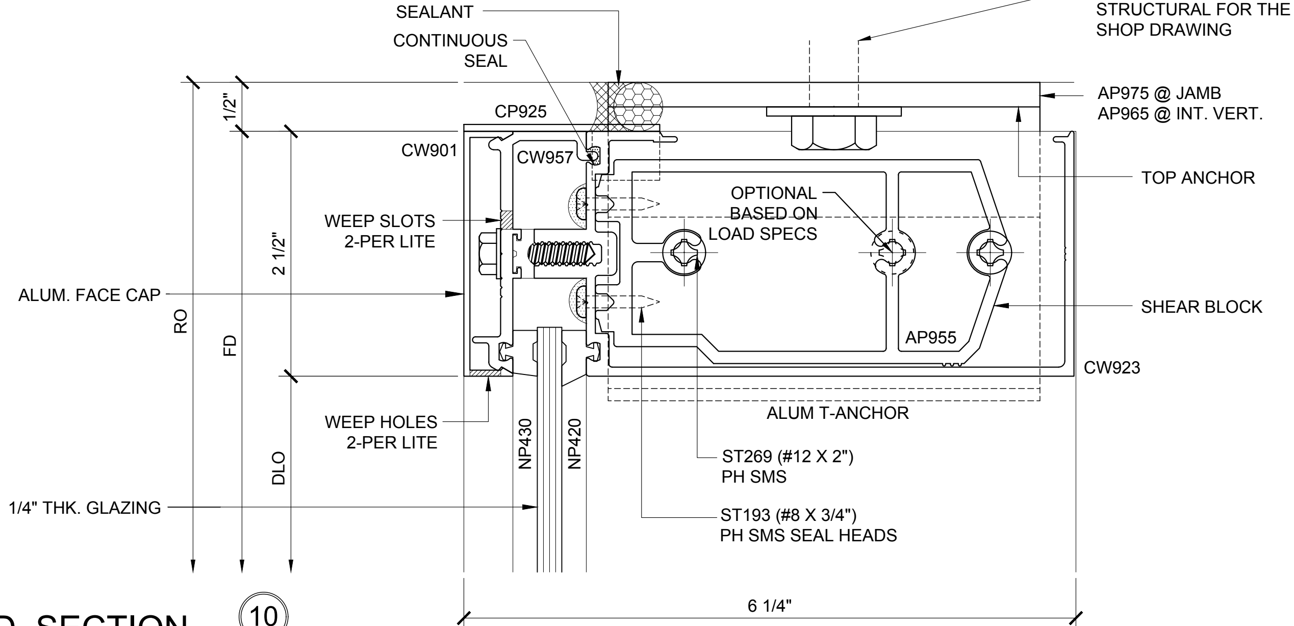
HEAD SECTION 10
