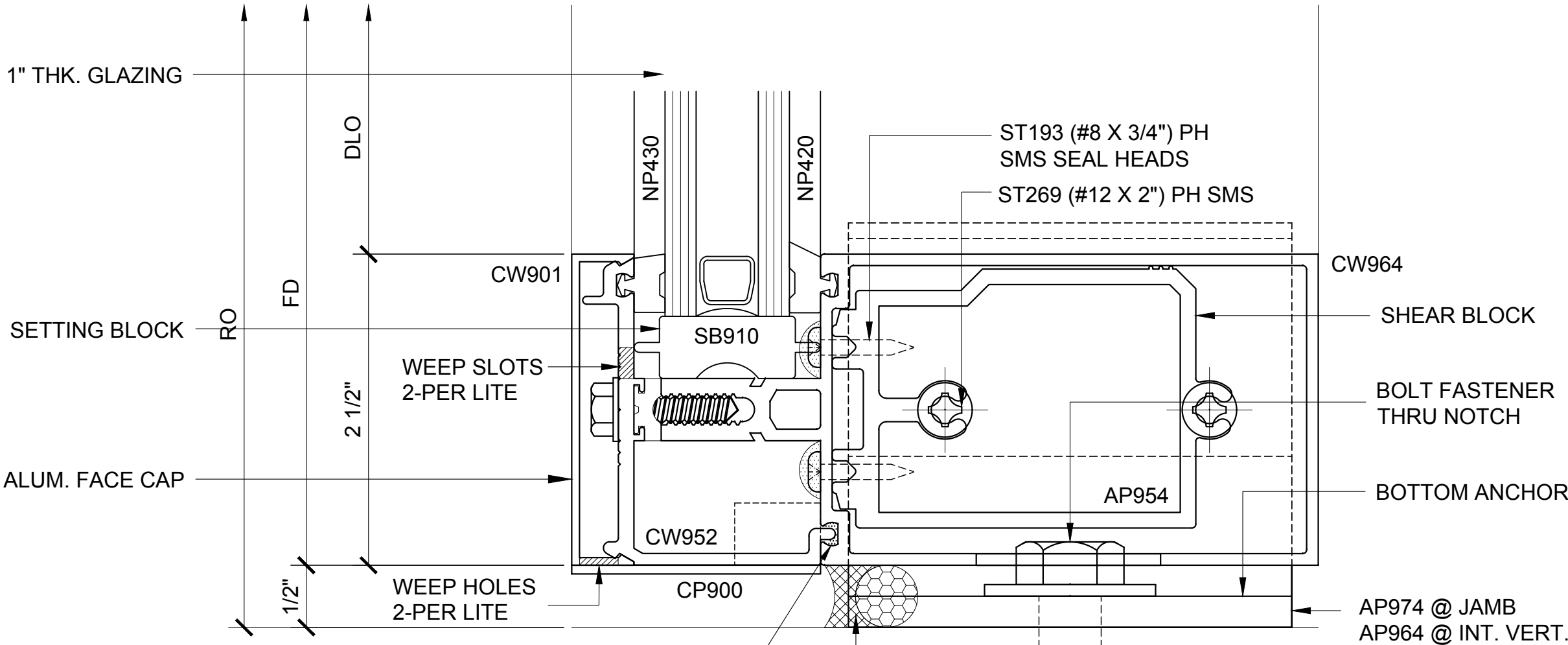
SILL SECTION
