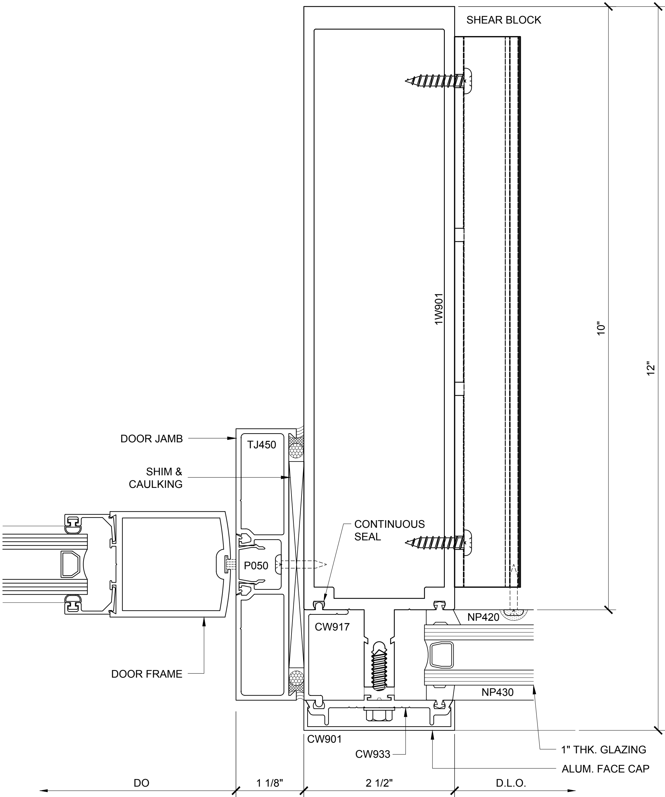
DOOR JAMB PLAN 184 3250.3.3.4.184 DOUBLE GLAZED 10" VERTICALS W/ 10" BACK MEMBER CH DOOR FRAMING
