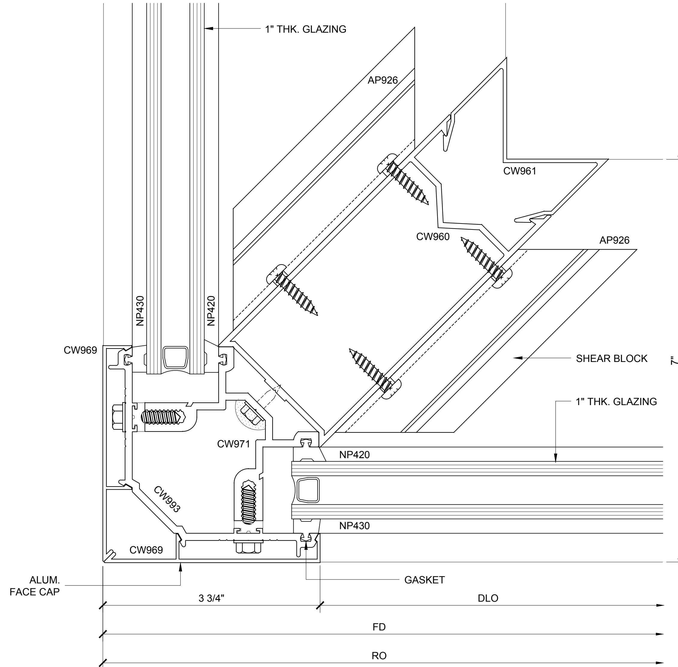
COR. VERT. PLAN 72
