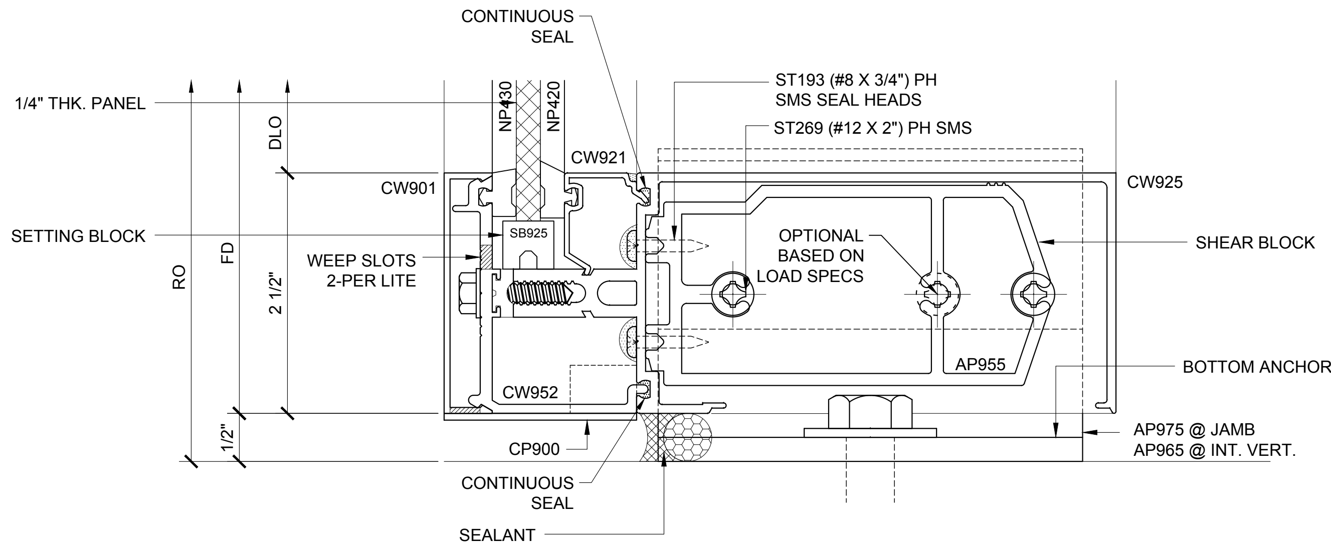
SILL SECTION 109
