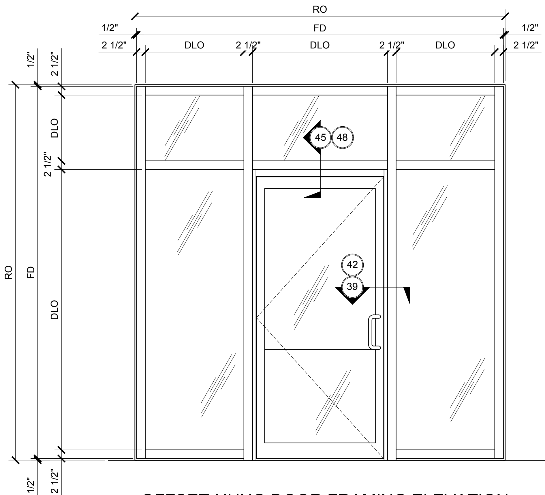
OFFSET-HUNG DOOR FRAMING ELEVATION
