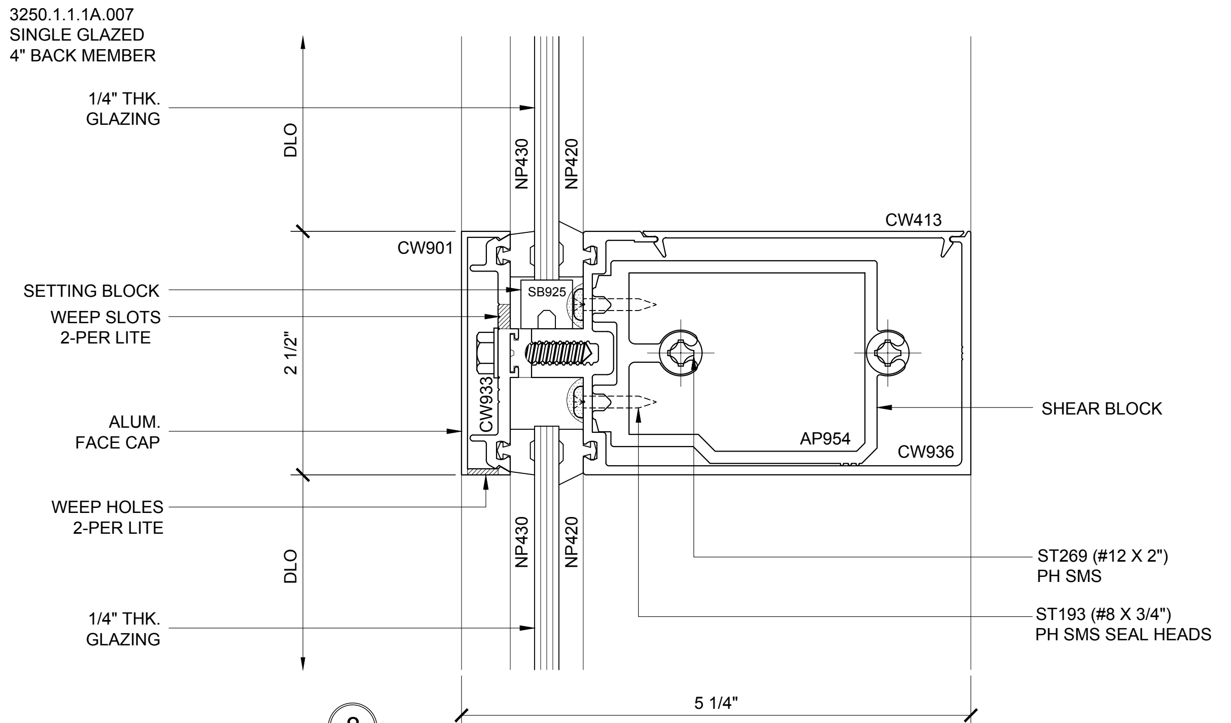
INT. HOR. SECTION 8
