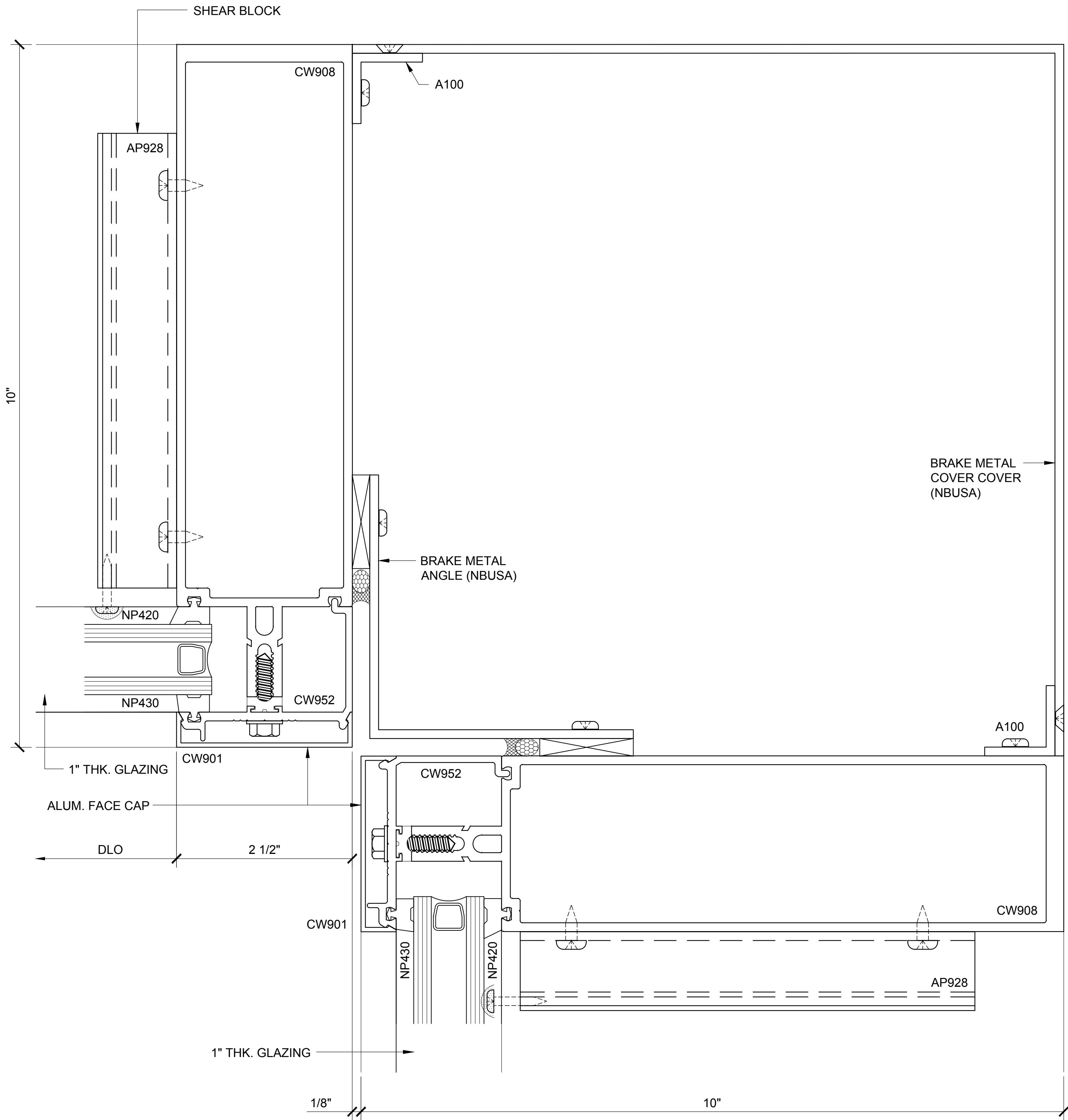
COR. VERT. SECTION 117
