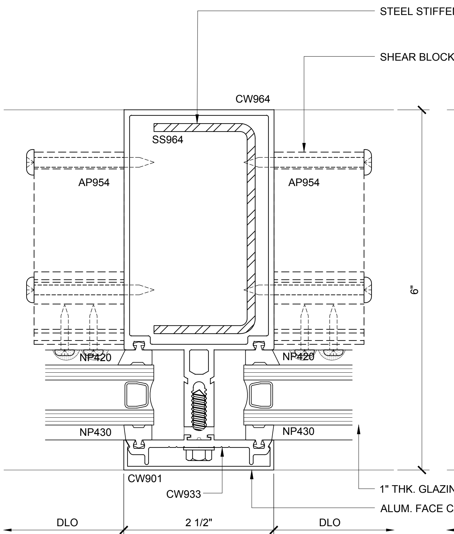
INT. VERT. PLAN 51 3250.2.1.1B.051 DOUBLE GLAZED 4" BACK MEMBER
