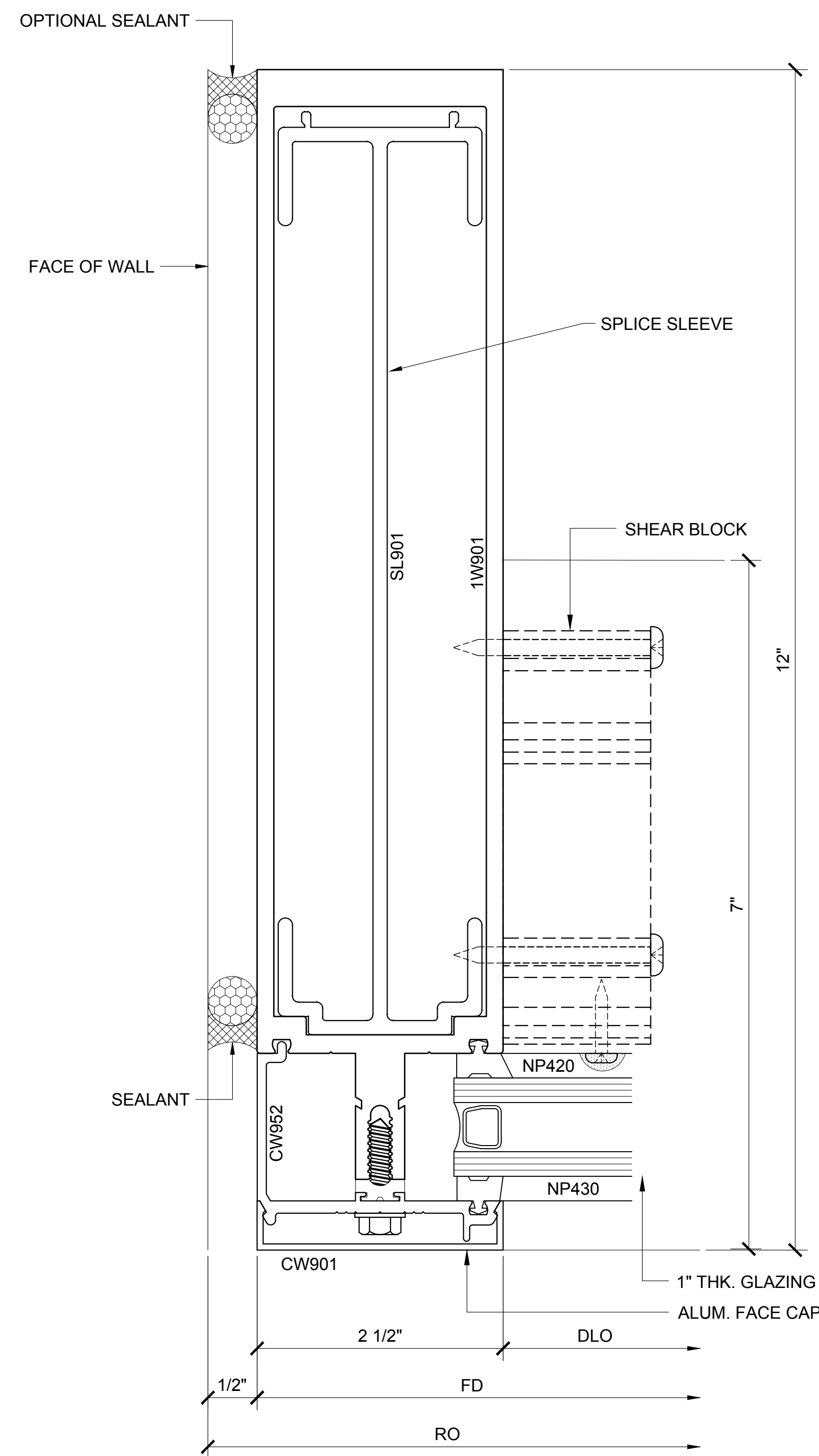
JAMB PLAN 146 3250.3.1.4.146 DOUBLE GLAZED 10" VERTICALS W/ 5" BACK MEMBER
