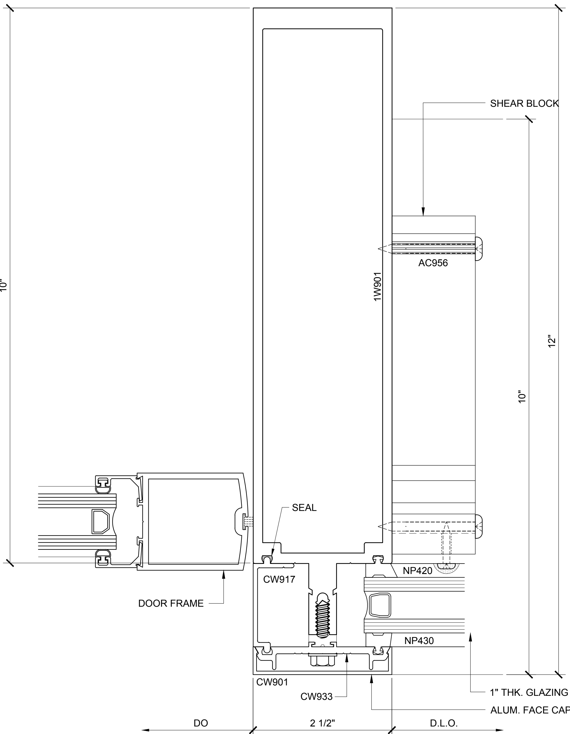
INT. VERT. PLAN 170 3250.3.2.7.170 DOUBLE GLAZED 10" VERTICALS W/ 8" BACK MEMBER CH DOOR FRAMING
