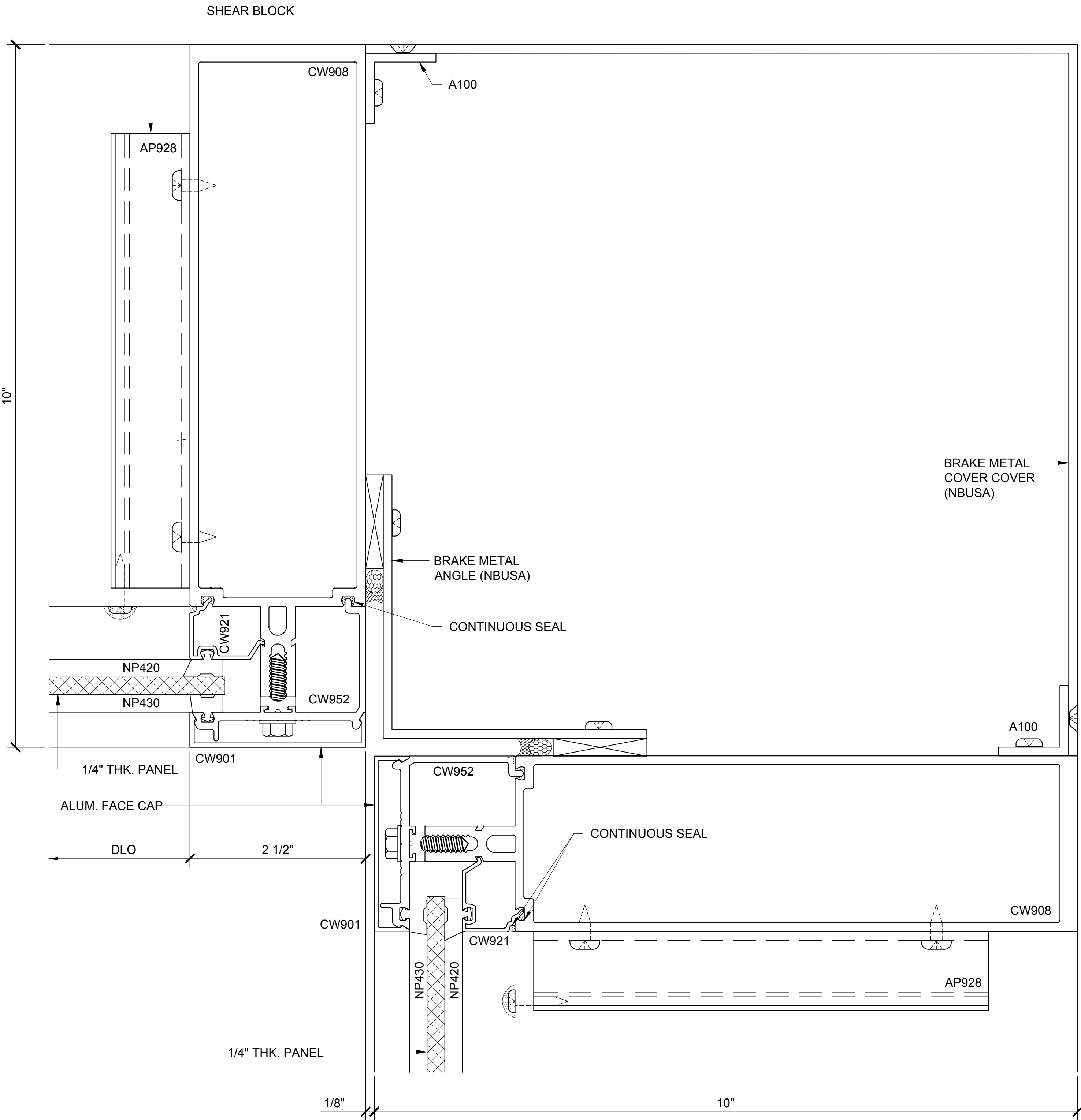
COR. VERT. SECTION 117A
