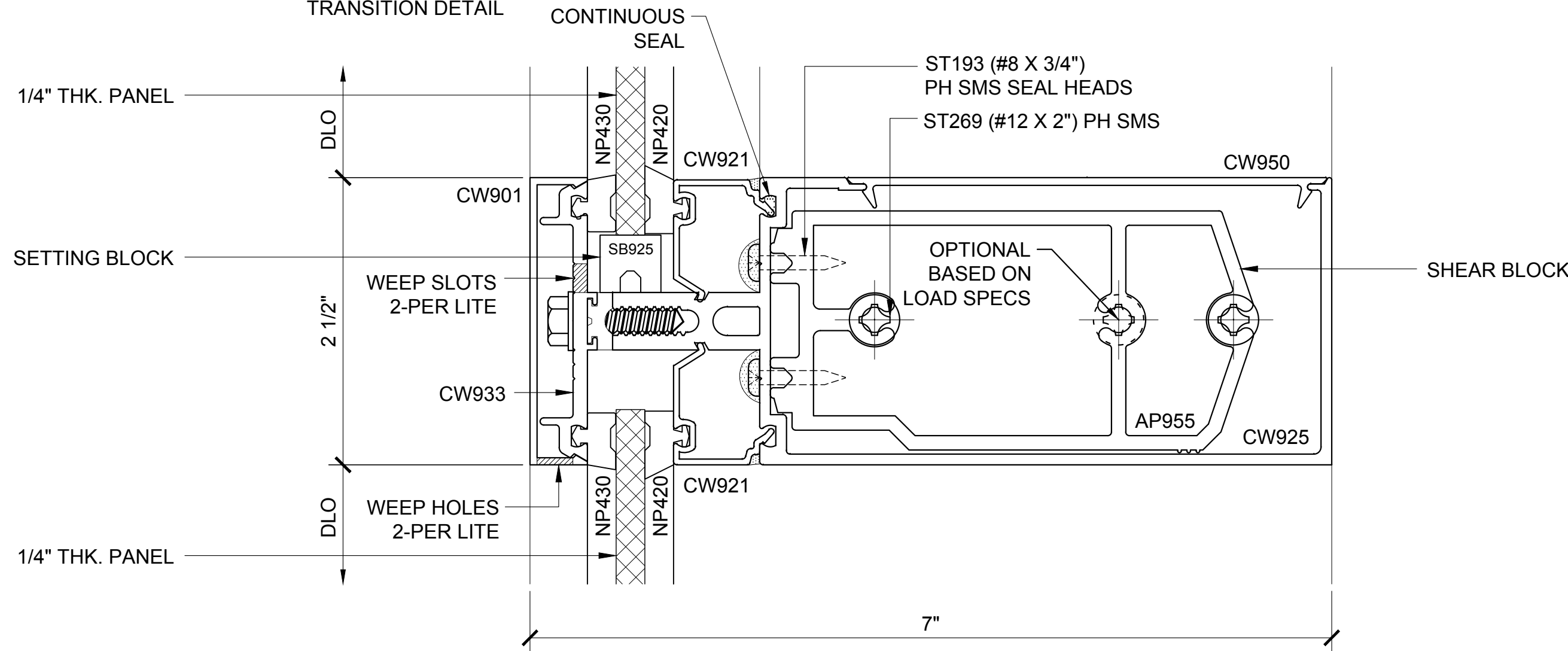
HEAD SECTION 107B
