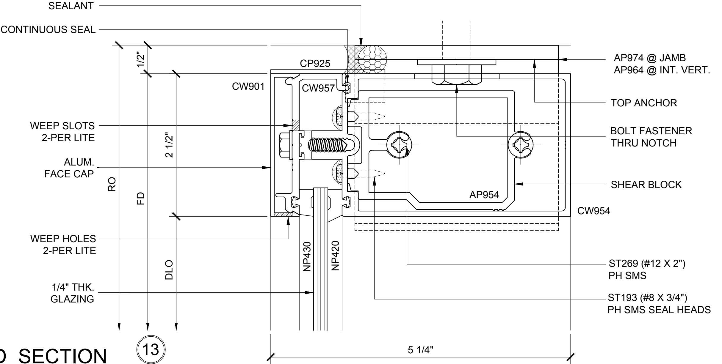
HEAD SECTION 13
