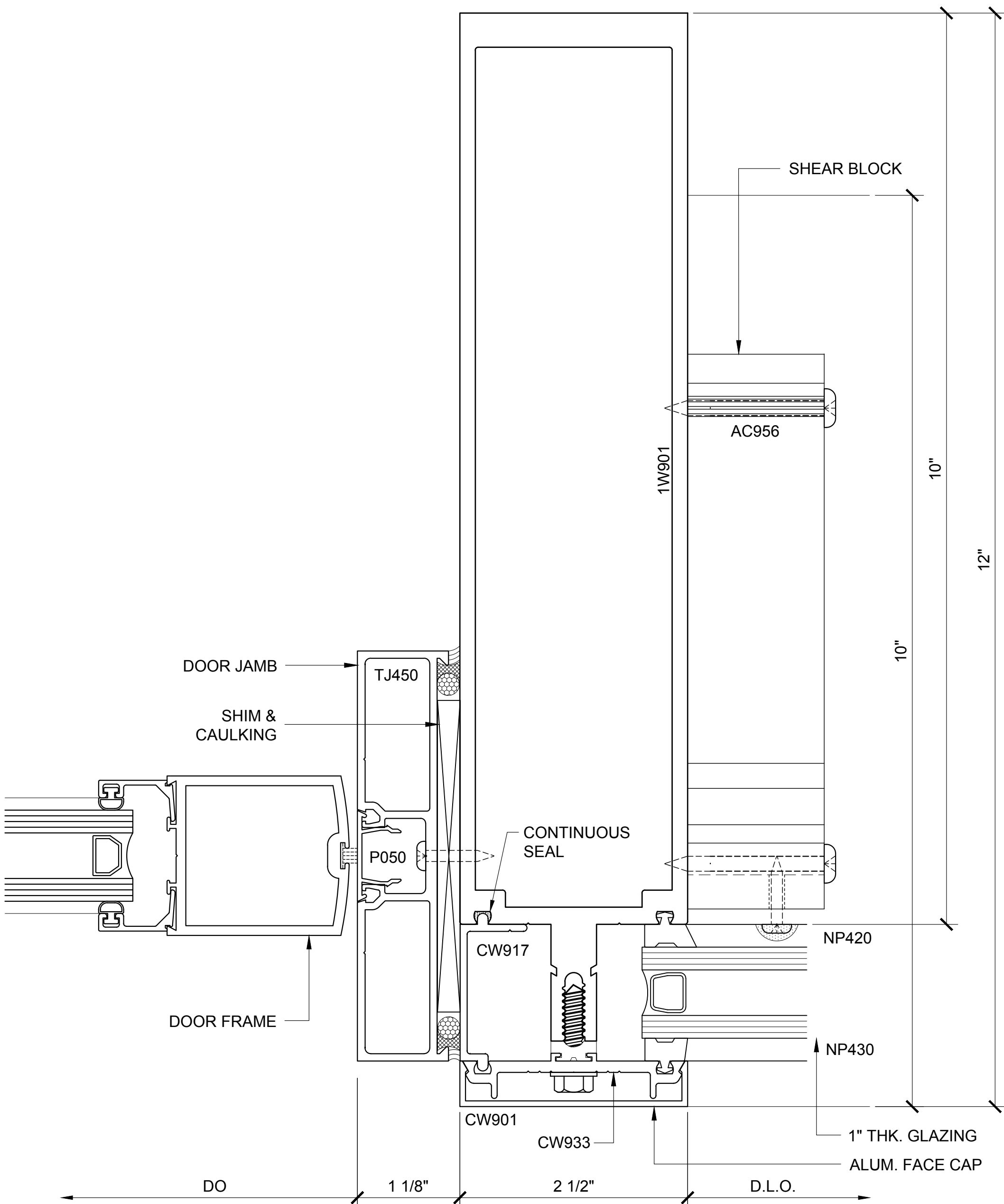
DOOR JAMB PLAN 171 3250.3.2.7.171 DOUBLE GLAZED 10" VERTICALS W/ 8" BACK MEMBER CH DOOR FRAMING
