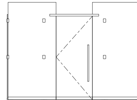
⑤ Klarity Partition w/Swinging Door Option 1/2" = 1'-0"
