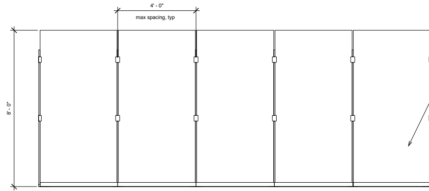
① KPOSTBS (84" tall) 1/2" = 1'-0"
