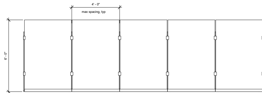
③ KPOSTBS (60" Tall) 1/2" = 1'-0"
