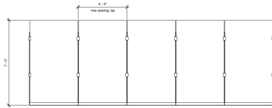
② KPOSTBS (72" Tall) 1/2" = 1'-0"
