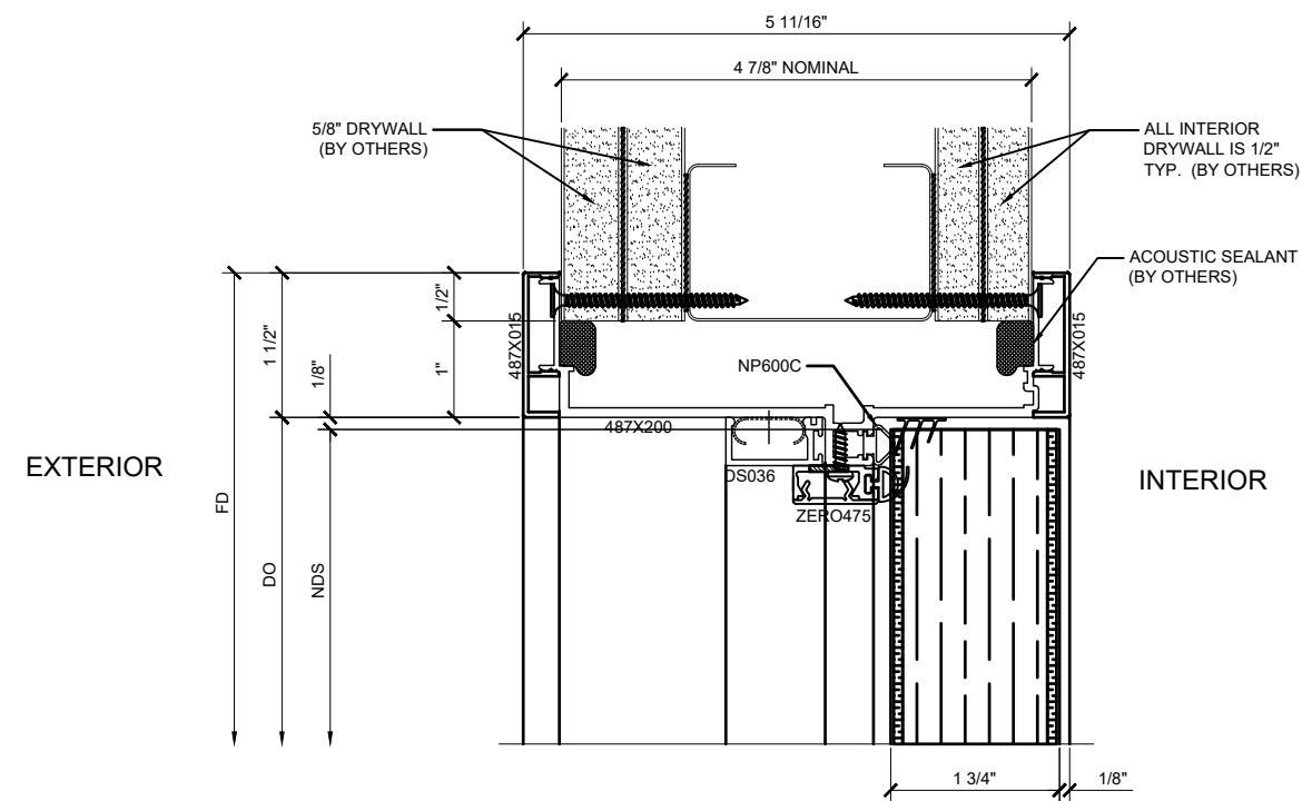
① DOOR HEAD DETAIL WITH RATED DOOR ARCH REF: 1'-0"=1'-0" SHOWN WITH AN STC - 39 DOOR AND FRAME
