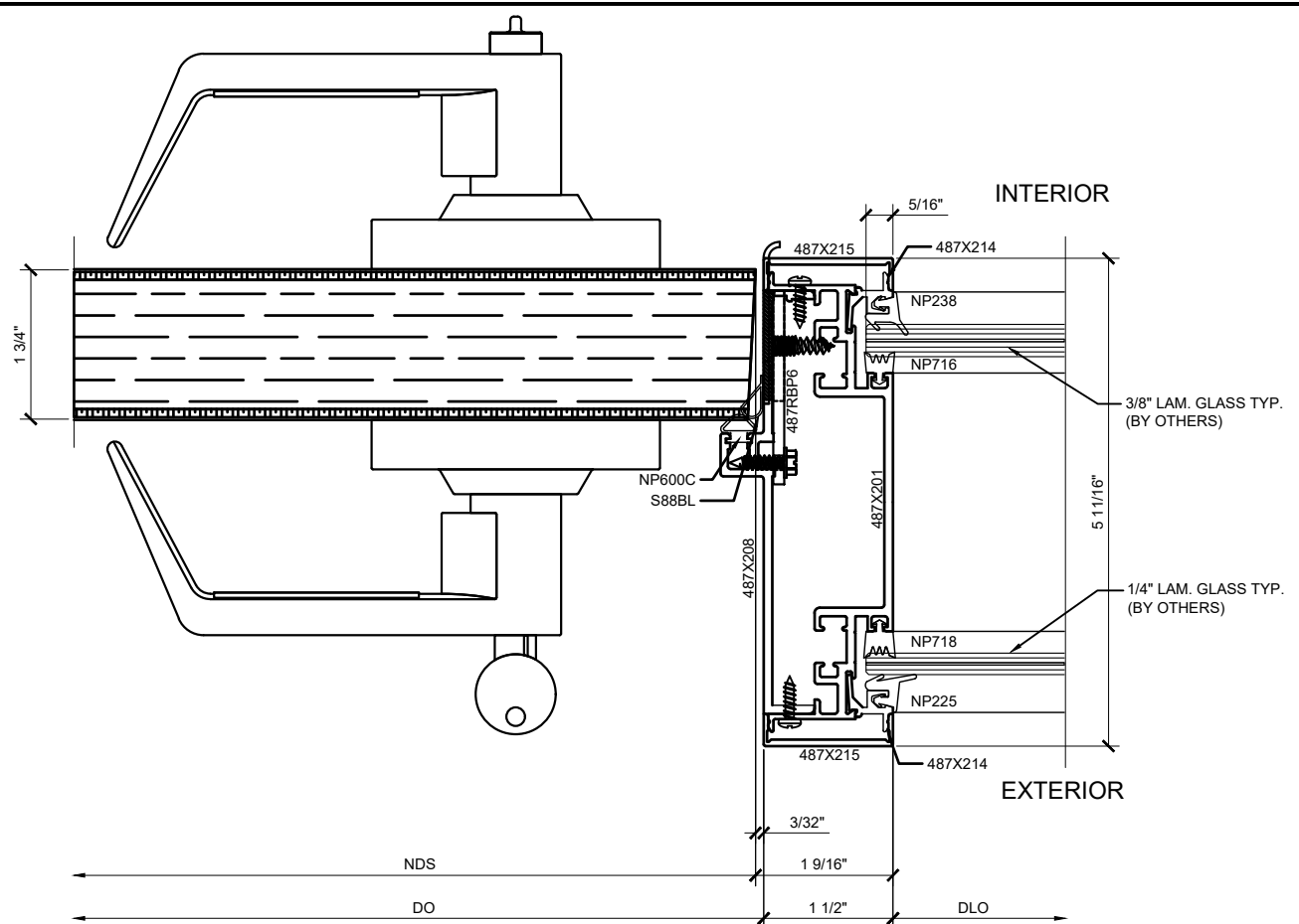
② DOOR JAMB DETAIL AT STRIKE SIDE W/ SIDELITE ARCH REF: 1'-0"=1'-0" SHOWN WITH AN STC - 35 DOOR AND FRAME
