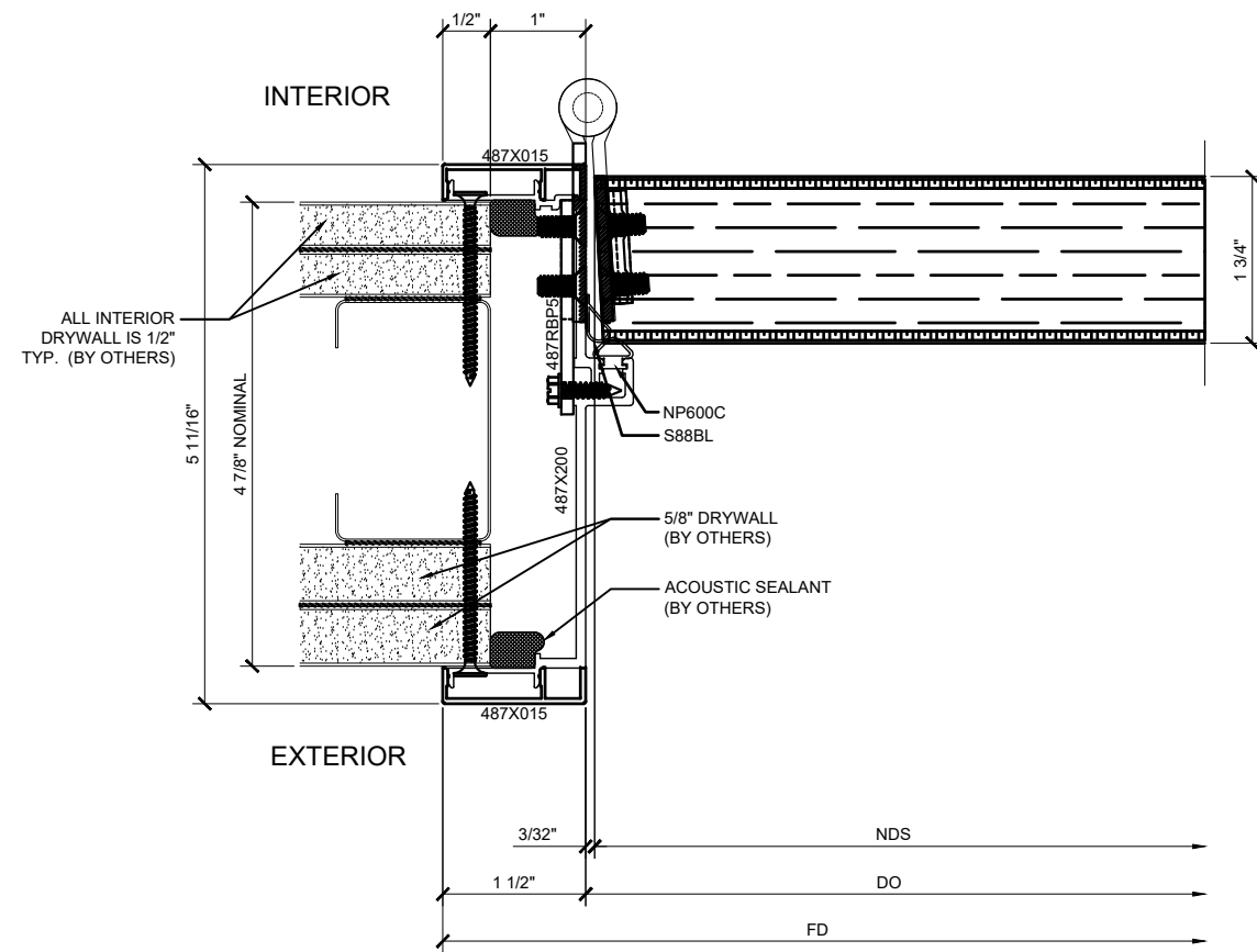
① DOOR JAMB DETAIL AT HINGE SIDE ARCH REF: 1'-0"=1'-0" SHOWN WITH AN STC - 35 DOOR AND FRAME
