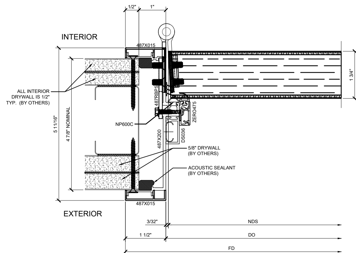
② DOOR JAMB DETAIL AT HINGE SIDE WITH RATED DOOR ARCH REF: 1'-0"=1'-0" SHOWN WITH AN STC - 39 DOOR AND FRAME
