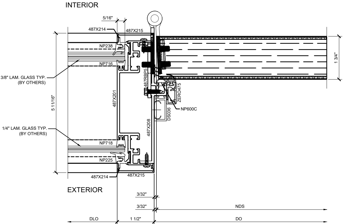
① DOOR JAMB DETAIL AT HINGE SIDE W/ SIDELITE WITH RATED DOOR
