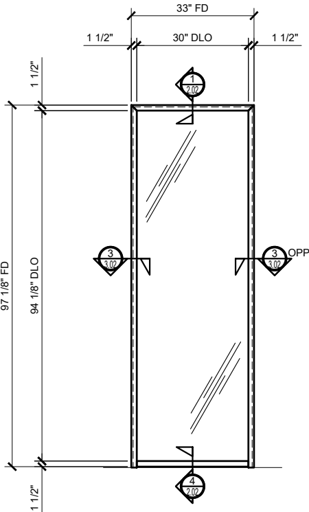
④ SINGLE BORROWED LITE TO FLOOR ARCH REF: NONE 3/4"=1'-0"
