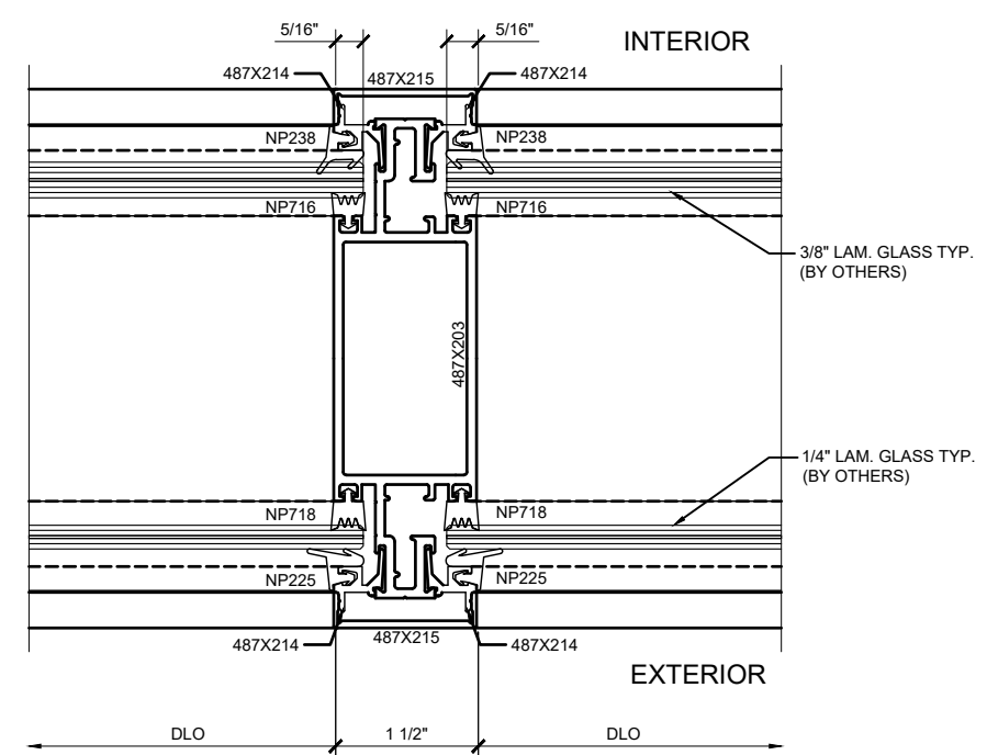
④ SIDELITE INTERMEDIATE VERTICAL DETAIL ARCH REF: 1'-0"=1'-0"
