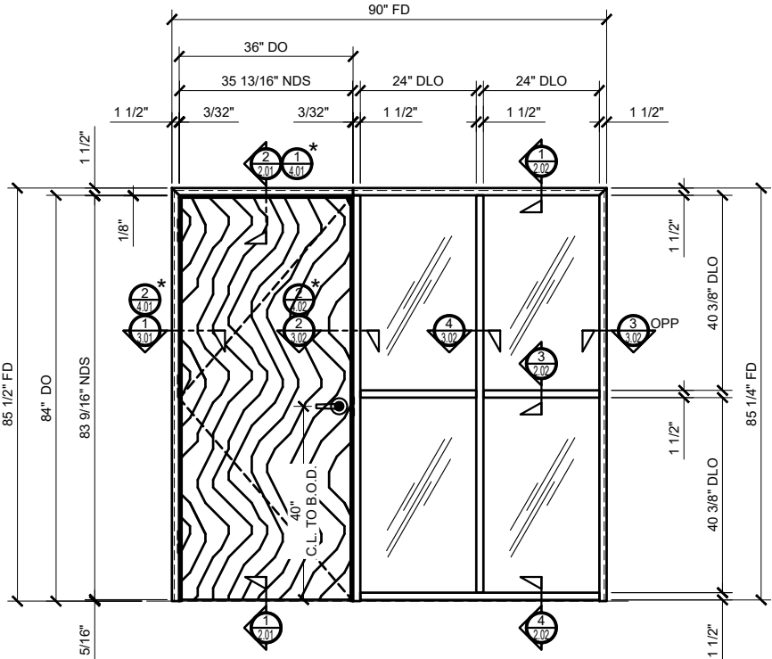
2 SINGLE BUTT HUNG DOOR WITH MULTIPLE SIDELITES
