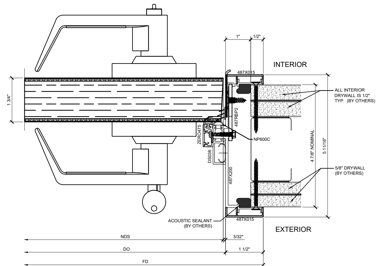
③ DOOR JAMB DETAIL AT STRIKE SIDE WITH RATED DOOR ARCH REF: 1'-0"=1'-0" SHOWN WITH AN STC - 39 DOOR AND FRAME
