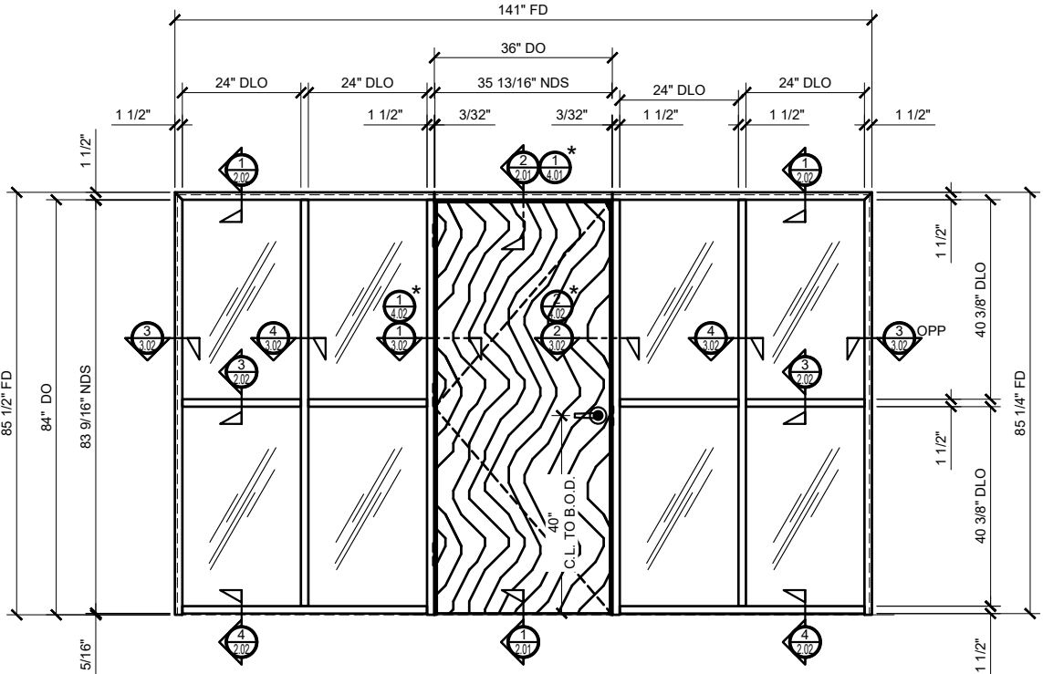
1 SINGLE BUTT HUNG DOOR WITH MULTIPLE SIDELITES BOTH SIDES
