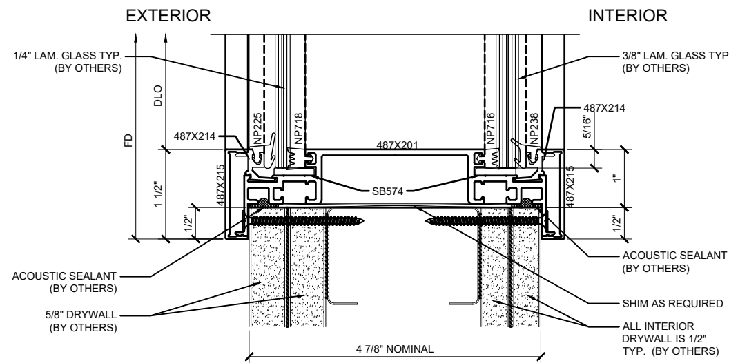
② SIDELITE SILL DETAIL ABOVE FLOOR ARCH REF: 1'-0"=1'-0"
