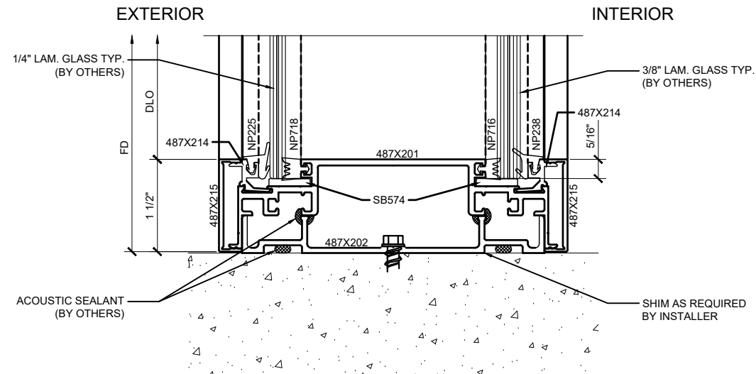
④ SIDELITE SILL DETAIL AT FLOOR ARCH REF: 1'-0"=1'-0"
