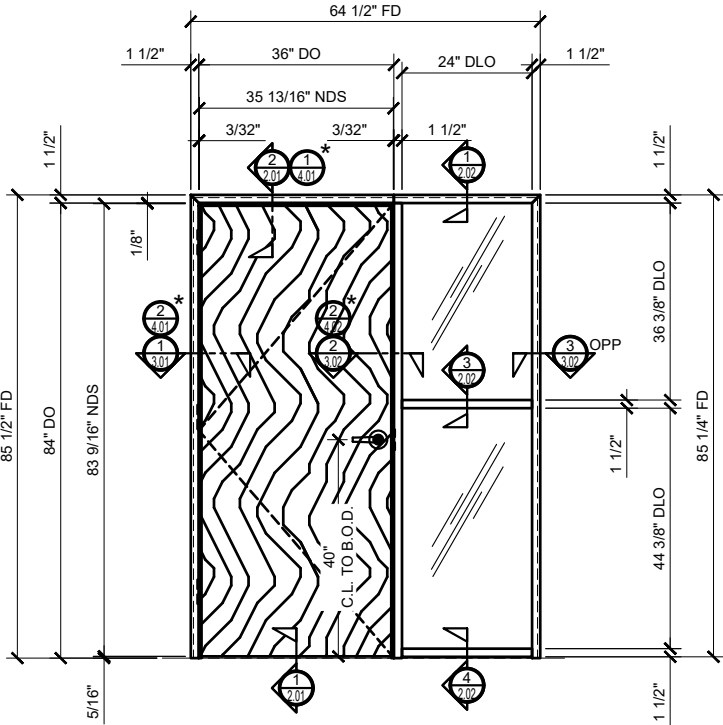
③ SINGLE BUTT HUNG DOOR WITH SIDELITE TO FLOOR ARCH REF: NONE 3/4"=1'-0"
