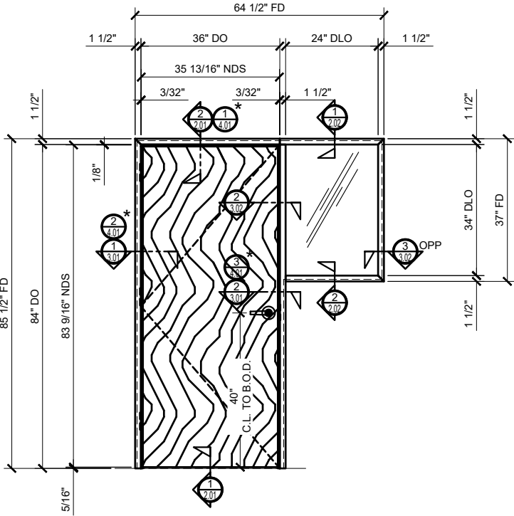
② SINGLE BUTT HINGE HUNG DOOR WITH SIDELITE ABOVE FLOOR ARCH REF: NONE 3/4"=1'-0"
