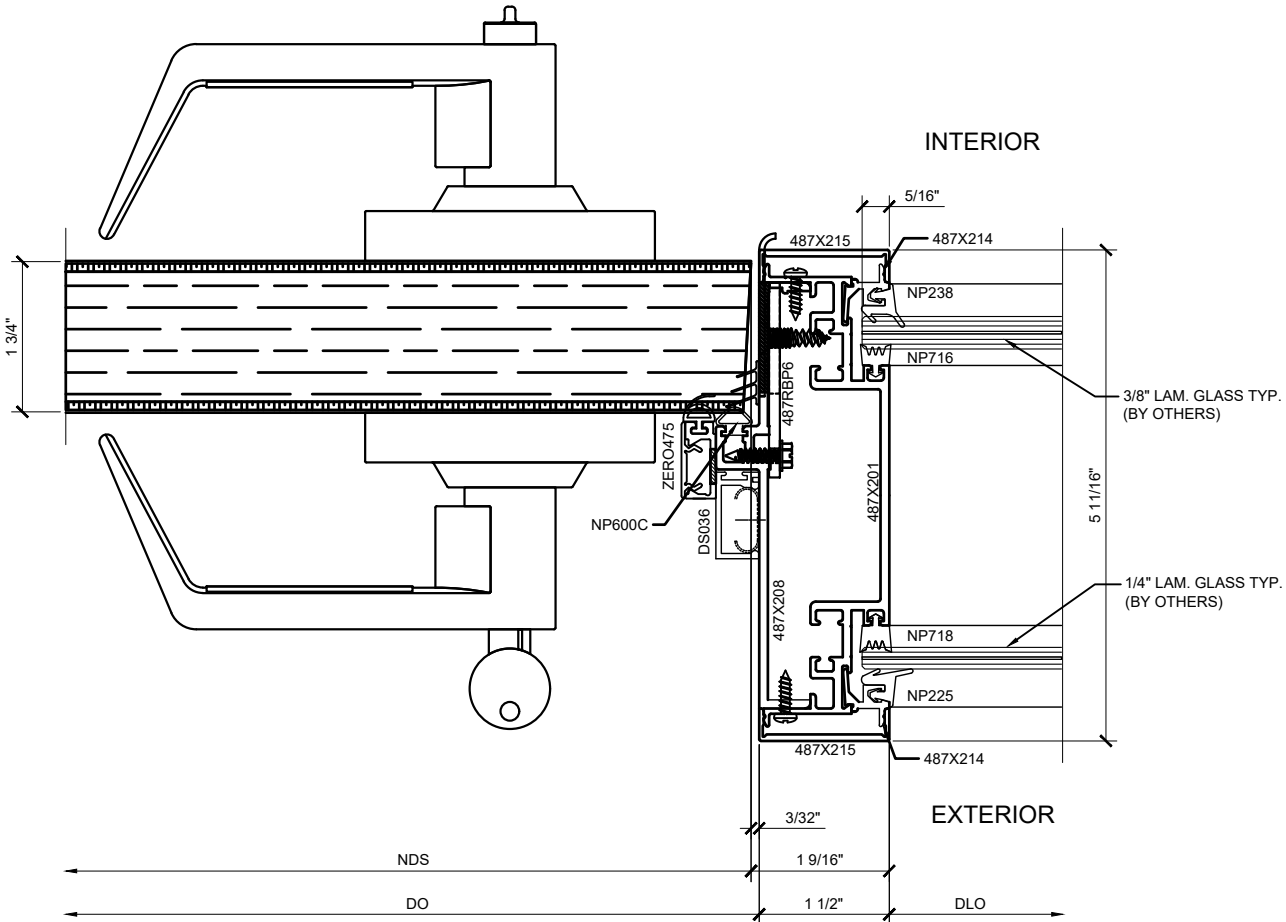
② DOOR JAMB DETAIL AT STRIKE SIDE W/ SIDELITE WITH RATED DOOR
