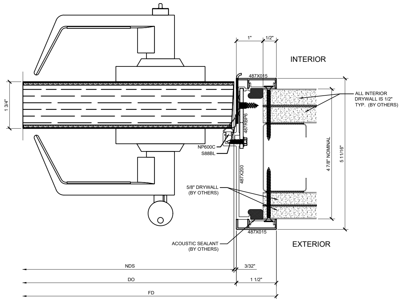
② DOOR JAMB DETAIL AT STRIKE SIDE ARCH REF: 1'-0"=1'-0" SHOWN WITH AN STC - 35 DOOR AND FRAME
