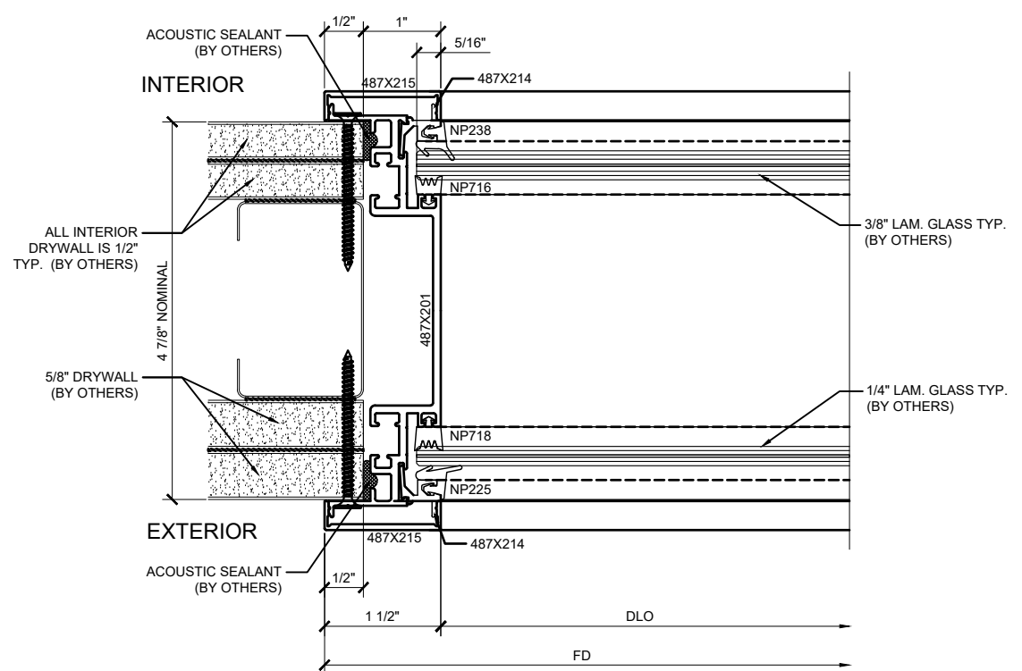
③ SIDELITE JAMB DETAIL ARCH REF: 1'-0"=1'-0"
