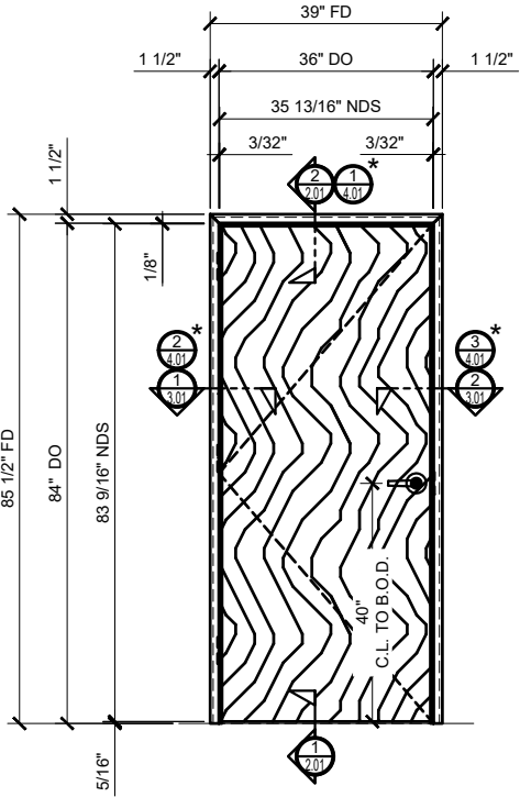
① SINGLE BUTT HUNG DOOR ARCH REF: NONE 3/4"=1'-0"
