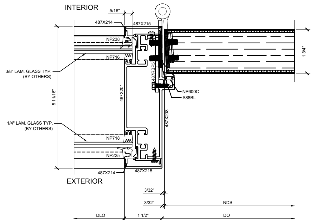
① DOOR JAMB DETAIL AT HINGE SIDE W/ SIDELITE ARCH REF: 1'-0"=1'-0" SHOWN WITH AN STC - 35 DOOR AND FRAME
