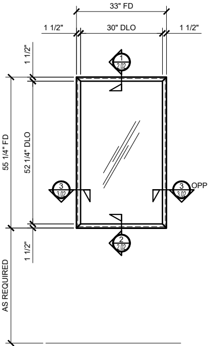
⑤ SINGLE BORROWED LITE ABOVE FLOOR ARCH REF: NONE 3/4"=1'-0"
