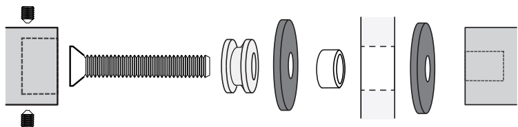
5/16"-18 Back-to-Back Glass Door Mount Shown
