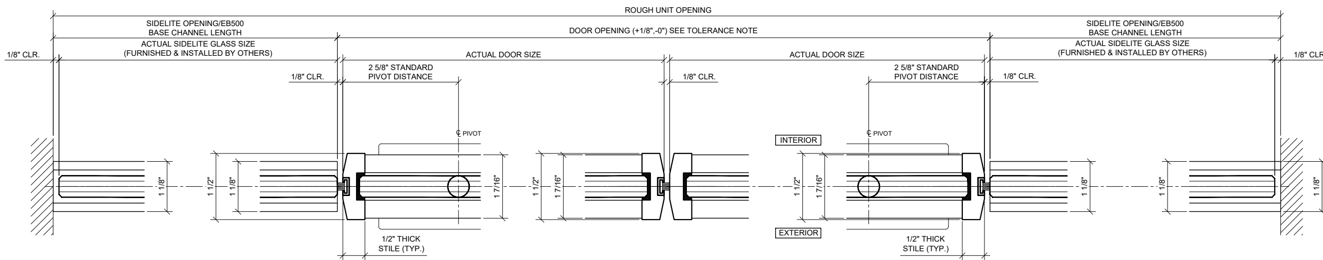
1A PLAN: WALL TO SIDE LITE 1B PLAN: SIDELITE TO DOOR 1C PLAN: MEETING STILE 1D PLAN: DOOR TO SIDELITE 1E PLAN: SIDELITE TO WALL
