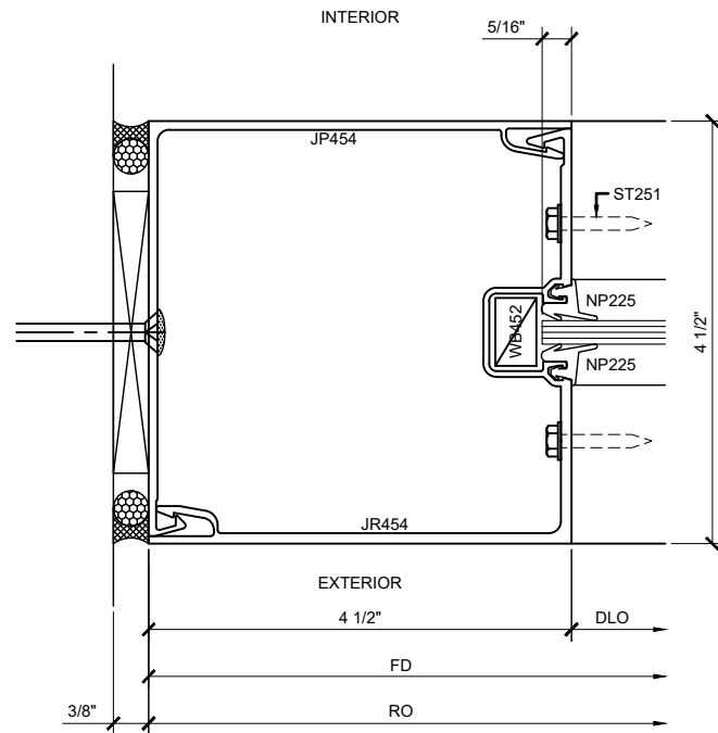
SECTION DETAIL AT WIDE STYLE JAMB ①
