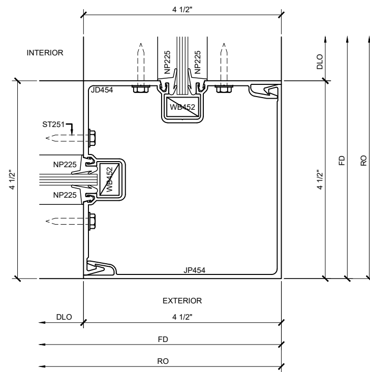
SECTION DETAIL AT WIDE STYLE CORNER VERTICAL ④
