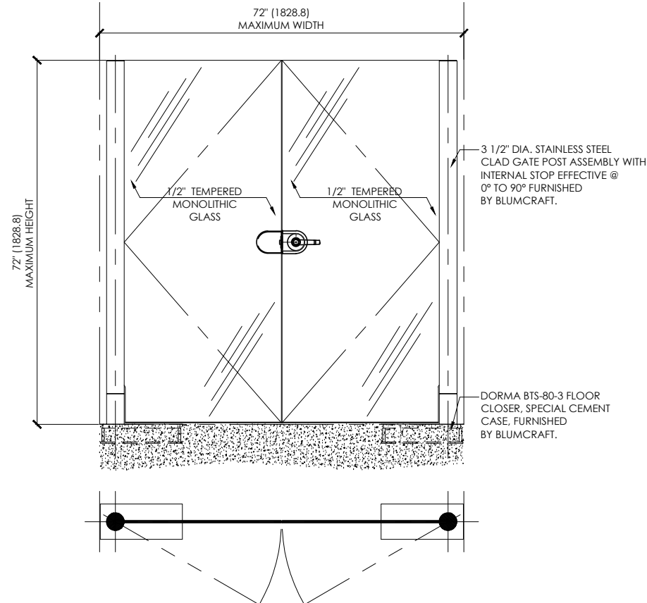
TYPICAL BLUMCRAFT 1200 SERIES GLASS GATE ELEVATION FREE STANDING FRAMELESS GATE SYSTEM
