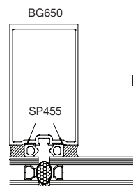
③ LEFT JAMBS
