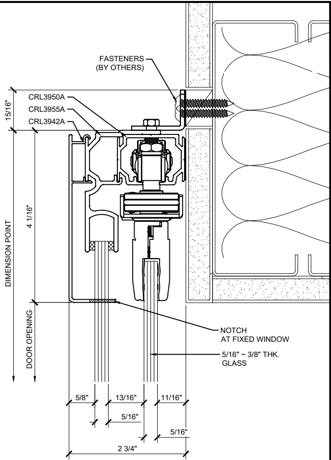
④ SECTION DETAIL @ HEAD ARCH REF: NONE 1'-0"=1'-0"
