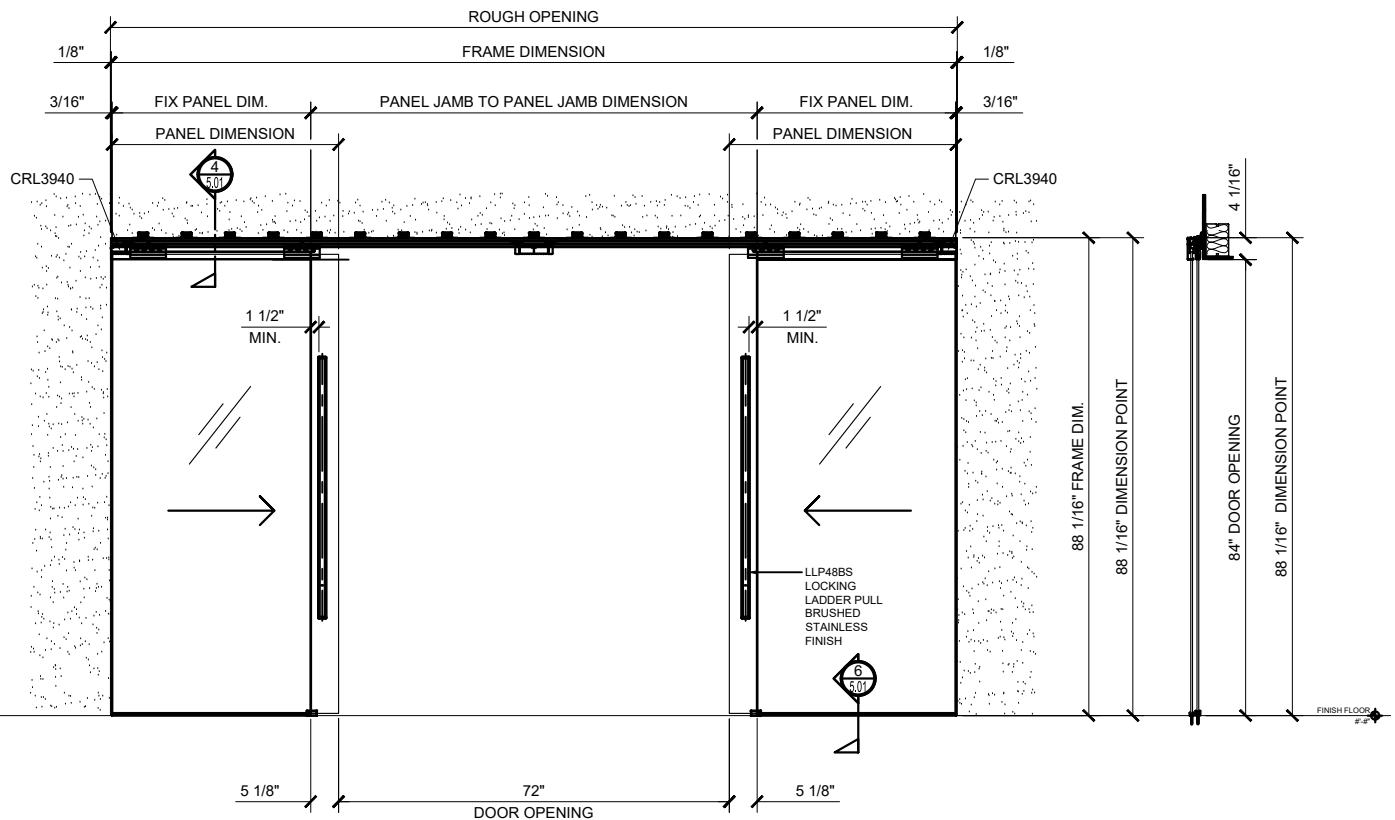
②A CRL 502 S2 BI-PARTING w/ 2 FIXED PANELS SYNC. WALL MOUNT ~ DOOR OPENED ARCH REF: NONE 3/4"=1'-0"
