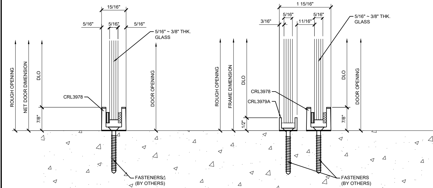
⑤ SECTION DETAIL @ SILL ARCH REF: NONE 1'-0"=1'-0"
