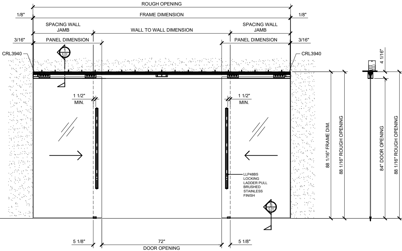
①A CRL 50 CS2 BI-PARTING SYNC. CEILING MOUNT ~ DOOR OPENED ARCH REF: NONE 3/4"=1'-0"
