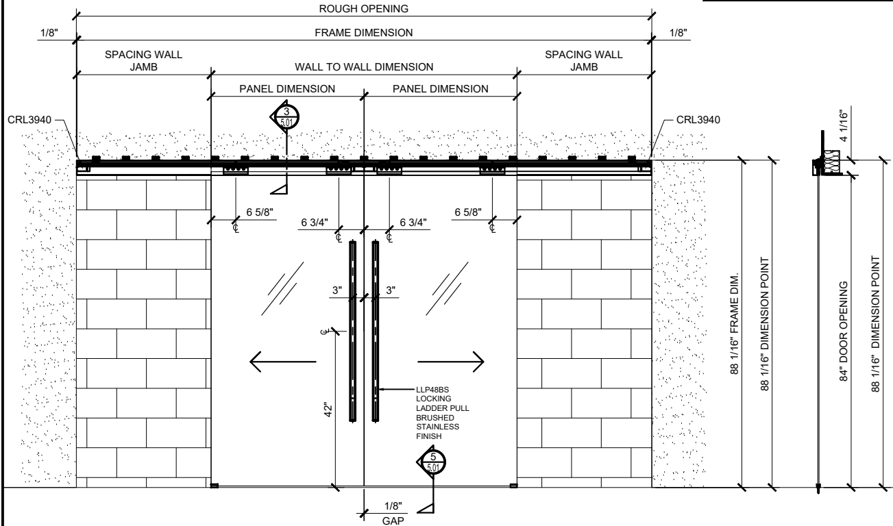
① CRL 50 S2 BI-PARTING SYNC. WALL MOUNT ~ DOOR CLOSED ARCH REF: NONE 3/4"=1'-0"
