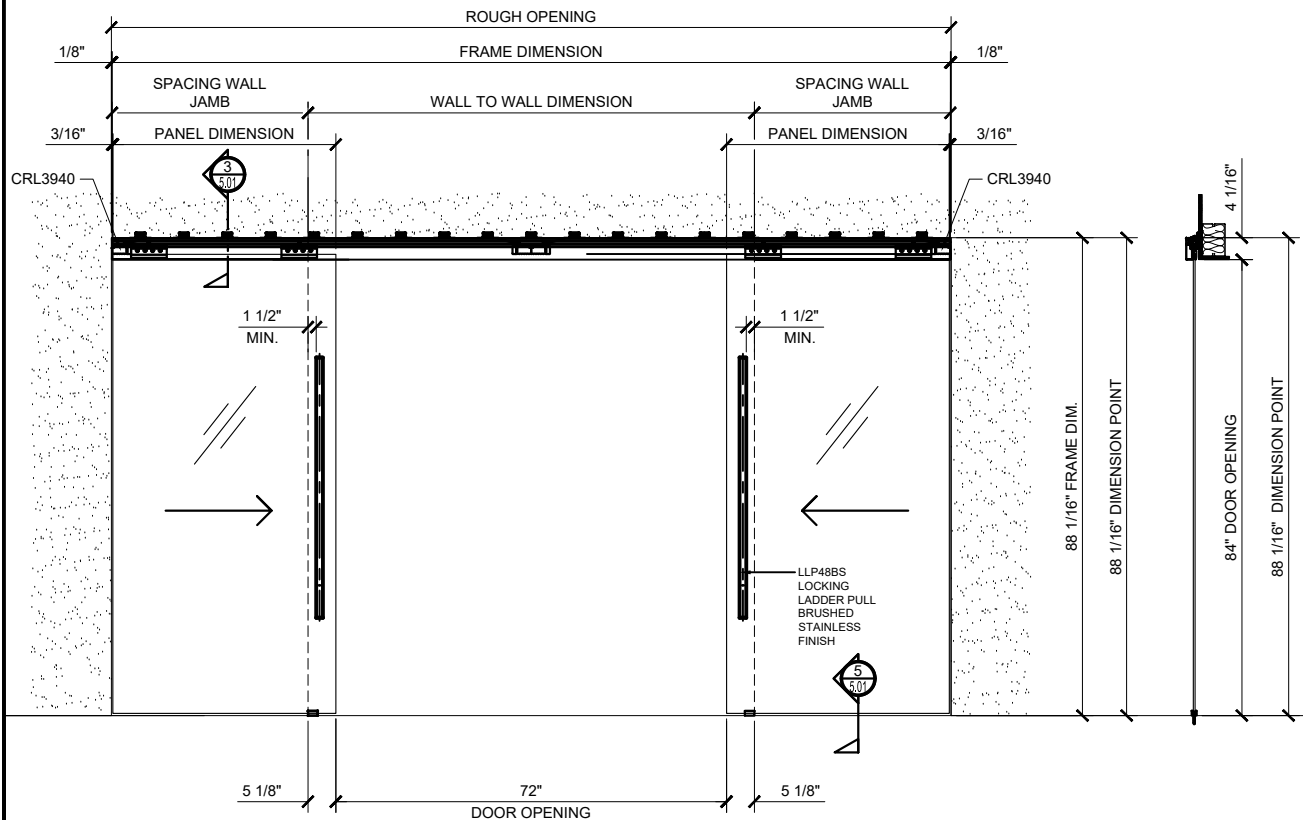
①A CRL 50 S2 BI-PARTING SYNC. WALL MOUNT ~ DOOR OPENED ARCH REF: NONE 3/4"=1'-0"
