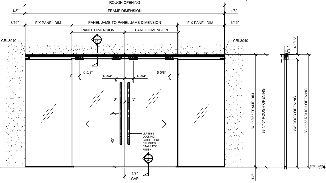
② CRL 502 CS2 BI-PARTING w/ 2 FIXED PANELS SYNC. CEILING MOUNT ~ DOOR CLOSED ARCH REF: NONE 3/4"=1'-0"
