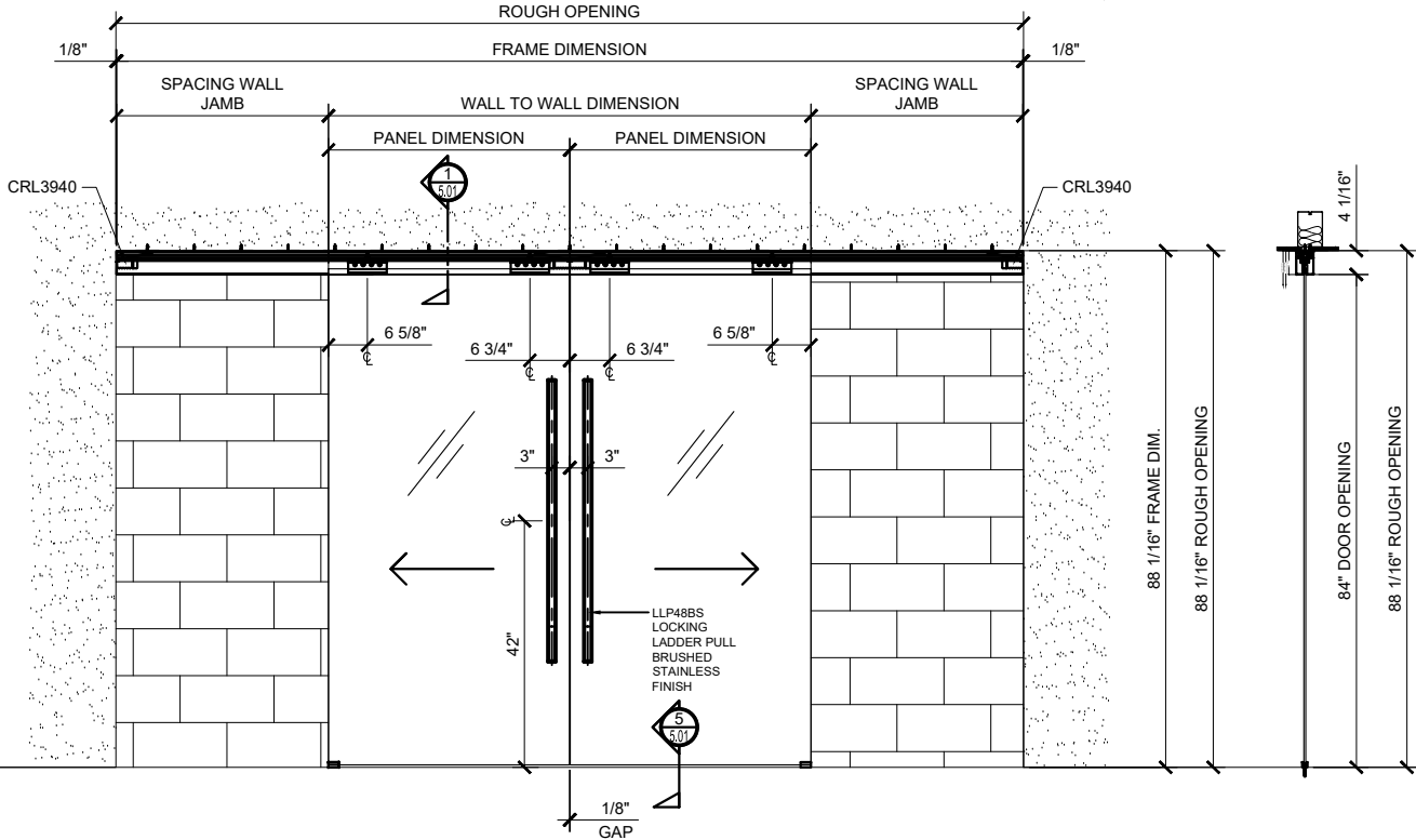
① CRL 50 CS2 BI-PARTING SYNC. CEILING MOUNT ~ DOOR CLOSED ARCH REF: NONE 3/4"=1'-0"
