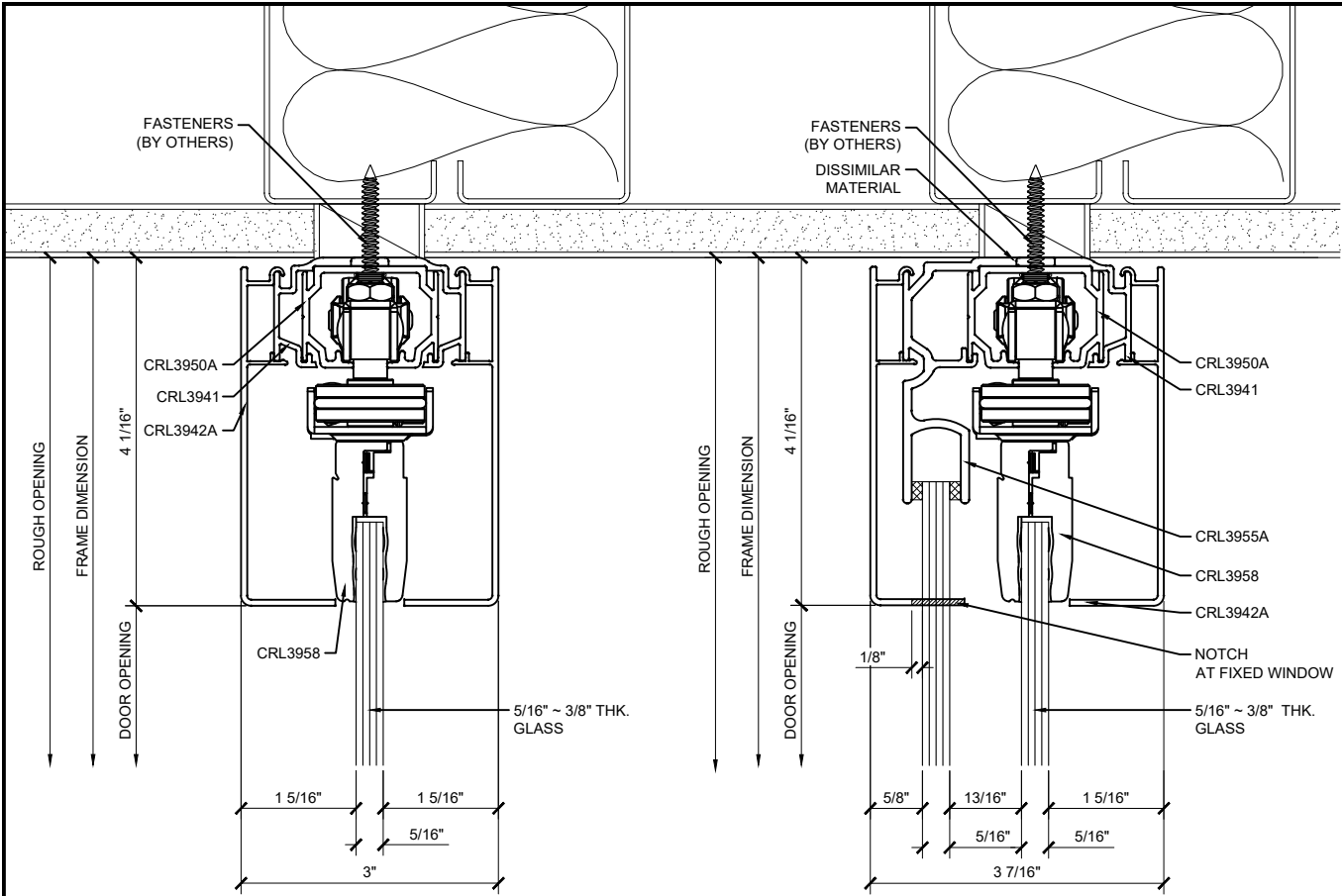
① SECTION DETAIL @ HEAD ARCH REF: NONE 1'-0"=1'-0"
