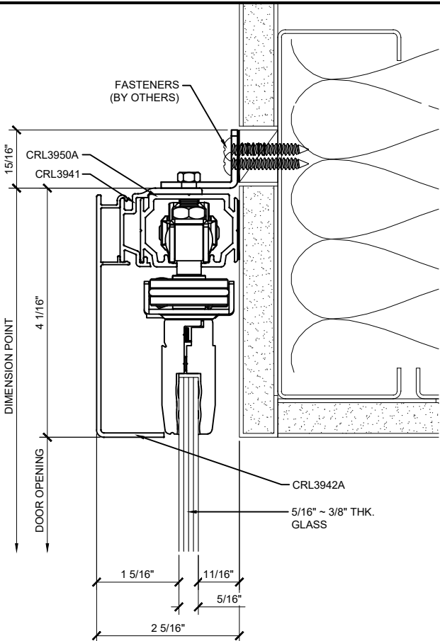
③ SECTION DETAIL @ HEAD ARCH REF: NONE 1'-0"=1'-0"
