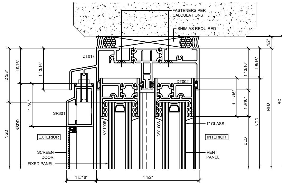
③ SCREEN DOOR / FIXED PANEL / VENT PANEL SECTION DETAIL AT HEAD
