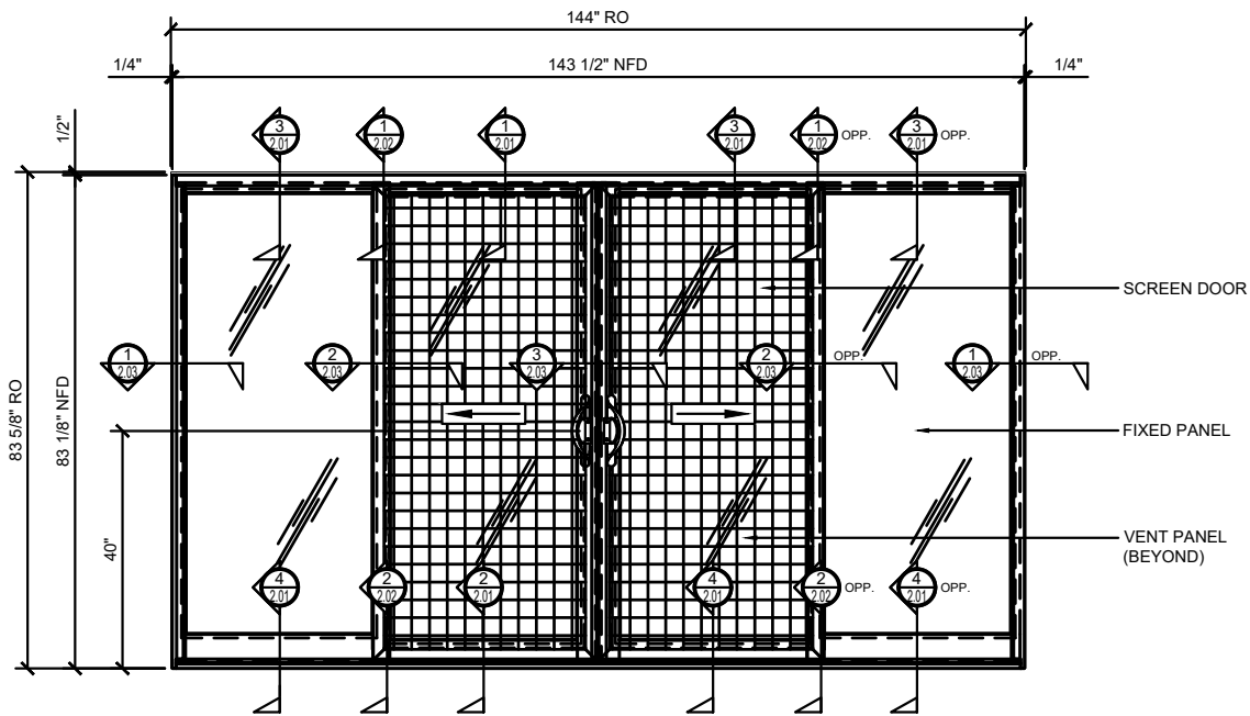
CRL 3025 SERIES SLIDING DOOR ELEVATION - OXOX CONFIGURATION FIN FRAME APPLICATION
