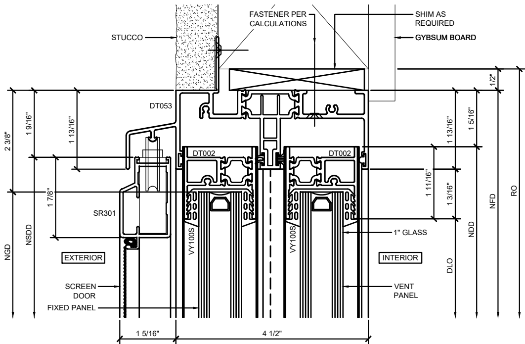
① SCREEN DOOR / FIXED PANEL / VENT PANEL SECTION DETAIL AT HEAD
