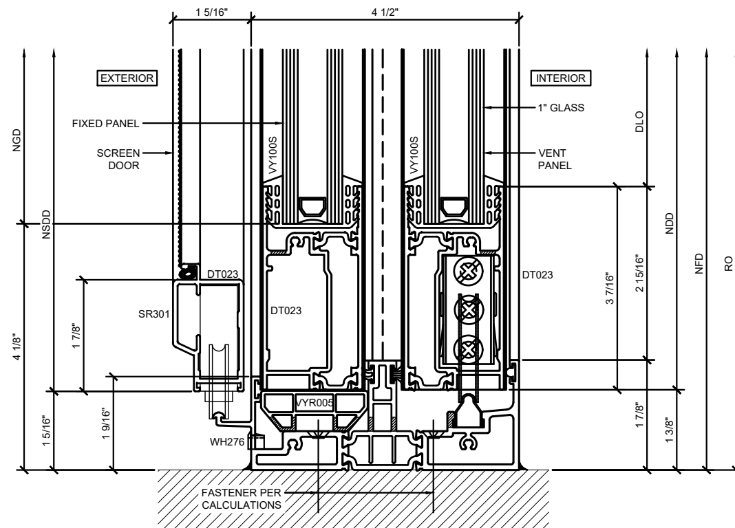
④ SCREEN DOOR / FIXED PANEL / VENT PANEL SECTION DETAIL AT SILL
