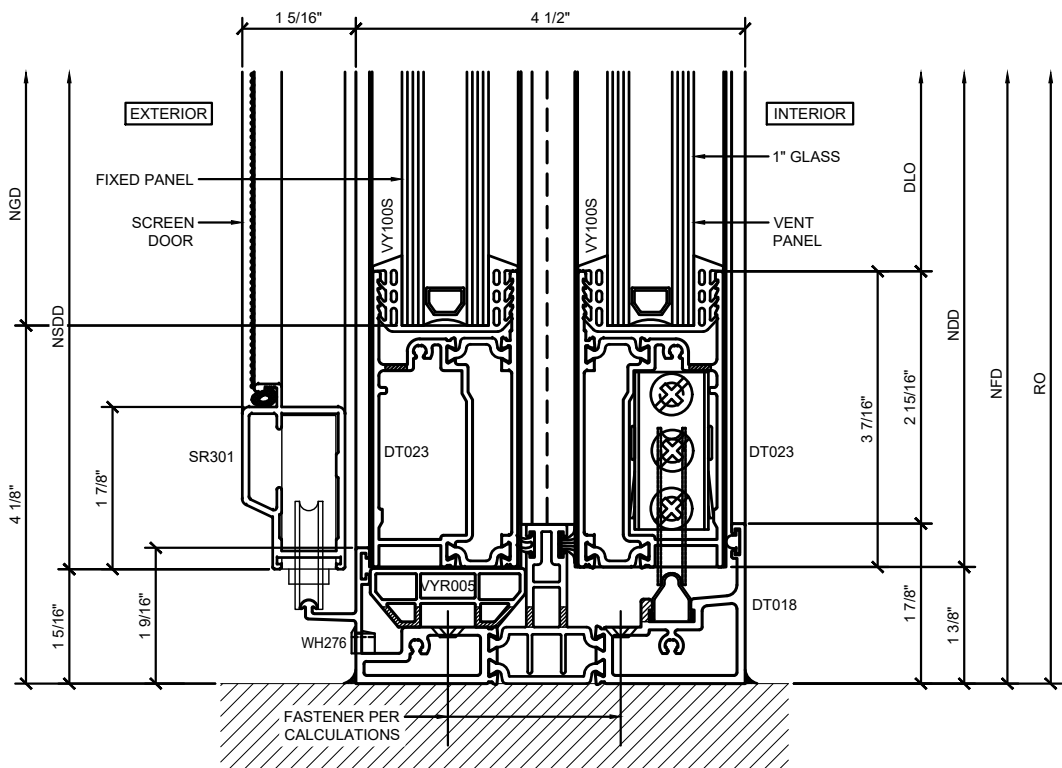
② SCREEN DOOR / FIXED PANEL / VENT PANEL SECTION DETAIL AT SILL
