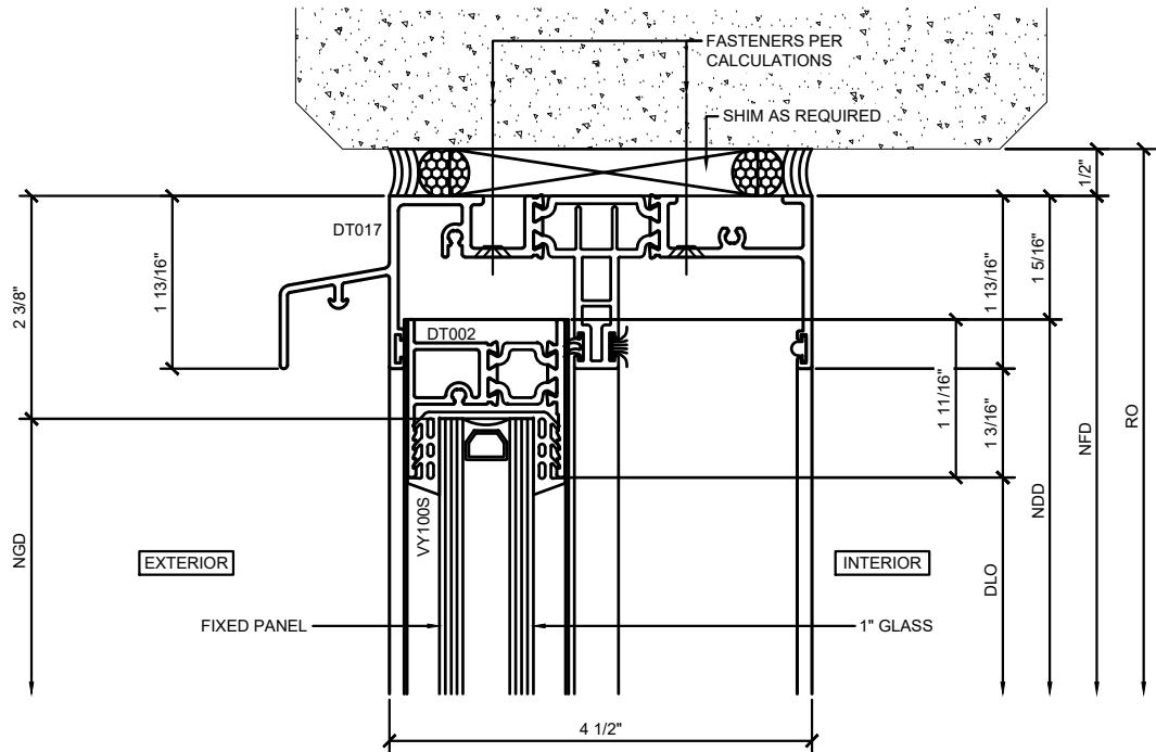
③ FIXED PANEL SECTION DETAIL AT HEAD
