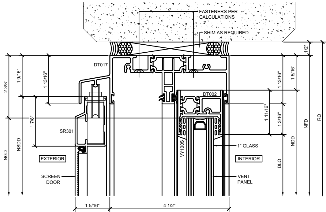
① SCREEN DOOR / VENT PANEL SECTION DETAIL AT HEAD
