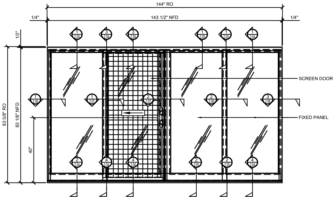
CRL 3025 SERIES SLIDING DOOR ELEVATION - OXOO(R) CONFIGURATION (AS SHOWN)
