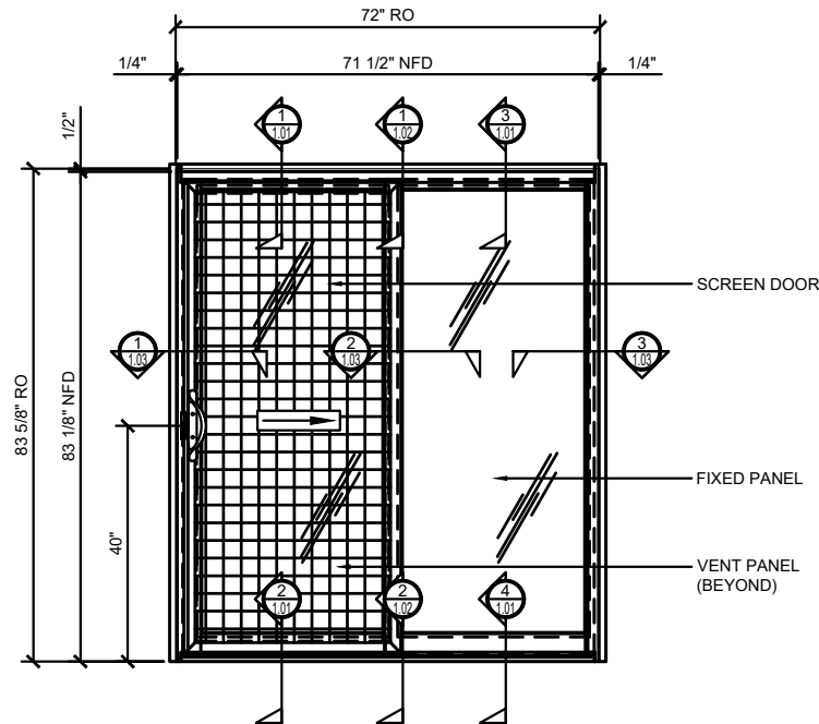
CRL 3025 SERIES SLIDING DOOR ELEVATION - XO CONFIGURATION FIN FRAME APPLICATION
