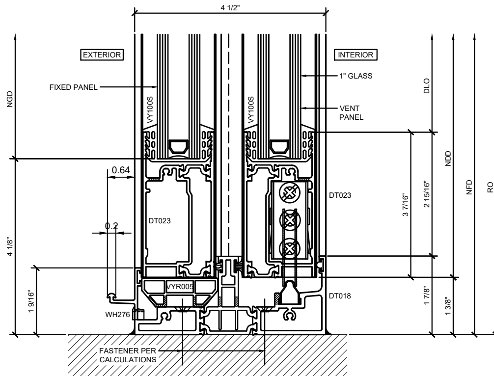
② FIXED PANEL / VENT PANEL SECTION DETAIL AT SILL
