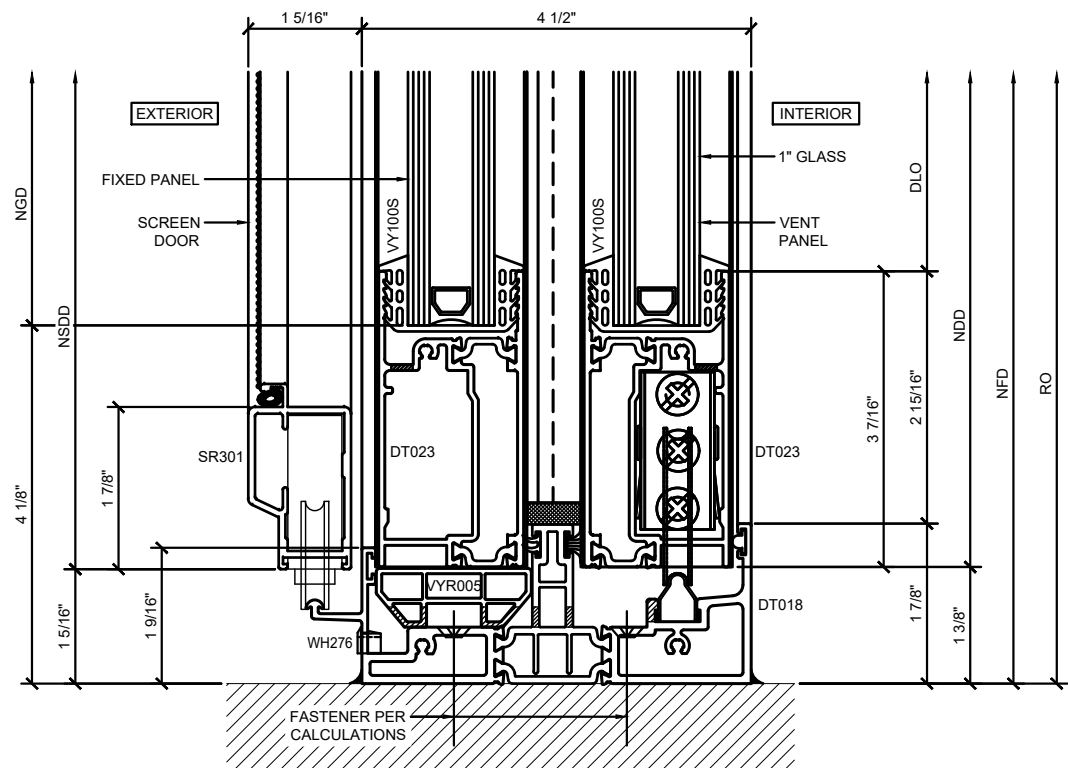
② SCREEN DOOR / FIXED PANEL / VENT PANEL SECTION DETAIL AT SILL ARCH REF: N/A 1'-0"=1'-0"
