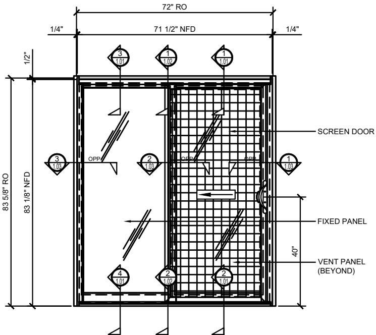
CRL 3025 SERIES SLIDING DOOR ELEVATION - OX CONFIGURATION FIN FRAME APPLICATION
