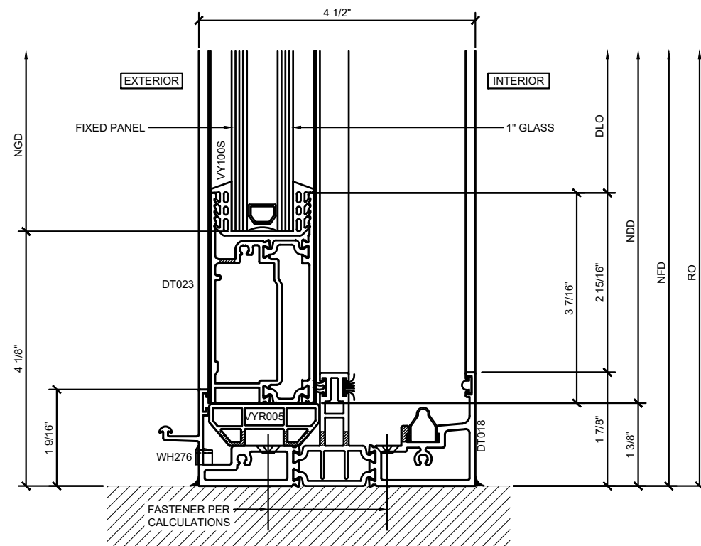
② FIXED PANEL SECTION DETAIL AT SILL
