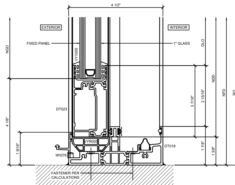
④ FIXED PANEL SECTION DETAIL AT SILL
