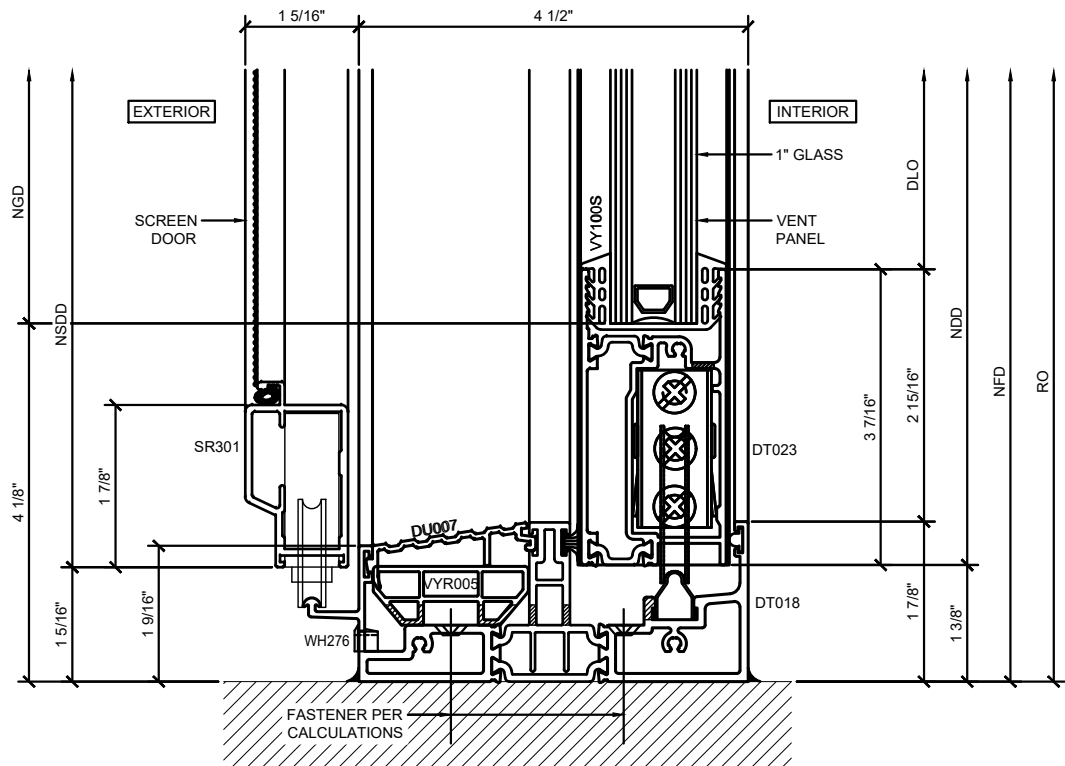
② SCREEN DOOR / VENT PANEL SECTION DETAIL AT SILL
