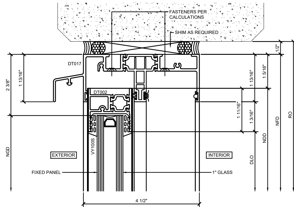
① FIXED PANEL SECTION DETAIL AT HEAD
