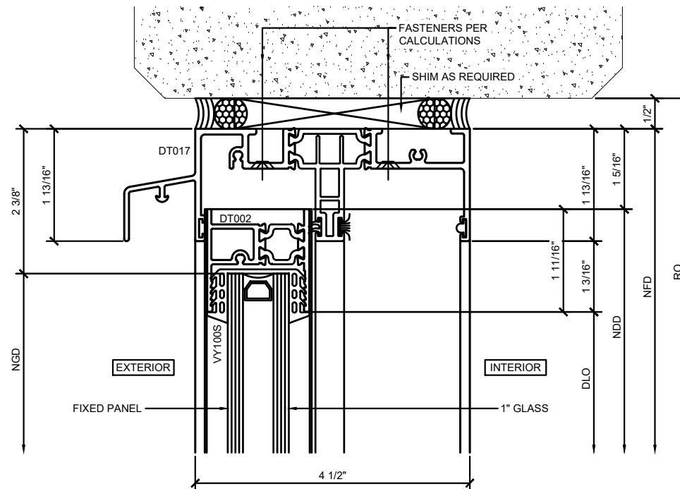
③ FIXED PANEL SECTION DETAIL AT HEAD
