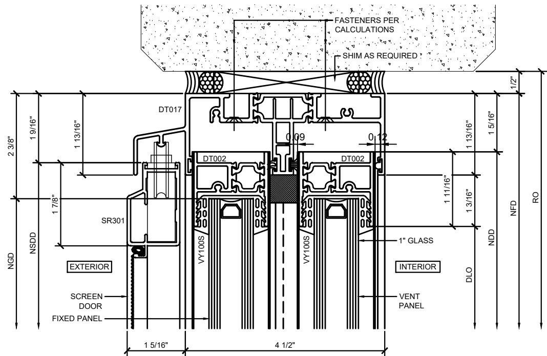
① SCREEN DOOR / FIXED PANEL / VENT PANEL SECTION DETAIL AT HEAD ARCH REF: N/A 1'-0"=1'-0"
