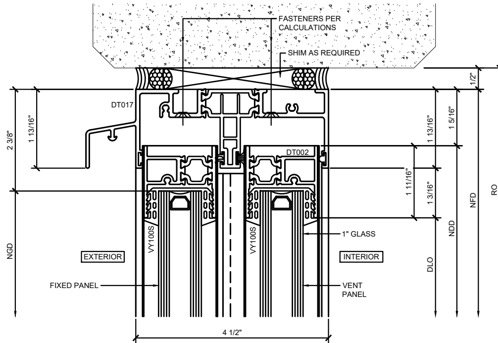
① FIXED PANEL / VENT PANEL SECTION DETAIL AT HEAD
