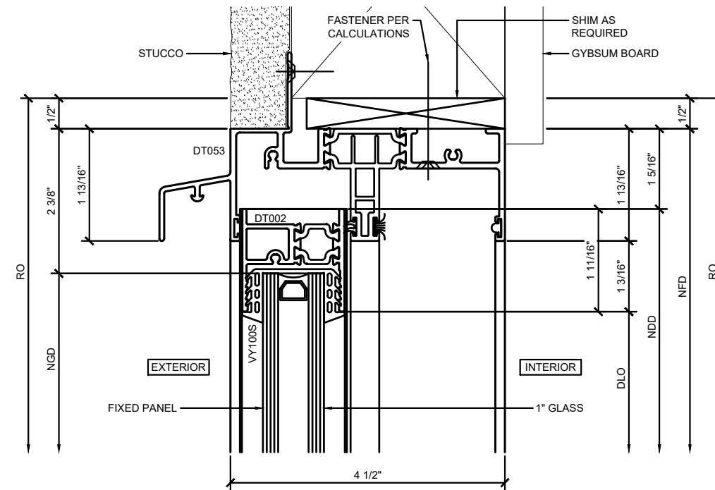
③ FIXED PANEL SECTION DETAIL AT HEAD
