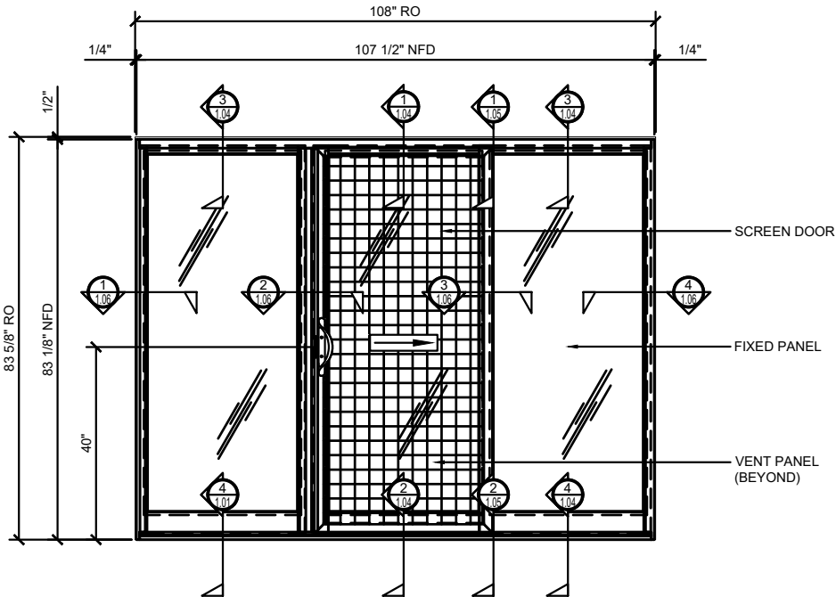
CRL 3025 SERIES SLIDING DOOR ELEVATION - OXO(R) CONFIGURATION (AS SHOWN)
