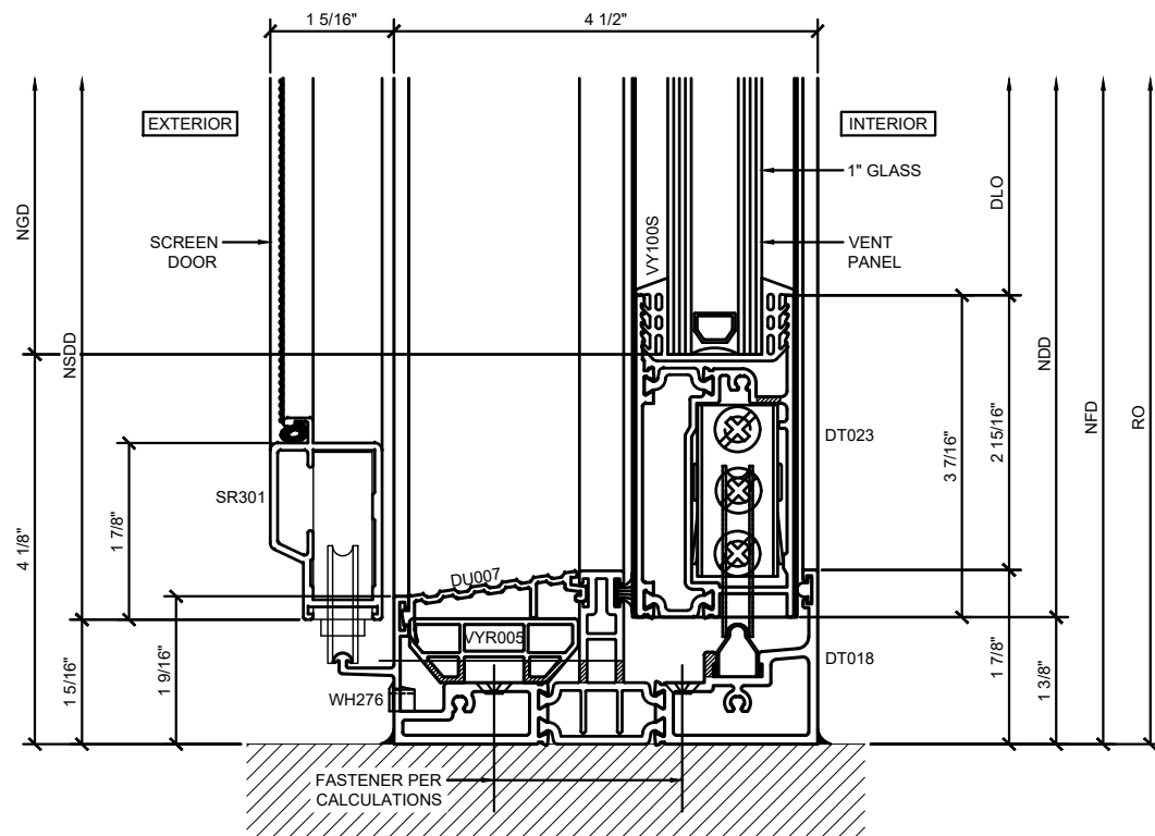
② SCREEN DOOR / VENT PANEL SECTION DETAIL AT SILL
