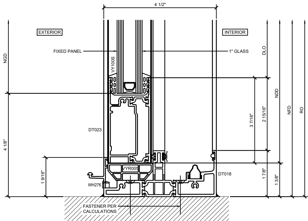
④ FIXED PANEL SECTION DETAIL AT SILL
