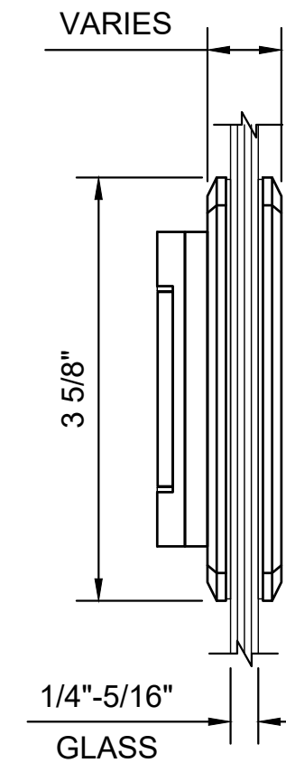
GLASS FABRICATION TEMPLATE
