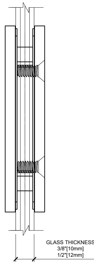
GLASS FABRICATION TEMPLATE
