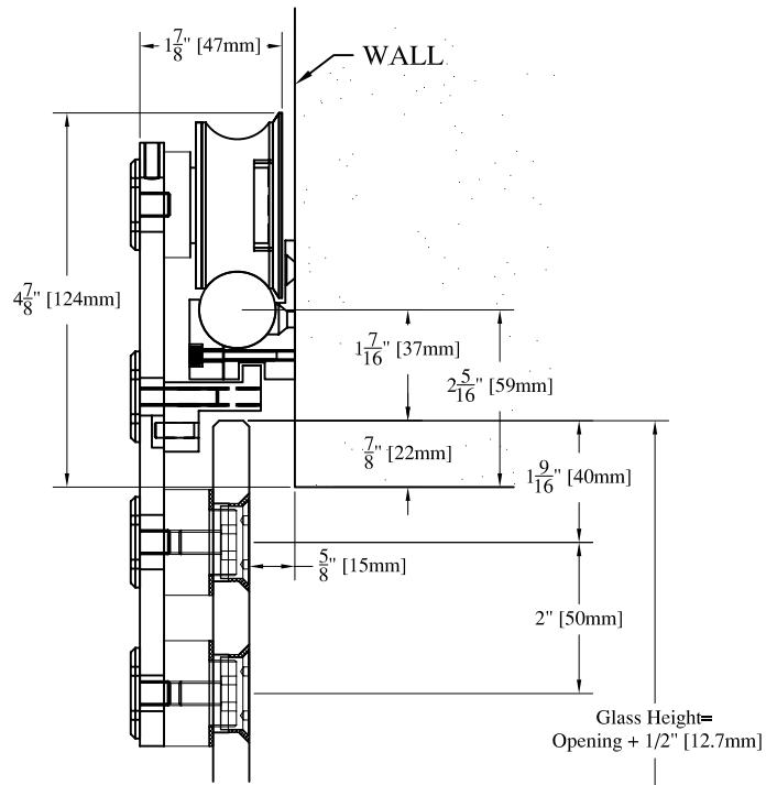
FLUSH MOUNT
