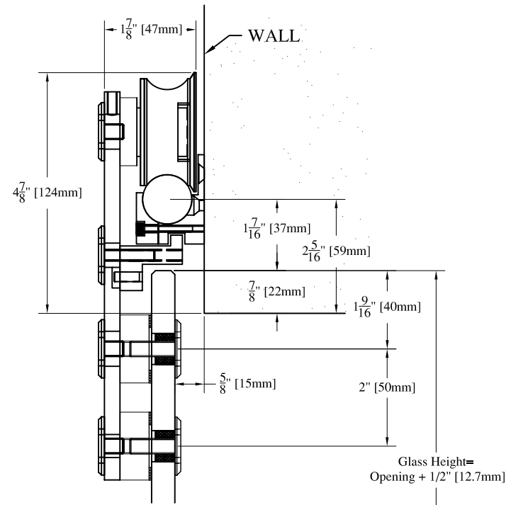
SURFACE MOUNT
