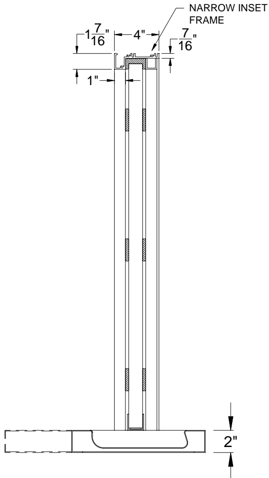
VERTICAL SECTION
