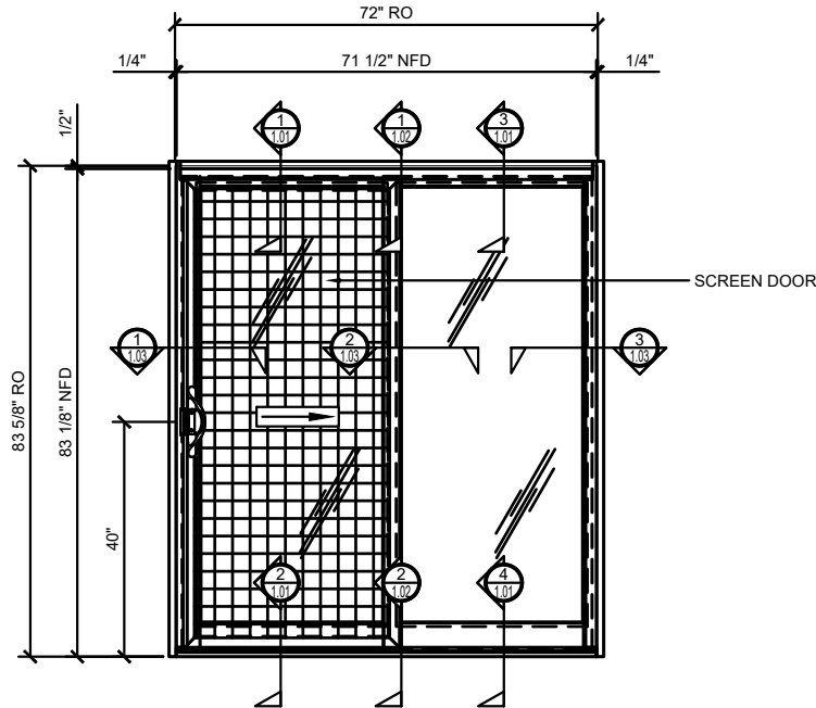
CRL 3040 SERIES SLIDING DOOR ELEVATION - XO CONFIGURATION FIN FRAME APPLICATION
