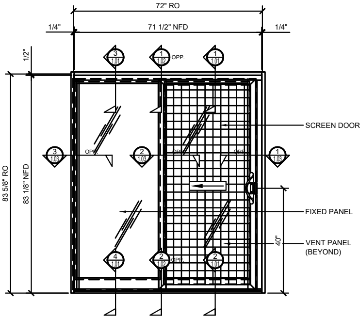
CRL 3040 SERIES SLIDING DOOR ELEVATION - OX CONFIGURATION FIN FRAME APPLICATION
