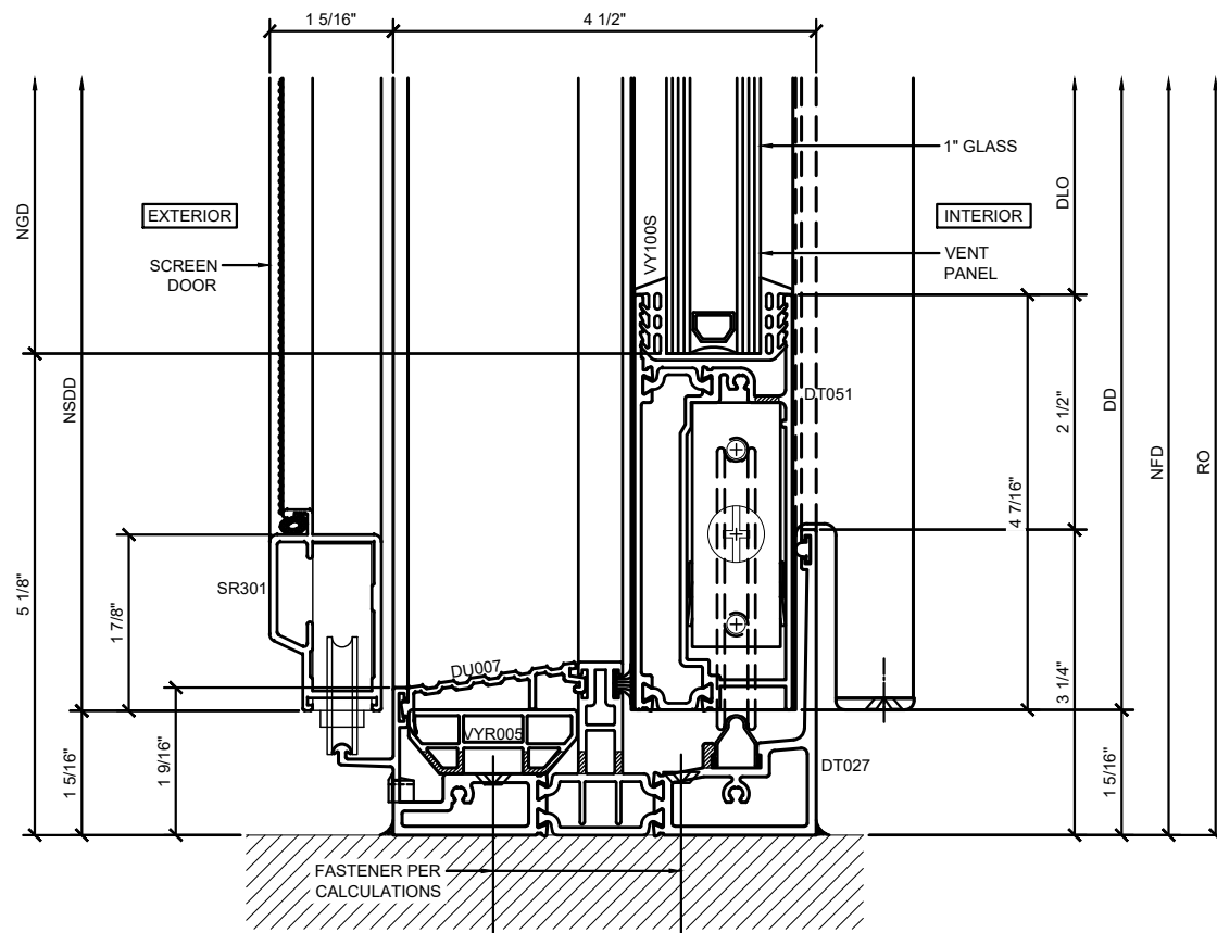
② SCREEN DOOR / VENT PANEL SECTION DETAIL AT SILL
