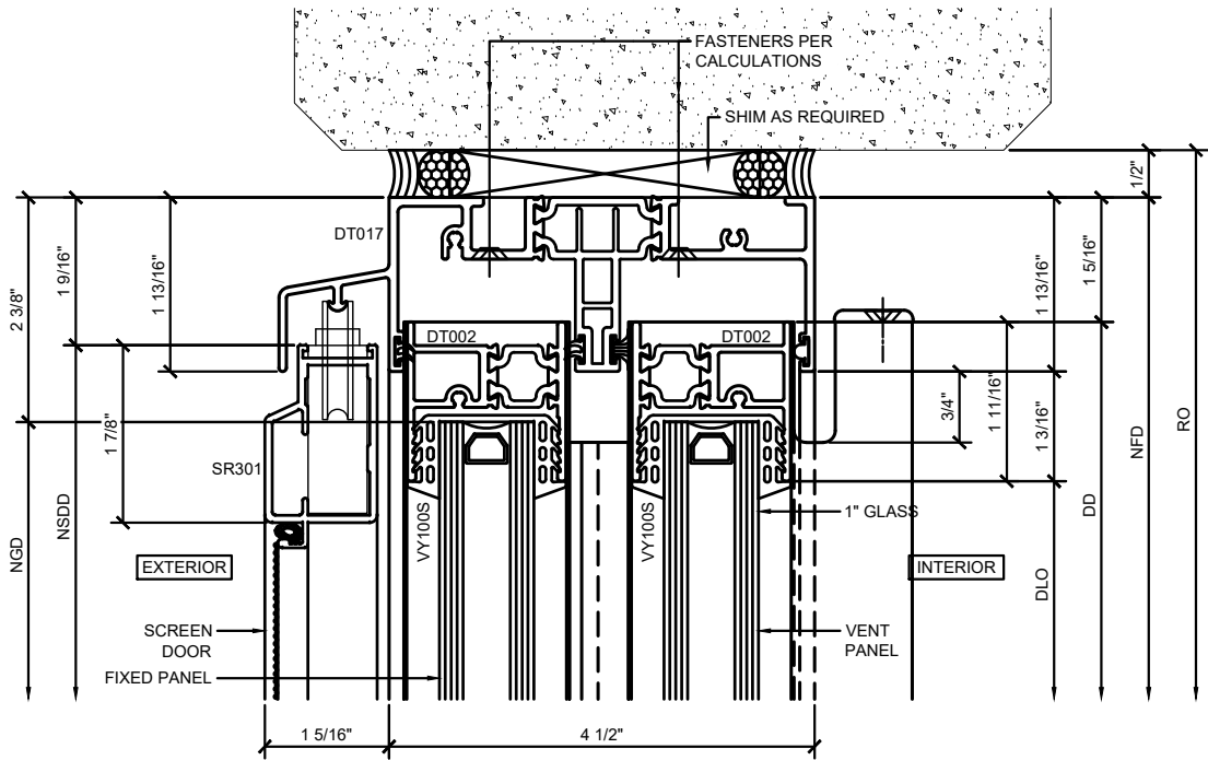
① SCREEN DOOR / FIXED PANEL / VENT PANEL SECTION DETAIL AT HEAD
