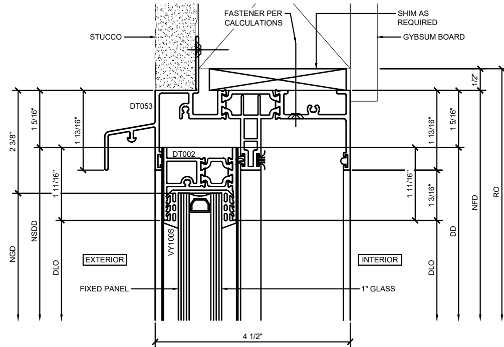
③ FIXED PANEL SECTION DETAIL AT HEAD
