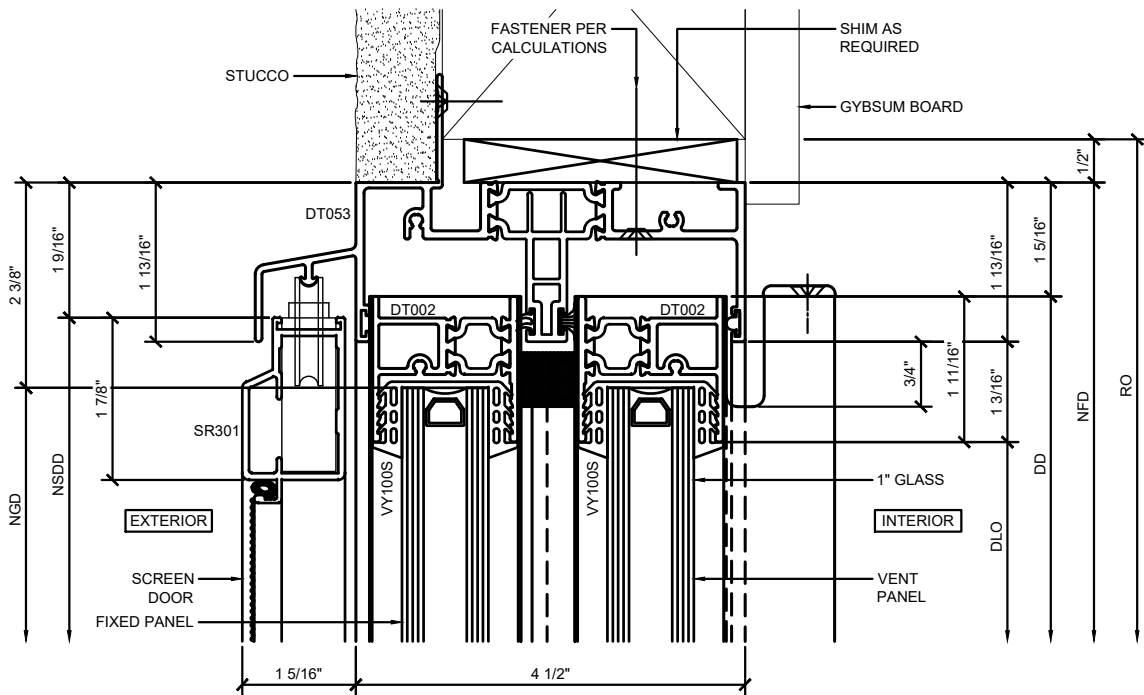
① SCREEN DOOR / FIXED PANEL / VENT PANEL SECTION DETAIL AT HEAD
