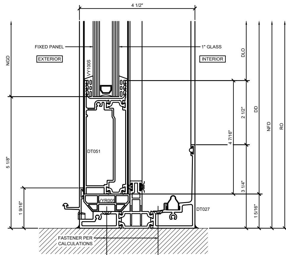
④ FIXED PANEL SECTION DETAIL AT SILL
