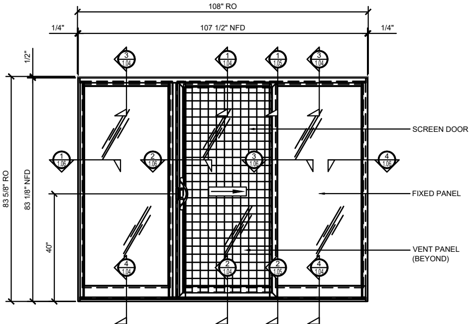
CRL 3040 SERIES SLIDING DOOR ELEVATION - OXO(R) CONFIGURATION (AS SHOWN) CRL 3040 SERIES SLIDING DOOR ELEVATION - OXO(L) CONFIGURATION (OPP)
