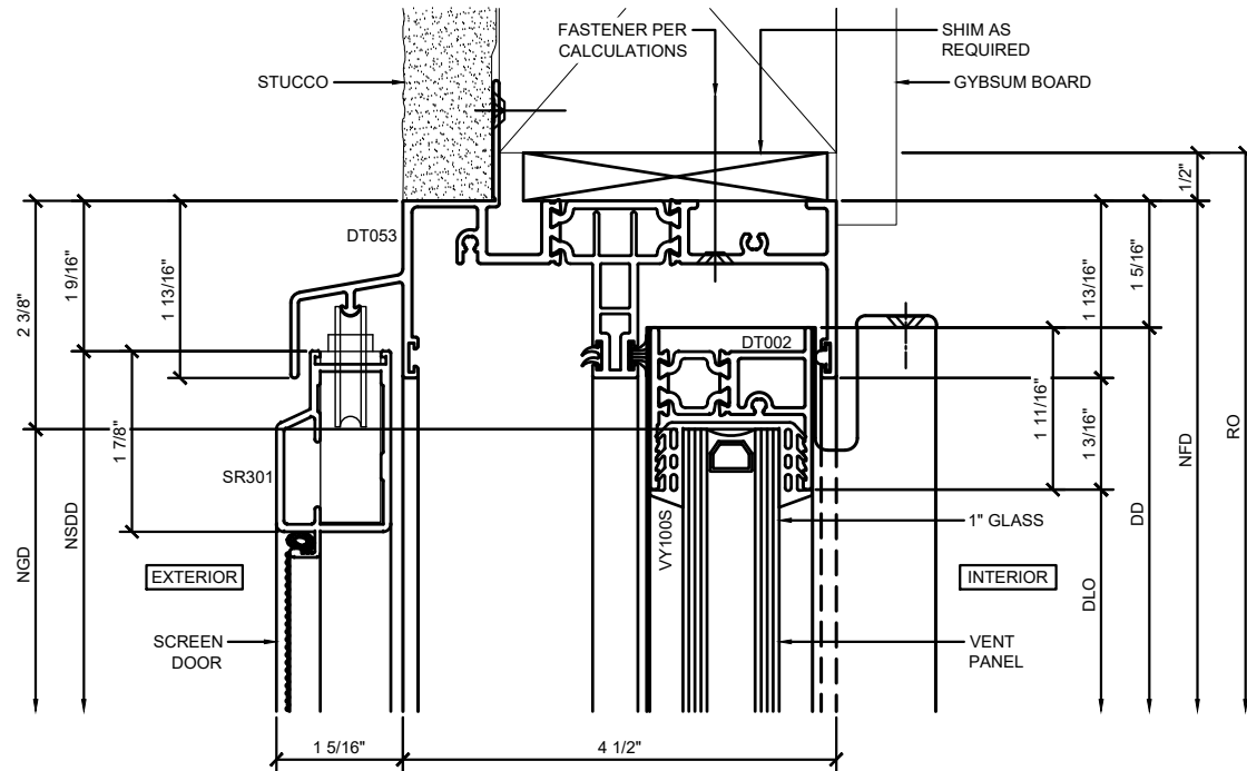
① SCREEN DOOR / VENT PANEL SECTION DETAIL AT HEAD
