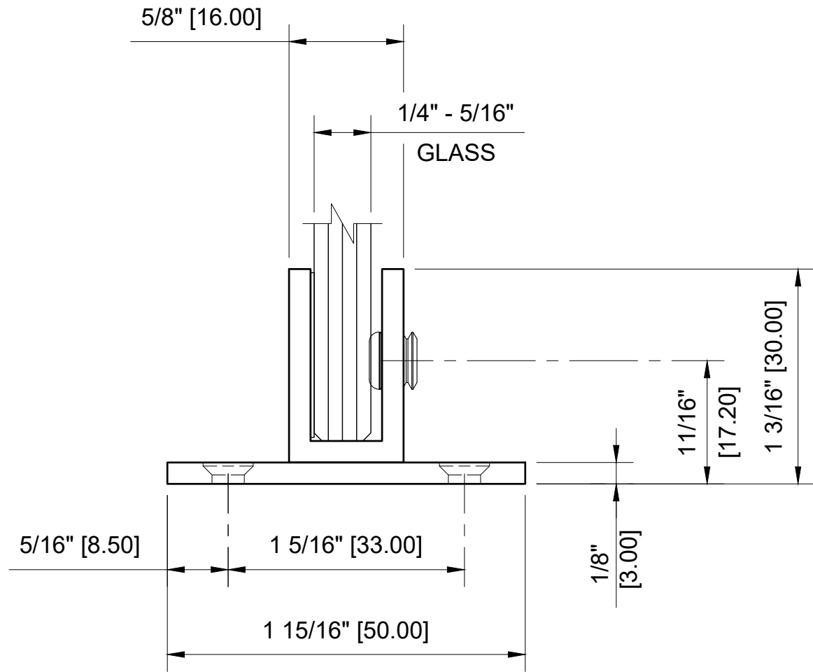
CRL - EH47 BRUSHED NICKEL SHORT LEG SET SCREW CLAMP FOR 1/4" - 5/16" GLASS
