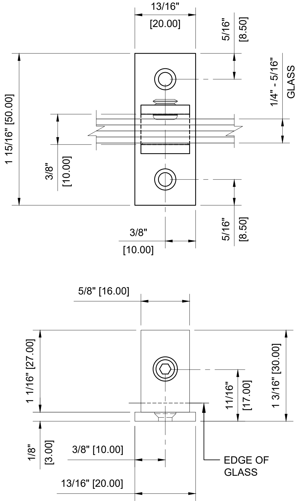
CRL - EH47 BRUSHED NICKEL SHORT LEG SET SCREW CLAMP FOR 1/4" - 5/16" GLASS
