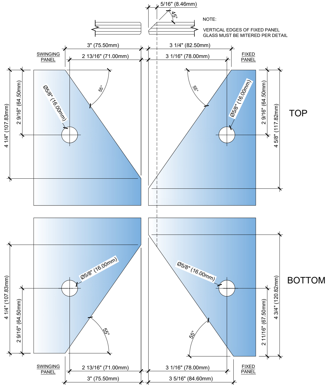
3A GLASS CUT OUT DETAIL - 1MM FIXED PANEL GAP ARCH REF: SCALE: 1'-0"=1'-0"
