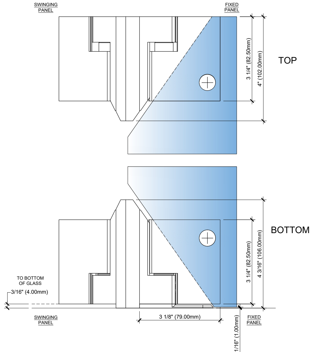
2A SIDE VIEW DETAIL @1MM FIXED PANEL GAP ARCH REF: SCALE: 1'-0"=1'-0"
