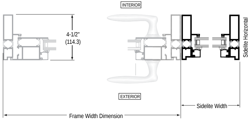
SINGLE DOOR WITH SIDELITE SHOWN
