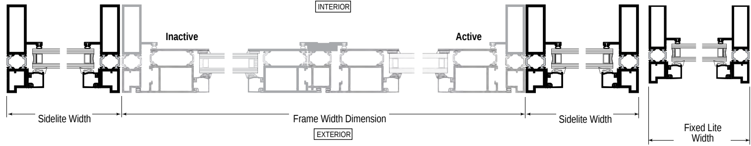
PAIR OF DOORS WITH SIDELITE SHOWN
