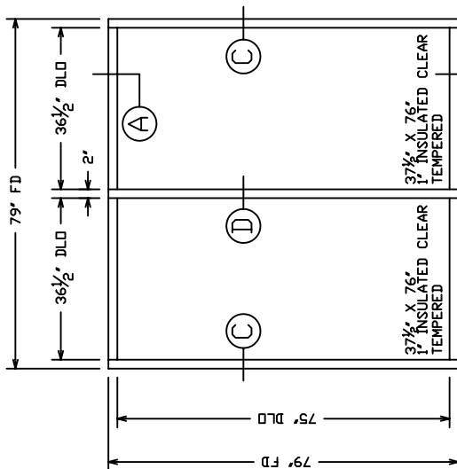
ELEVATION DRAWING NOT TO SCALE
