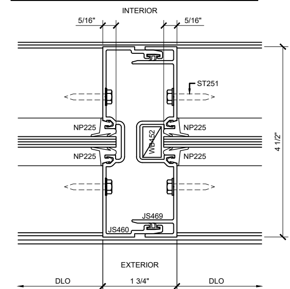
SECTION DETAIL AT EXPANSION MULLION ⑦
