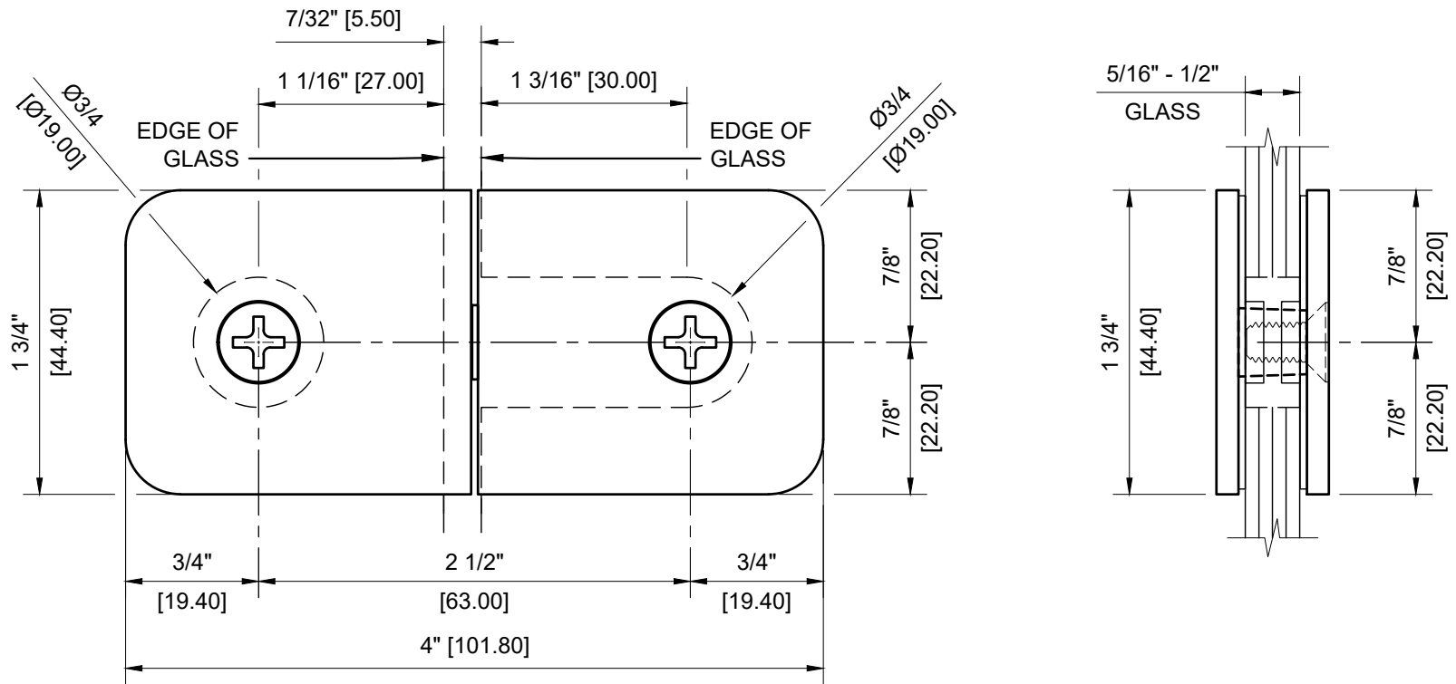
CRL - GCB188 180 DEGREE GLASS TO GLASS STANDARD MOVABLE TRANSOM 5/16" - 1/2" GLASS
