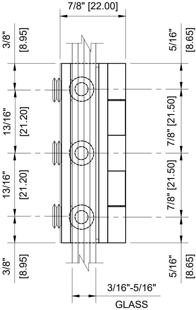
CRL - EH168 LARGE 2-3/8" WALL MOUNT HINGE FOR 3/16" - 5/16" GLASS
