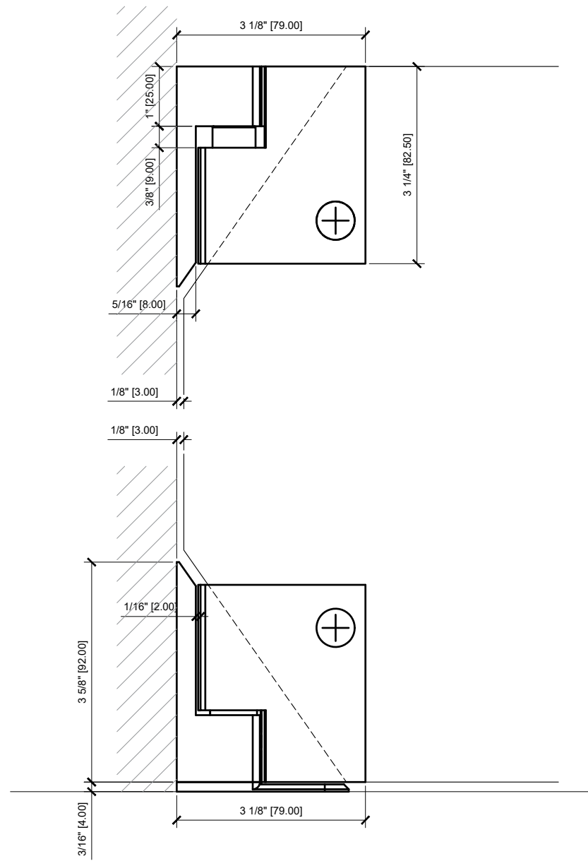
② SIDE VIEW DETAIL
