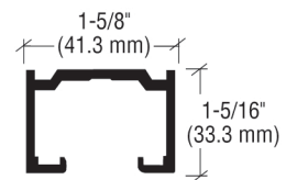
STANDARD D6 OVERHEAD TRACK SPECIFY D1043 ASSEMBLY (NO JAMBS)*
