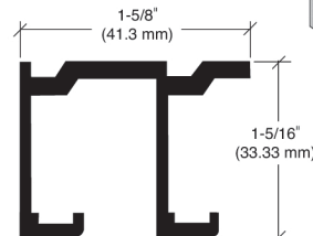
D4 OVERHEAD TRACK Open Back Header for Shallow Showcase Application. Specify D1042 Assembly (No Jambs)*
