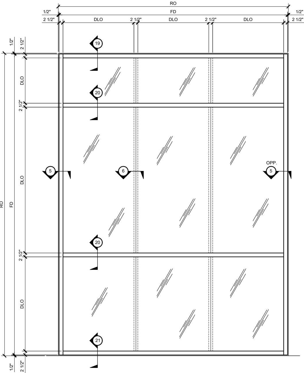
TYPICAL CURTAIN WALL ELEVATION
