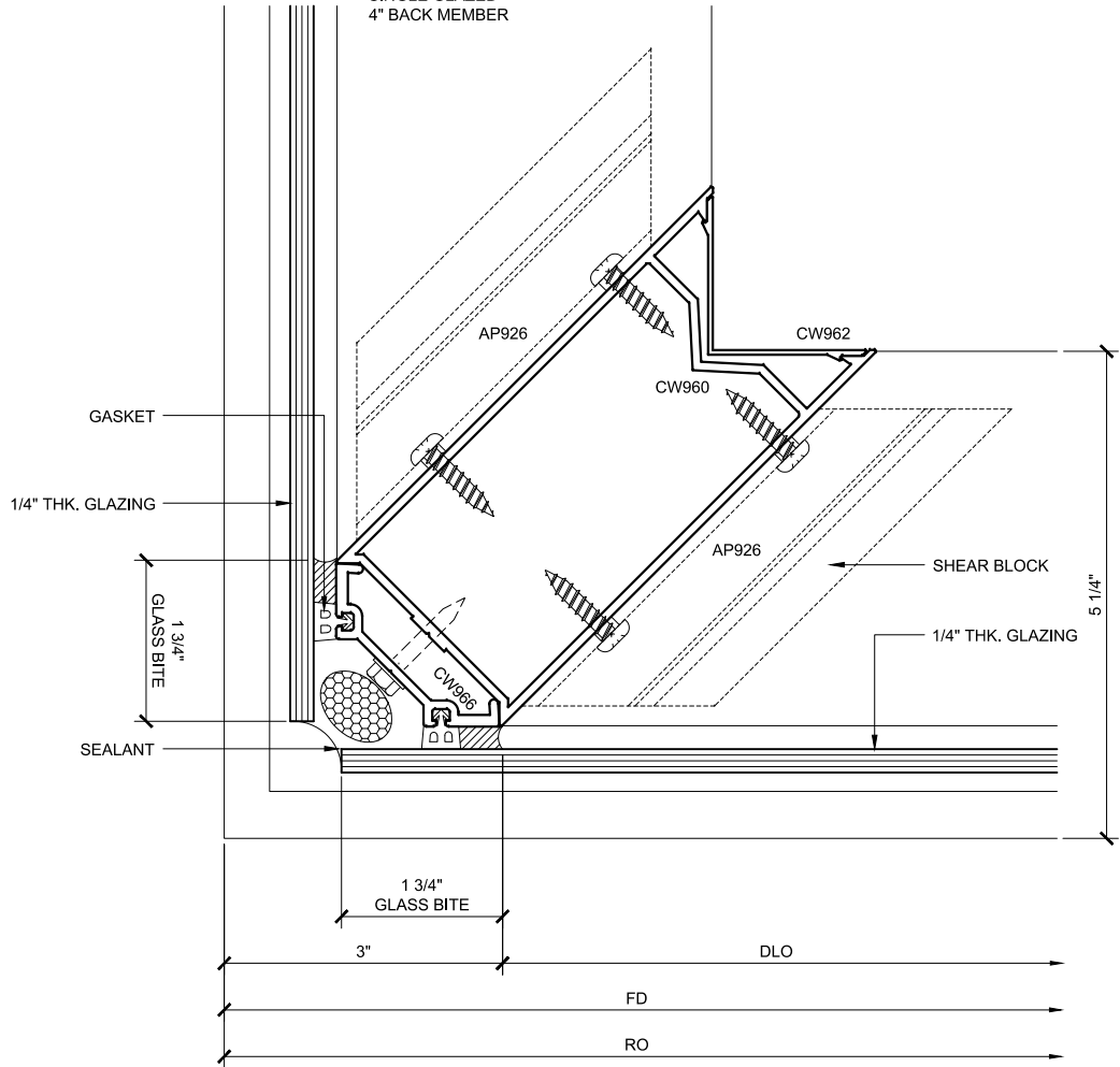
COR. VERT. PLAN ②②
