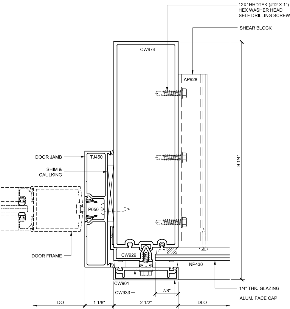
DOOR JAMB PLAN 28 SINGLE GLAZED 8" BACK MEMBER CH DOOR FRAMING
