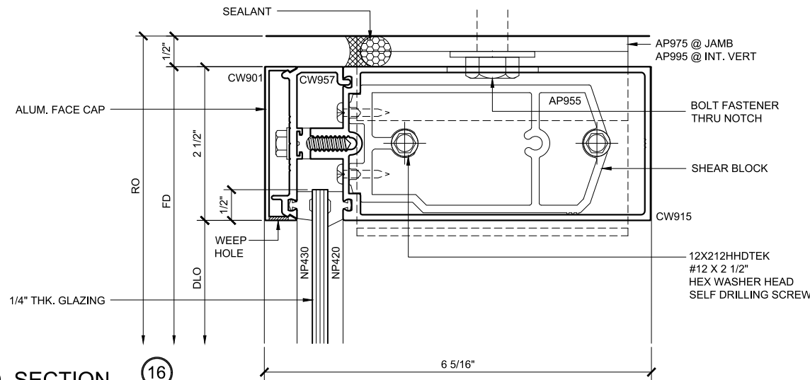
HEAD SECTION 16 SINGLE GLAZED 5" BACK MEMBER
