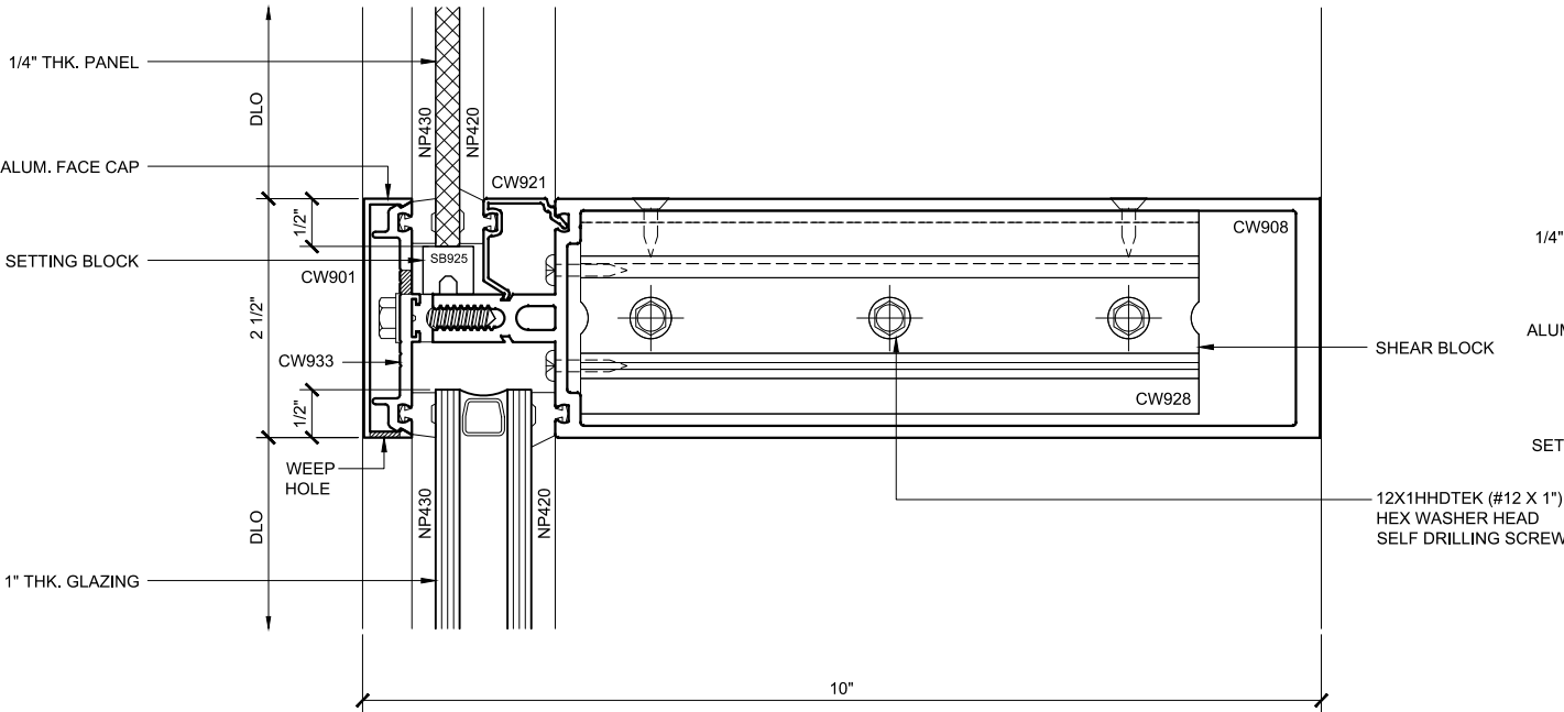
INT. HORIZ. SECTION 108 DOUBLE GLAZED 8\"/>
