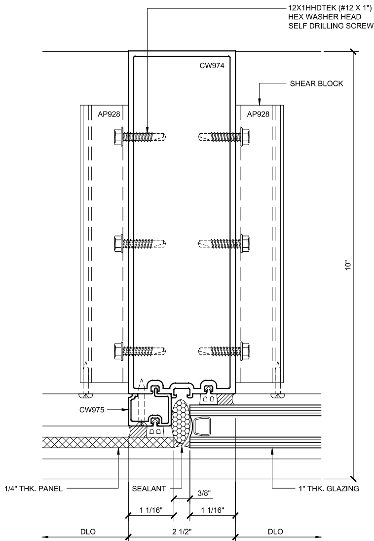
INT. VERT. PLAN 104 DOUBLE GLAZED 8" BACK MEMBER TRANSITION DETAIL
