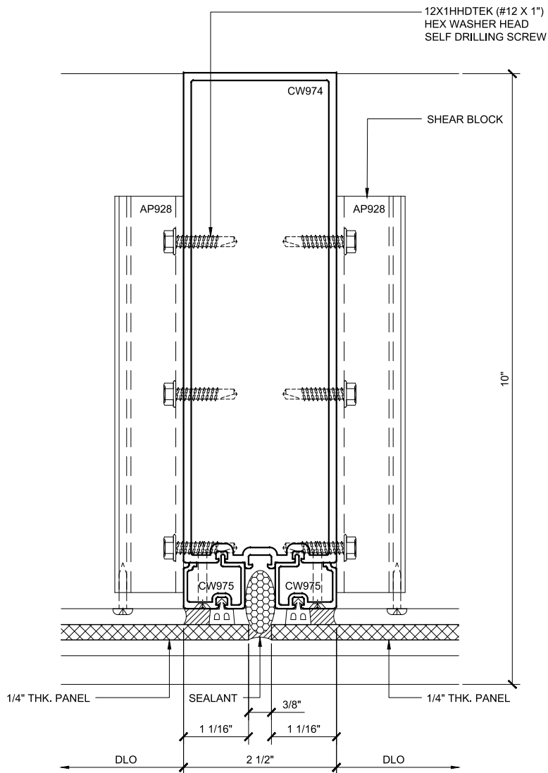
INT. VERT. PLAN 102 DOUBLE GLAZED 8" BACK MEMBER TRANSITION DETAIL
