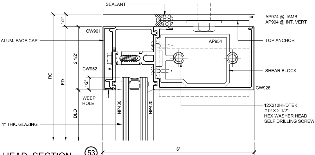
HEAD SECTION 53 DOUBLE GLAZED 4" BACK MEMBER
