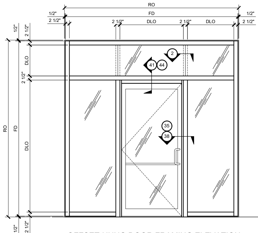
OFFSET-HUNG DOOR FRAMING ELEVATION
