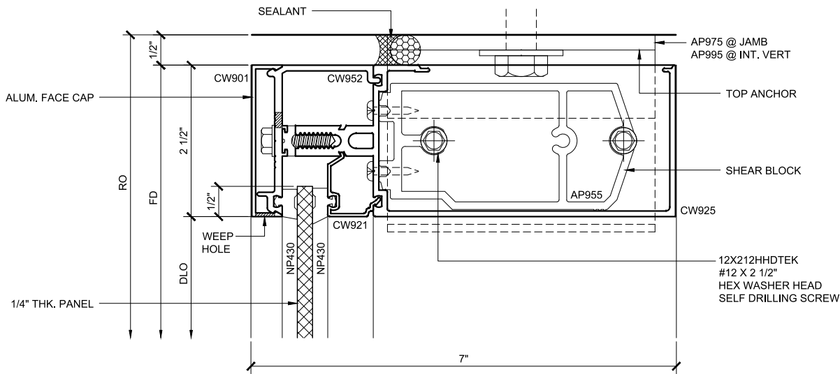
HEAD SECTION 105 DOUBLE GLAZED 5" BACK MEMBER TRANSITION DETAIL
