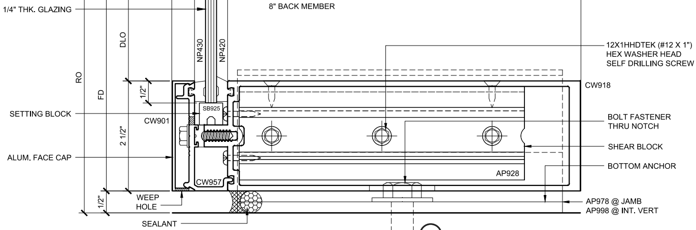
SILL SECTION 21
