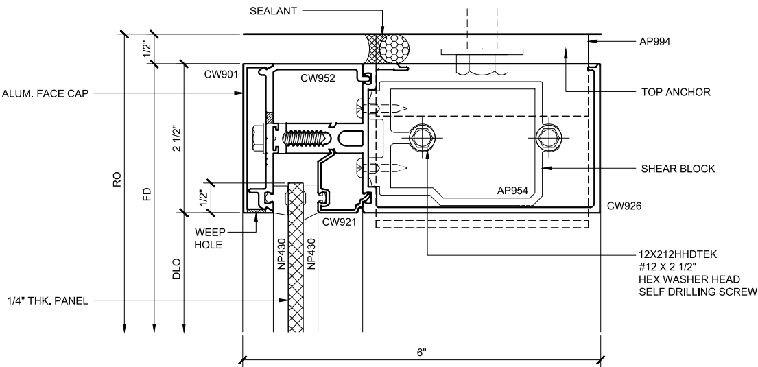
HEAD SECTION 76 DOUBLE GLAZED 4\"/>
