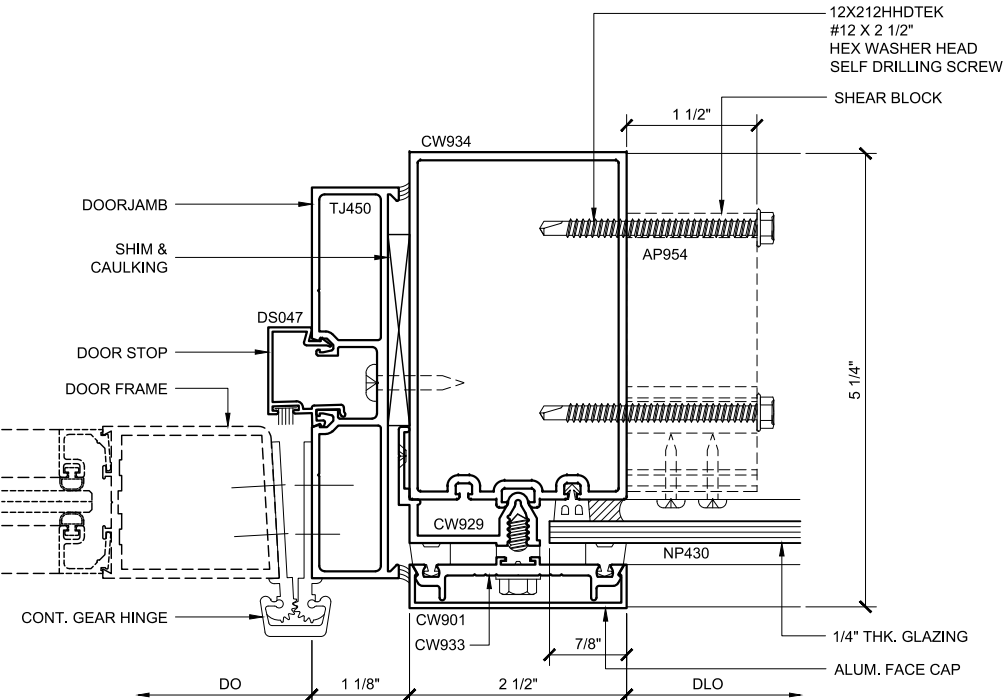
DOOR JAMB PLAN 38 SINGLE GLAZED 4" BACK MEMBER OH DOOR FRAMING
