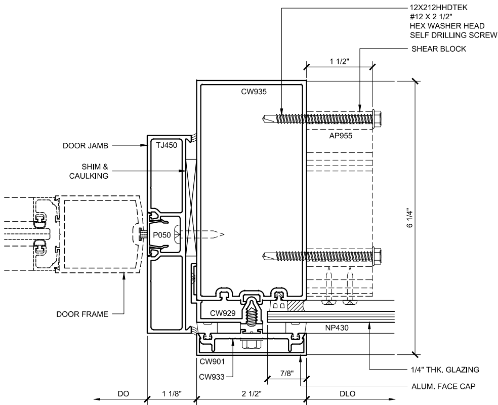
INT. VERT. PLAN 27 SINGLE GLAZED 5" BACK MEMBER CH DOOR FRAMING
