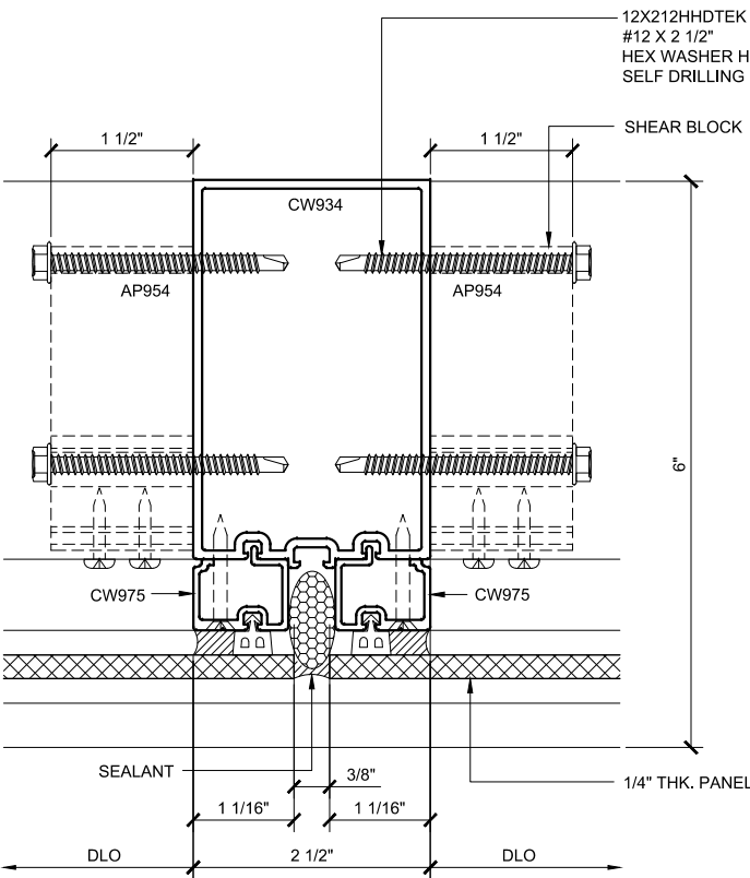
INT. VERT. PLAN 72 DOUBLE GLAZED 4\"/>
