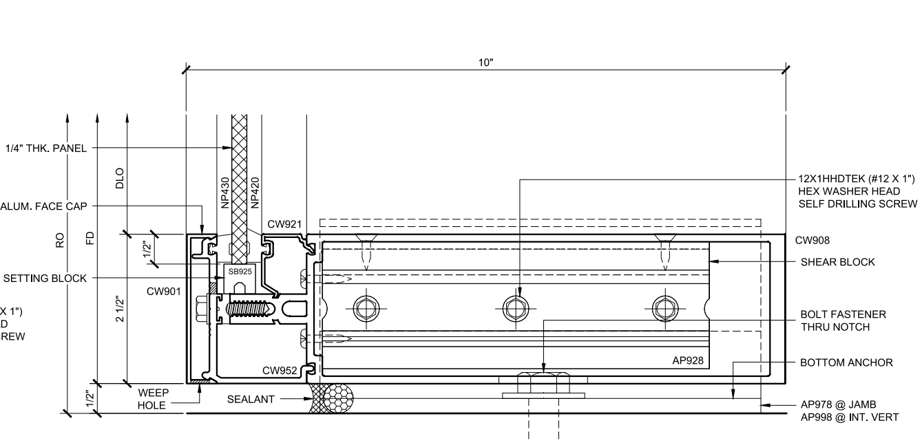
SILL SECTION 112 DOUBLE GLAZED 8\"/>
