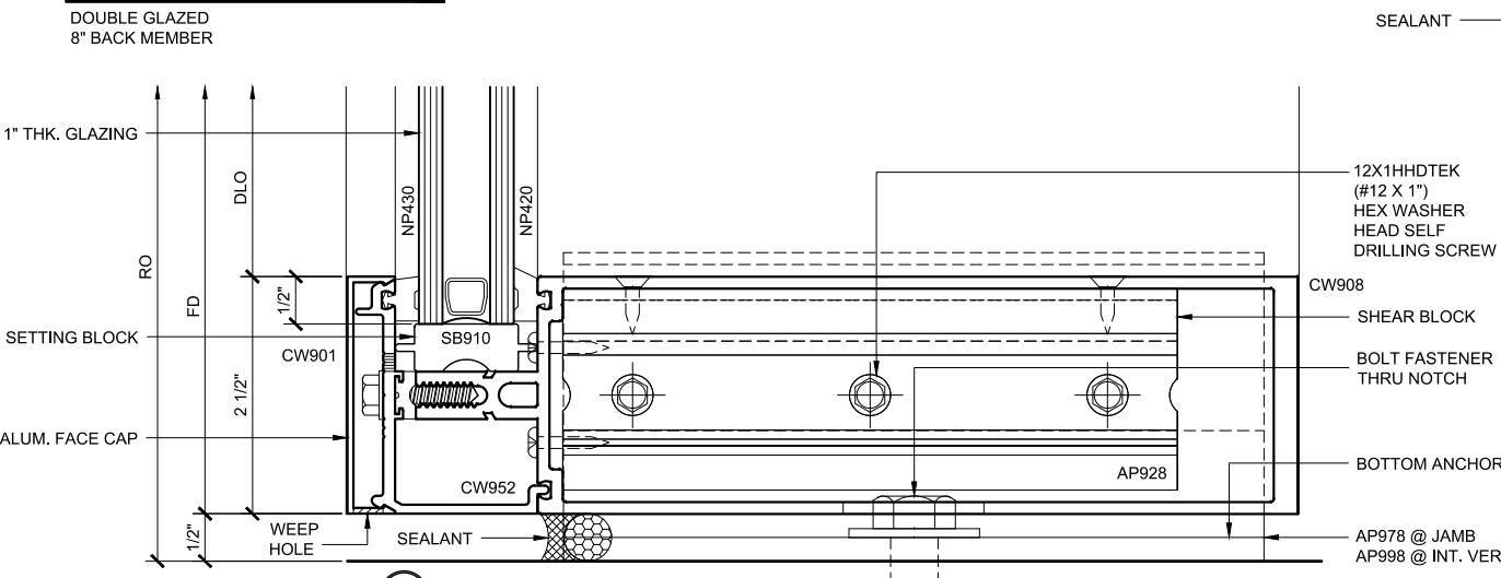
SILL SECTION 67
