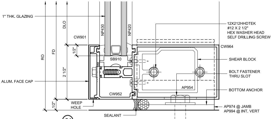
SILL SECTION 61 DOUBLE GLAZED 4" BACK MEMBER
