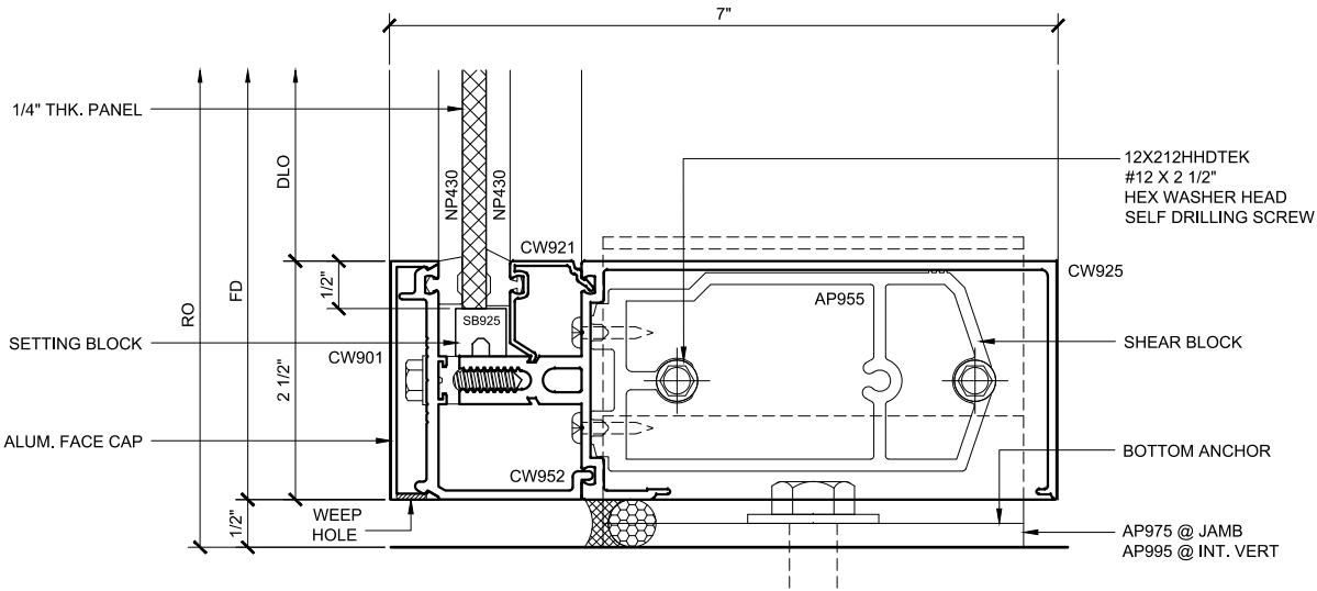
SILL SECTION 111 DOUBLE GLAZED 5" BACK MEMBER TRANSITION DETAILS
