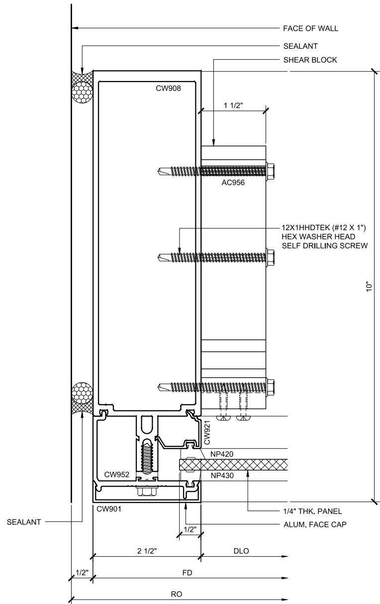
JAMB PLAN 123A DOUBLE GLAZED 8" BACK MEMBER TRANSITION DETAIL
