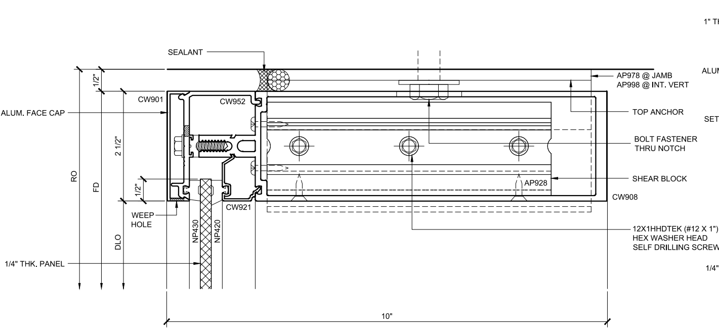
HEAD SECTION 106 DOUBLE GLAZED 8\"/>
