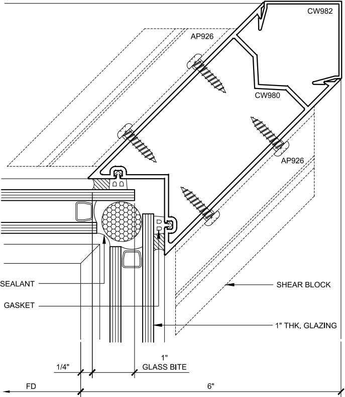
COR. VERT. PLAN 70
