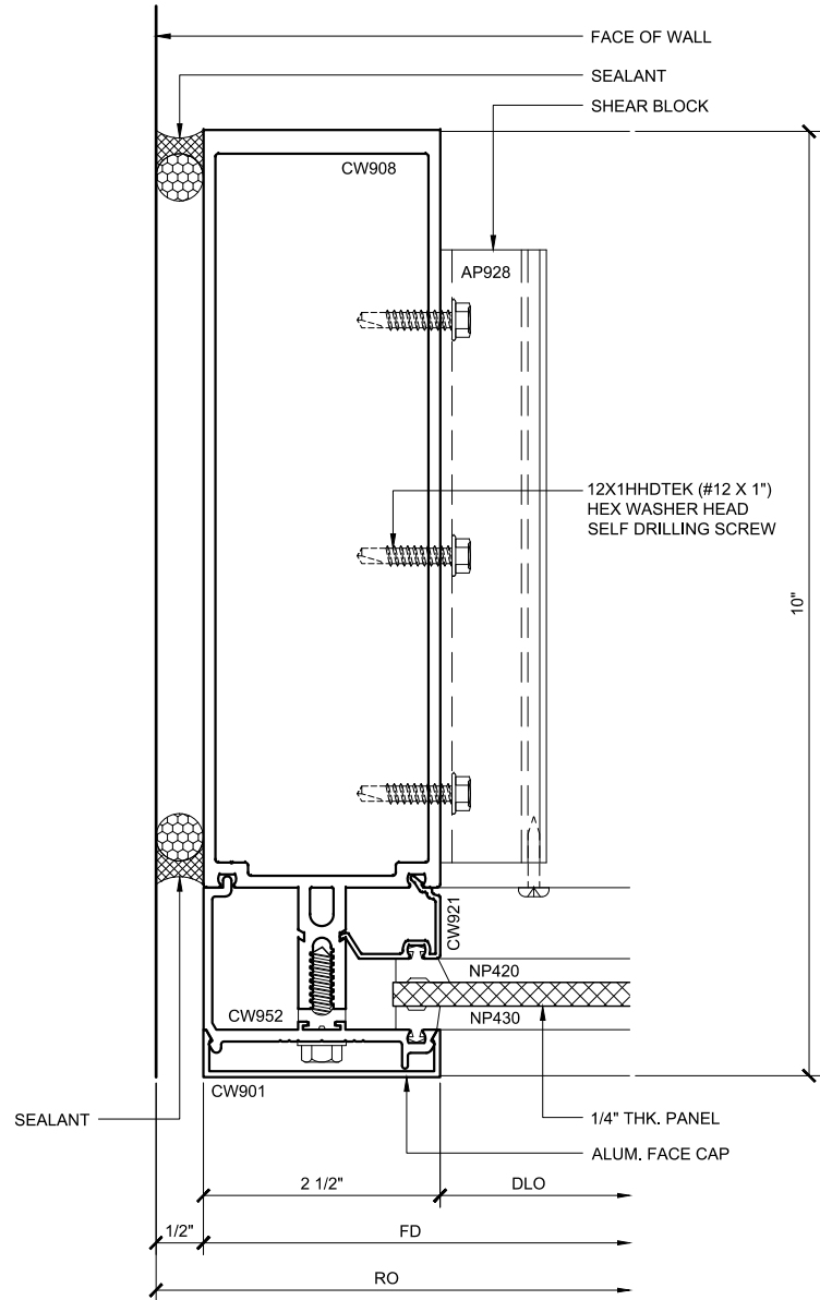
JAMB PLAN 51A DOUBLE GLAZED 8" BACK MEMBER TRANSITION DETAIL
