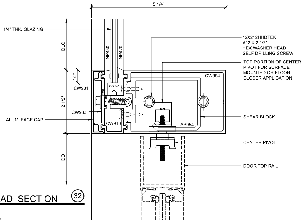
DOOR HEAD SECTION (29) SINGLE GLAZED 4" BACK MEMBER CH DOOR FRAMING
