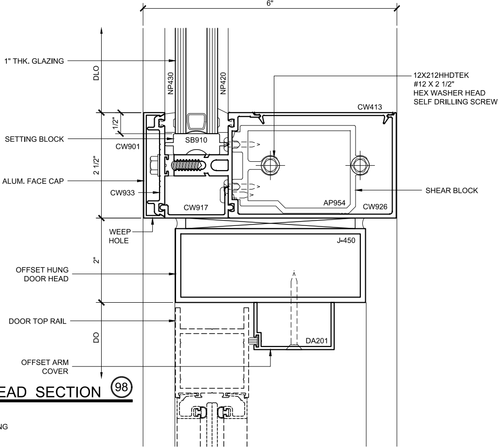
DOOR HEAD SECTION 95 DOUBLE GLAZED 4" BACK MEMBER OH DOOR FRAMING
