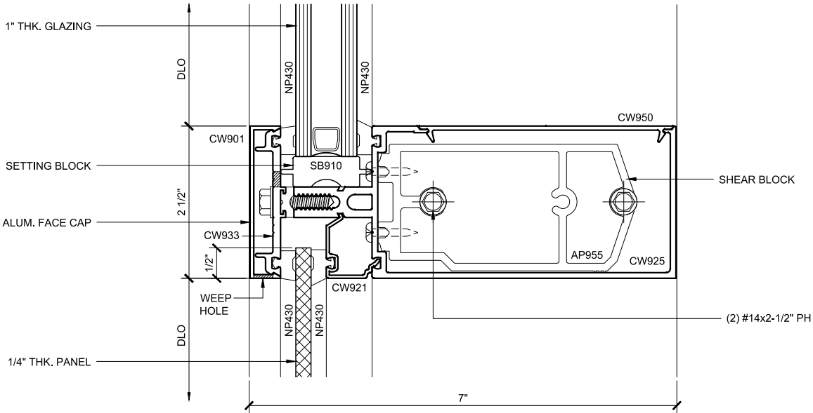
INT. HORIZ. SECTION 109 DOUBLE GLAZED 5" BACK MEMBER TRANSITION DETAILS
