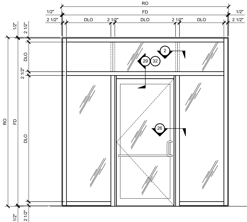
CENTER-HUNG DOOR FRAMING ELEVATION
