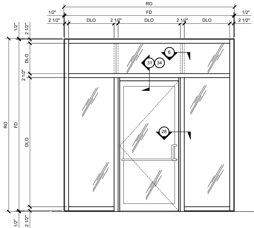
CENTER-HUNG DOOR FRAMING ELEVATION
