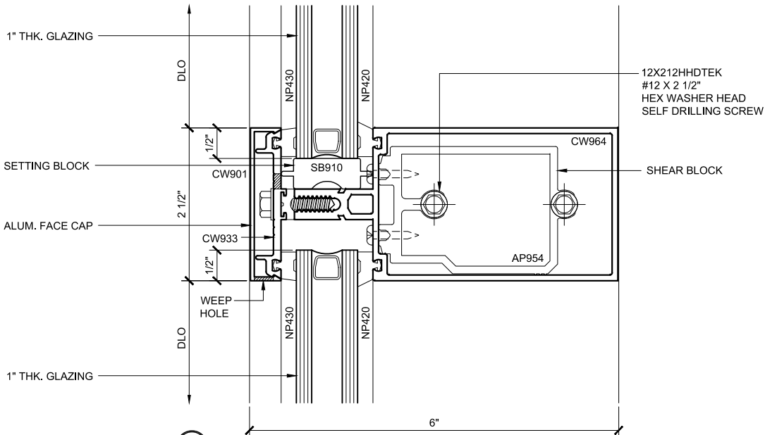
INT. HOR. SECTION 60 DOUBLE GLAZED 4" BACK MEMBER
