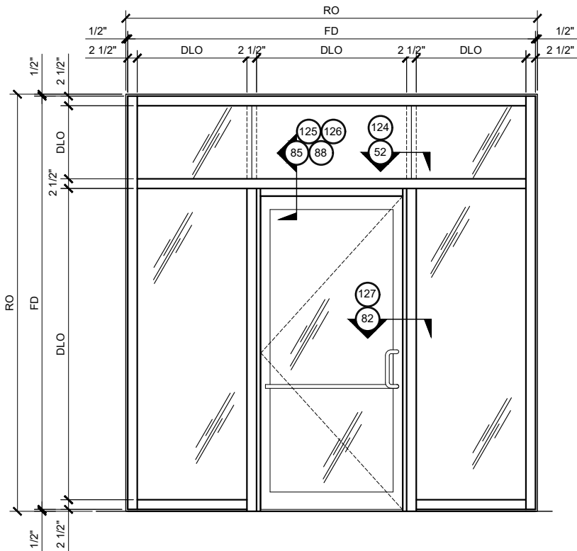
CENTER-HUNG DOOR FRAMING ELEVATION
