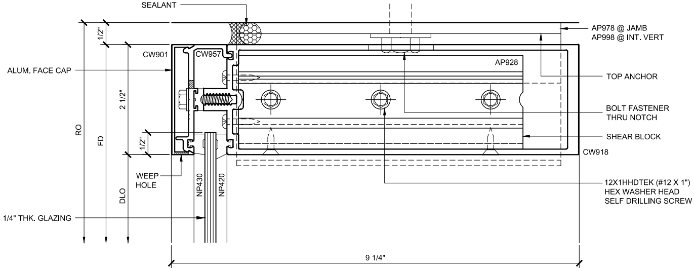
HEAD SECTION 19
