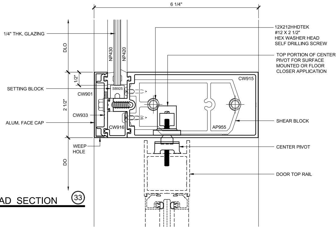
DOOR HEAD SECTION 30 SINGLE GLAZED 5" BACK MEMBER CH DOOR FRAMING
