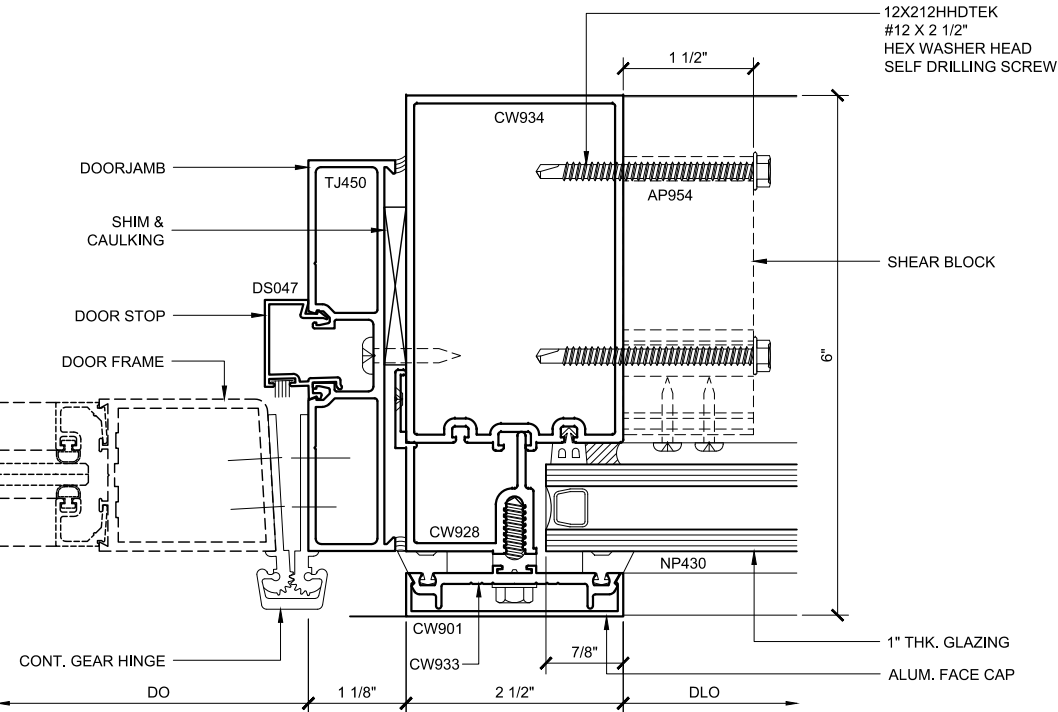
DOOR JAMB PLAN 92 DOUBLE GLAZED 4" BACK MEMBER OH DOOR FRAMING
