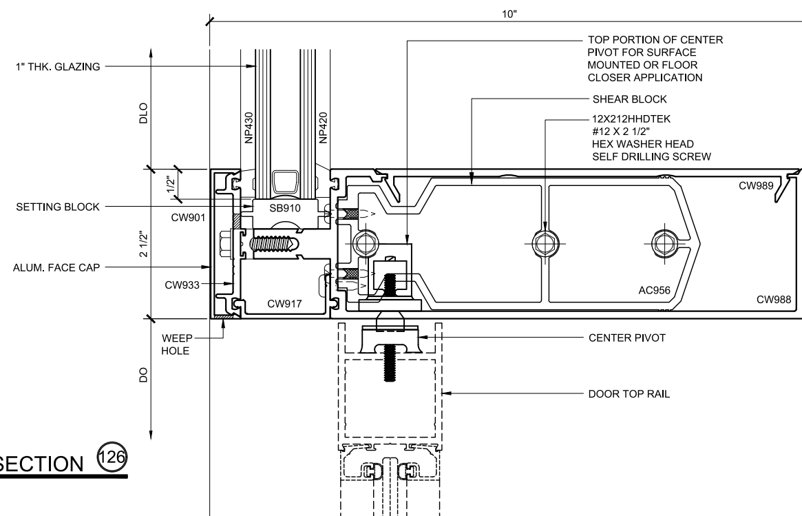
DOUBLE GLAZED 8" BACK MEMBER CH DOOR FRAMING
