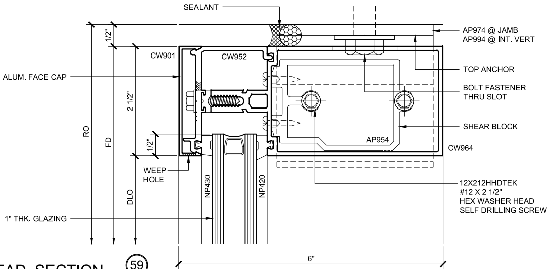
HEAD SECTION 59 DOUBLE GLAZED 4" BACK MEMBER
