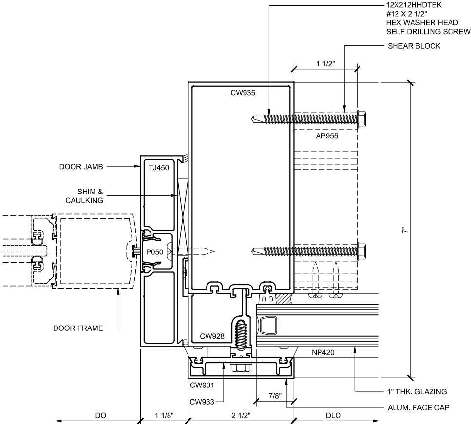
DOOR JAMB PLAN (81) DOUBLE GLAZED 5" BACK MEMBER CH DOOR FRAMING
