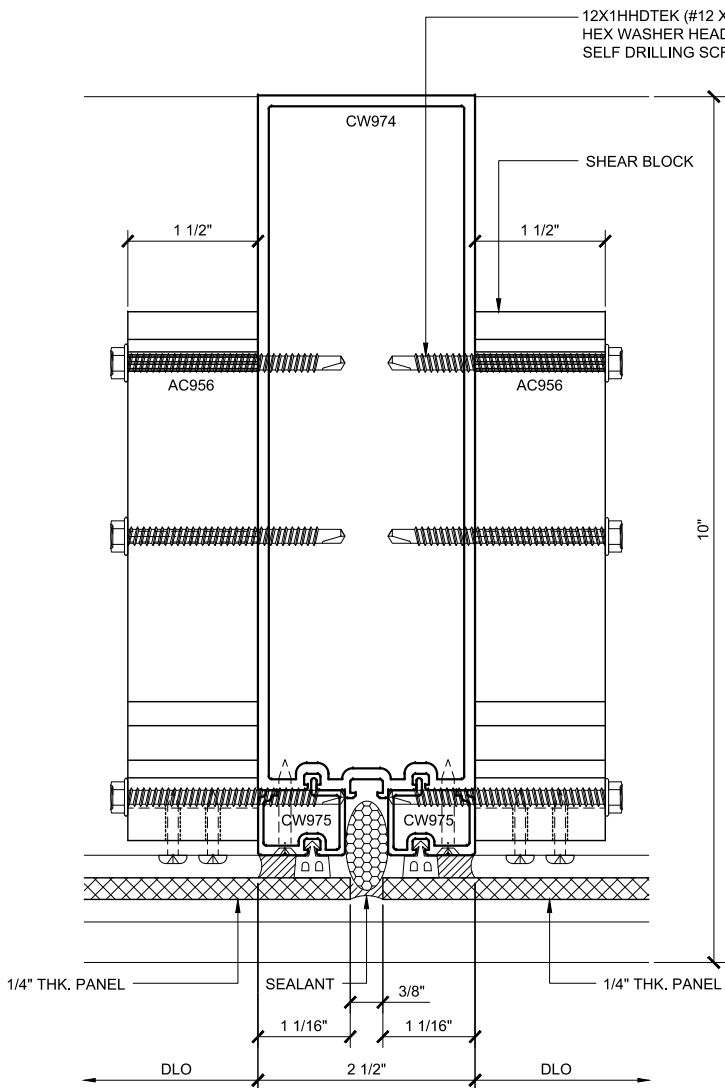
INT. VERT. PLAN 136 DOUBLE GLAZED 8" BACK MEMBER TRANSITION DETAIL
