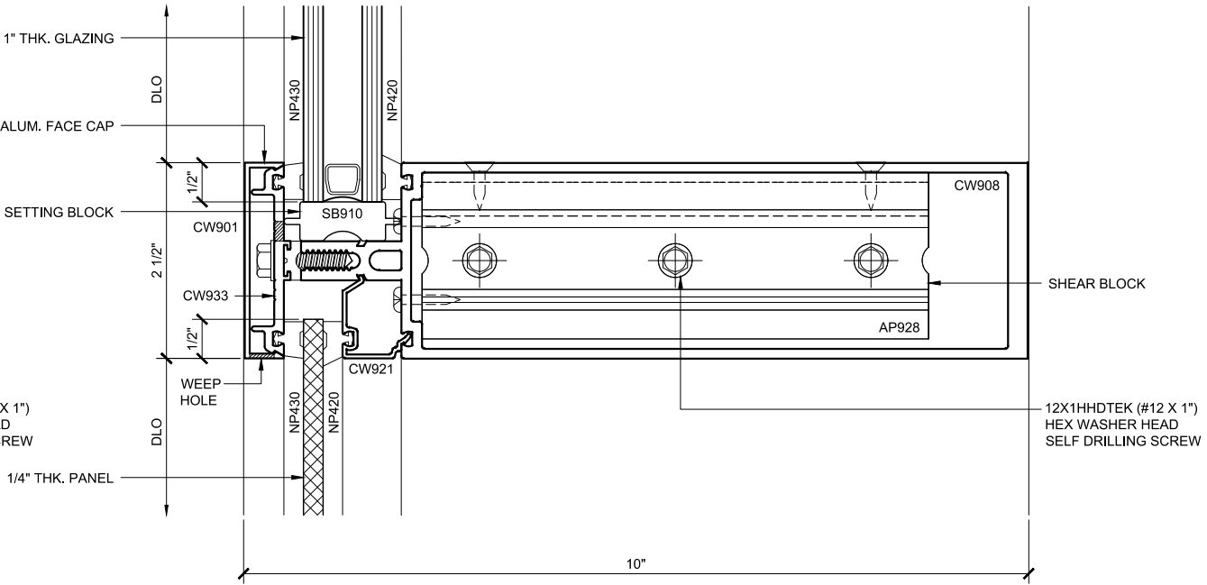
INT. HORIZ. SECTION 110 DOUBLE GLAZED 8\"/>
