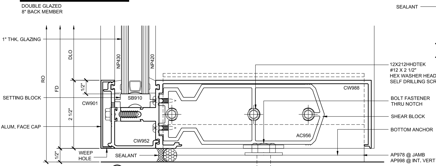
SILL SECTION 122
