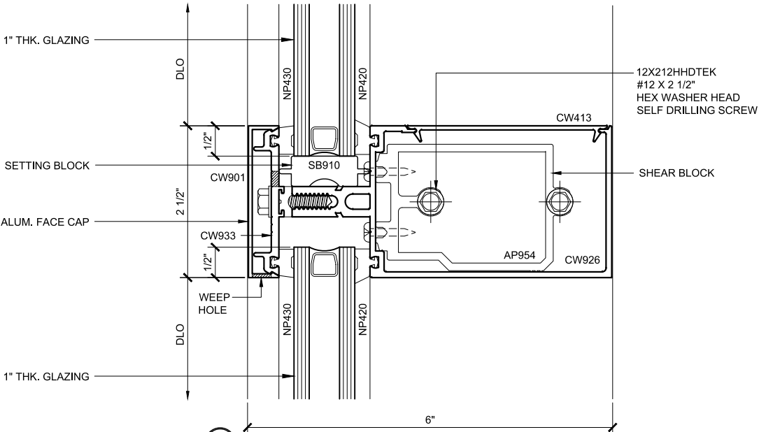
INT. HOR. SECTION 54 DOUBLE GLAZED 4" BACK MEMBER
