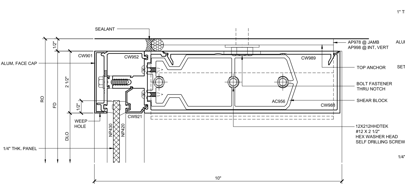
HEAD SECTION 132 DOUBLE GLAZED 8" BACK MEMBER TRANSITION DETAIL
