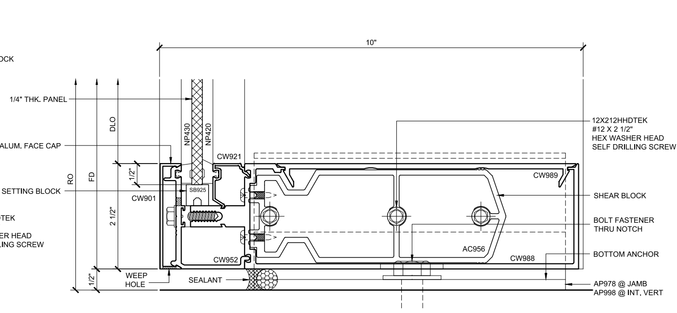
SILL SECTION 135 DOUBLE GLAZED 8" BACK MEMBER TRANSITION DETAILS
