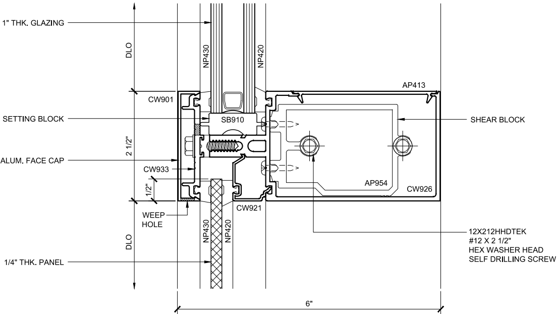
INT. HORIZ. SECTION 78 DOUBLE GLAZED 4\"/>
