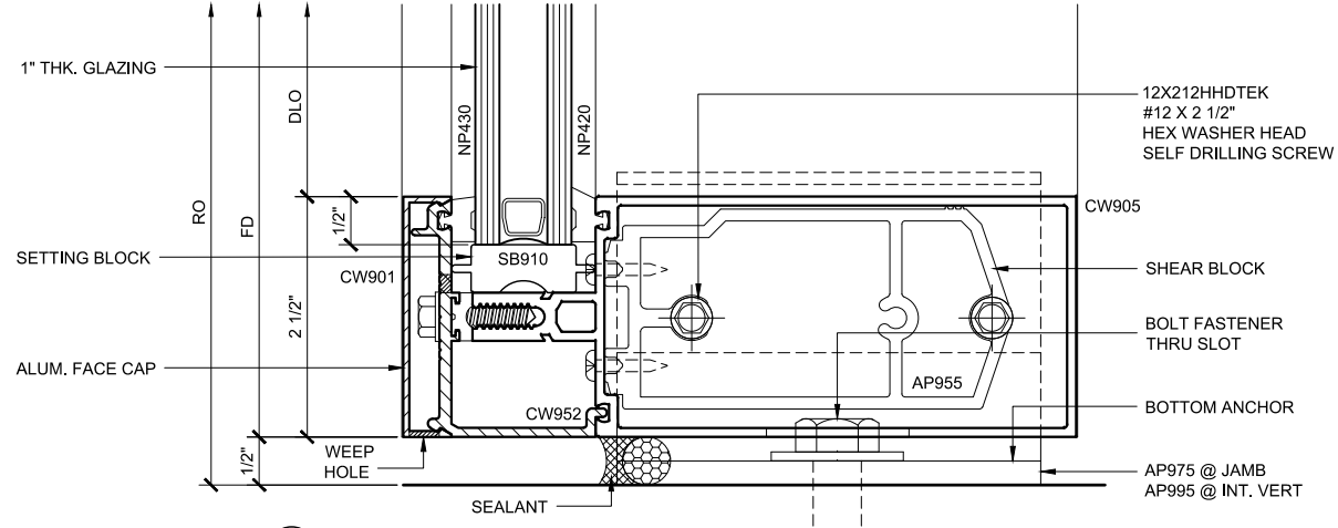
SILL SECTION
