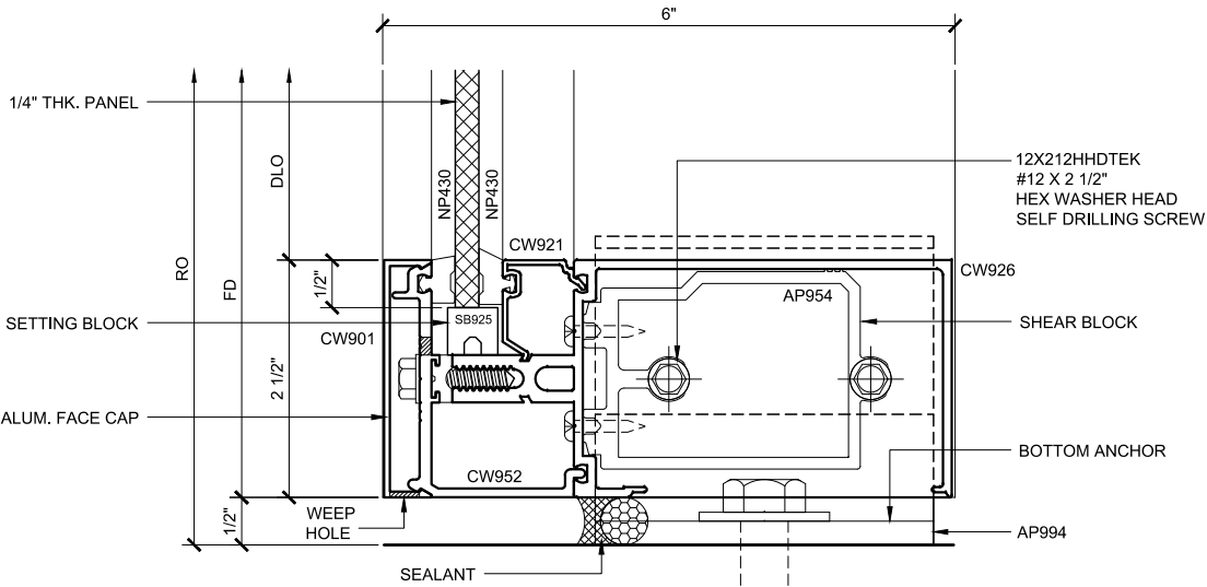
SILL SECTION 79 DOUBLE GLAZED 4\"/>
