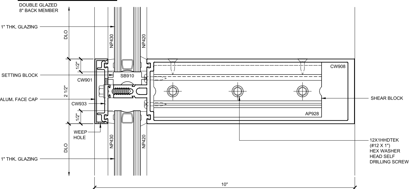
INT. HOR. SECTION 66
