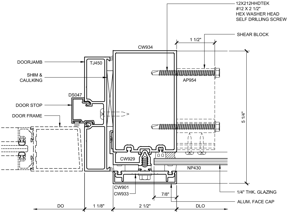
DOOR JAMB PLAN 35 SINGLE GLAZED 4" BACK MEMBER OH DOOR FRAMING
