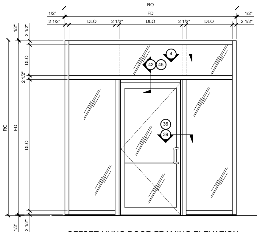
OFFSET-HUNG DOOR FRAMING ELEVATION
