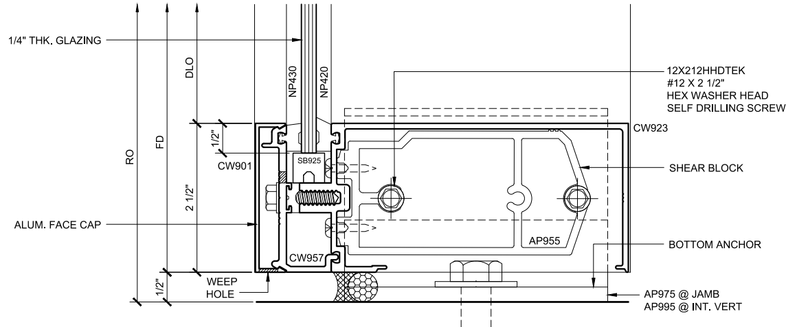
SILL SECTION 12 SINGLE GLAZED 5" BACK MEMBER
