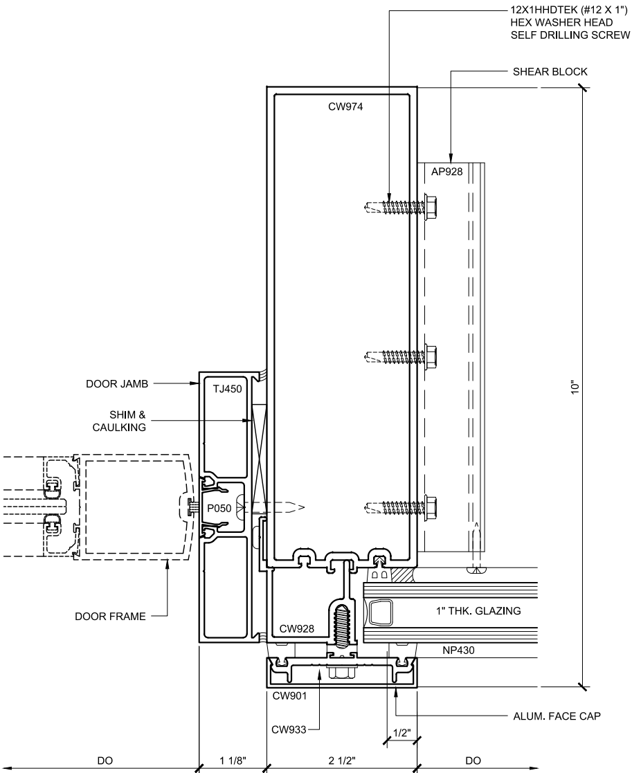
DOOR JAMB PLAN 82 DOUBLE GLAZED 8" BACK MEMBER CH DOOR FRAMING
