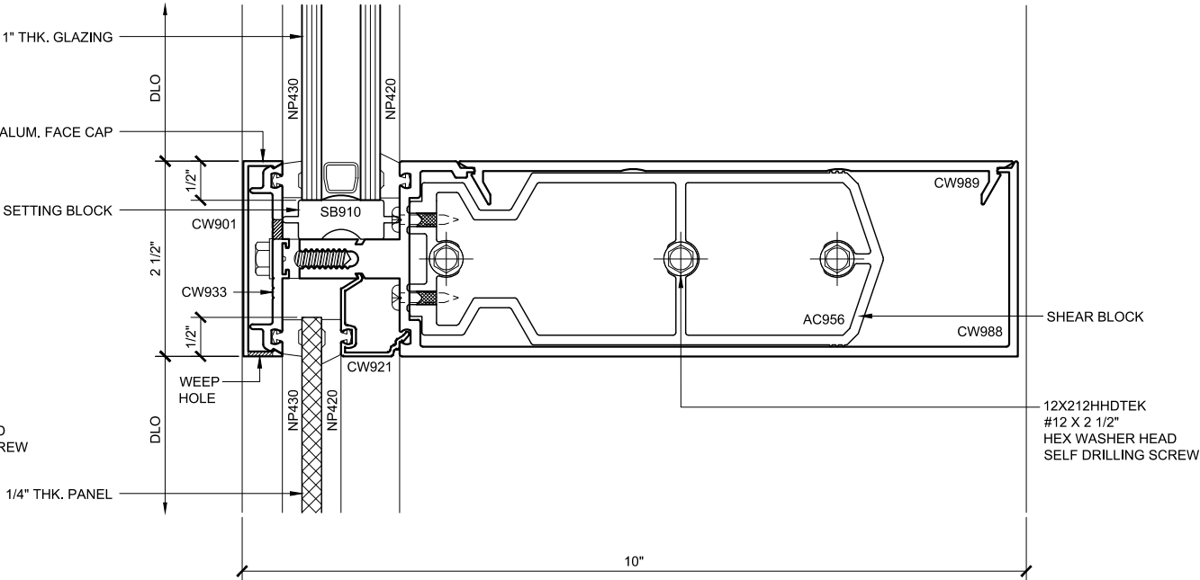
INT. HORIZ. SECTION 134 DOUBLE GLAZED 8" BACK MEMBER TRANSITION DETAILS
