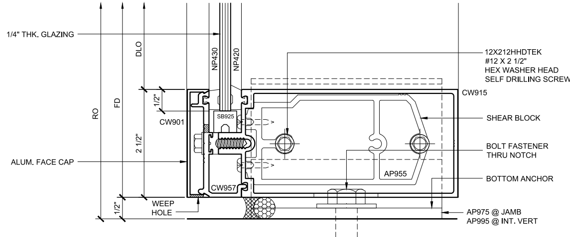
SILL SECTION 18 SINGLE GLAZED 5" BACK MEMBER
