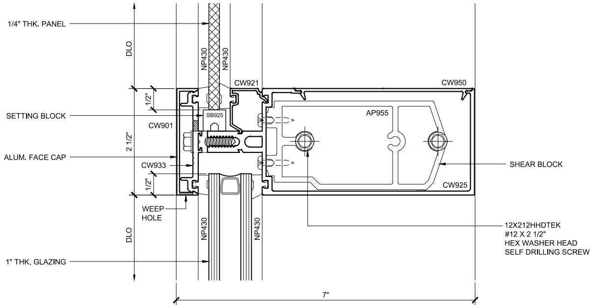
INT. HORIZ. SECTION 107 DOUBLE GLAZED 5" BACK MEMBER TRANSITION DETAILS
