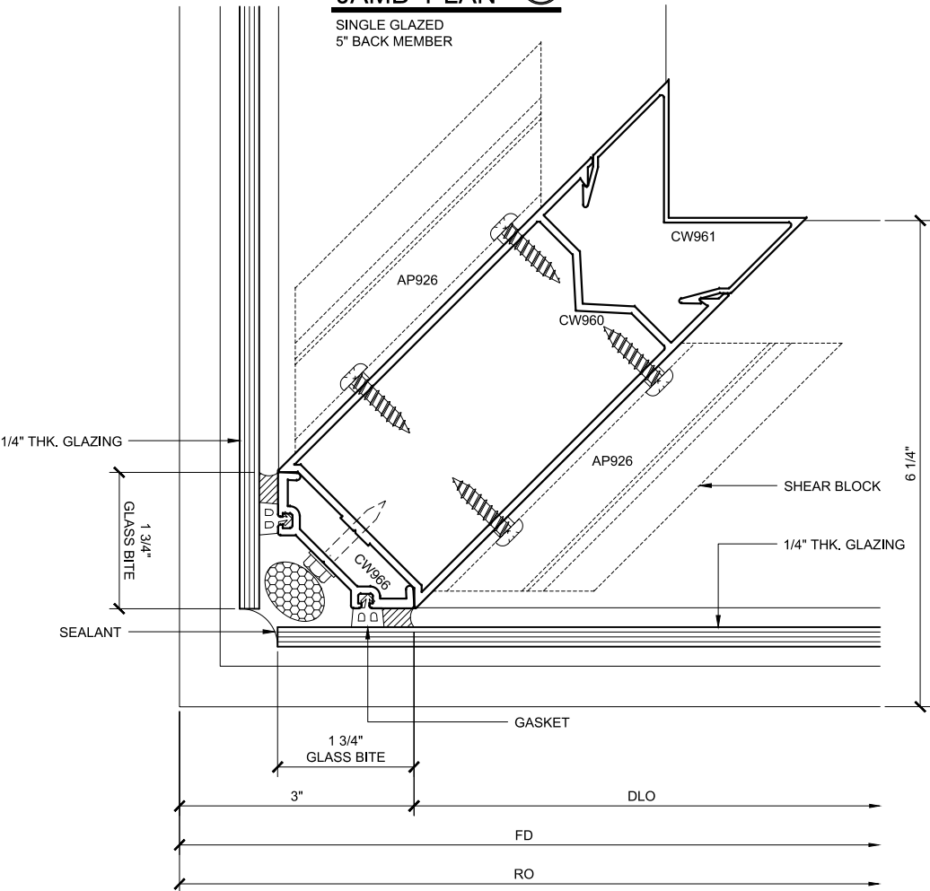
COR. VERT. PLAN 23
