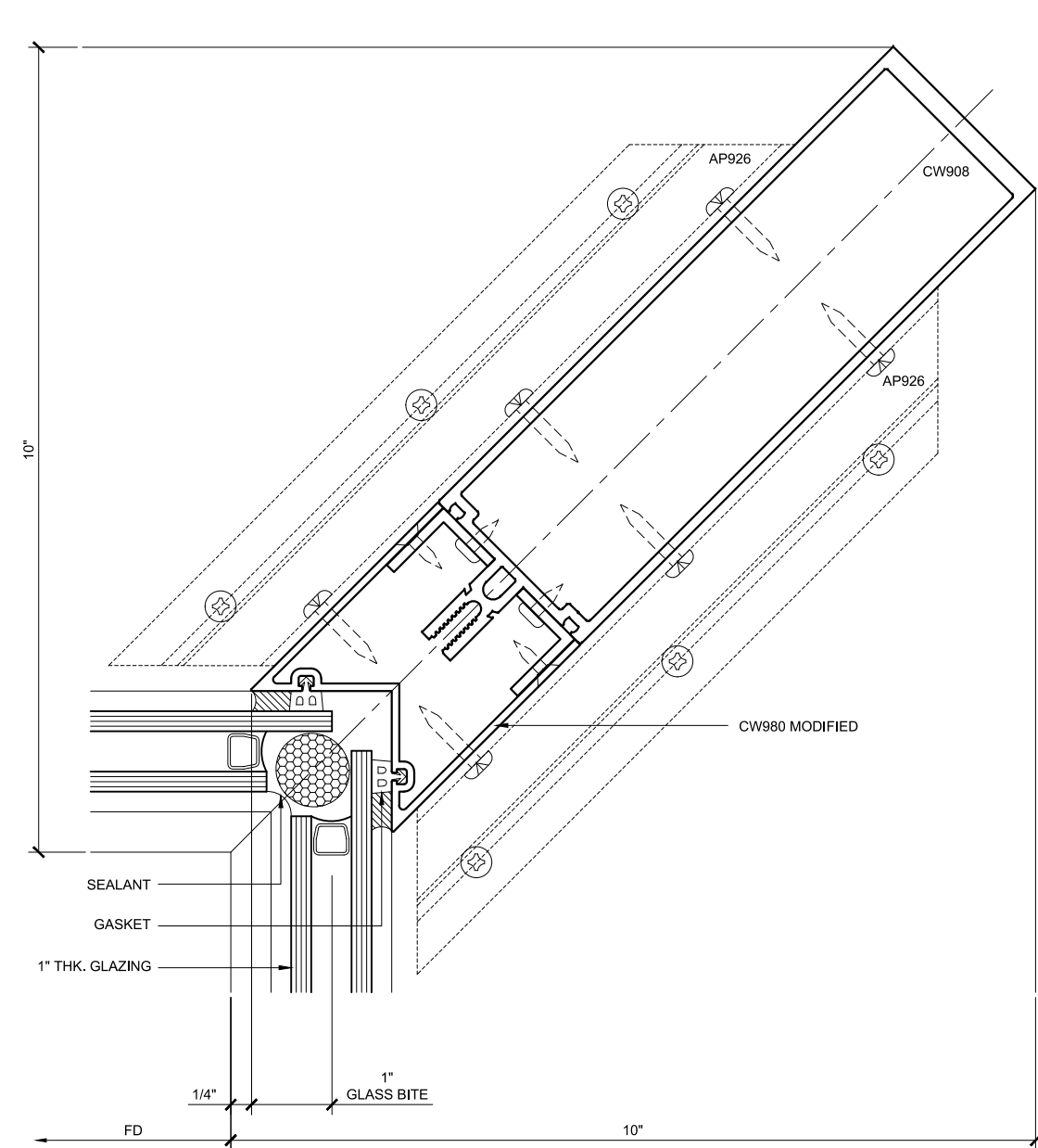
INSIDE COR. VERT. SECTION 117 DOUBLE GLAZED 8" BACK MEMBER TRANSITION DETAIL
