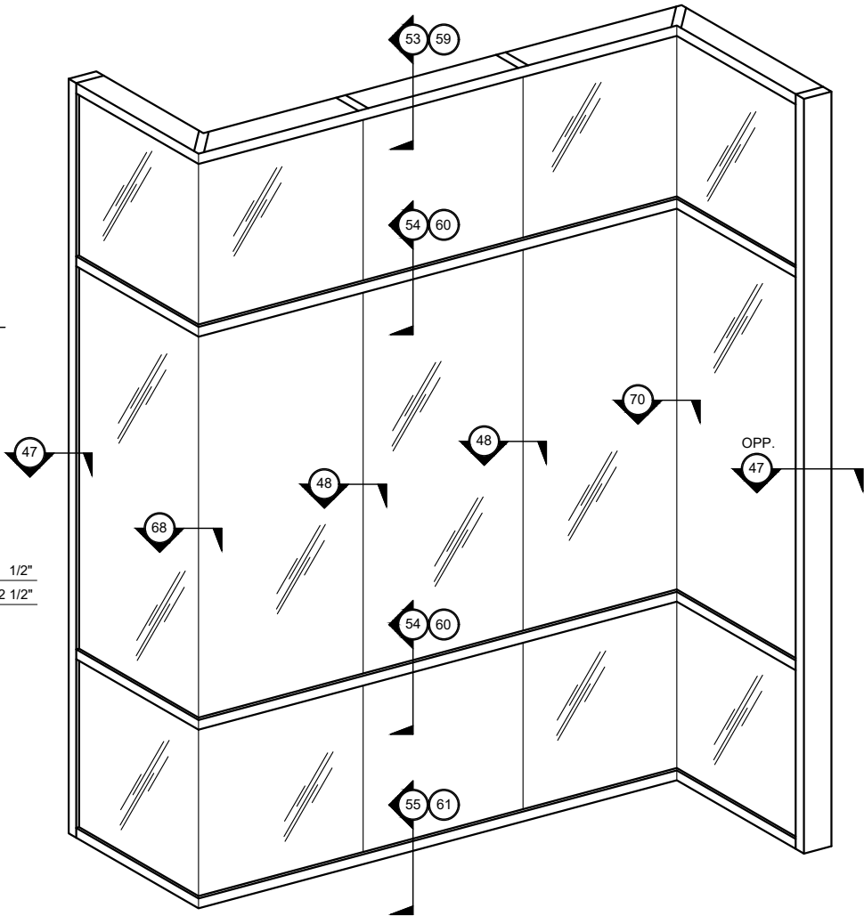
CENTER-HUNG DOOR FRAMING ELEVATION DOUBLE GLAZED 4" BACK MEMBER
