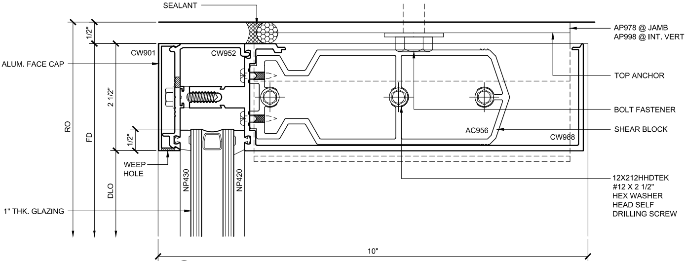
HEAD SECTION 120
