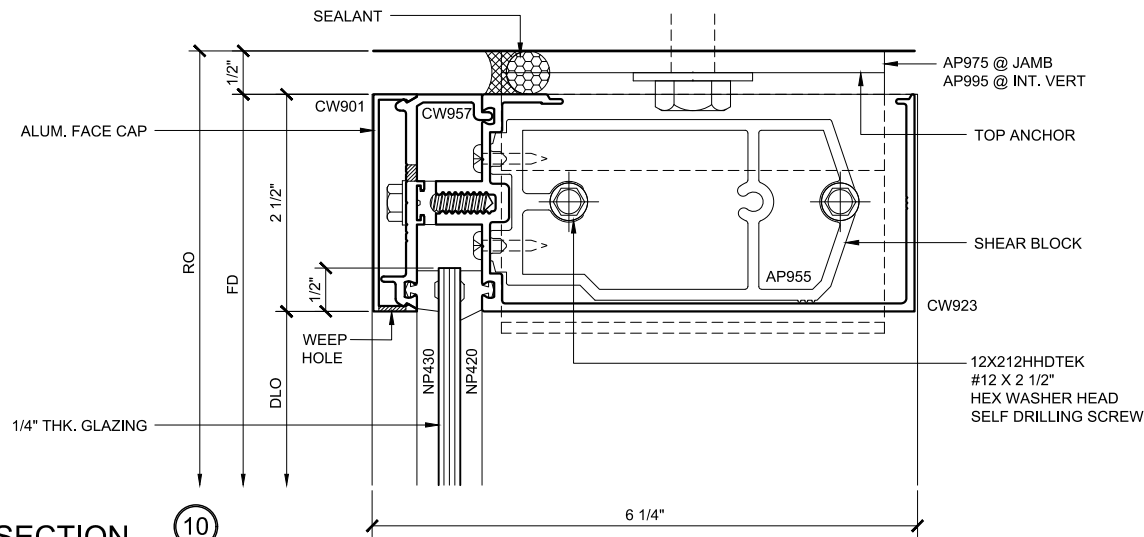
HEAD SECTION 10 SINGLE GLAZED 5" BACK MEMBER
