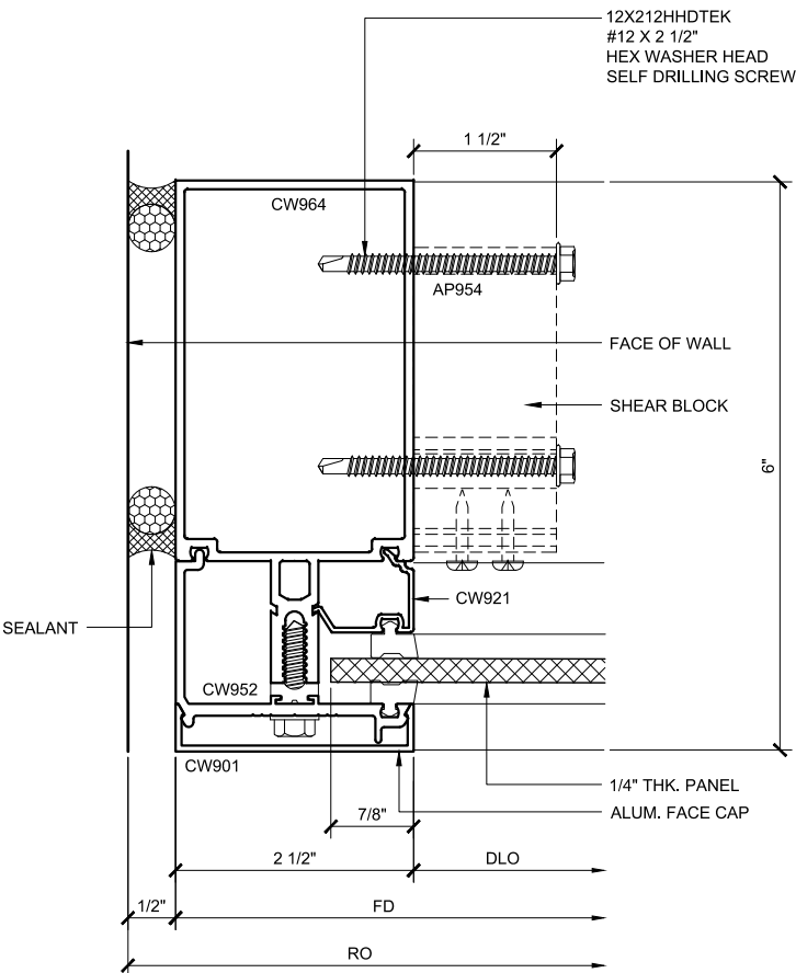
JAMB PLAN 47A DOUBLE GLAZED 4\"/>
