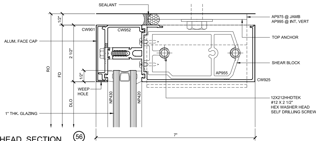
HEAD SECTION
