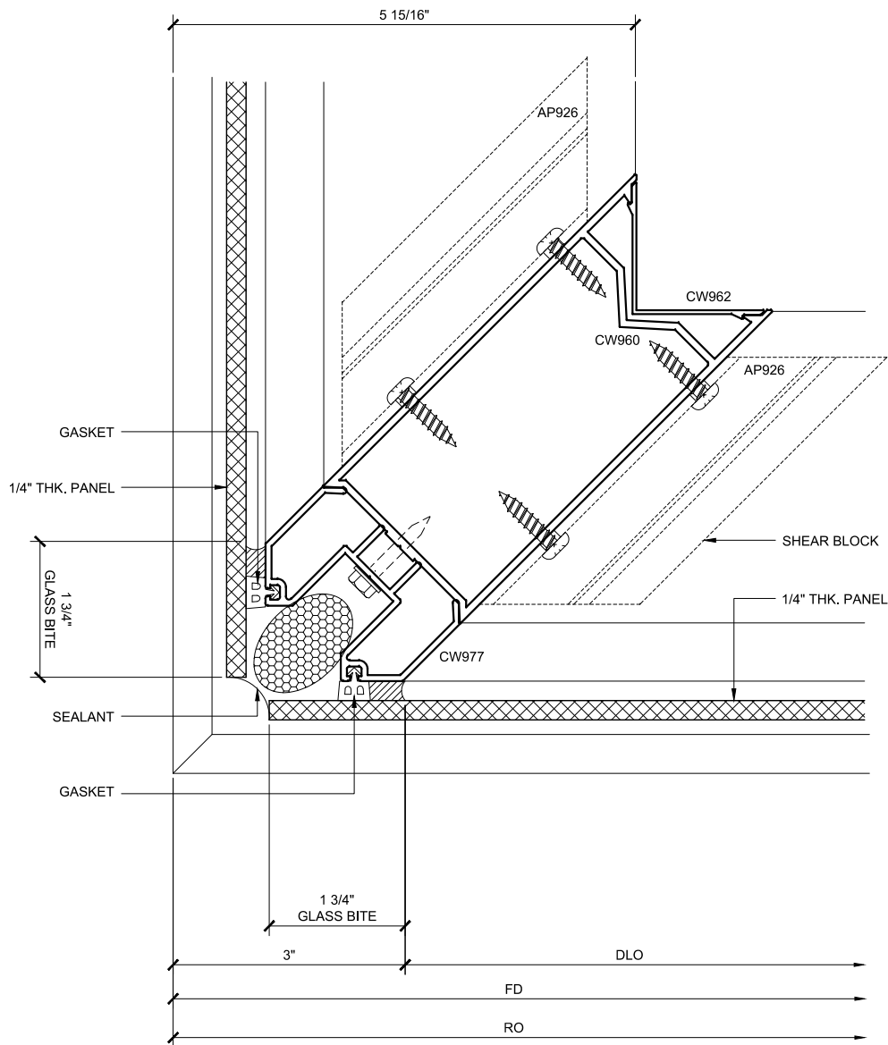
COR. VERT. SECTION 74 DOUBLE GLAZED 4\"/>
