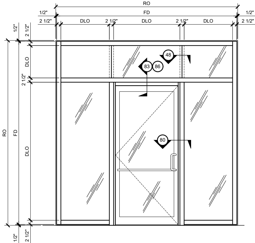
CENTER-HUNG DOOR FRAMING ELEVATION DOUBLE GLAZED 4" BACK MEMBER
