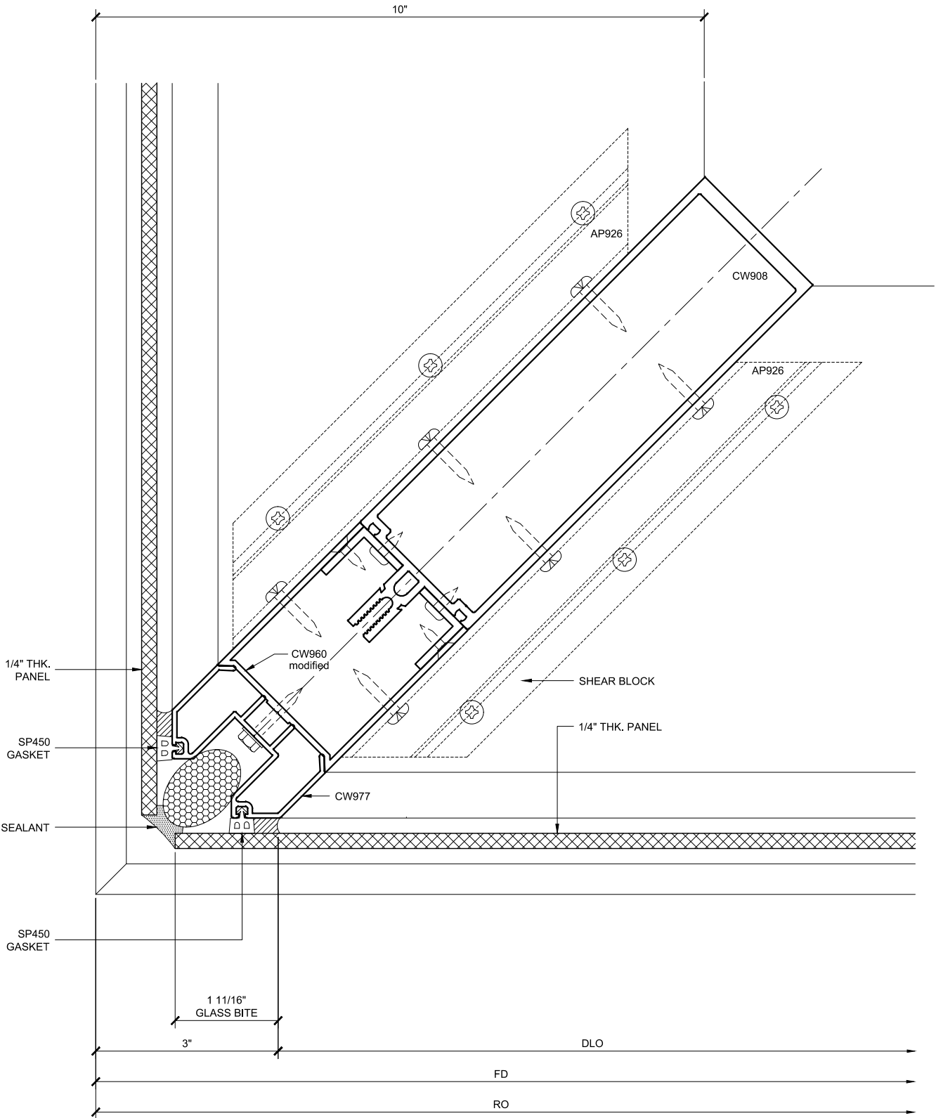
OUTSIDE COR. VERT. SECTION 114 DOUBLE GLAZED 8" BACK MEMBER TRANSITION DETAIL
