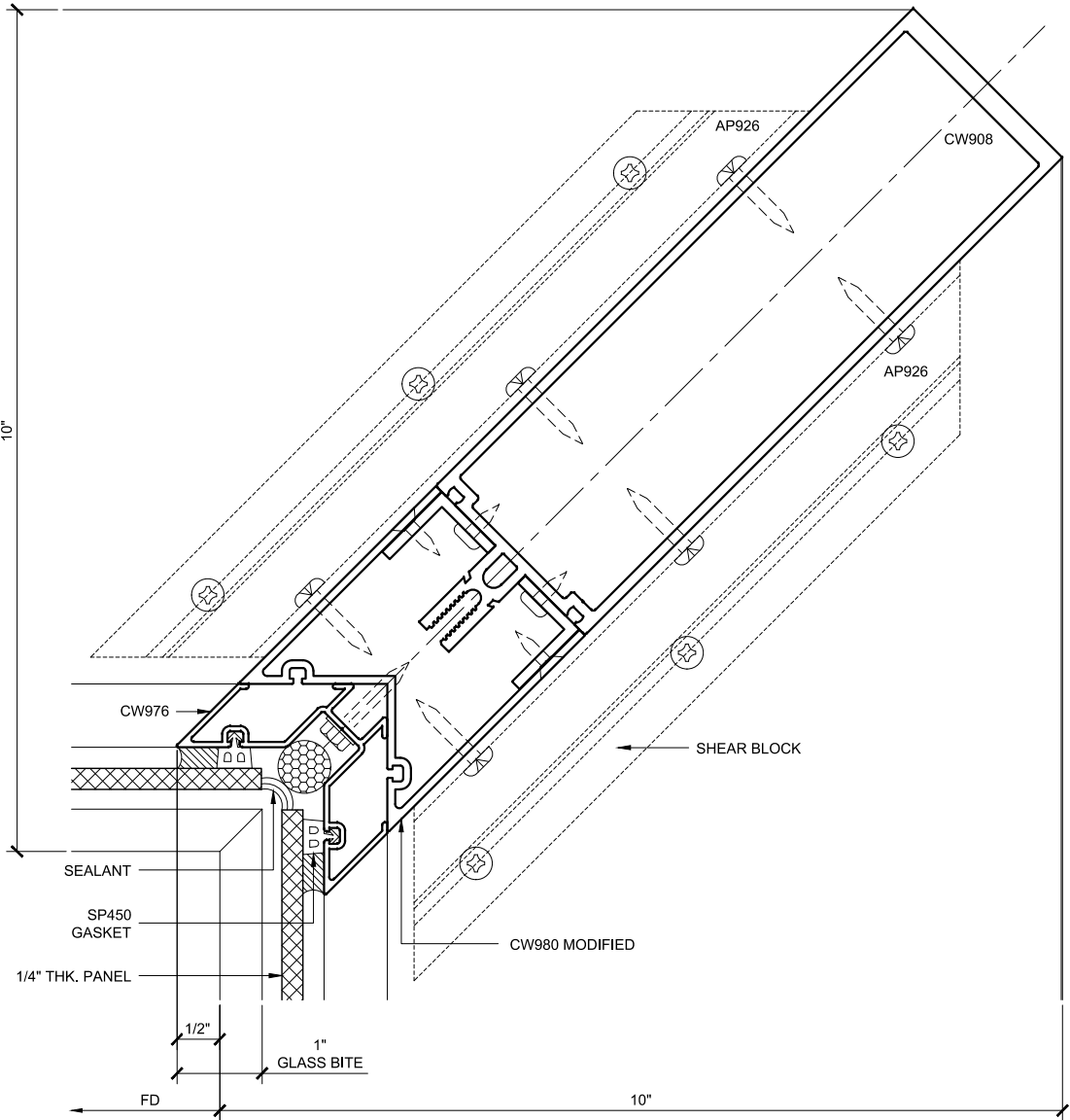
INSIDE COR. VERT. SECTION 116 DOUBLE GLAZED 8" BACK MEMBER TRANSITION DETAIL
