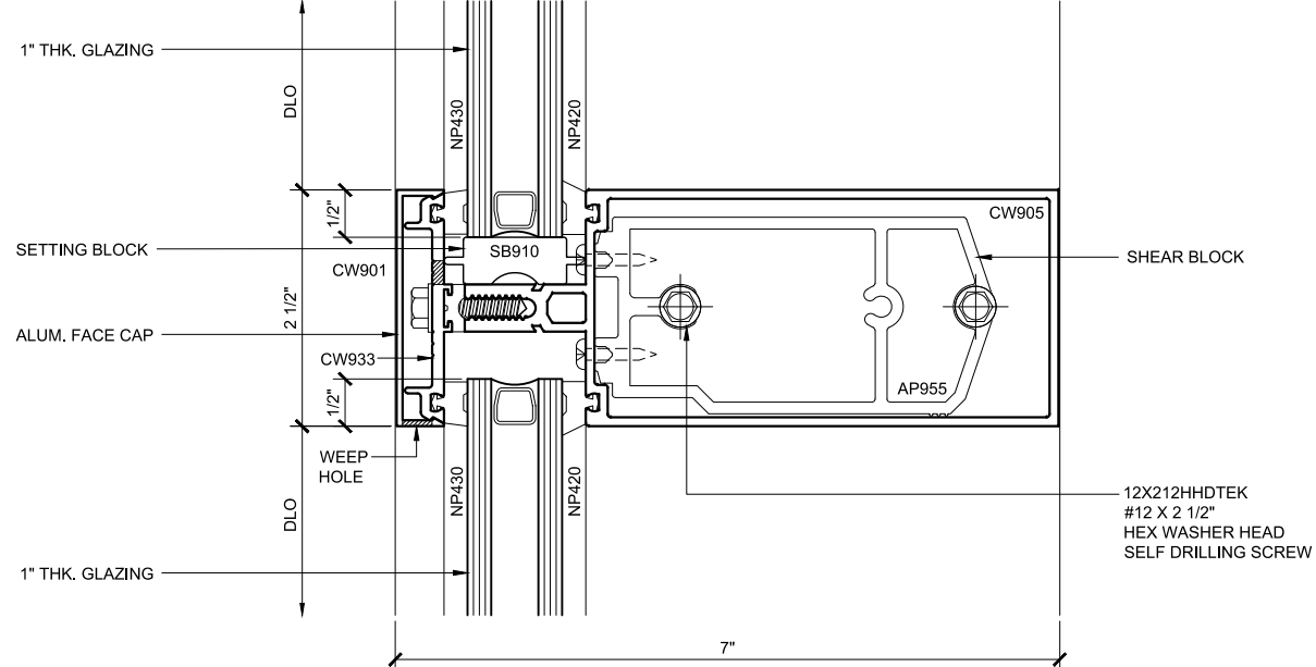
INT. HOR. SECTION
