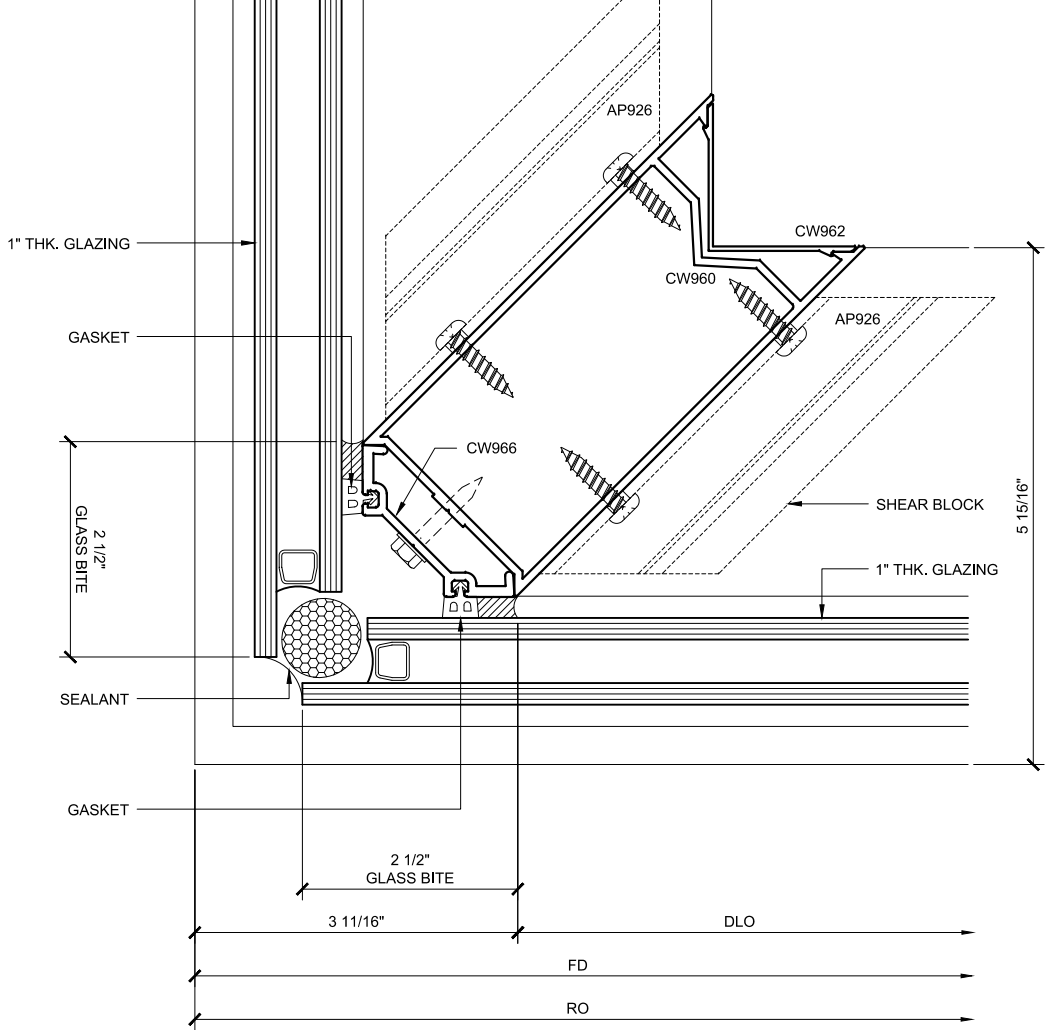
COR. VERT. PLAN 68
