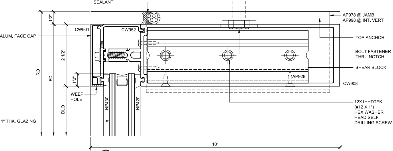
HEAD SECTION 65
