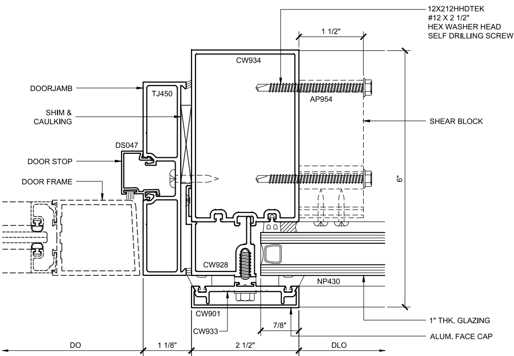
DOOR JAMB PLAN 89 DOUBLE GLAZED 4" BACK MEMBER OH DOOR FRAMING
