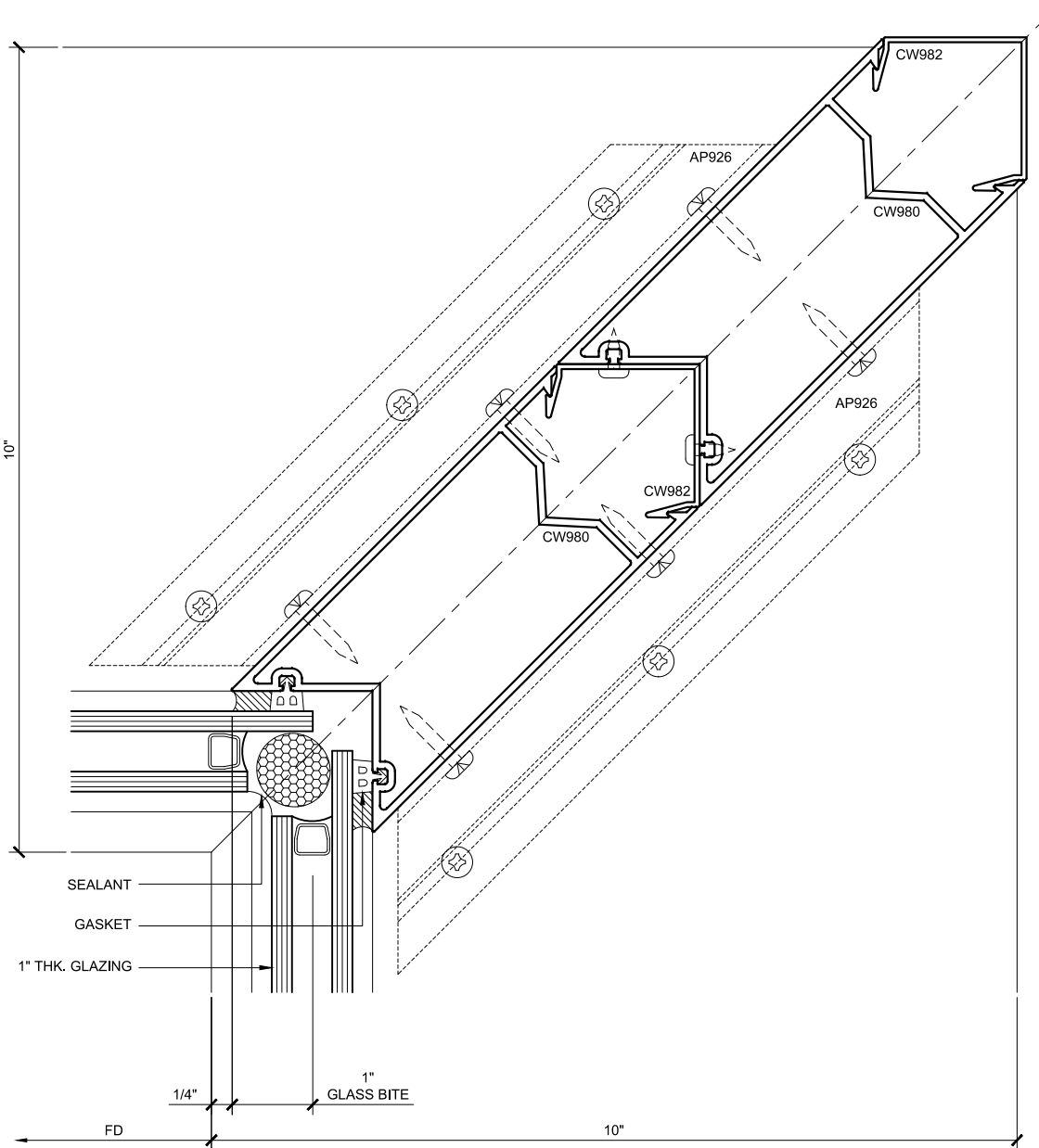
INSIDE COR. VERT. SECTION 17A DOUBLE GLAZED 8" BACK MEMBER TRANSITION DETAIL ALTERNATE DETAIL
