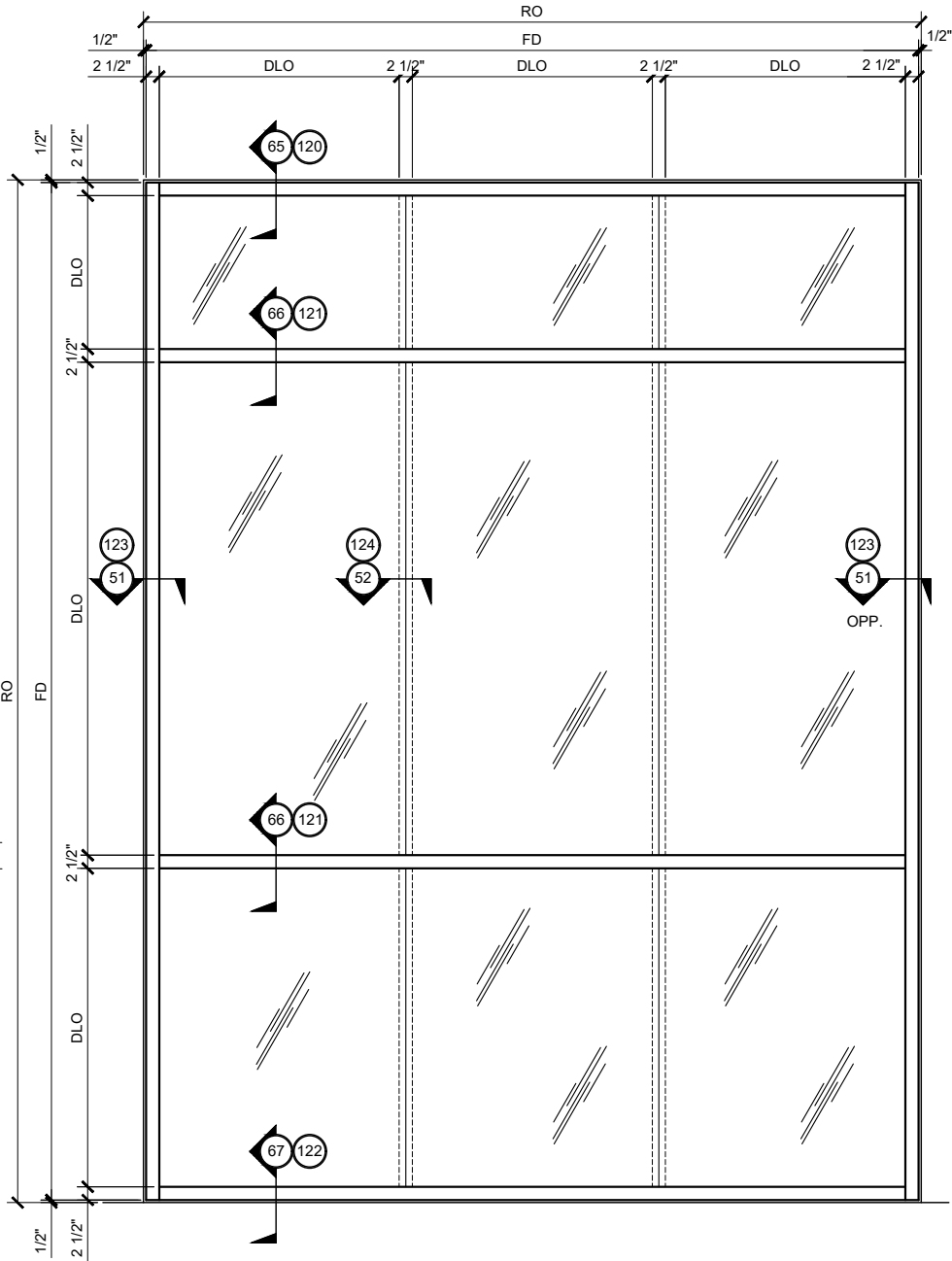
TYPICAL CURTAIN WALL ELEVATION
