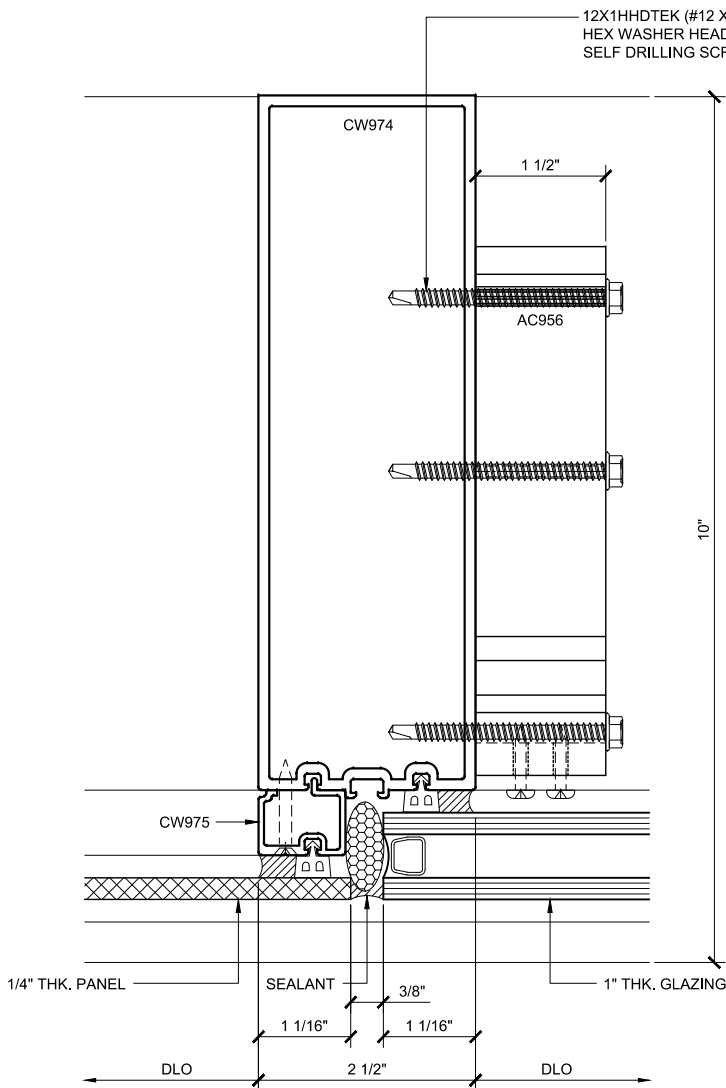
INT. VERT. PLAN 137 DOUBLE GLAZED 8" BACK MEMBER TRANSITION DETAIL
