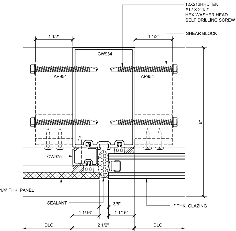
INT. VERT. PLAN 73 DOUBLE GLAZED 4\"/>
