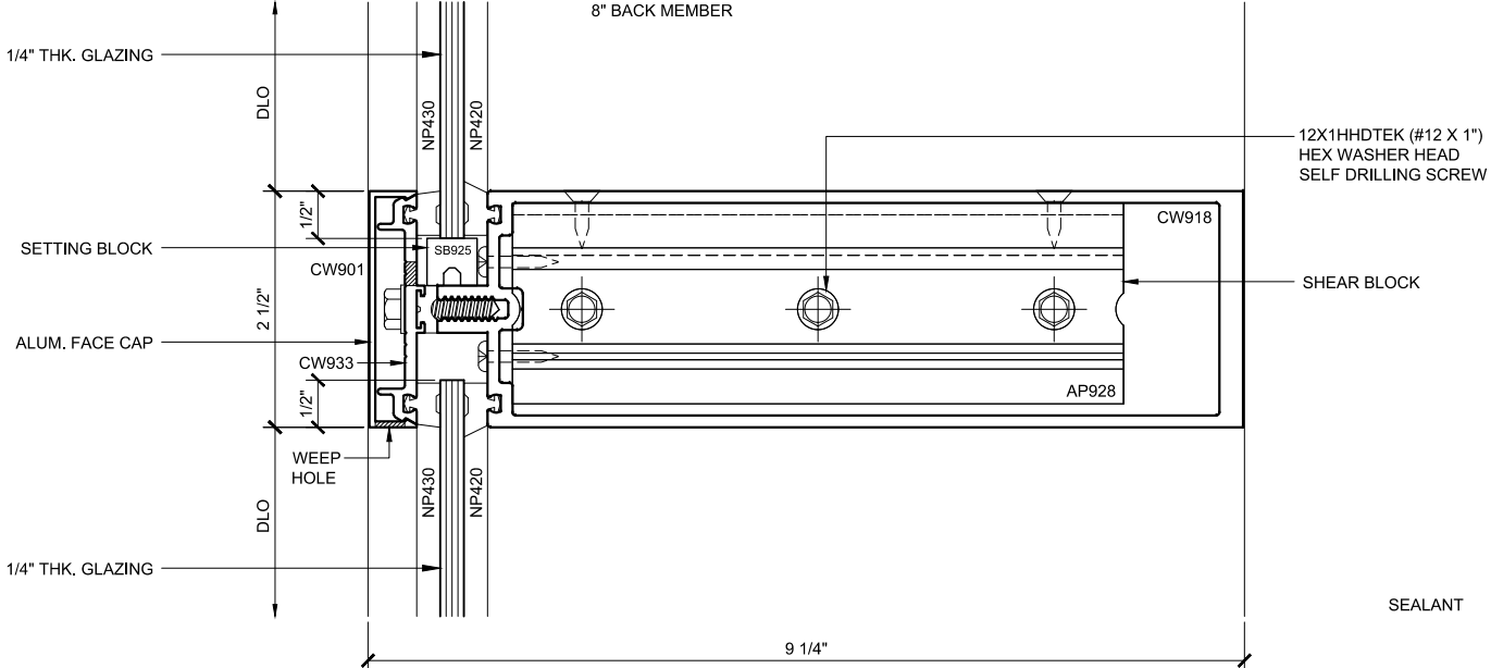
INT. HOR. SECTION 20
