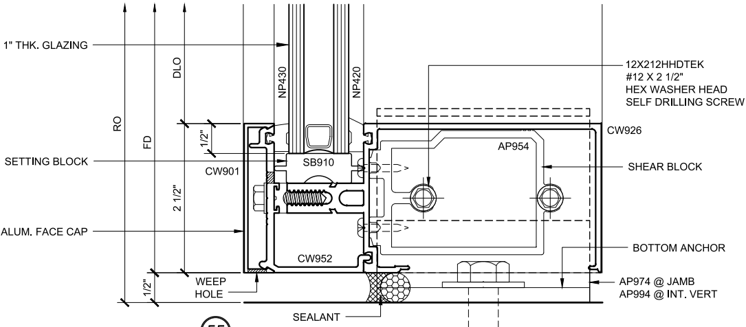
SILL SECTION 55 DOUBLE GLAZED 4" BACK MEMBER
