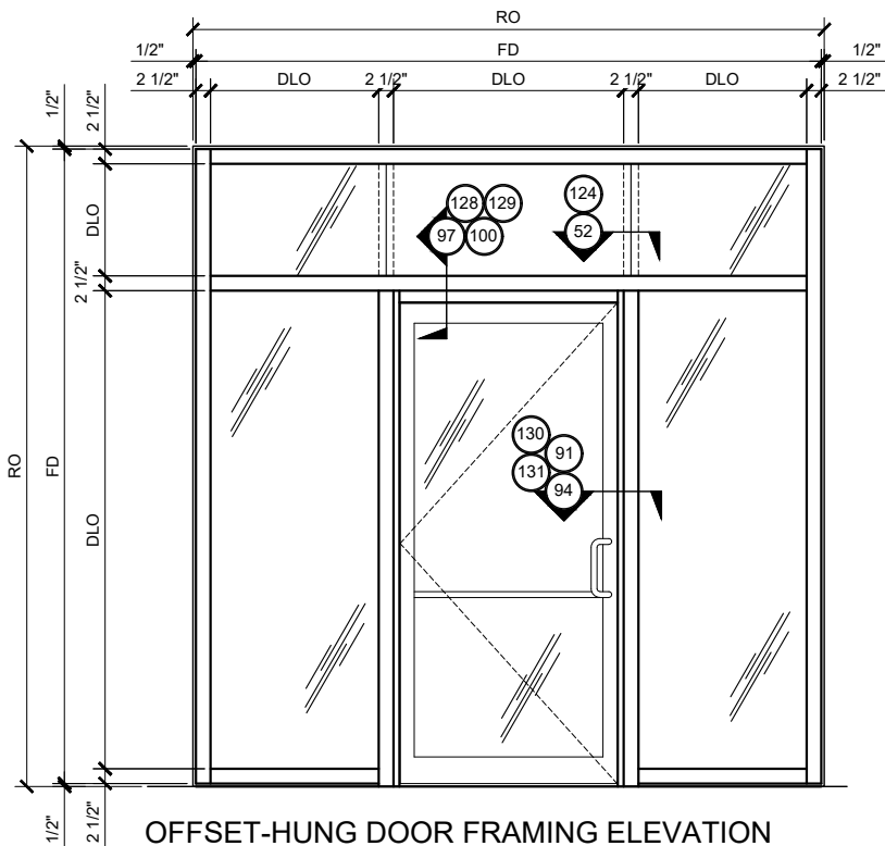
OFFSET-HUNG DOOR FRAMING ELEVATION
