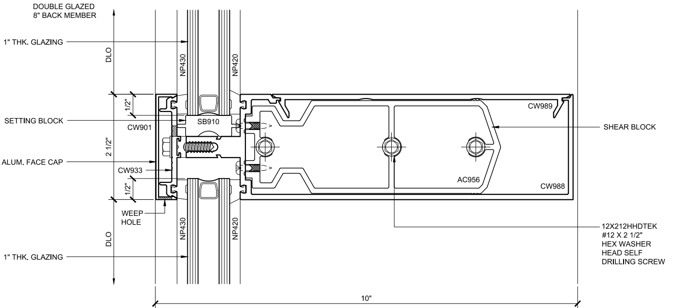
INT. HOR. SECTION 121
