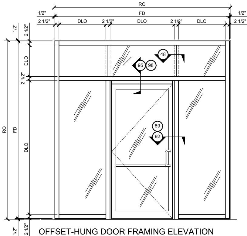
OFFSET-HUNG DOOR FRAMING ELEVATION DOUBLE GLAZED 4" BACK MEMBER
