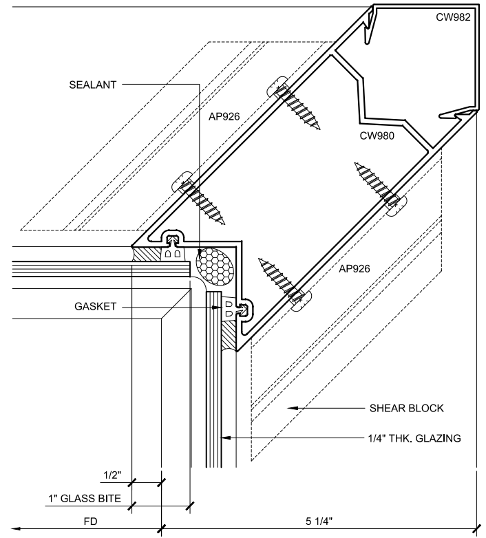
COR. VERT. PLAN ②④
