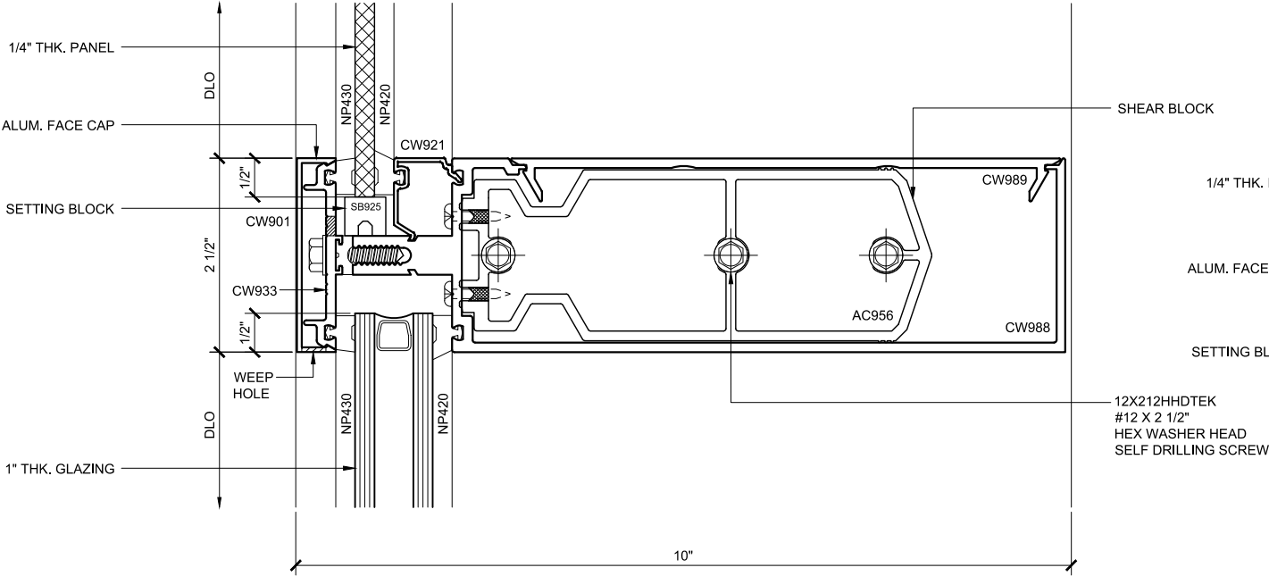
INT. HORIZ. SECTION 133 DOUBLE GLAZED 8" BACK MEMBER TRANSITION DETAILS
