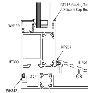
2 SILL
