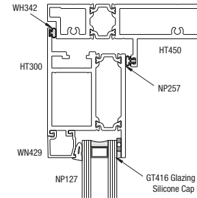
1 HEAD
