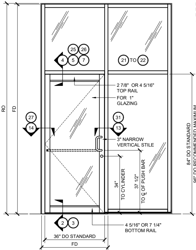
NARROW STILE SERIES 250AT DOOR TYP. ELEVATION (SINGLE DOOR @ TRANSOM FRAME ) 3/4" =1'-0"
