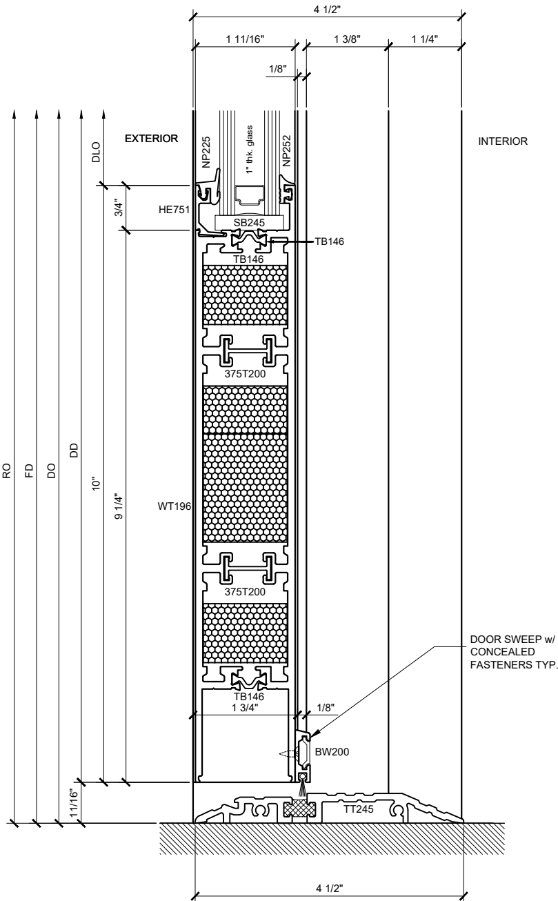
SECTION DETAIL @ 10" DOOR SILL ① SCALE: FULL SIZE
