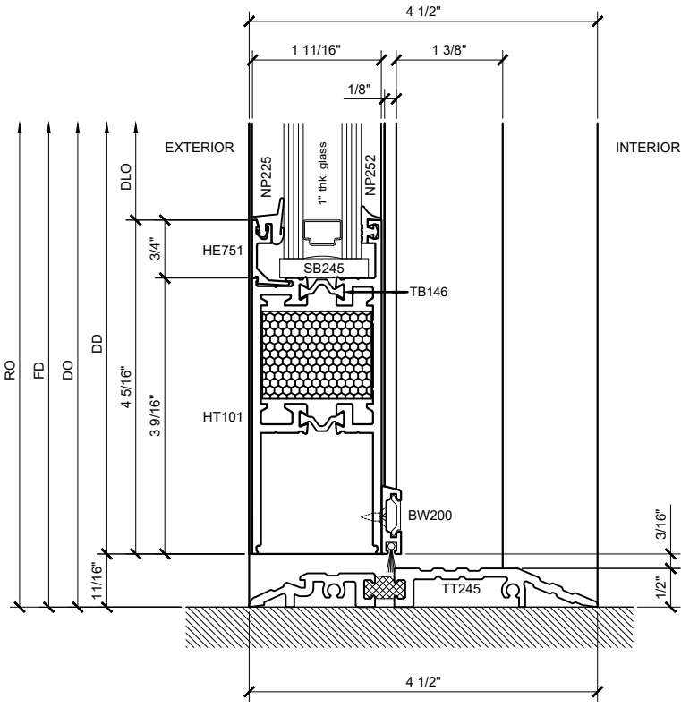
SECTION DETAIL @ 4 5/16" DOOR SILL ③ SCALE: FULL SIZE
