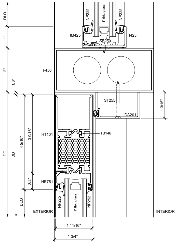
SECTION DETAIL @ 4-5/16" TOP RAIL w/ OHCC ④ SCALE: FULL SIZE
