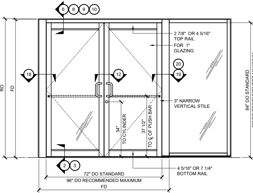
NARROW STILE SERIES 250AT DOOR TYP. ELEVATION (DOUBLE DOOR @ UP / OVER FRAME WITH SIDELITE) 3/4" =1'-0"
