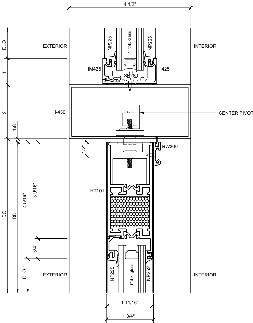
SECTION DETAIL @ 4-5/16" TO RAIL w/ OHCC 25 SCALE: FULL SIZE
