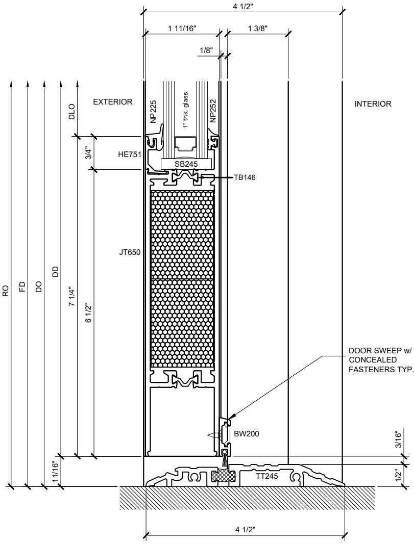
SECTION DETAIL @ 7 1/4" DOOR SILL ② SCALE: FULL SIZE
