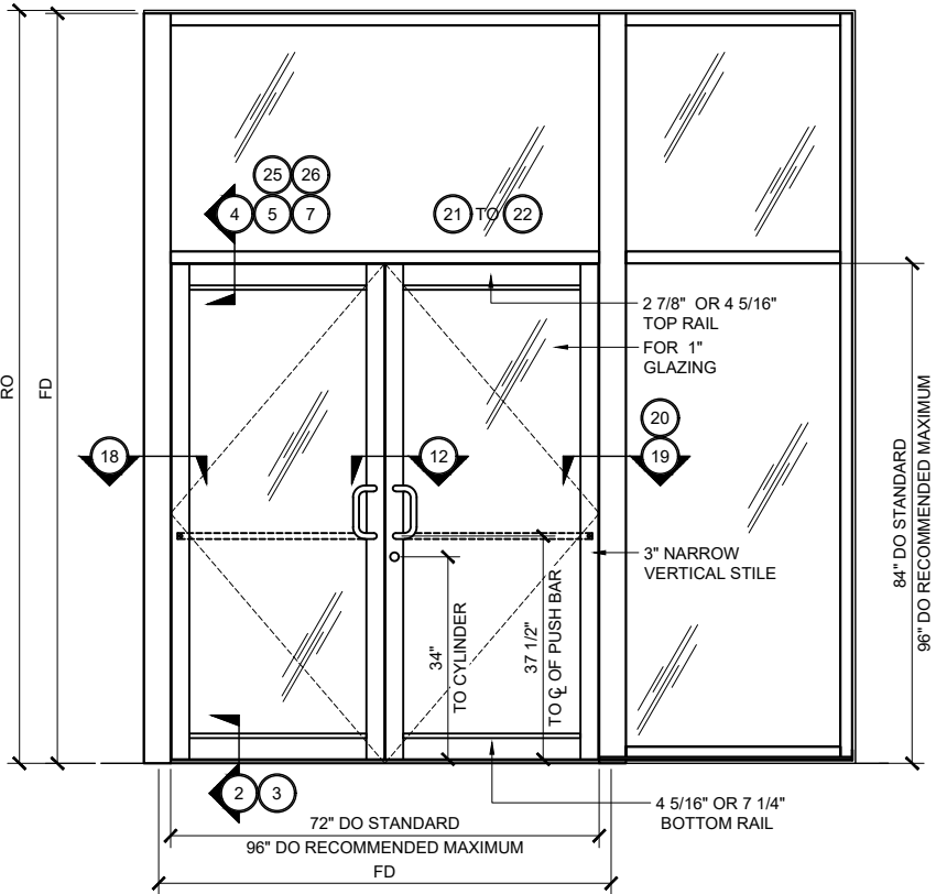
NARROW STILE SERIES 250AT DOOR TYP. ELEVATION (DOUBLE DOOR @ TRANSOM FRAME ) 3/4" =1'-0"
