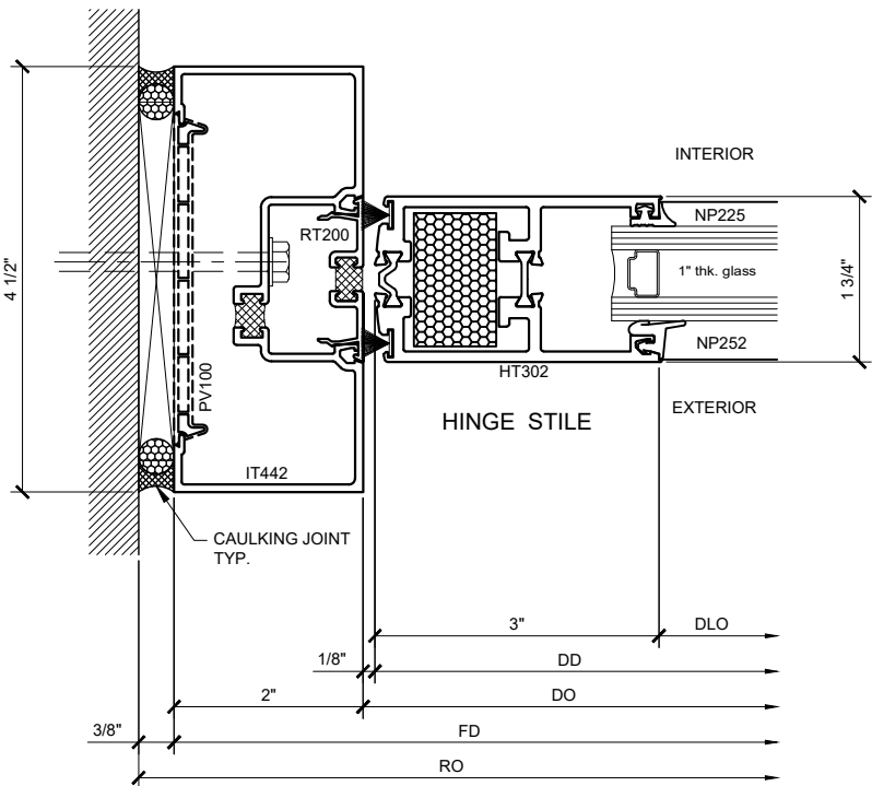
SECTION DETAIL @ DOOR JAMB 27 SCALE: FULL SIZE
