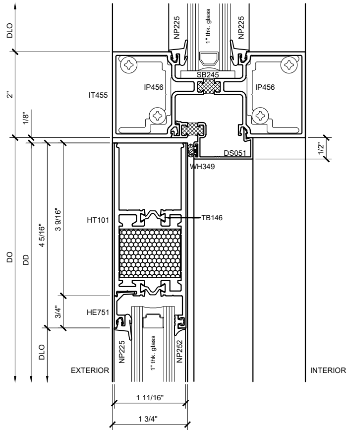
SECTION DETAIL @ 4-5/16" TOP RAIL ⑤ SCALE: FULL SIZE
