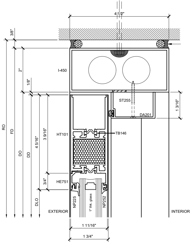
SECTION DETAIL @ 4-5/16" TO RAIL w/ OHCC ⑥ SCALE: FULL SIZE
