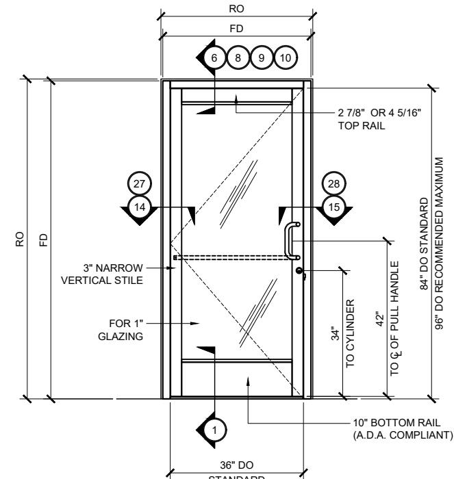
NARROW STILE SERIES 250AT DOOR TYP. ELEVATION (SINGLE DOOR @ UP / OVER FRAME ) (SHOWN W/ 10" BOTTOM RAIL) 3/4" =1'-0"
