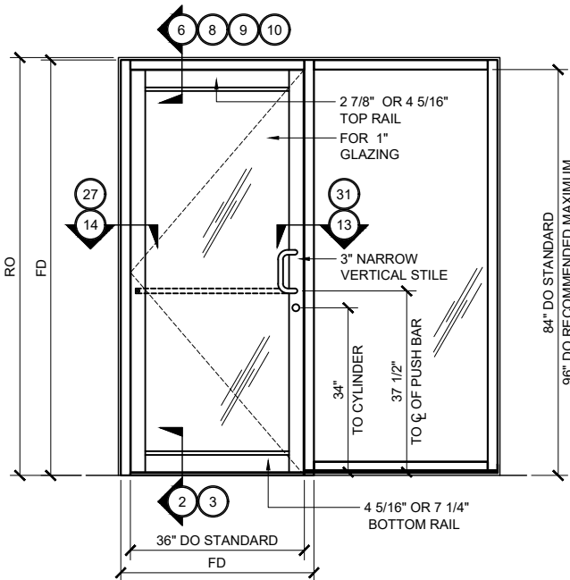
NARROW STILE SERIES 250AT DOOR TYP. ELEVATION (SINGLE DOOR @ UP / OVER FRAME WITH SIDELITE) 3/4" =1'-0"
