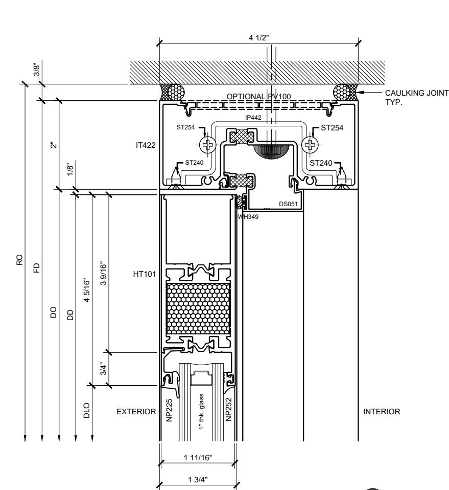
SECTION DETAIL @ 4-5/16" TOP RAIL ⑧ SCALE: FULL SIZE
