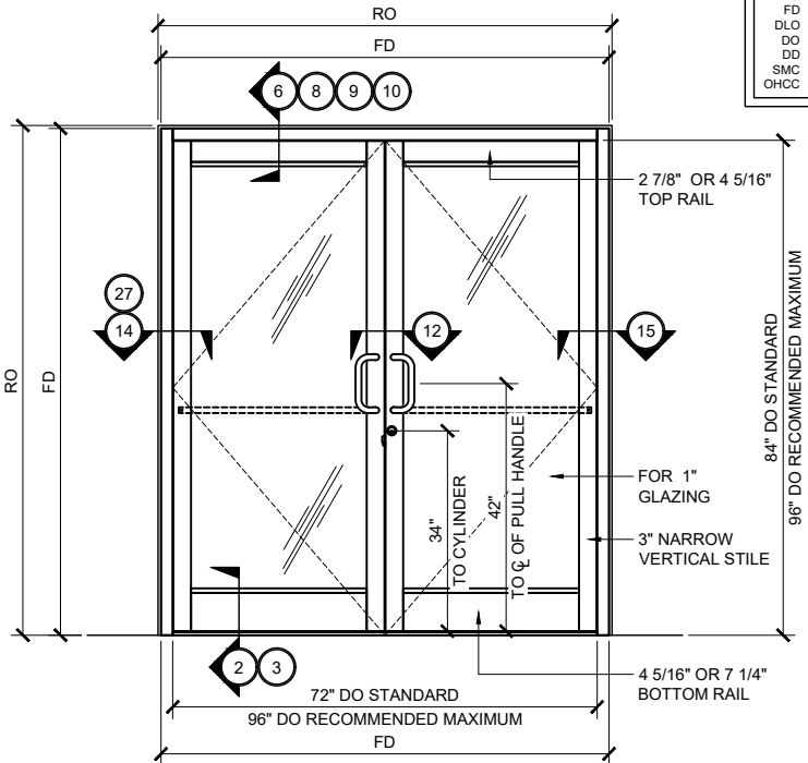
NARROW STILE SERIES 250AT DOOR TYP. ELEVATION (DOUBLE DOOR @ UP / OVER FRAME ) 3/4" =1'-0"
