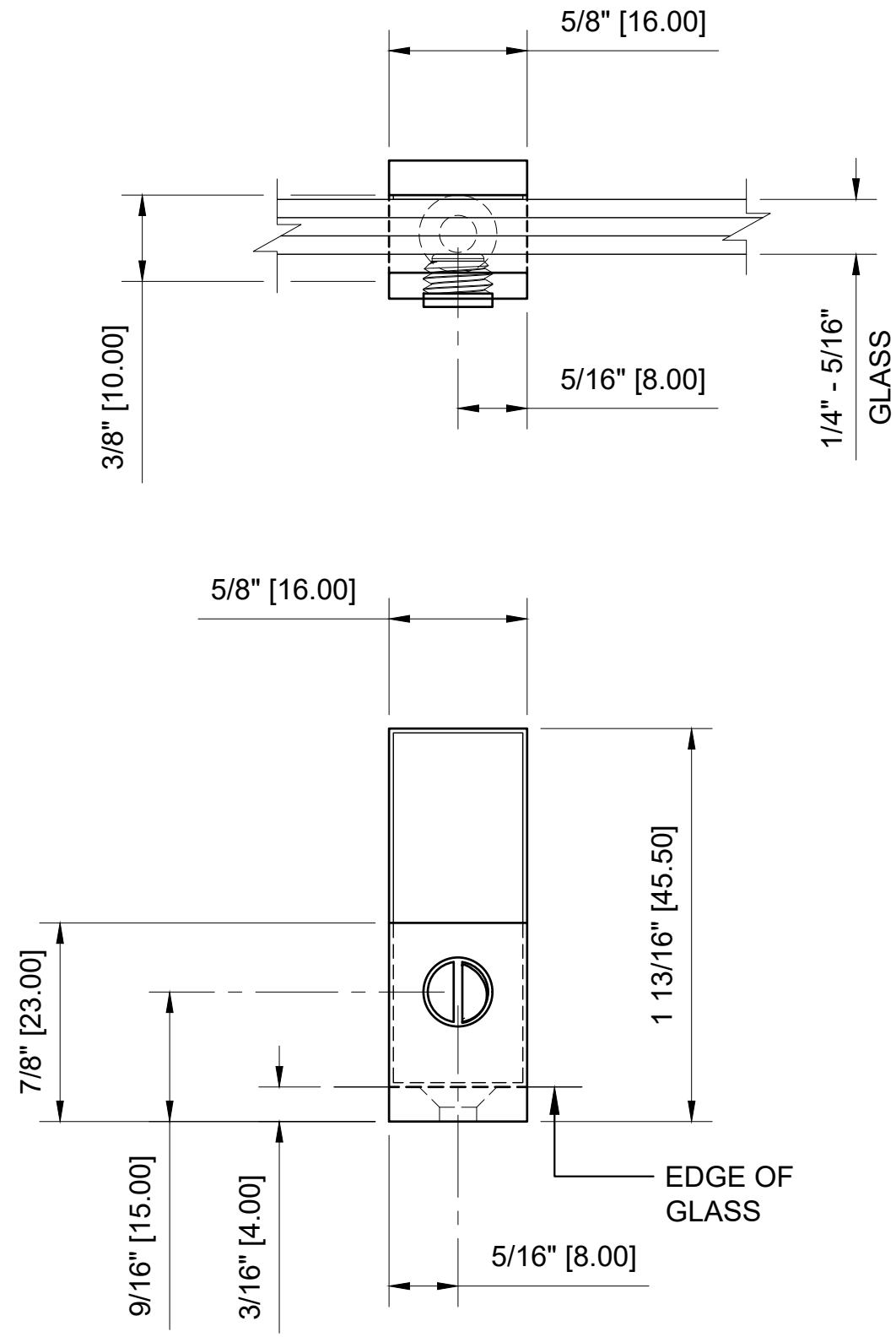
CRL - EH44 BRASS SLIM LINE "J" SET SCREW CLAMPS FOR 1/4" TO 5/16" GLASS
