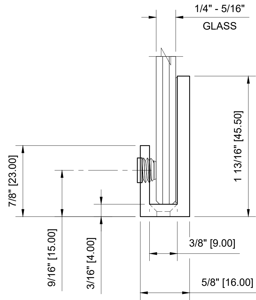
CRL - EH44 BRASS SLIM LINE "J" SET SCREW CLAMPS FOR 1/4" TO 5/16" GLASS
