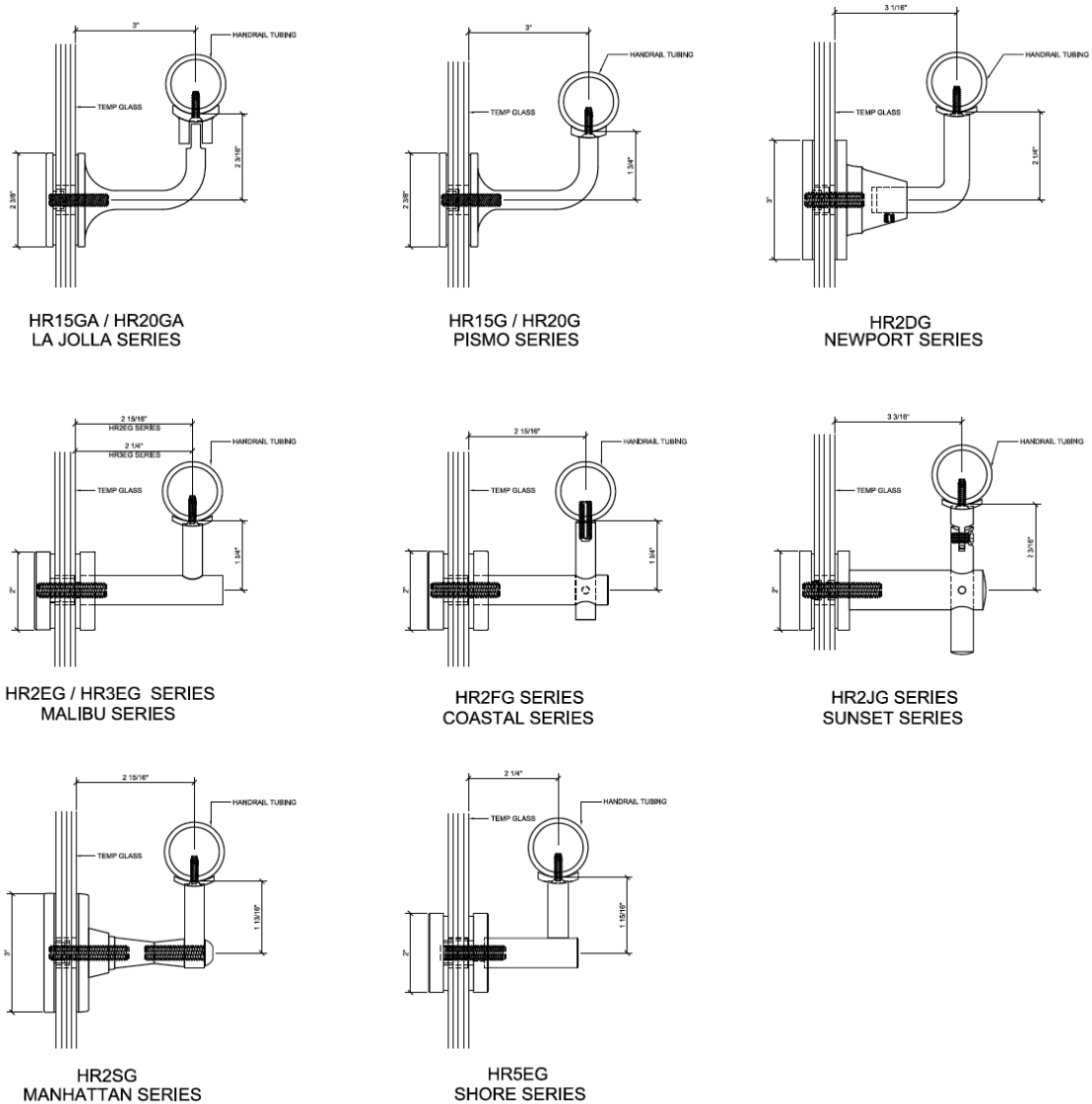
FIGURE 10—HANDRAIL BRACKETS
