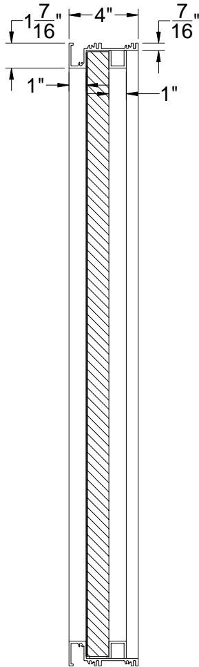
VERTICAL SECTION
