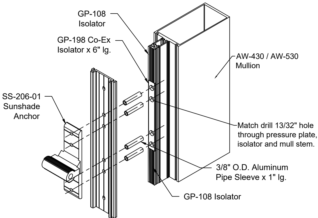
FIGURE 3 Reliance-TC Type II Curtain Wall
