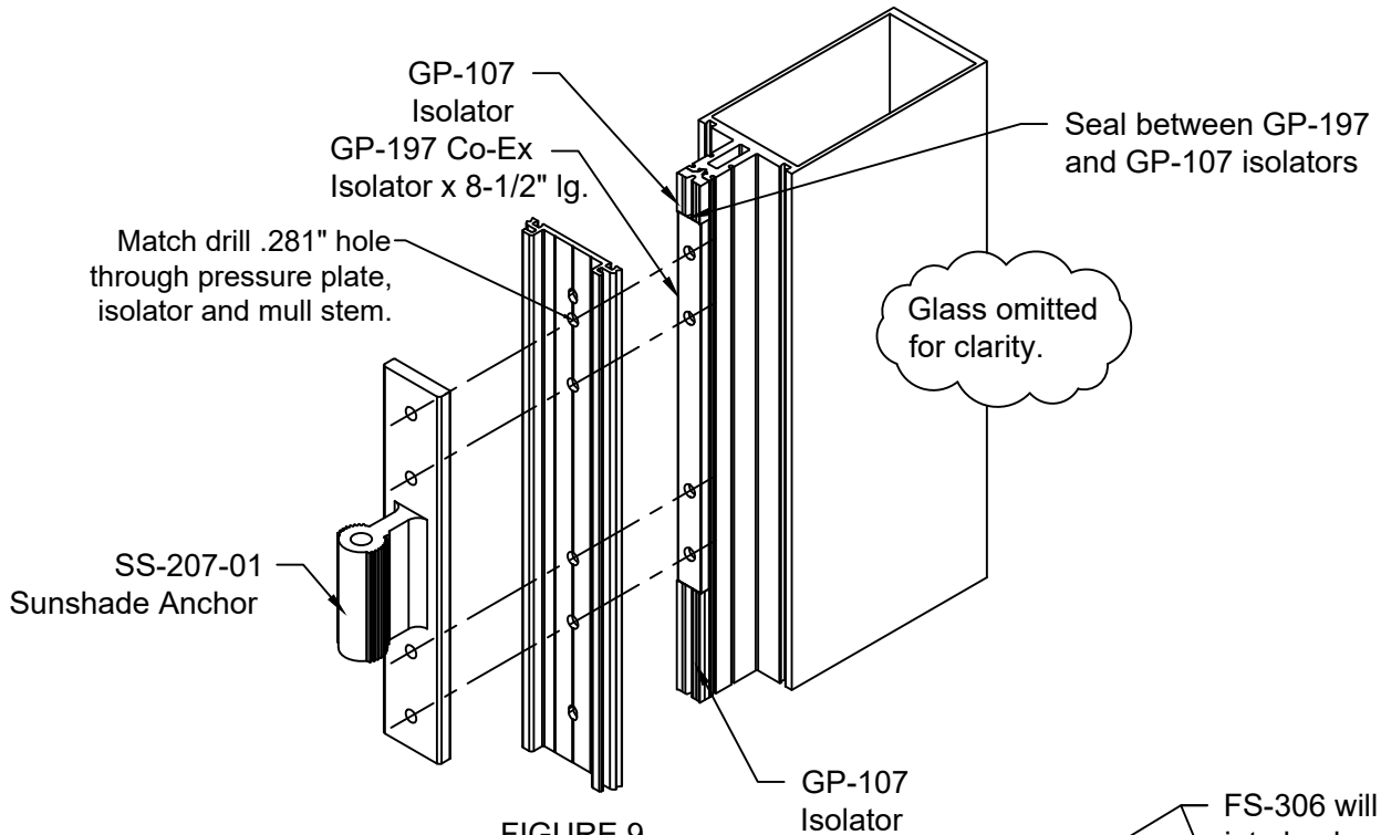
FIGURE 9 Reliance Curtain Wall
