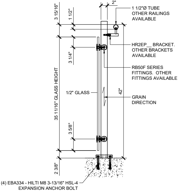
CONCRETE MOUNT SCALE: 1 1/2"=1'-0"
