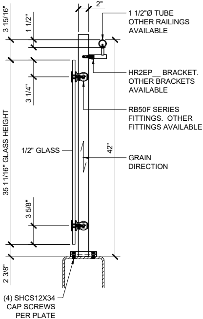
STEEL MOUNT SCALE: 1 1/2"=1'-0"
