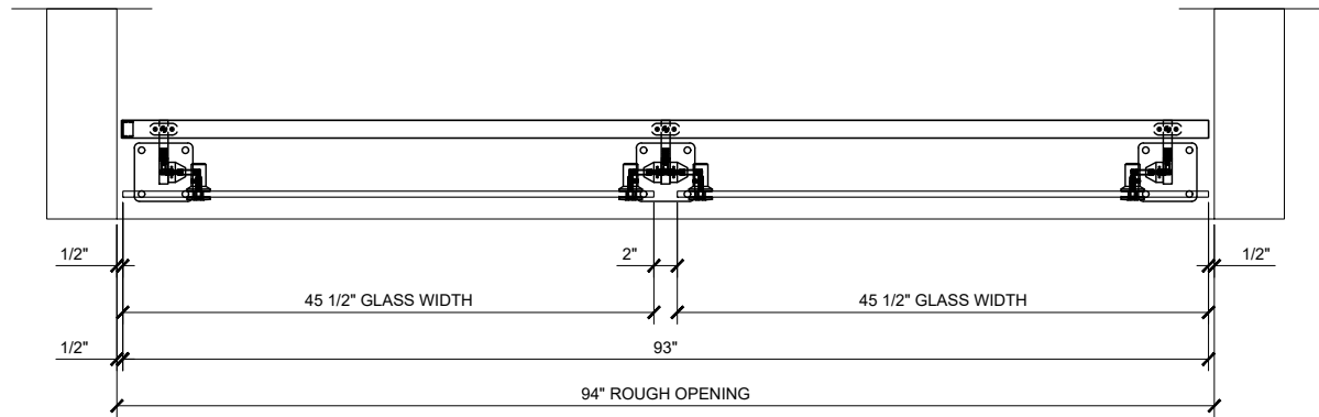
TYPICAL PLAN VIEW SCALE: 1 1/2"=1'-0"
