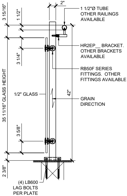
WOOD MOUNT SCALE: 1 1/2"=1'-0"
