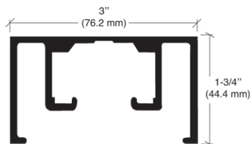
D1670 OVERHEAD TRACK When Matching a Store Front Extrusion, D1670 Upper Track may be used. Specify D1039 Assembly
