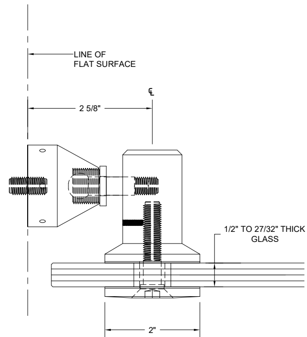
WALL MOUNT
