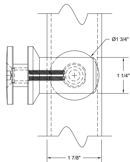
WALL MOUNT
