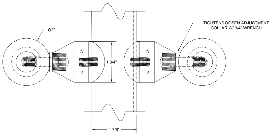
POST MOUNT
