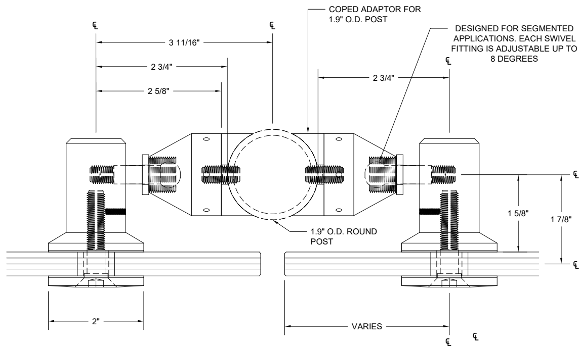
POST MOUNT
