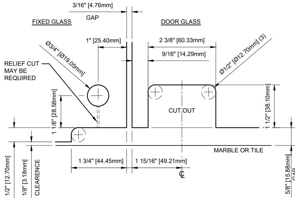
BOTTOM MOUNT METHOD
