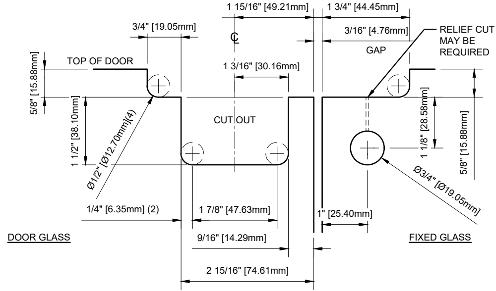
TOP FLUSH MOUNT METHOD
