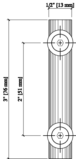
GLASS FABRICATION
