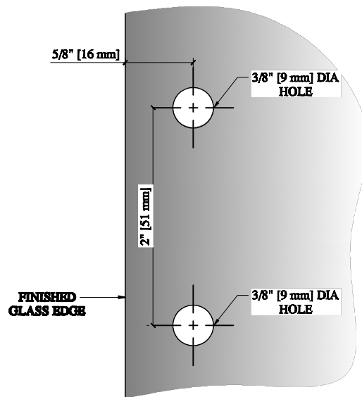
GLASS FABRICATION
