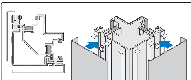
90° Inside Corner
