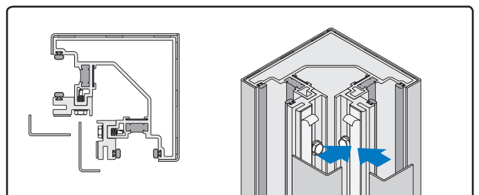
90° Outside Corner
