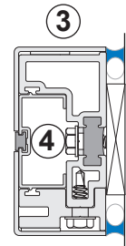
Doorway Jamb at Wall
