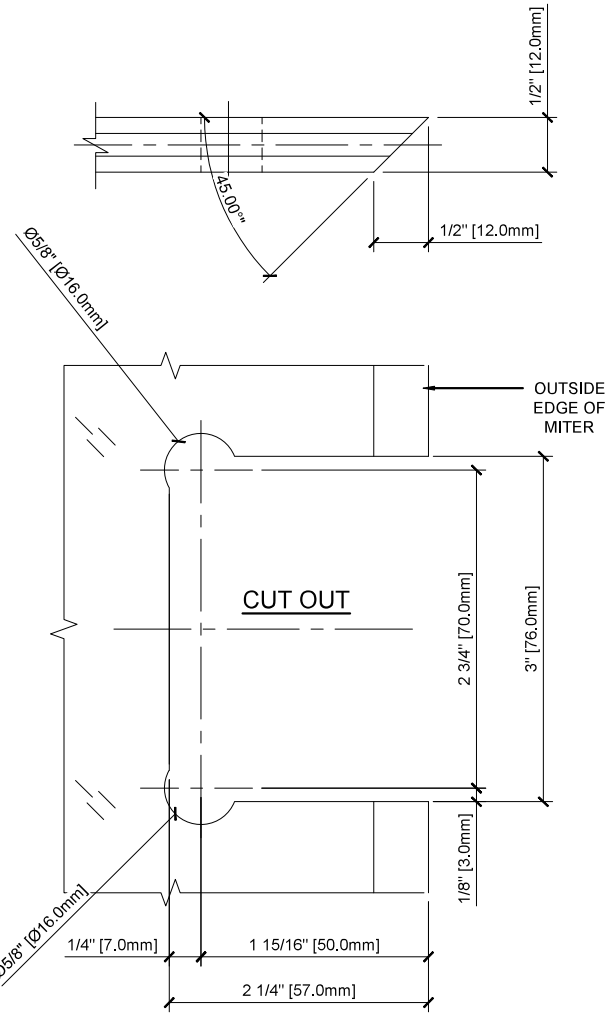
1/2" GLASS FABRICATION TEMPLATE FIXED PANEL
