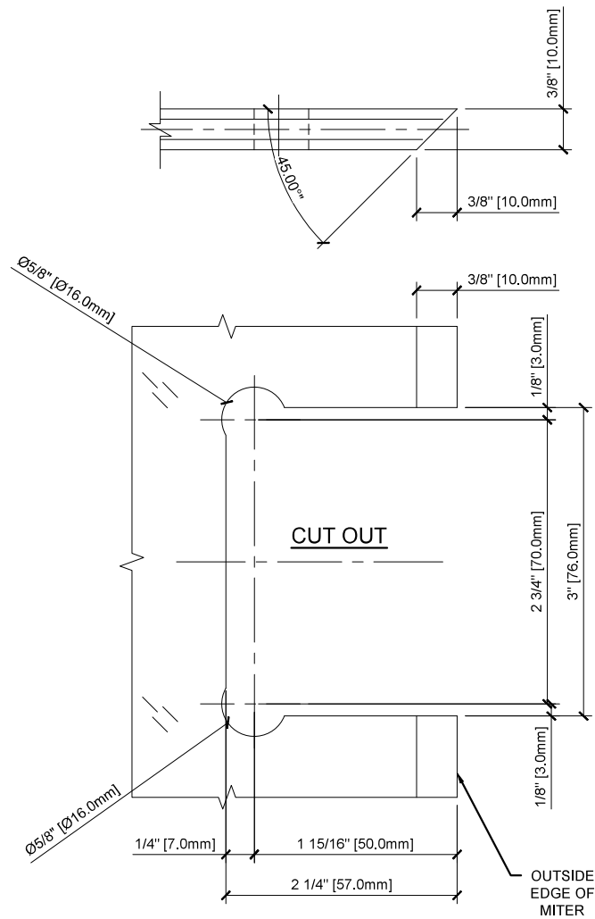
3/8" GLASS FABRICATION TEMPLATE FIXED PANEL
