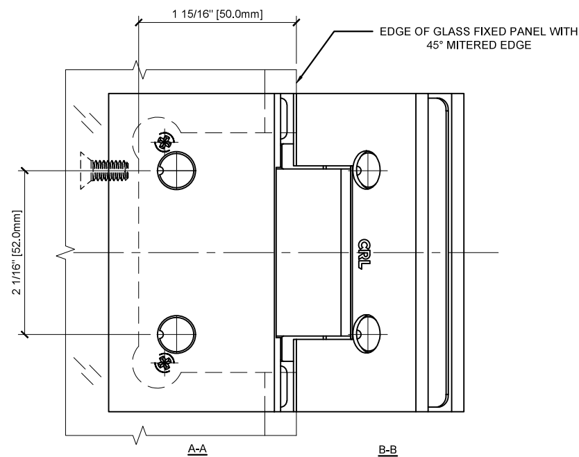
3/8" GLASS FABRICATION TEMPLATE FIXED PANEL
