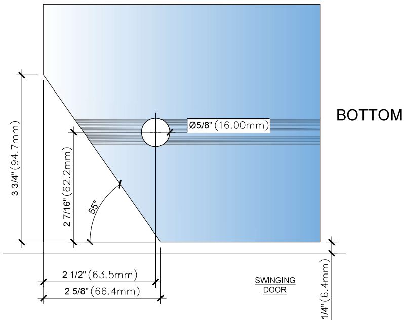
③ GLASS CUT OUT DETAIL ARCH REF: SCALE: 1'-0"=1'-0"
