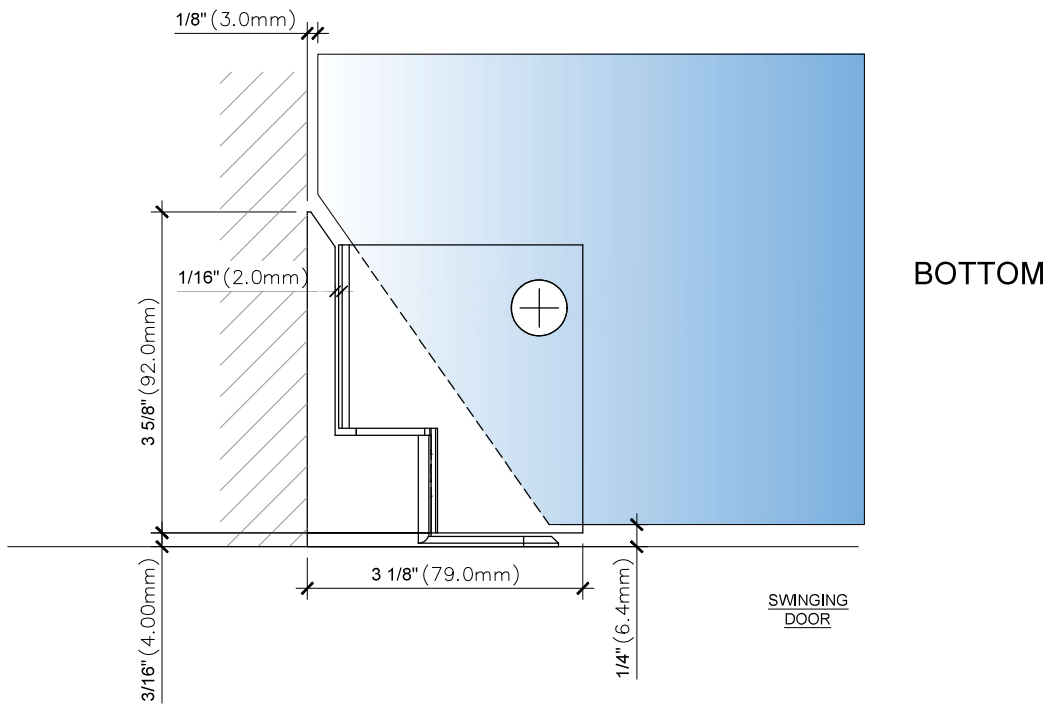
② FRONT VIEW DETAIL-WALL MOUNT SHOWN ARCH REF: SCALE: 1'-0"=1'-0"
