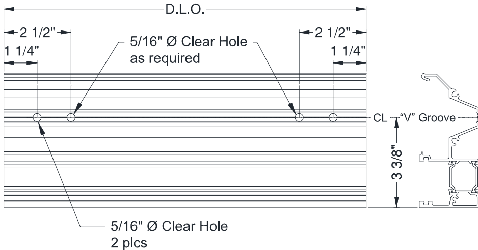
Figure 18: TWW-510 Sill Fabrication
