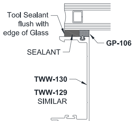
Figure 55: Structural Sealant at SSG Vertical Mullion
