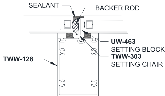
Figure 57: SSG Face Seal
