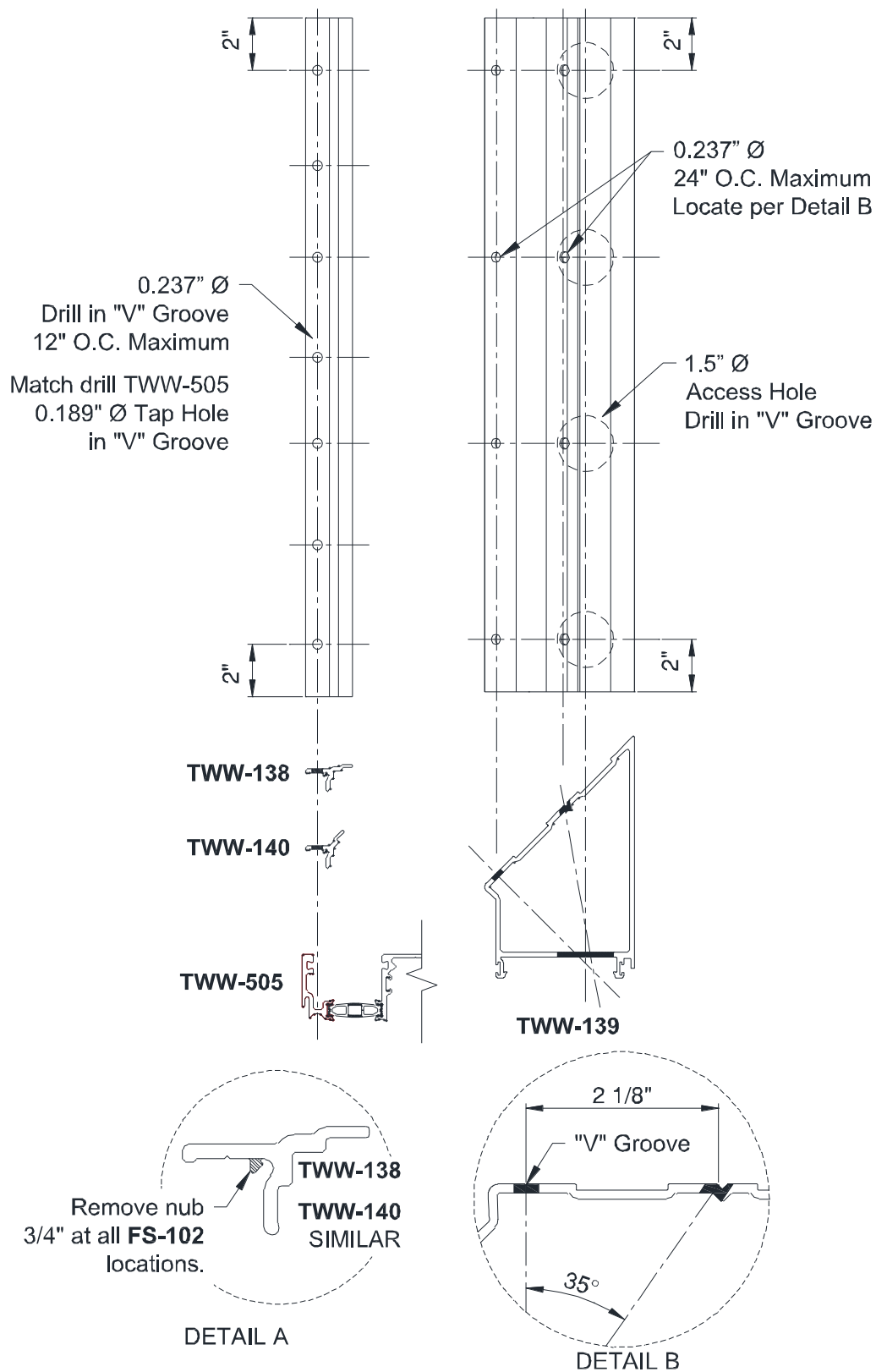
Figure 11: Inside Corner Mullion Reference Guide
