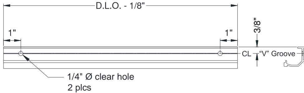
Figure 24: FWW-106 Glass Stop Fabrication
