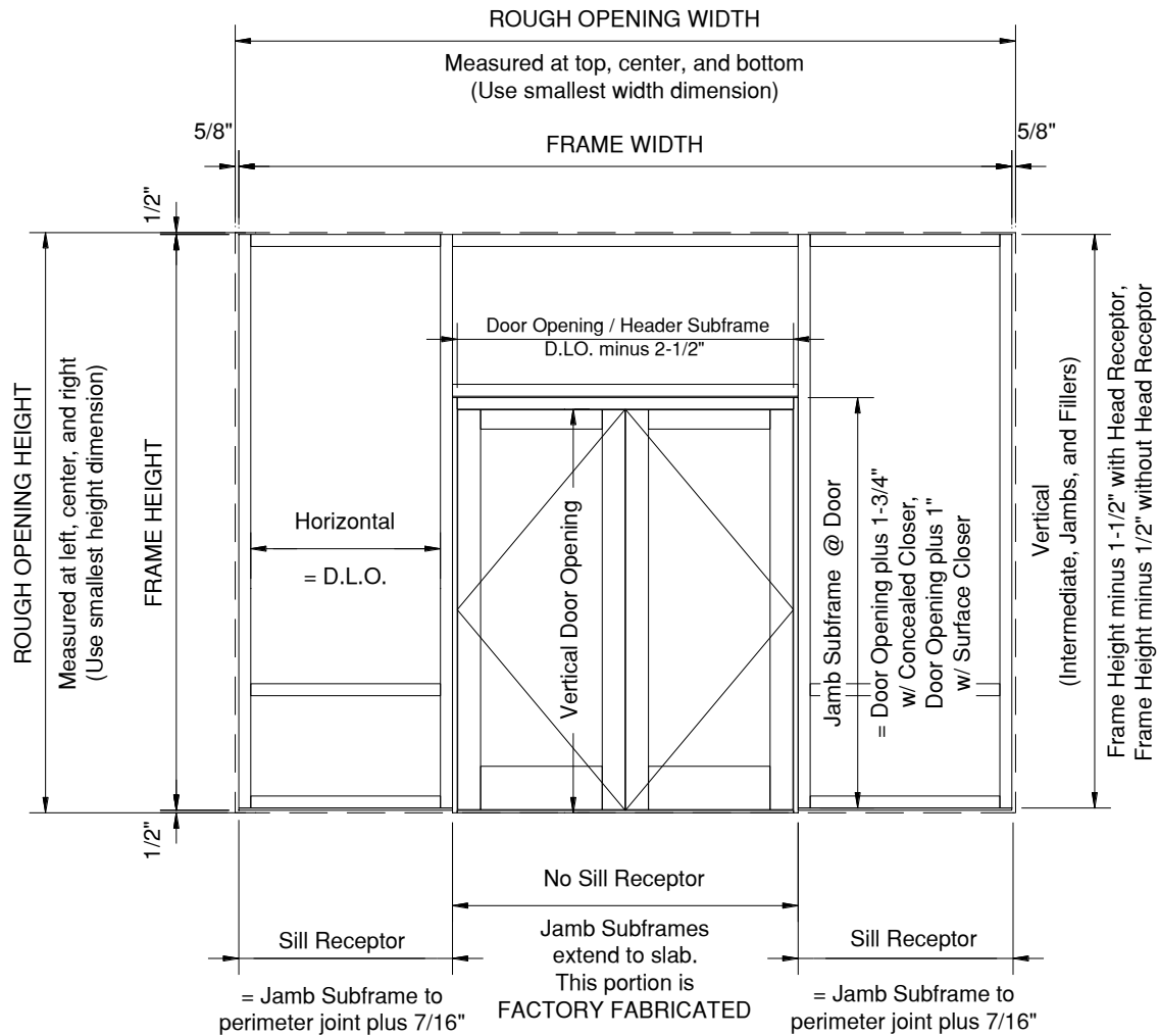
Figure 6: Measuring Rough Opening, Guide with Entrance
