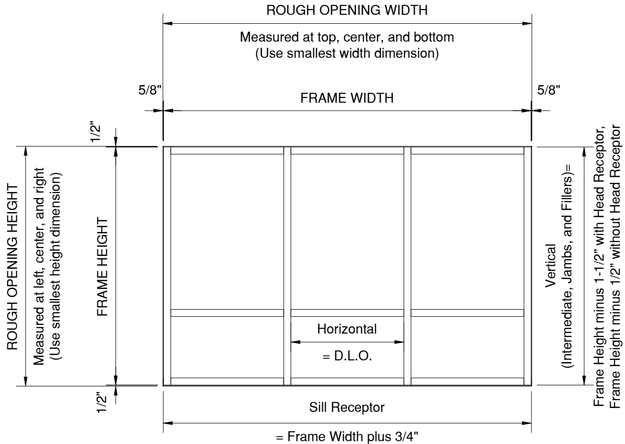
Figure 5: Measuring Rough Opening, Guide without Entrance
