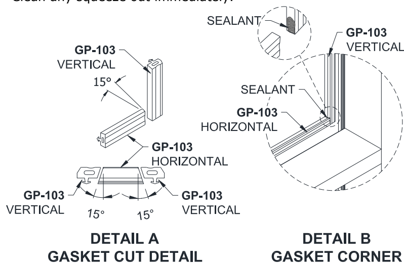
Figure 43: Fixed Gasket Installation
