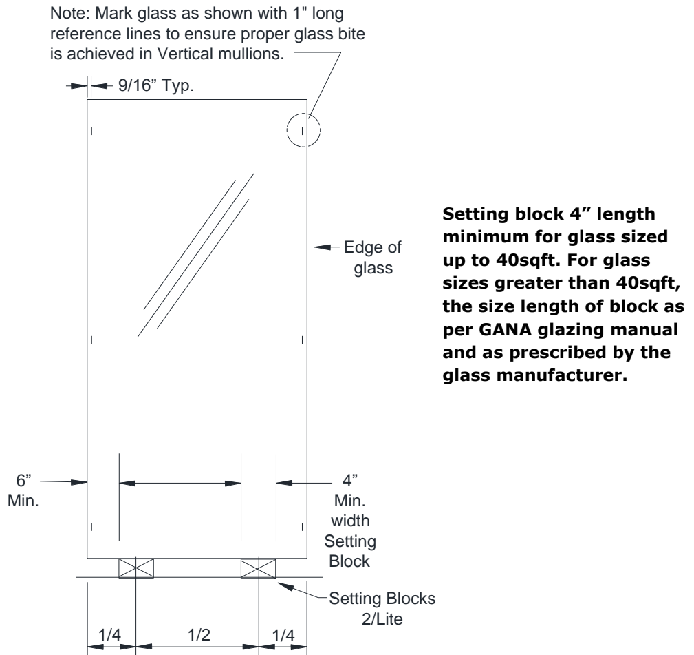
Figure 39: Glass Marking and Setting Block Locations
