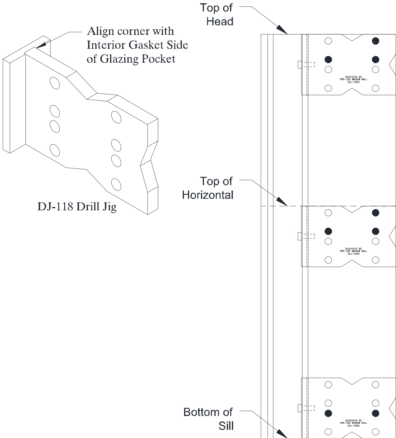
Figure 12: Drill Jig Reference Guide
