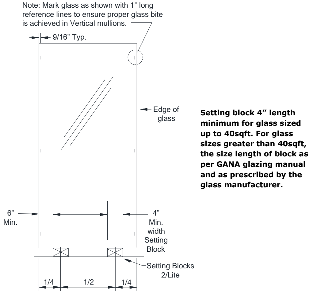
Figure 82: Glass Marking and Setting Block Locations
