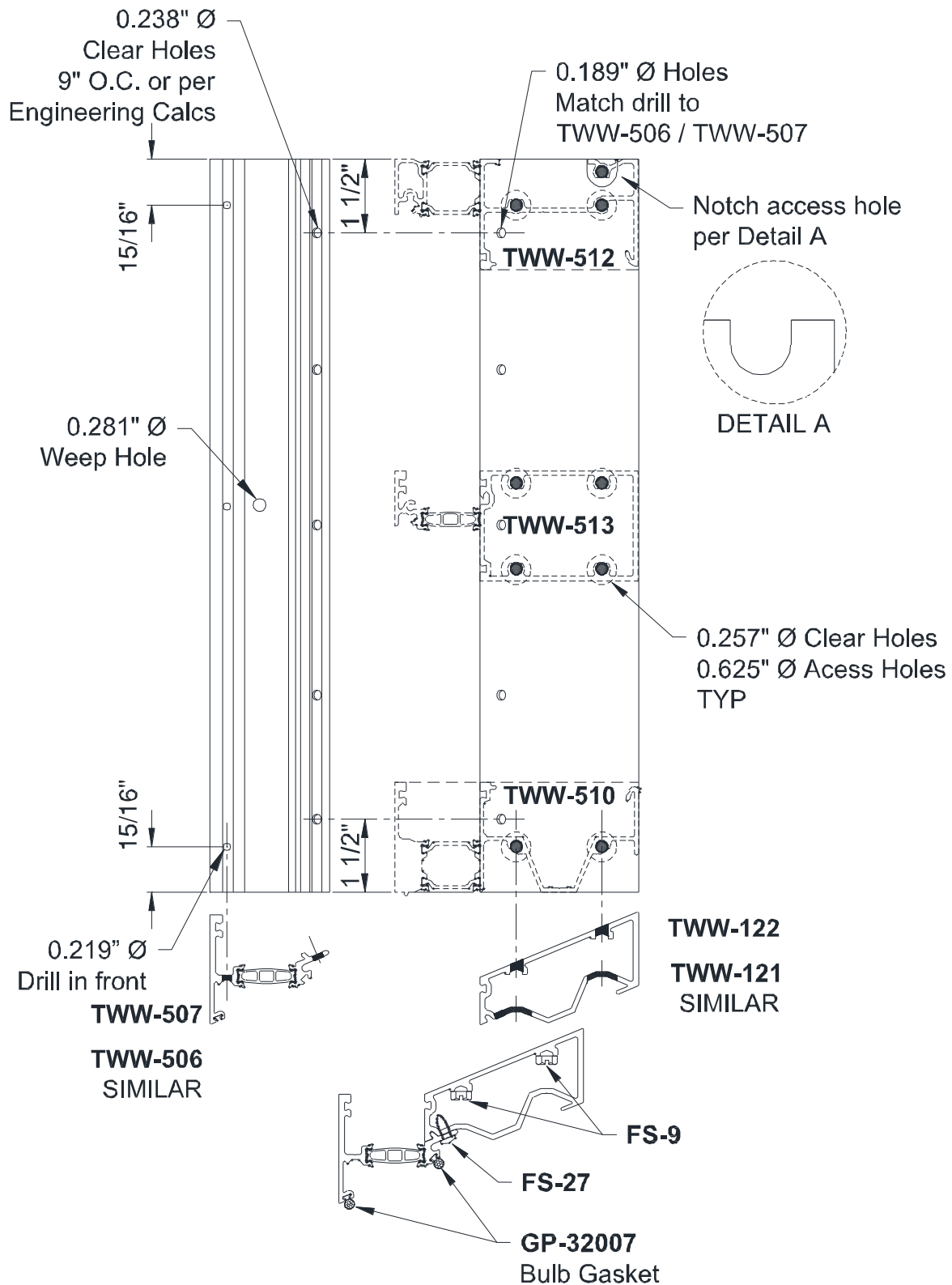
Figure 10: Outside Corner Mullion Reference Guide
