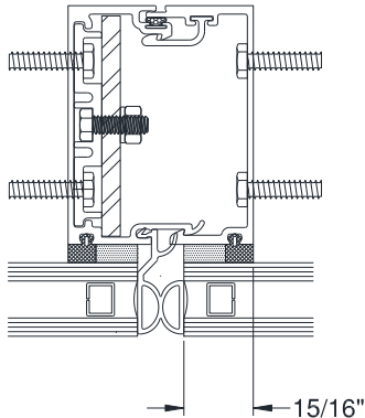
Figure 3: SSG Glass Width Guide
