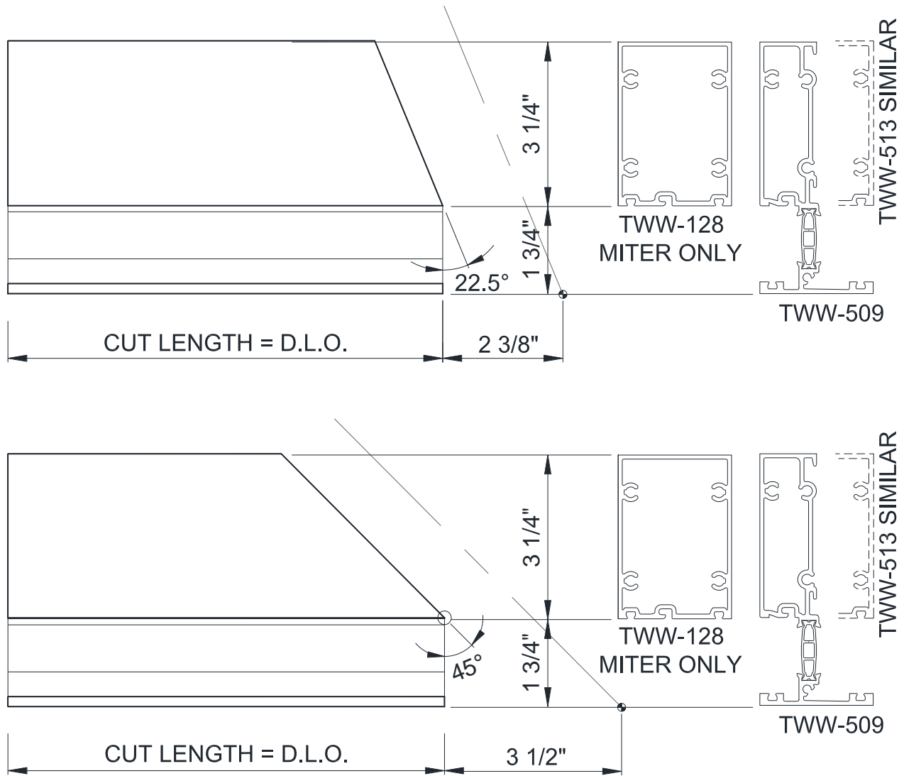
Figure 23: TWW-509 Horizontal Corner Fabrication
