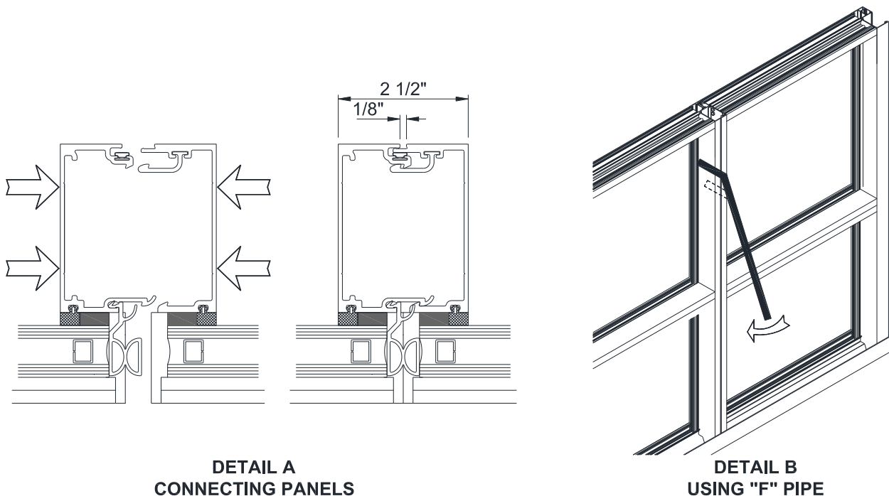
Figure 72: Panel Installation, Connecting Pre-Glazed Panels
