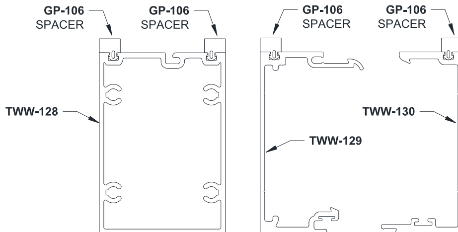
Figure 50: GP-106 Spacer Gasket Installation
