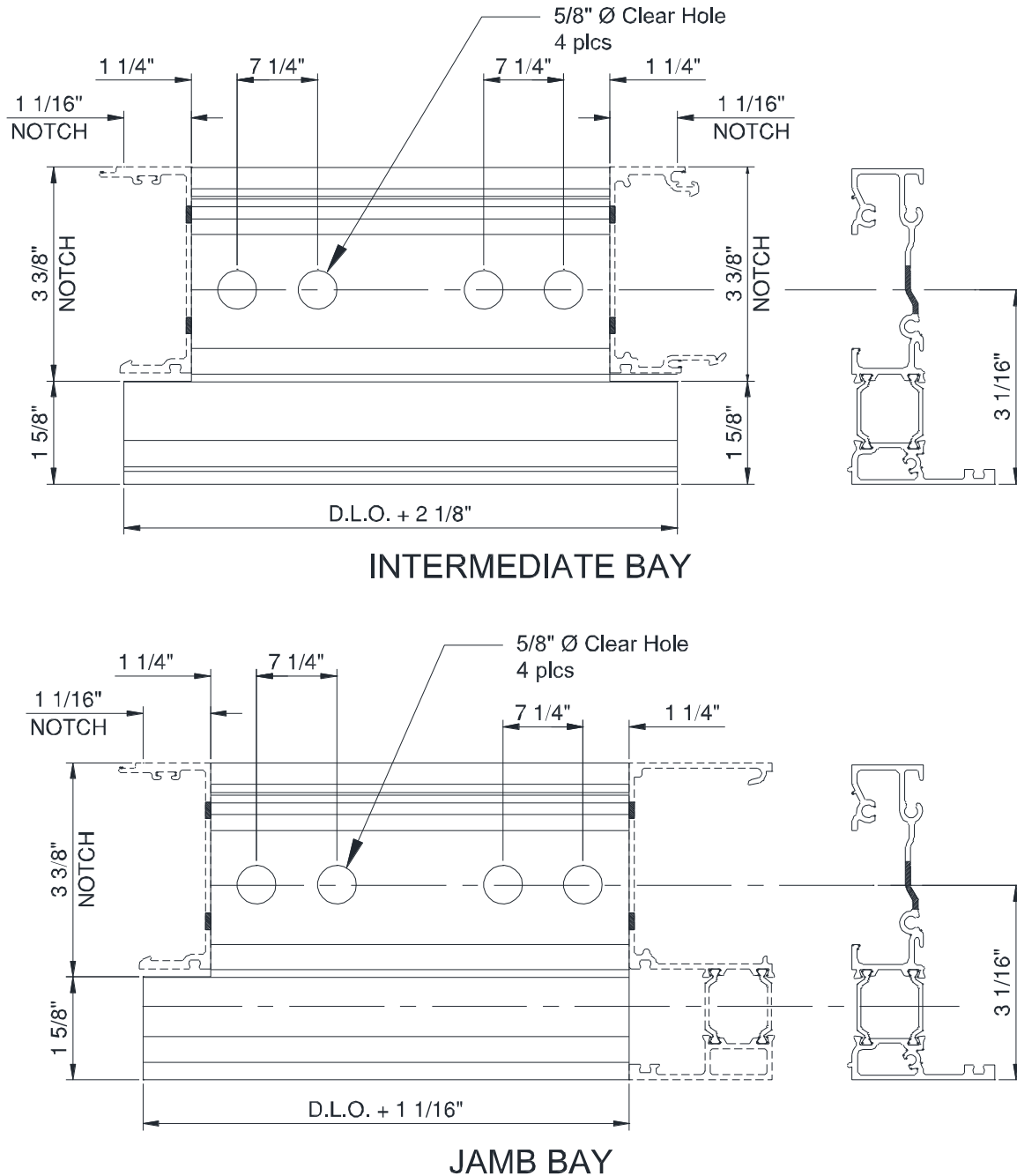
Figure 19: TWW-508 Head Fabrication
