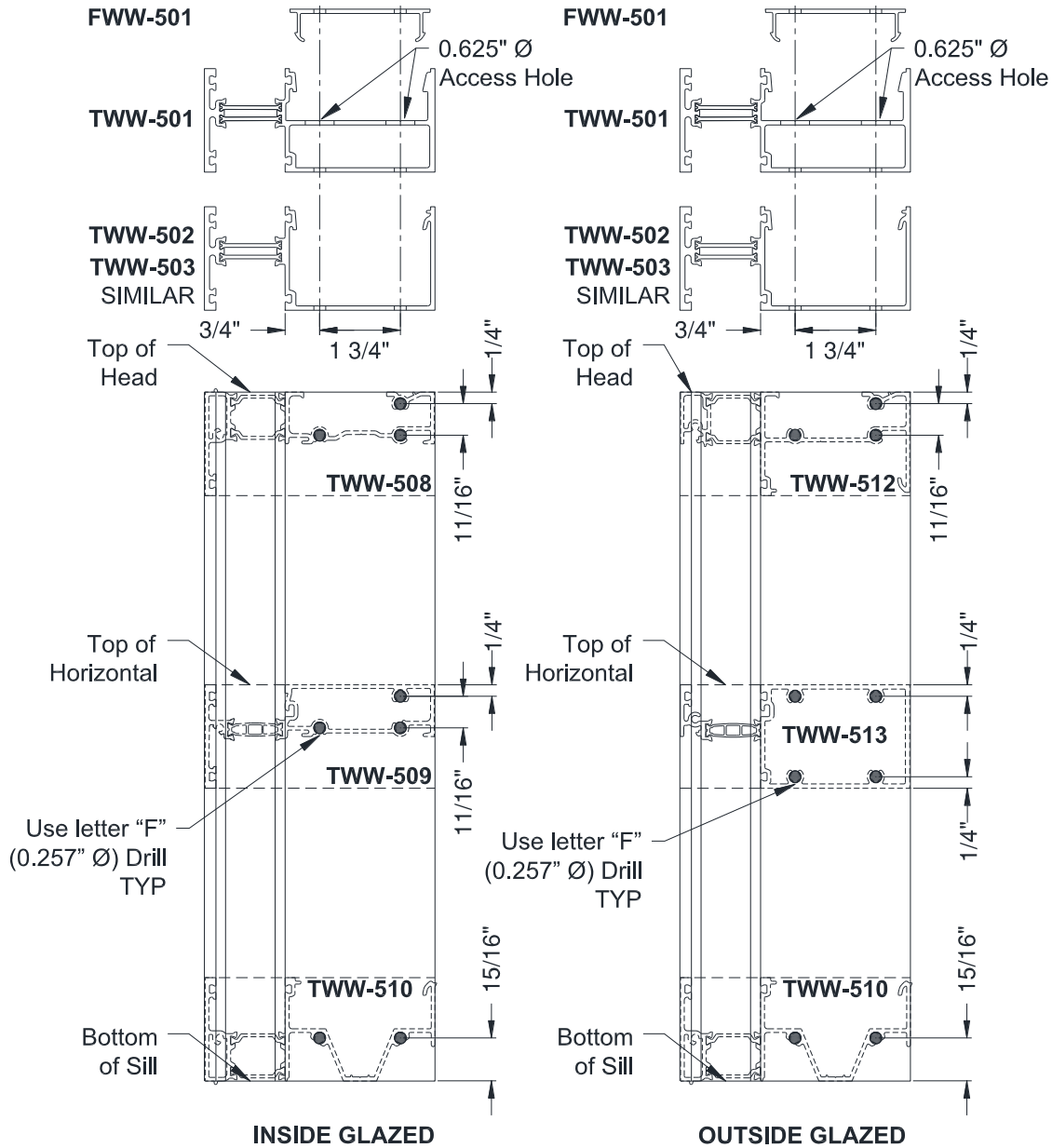
Figure 7: Field Glazed Vertical Mullion Fabrication, Jambes Similar
