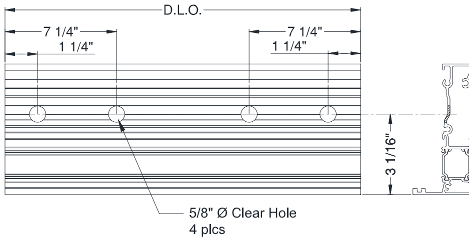
Figure 17: TWW-508 Head Fabrication
