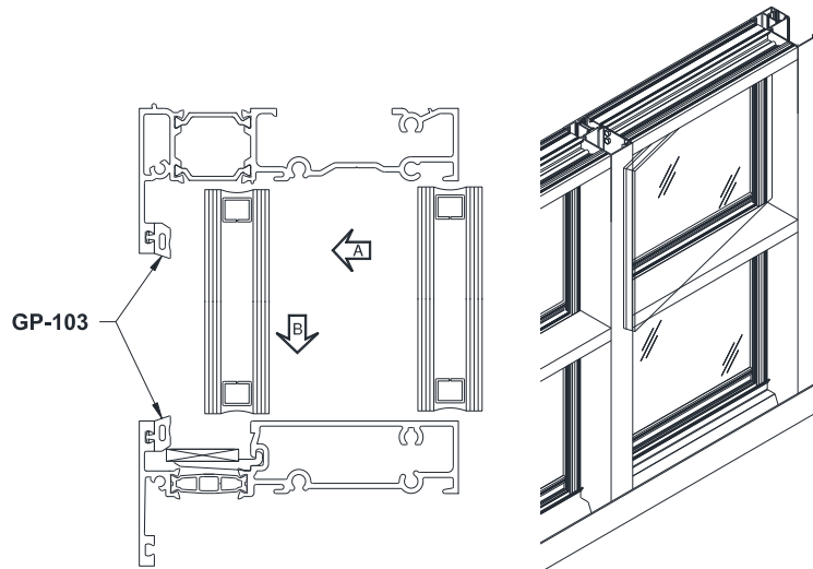
Figure 87: Glass Installation (Interior Glaze Shown)
