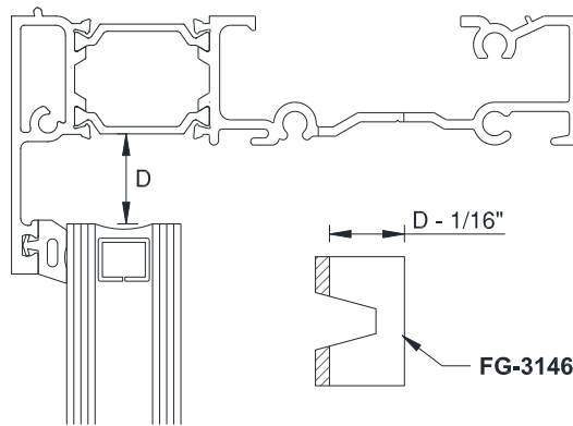
Figure 45: Optional Blocking at Head
