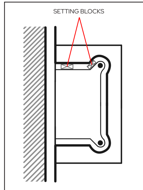
A wall mounted hinge door with setting block material between the body of the hinge and the glass cutout to block the glass into position.
