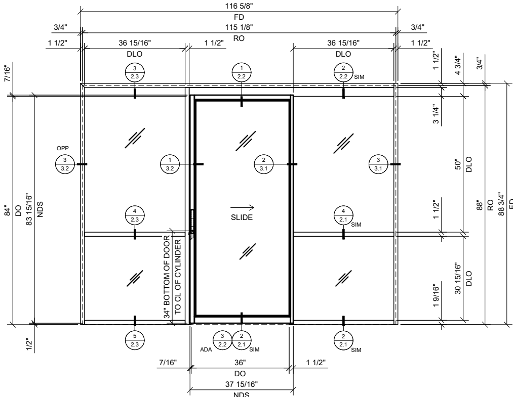
3 SINGLE SLIDER WITH BAY & SIDELITE
