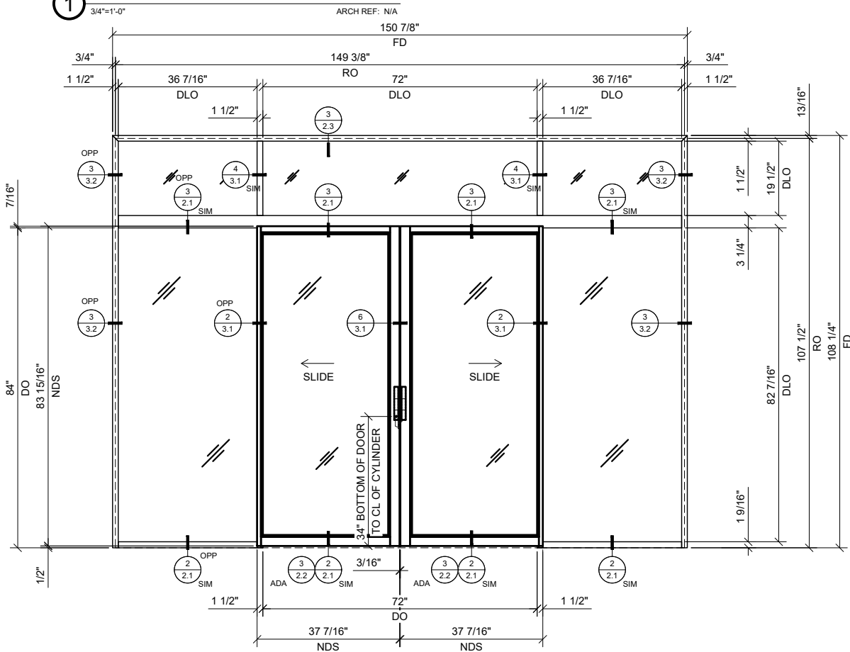
② BI-PART SLIDER WITH BAYS & TRANSOM
