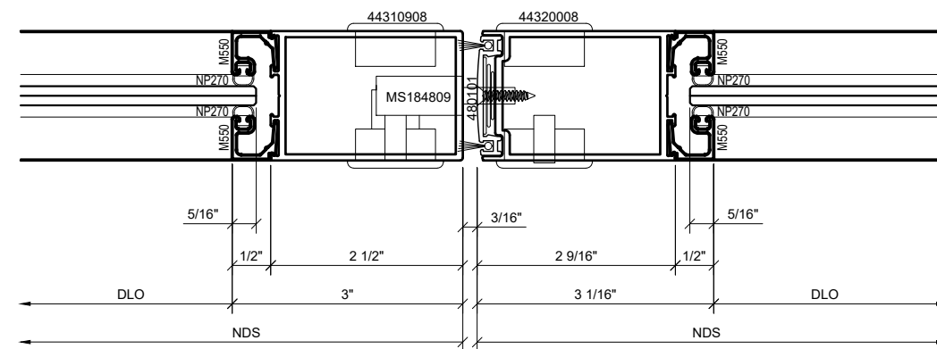
⑥ SERIES 487 OPS INTEGRATED SLIDER MEETING STILES AT DOOR PAIR DETAIL 1'-0"=1'-0" ARCH REF: N/A
