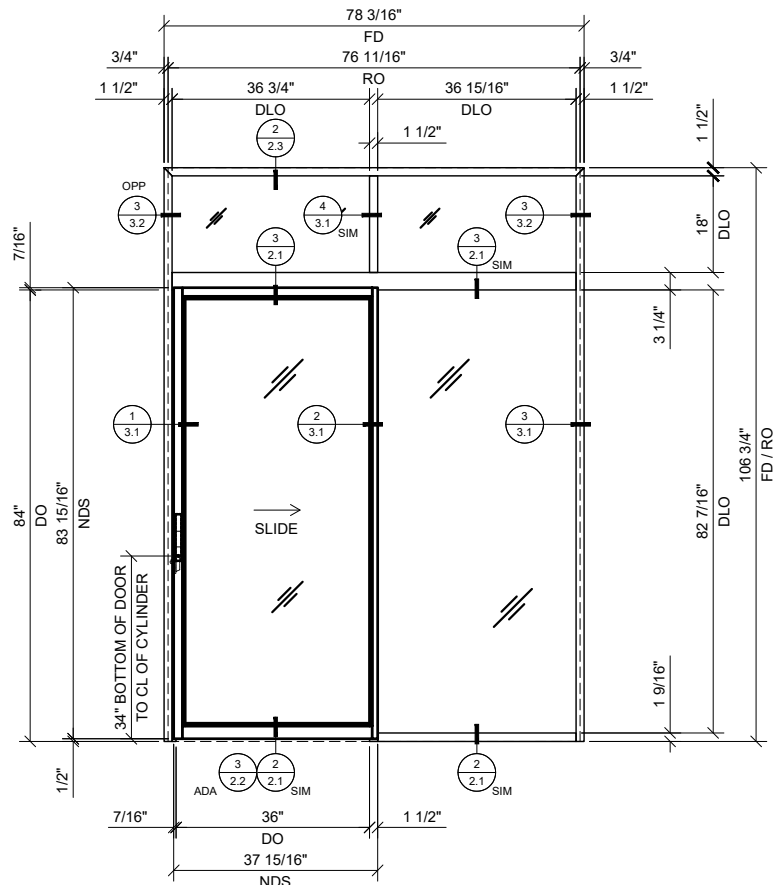
2 SINGLE SLIDER WITH BAY & TRANSOM
