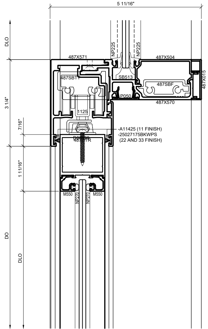
3 TRANSOM DETAIL AT SLIDER DOOR OPENING 1'-0"=1'-0" ARCH REF: N/A
