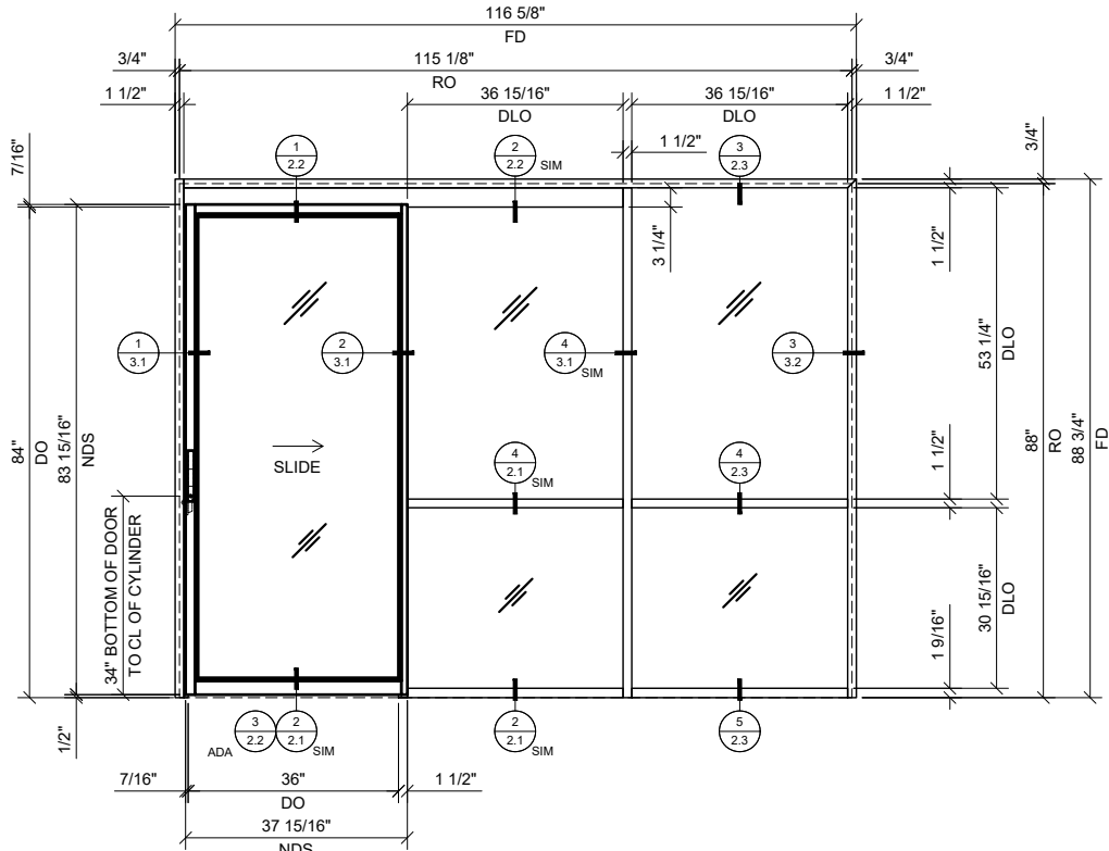
1 SINGLE SLIDER WITH BAY & SIDELITE
