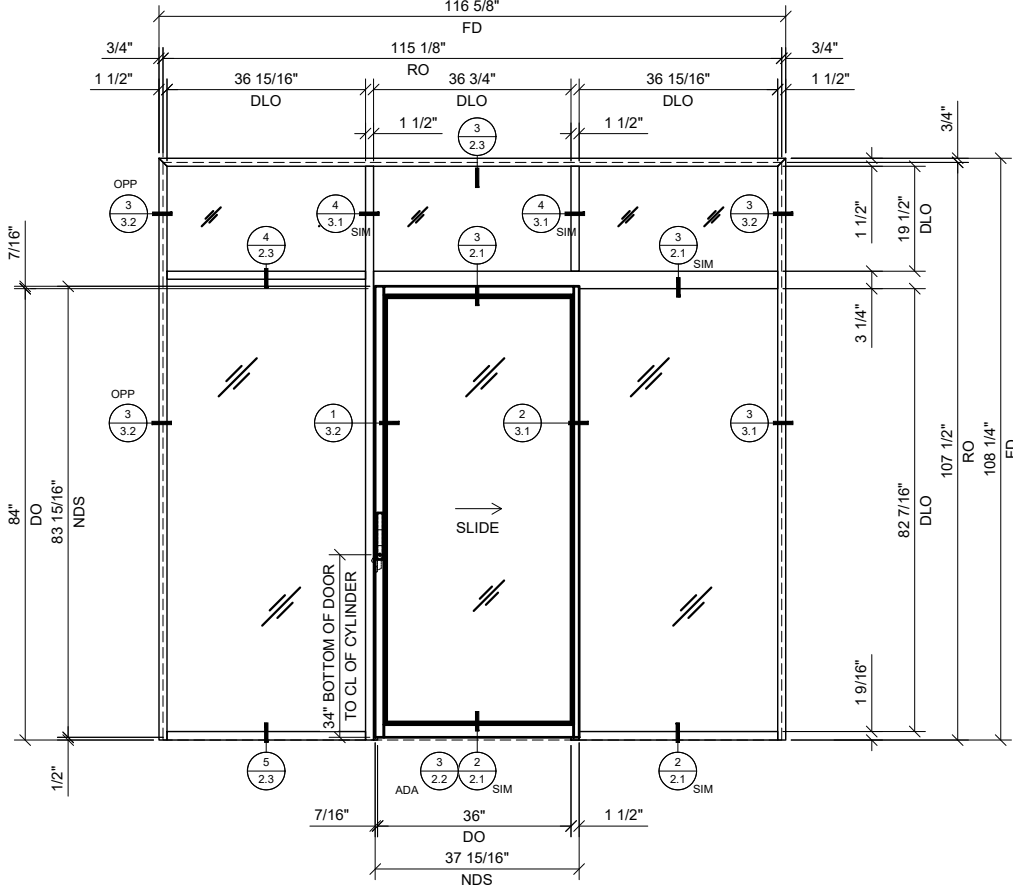
4 SINGLE SLIDER WITH BAY, TRANSOM & SIDELITE
