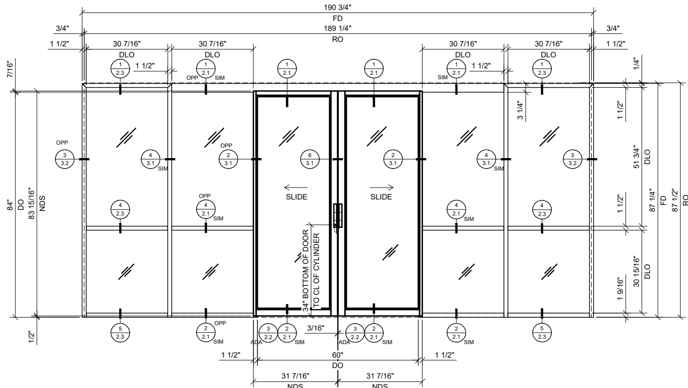
③ BI-PART SLIDER WITH BAYS & SIDELITES AT EACH END 3/4"=1'-0" ARCH REF: N/A
