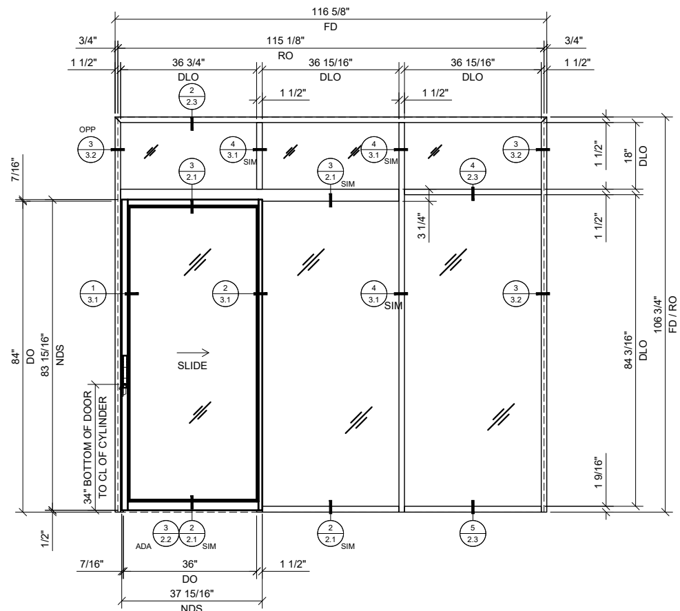
2 SINGLE SLIDER WITH BAY, TRANSOM & SIDELITE
