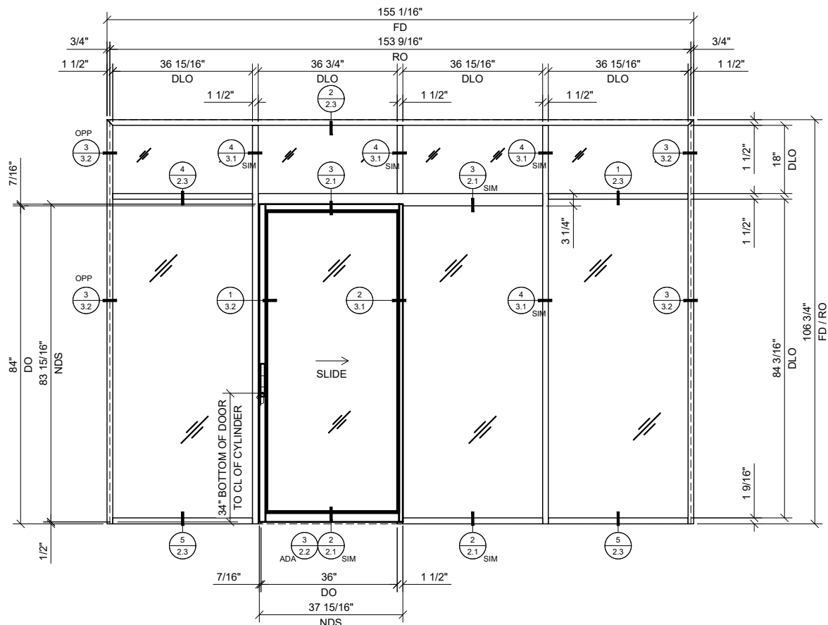
4 SINGLE SLIDER WITH BAY, TRANSOM & SIDELITE AT EACH END
