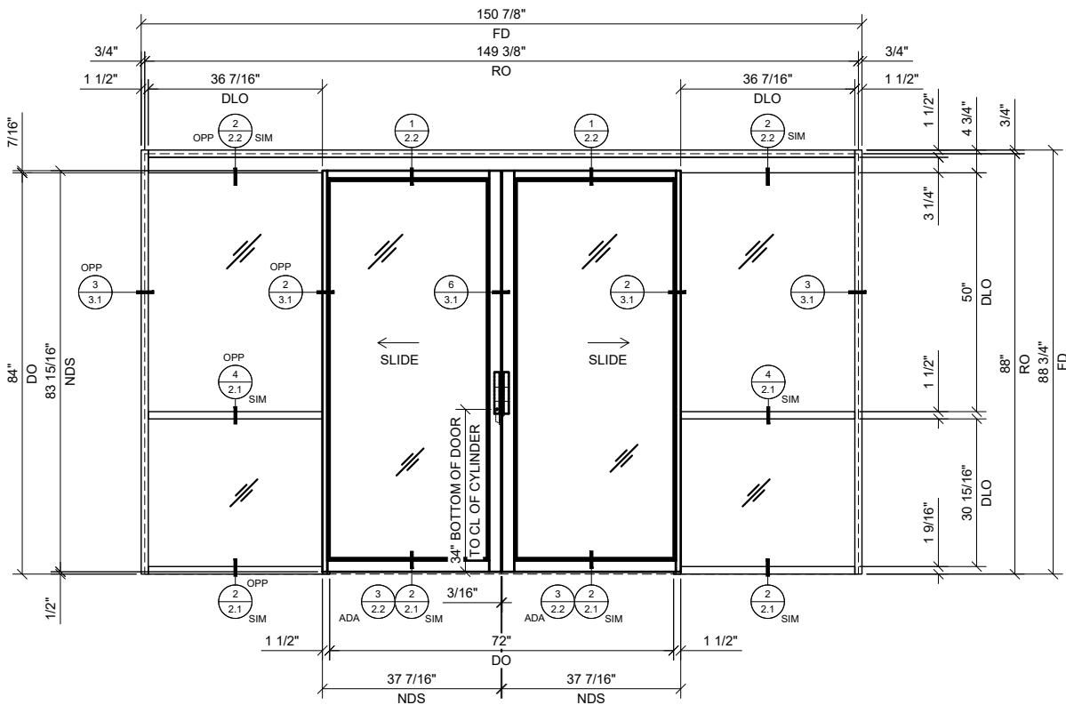
① BI-PART SLIDER WITH BAYS
