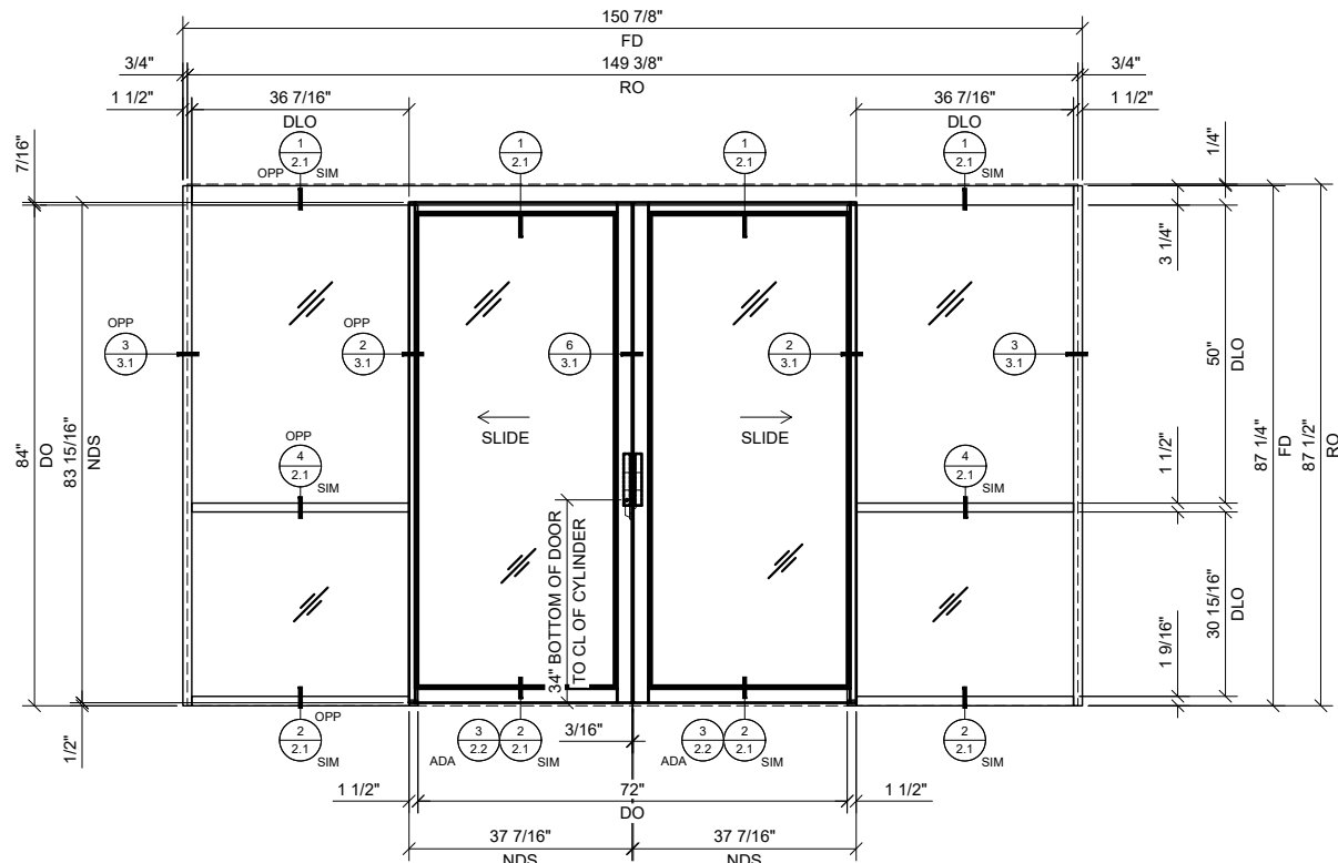
① BI-PART SLIDER WITH BAYS 3/4"=1'-0" ARCH REF: N/A
