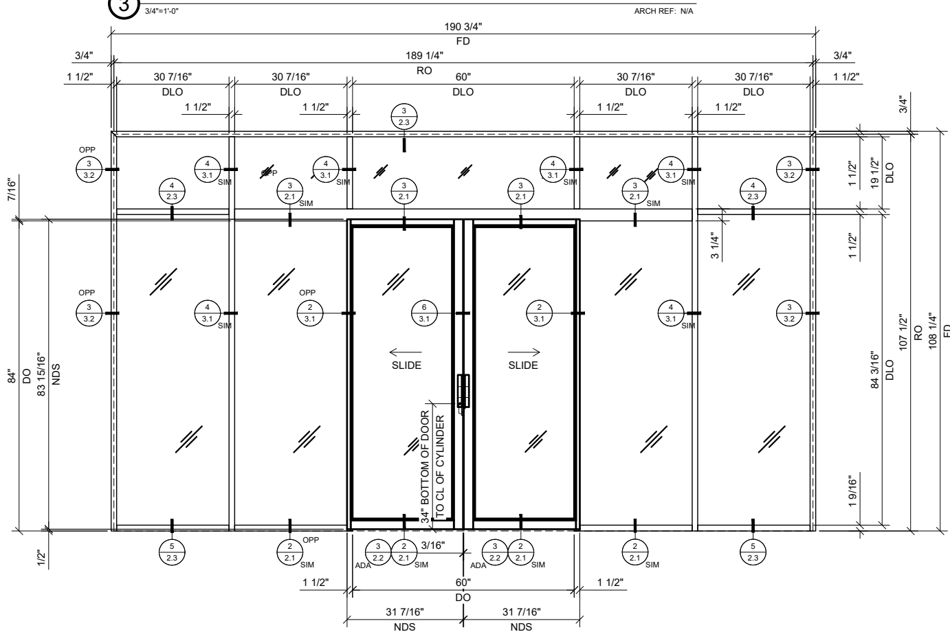
④ BI-PART SLIDER WITH BAYS, TRANSOM & SIDELITE AT EACH END
