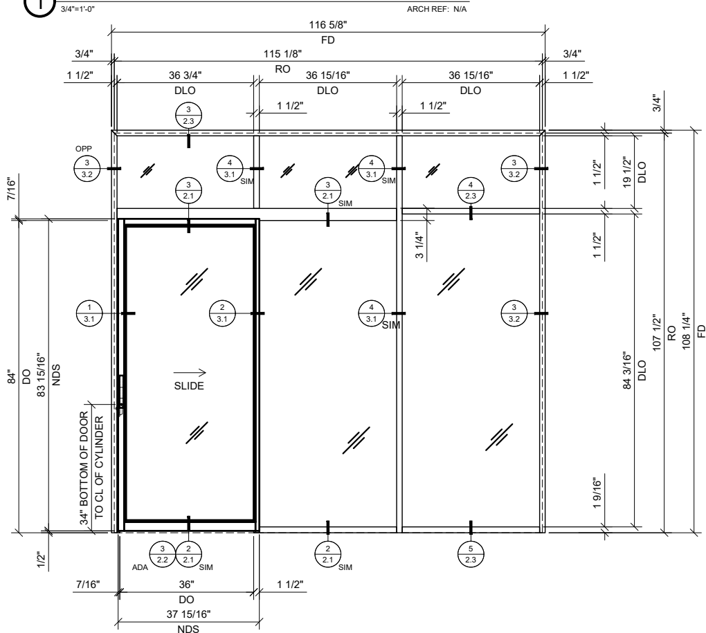
2 SINGLE SLIDER WITH BAY, TRANSOM & SIDELITE
