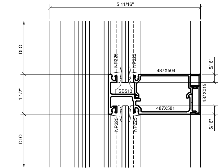
4 MUNTIN AT SLIDER BAY 1'-0"=1'-0" ARCH REF: N/A
