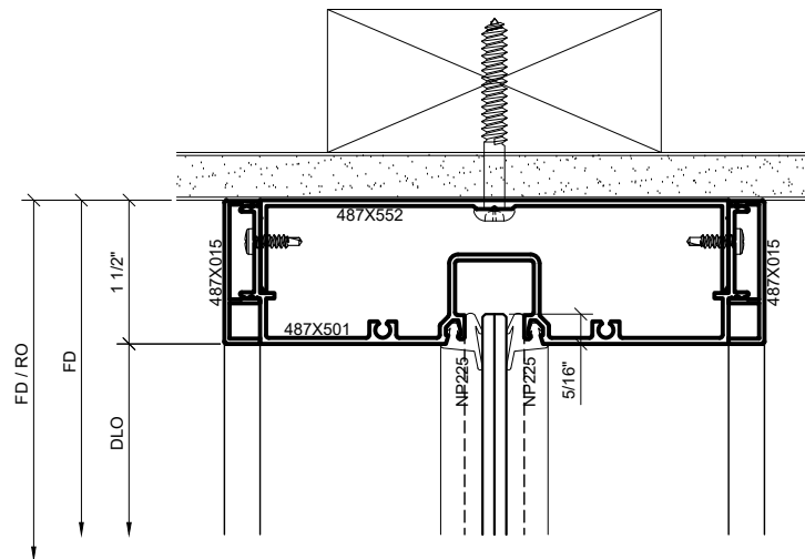
② SERIES 487 OPS SURFACE MOUNT HEAD DETAIL AT SIDELITE (NO SHIM) 1'-0\"=1'-0\" ARCH REF: N/A
