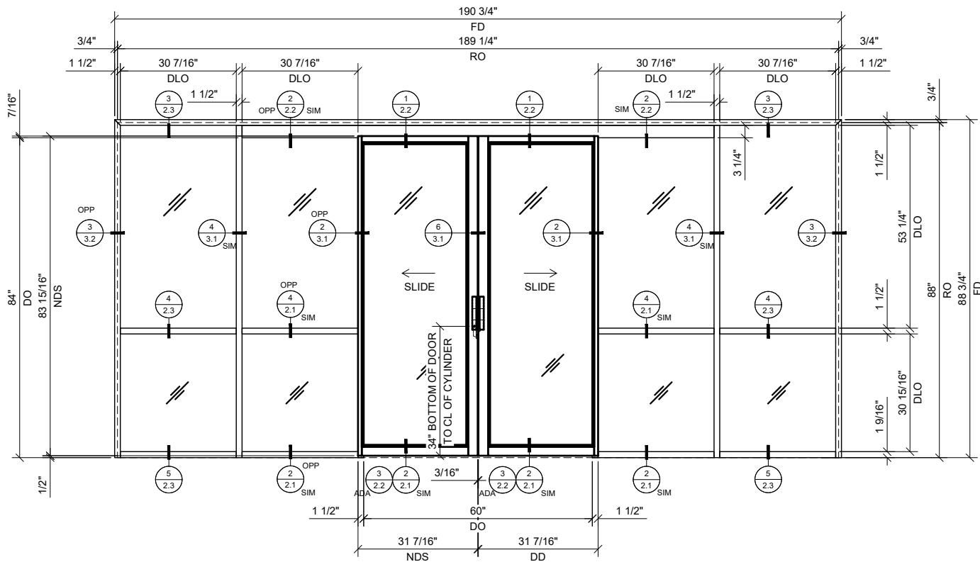
③ BI-PART SLIDER WITH BAYS & SIDELITE AT EACH END
