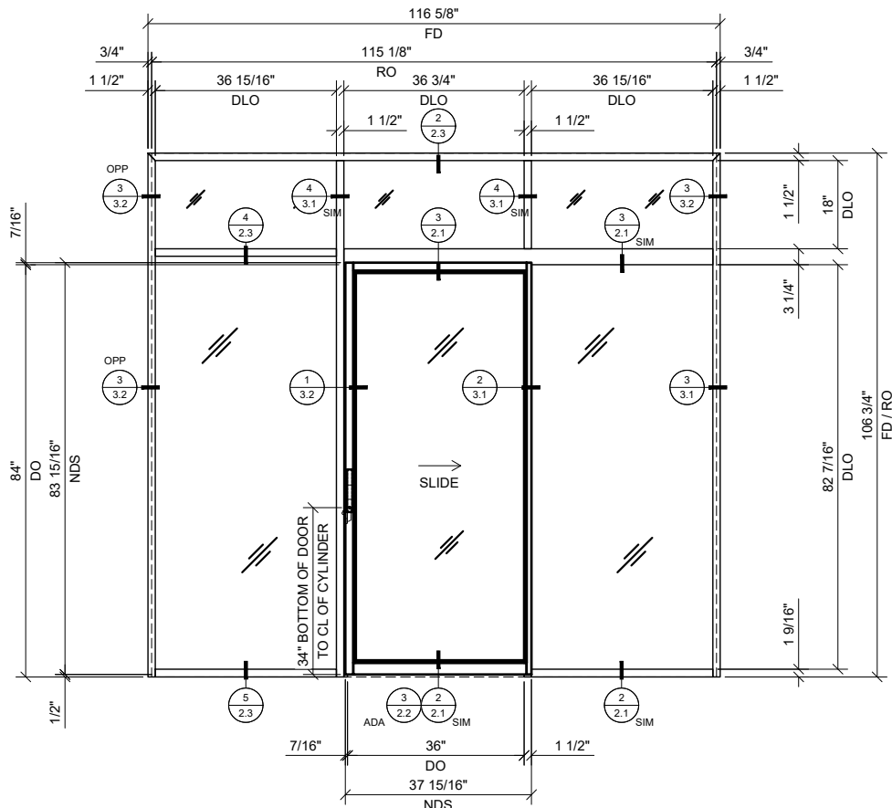
4 SINGLE SLIDER WITH BAY, TRANSOM & SIDELITE
