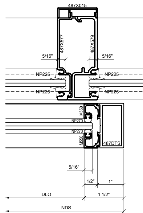
⑤ SERIES 487 OPS INTEGRATED SLIDER SHALLOW VERTICAL DETAIL (OPEN) 1'-0"=1'-0" ARCH REF: N/A
