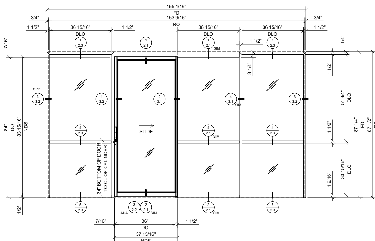
3 SINGLE SLIDER WITH BAY & SIDELITE AT BOTH ENDS
