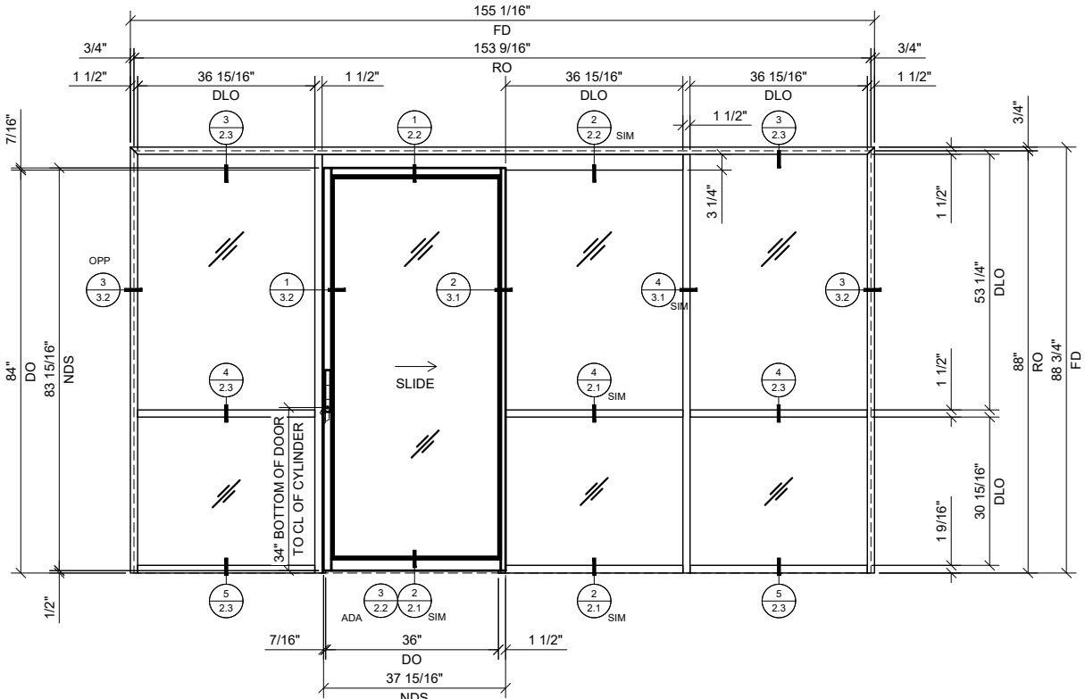
3 SINGLE SLIDER WITH BAY & SIDELITE AT EACH END
