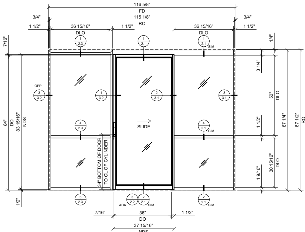
3 SINGLE SLIDER WITH BAY & SIDELITE
