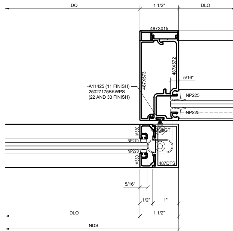
② SERIES 487 OPS INTEGRATED SLIDER INTERMEDIATE JAMB DETAIL (CLOSED) 1'-0"=1'-0" ARCH REF: N/A
