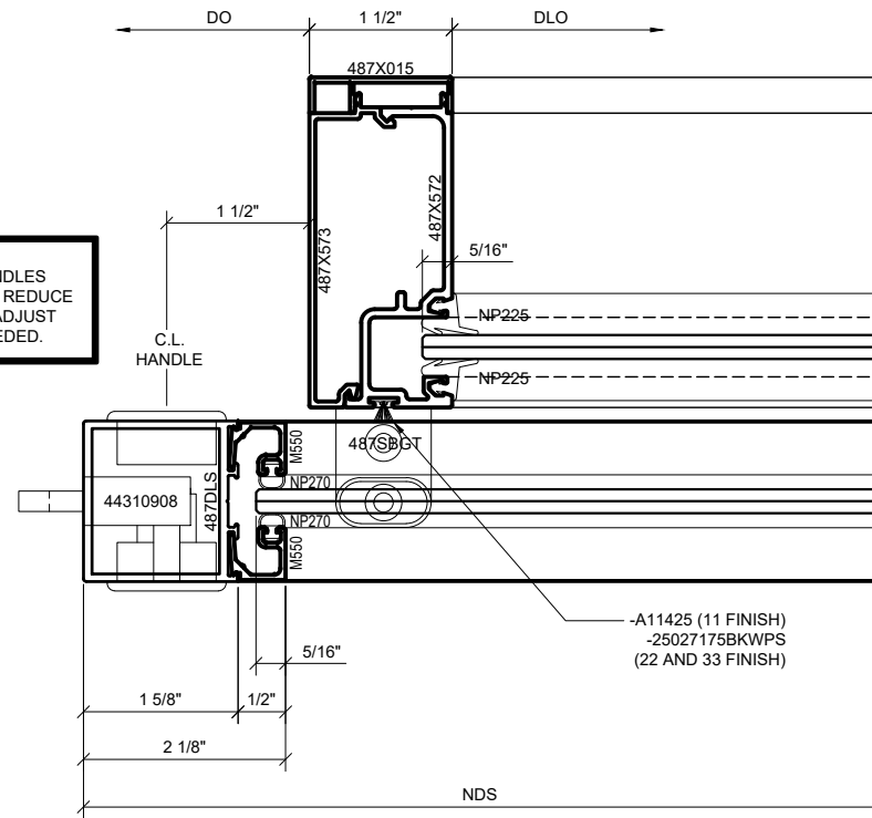
2 SERIES 487 OPS INTEGRATED SLIDER TRANSITION VERTICAL-STANDARD TO INTERMEDIATE JAMB DETAIL (OPEN)
