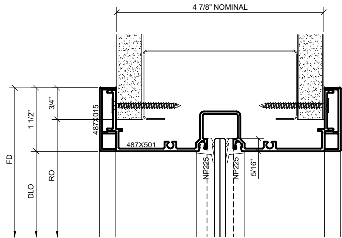
③ SERIES 487 OPS TRANSOM HEAD DETAIL AT INT. VERTICAL 1'-0\"=1'-0\" ARCH REF: N/A
