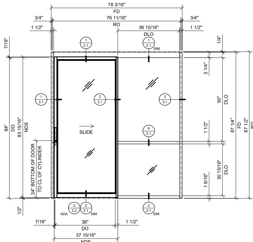
1 SINGLE SLIDER WITH BAY
