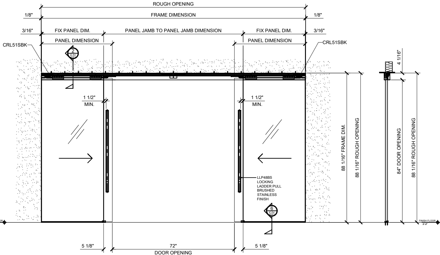
②A CRL 512 CS2 BI-PARTING w/ 2 FIXED PANELS SYNC. CEILING MOUNT ~ DOOR OPENED ARCH REF: NONE 3/4"=1'-0"
