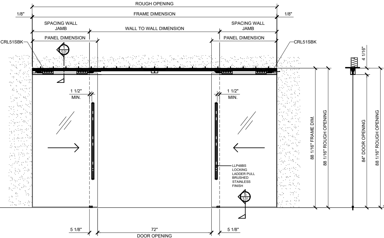
①A CRL 51 CS2 BI-PARTING SYNC. CEILING MOUNT ~ DOOR OPENED ARCH REF: NONE 3/4"=1'-0"
