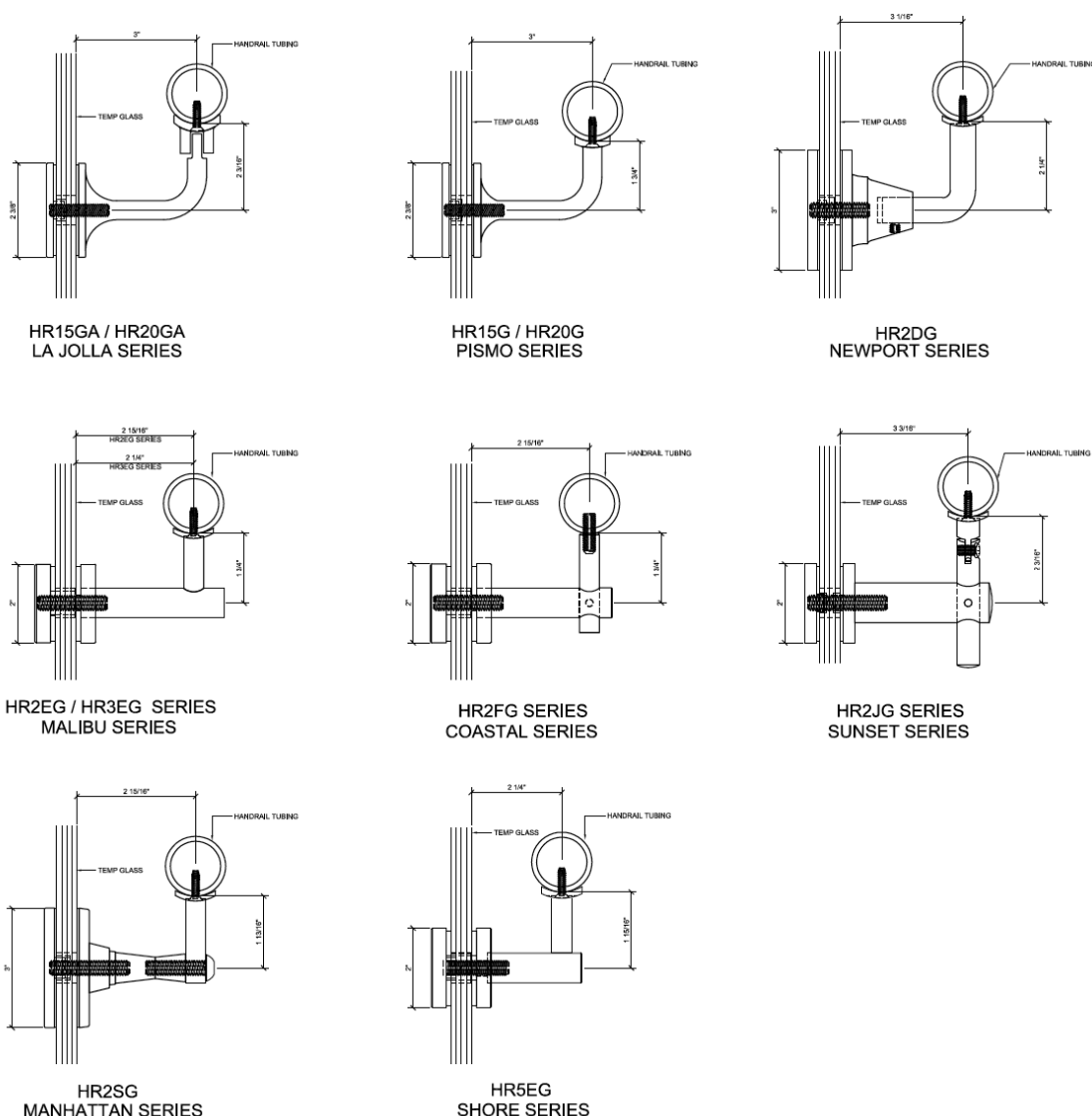
FIGURE 10—HANDRAIL BRACKETS
