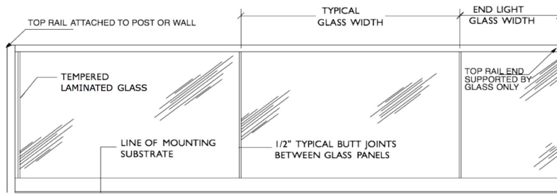
FIGURE 5—TOP RAIL SUPPORT OPTIONS
