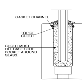
FIGURE 6—WET GLAZING
